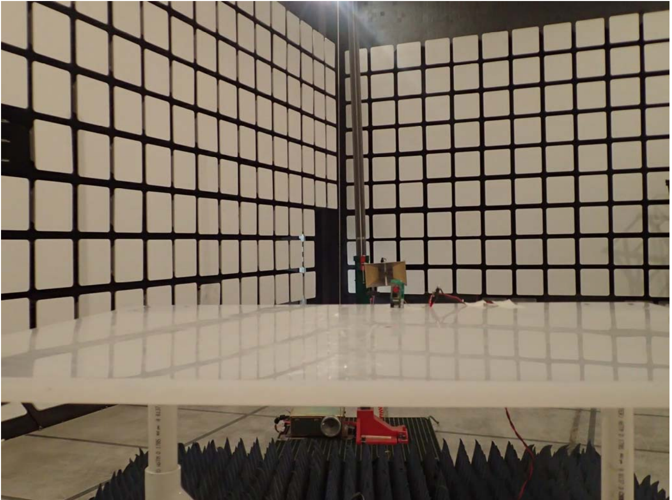
Radiated Emissions @ 3 m, Above 1 GHz, Orthogonal Position 3
