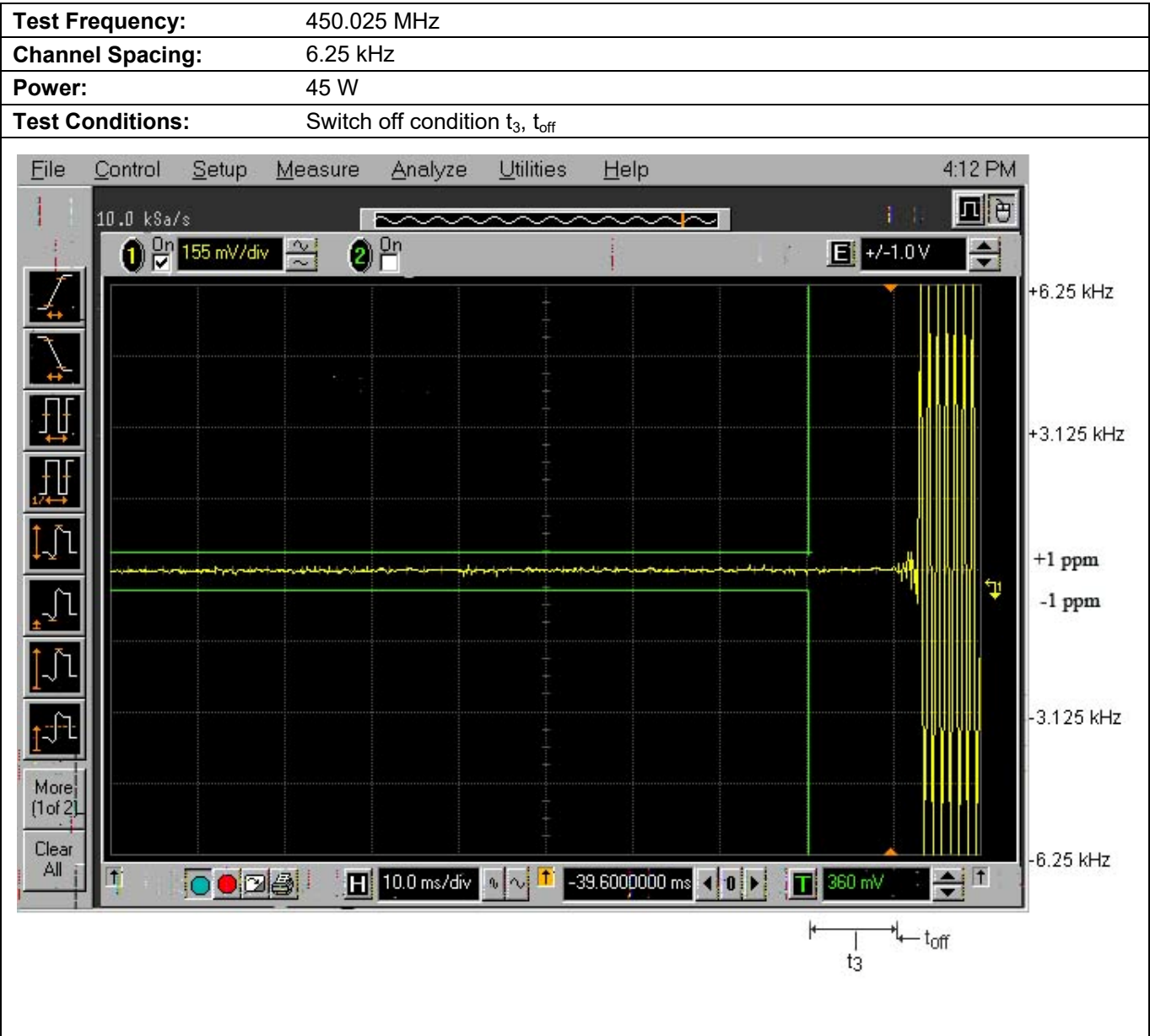
Plot 5.10.4.2. Transient Frequency Behavior for 6.25 kHz Channel Spacing
