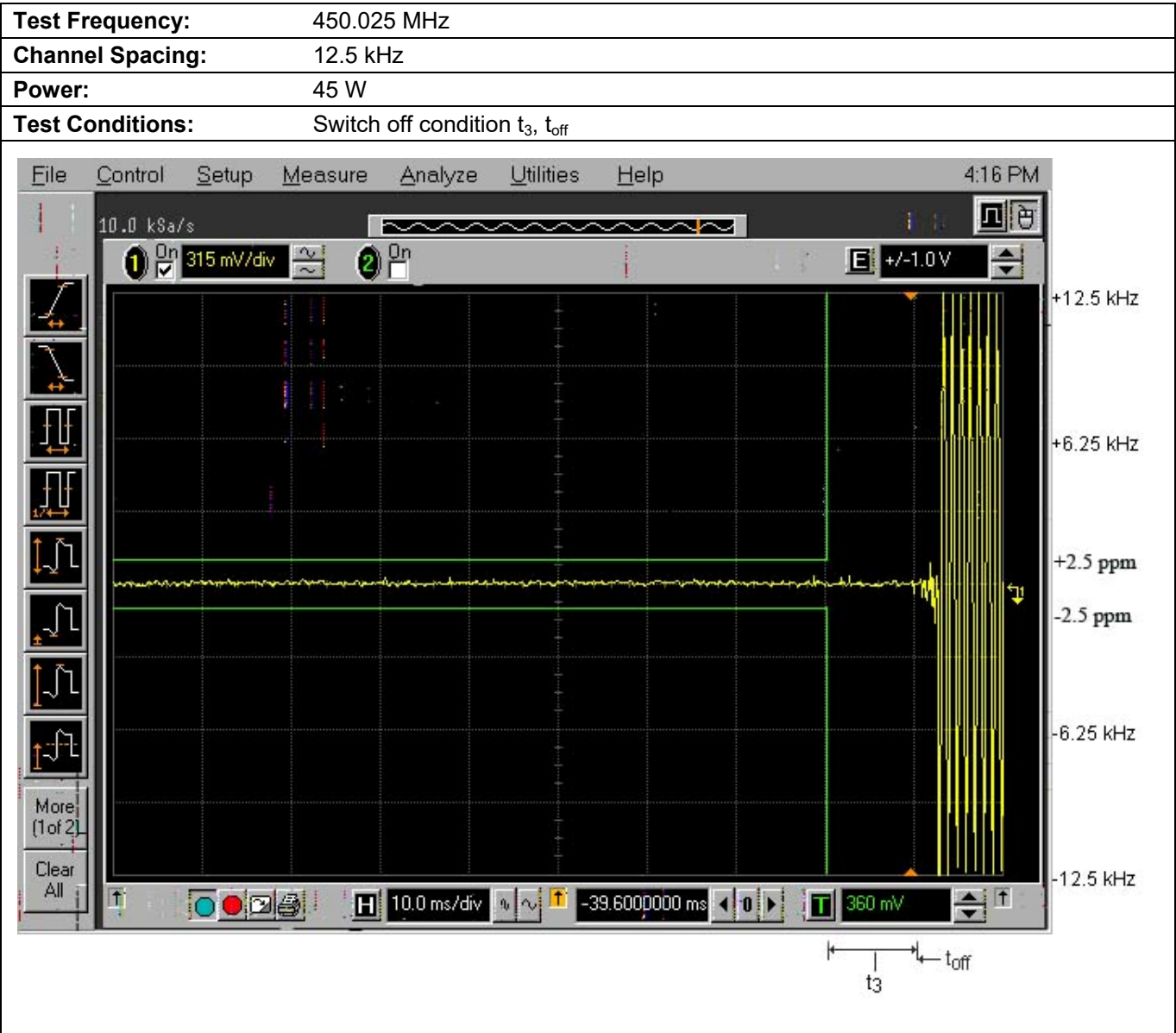
Plot 5.10.4.4. Transient Frequency Behavior for 12.5 kHz Channel Spacing
