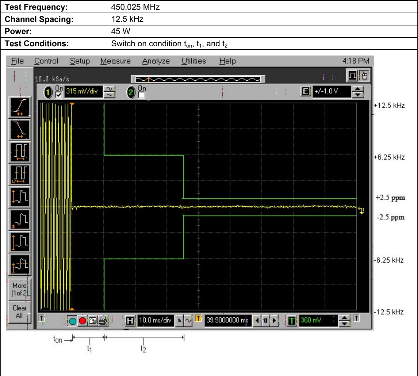
Plot 5.10.4.3. Transient Frequency Behavior for 12.5 kHz Channel Spacing
