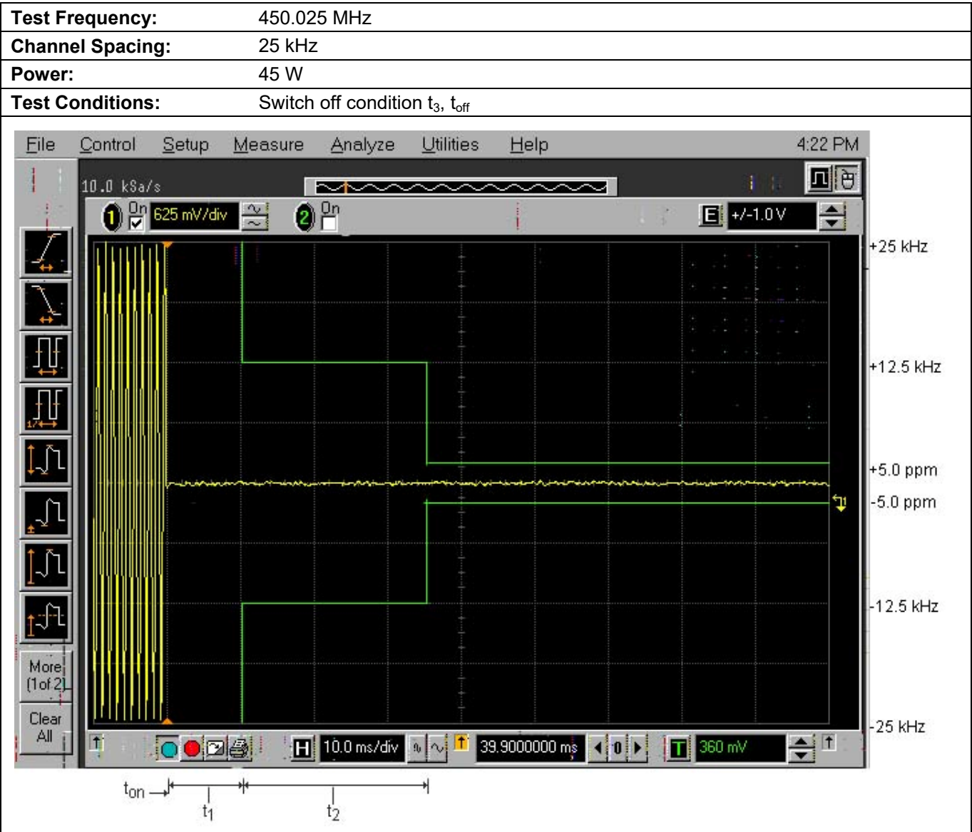
Plot 5.10.4.6. Transient Frequency Behavior for 25 kHz Channel Spacing
