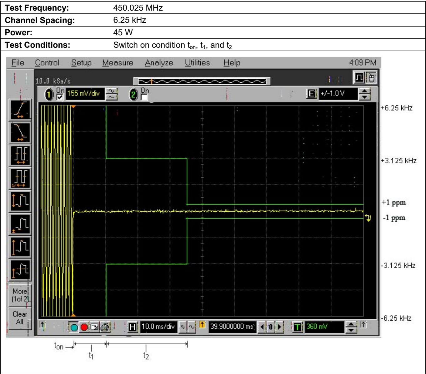
Plot 5.10.4.1. Transient Frequency Behavior for 6.25 kHz Channel Spacing
