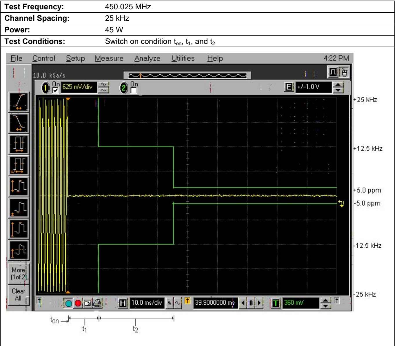
Plot 5.10.4.5. Transient Frequency Behavior for 25 kHz Channel Spacing
