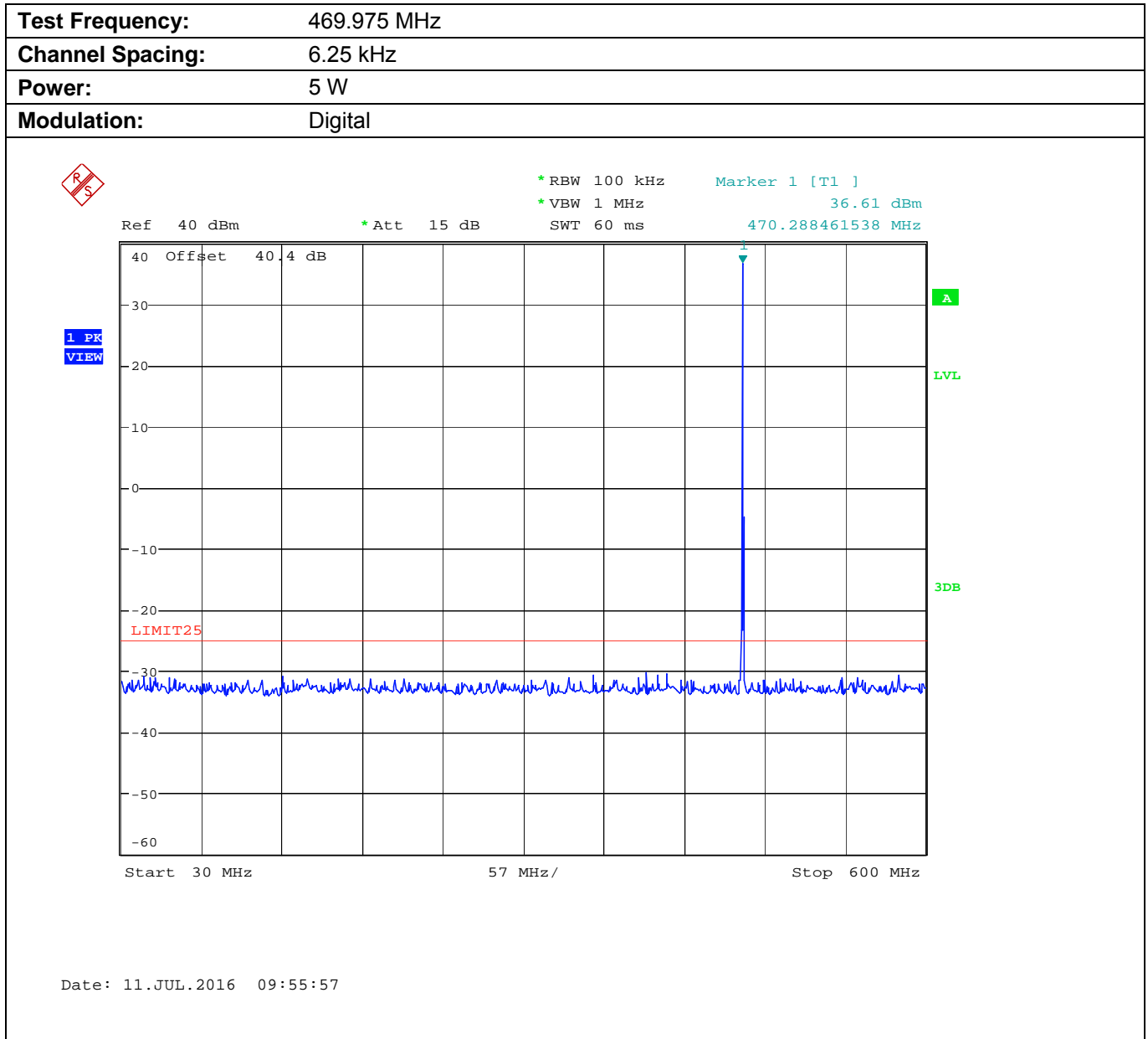
Plot 5.9.4.3.4. Conducted Transmitter Spurious Emissions for 469.975 MHz, Low Power, 30 MHz - 600 MHz
