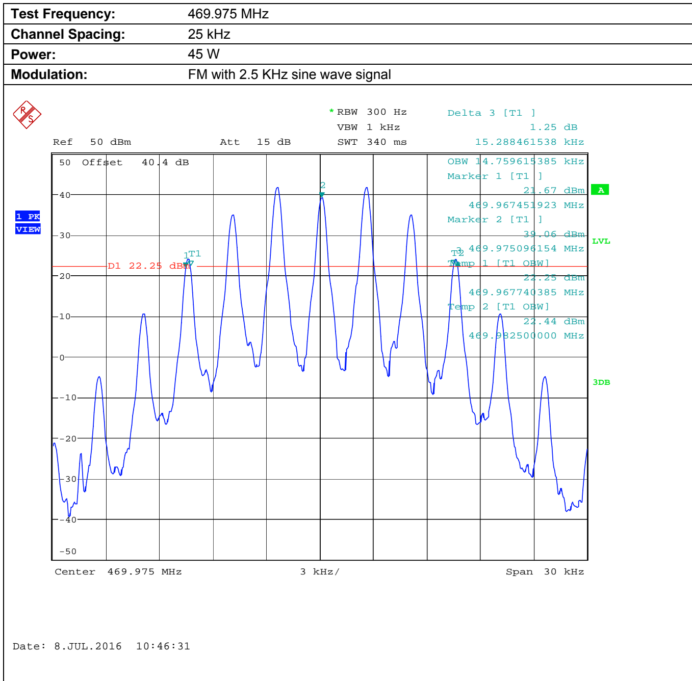
Plot 5.8.4.1.3. Occupied Bandwidth
