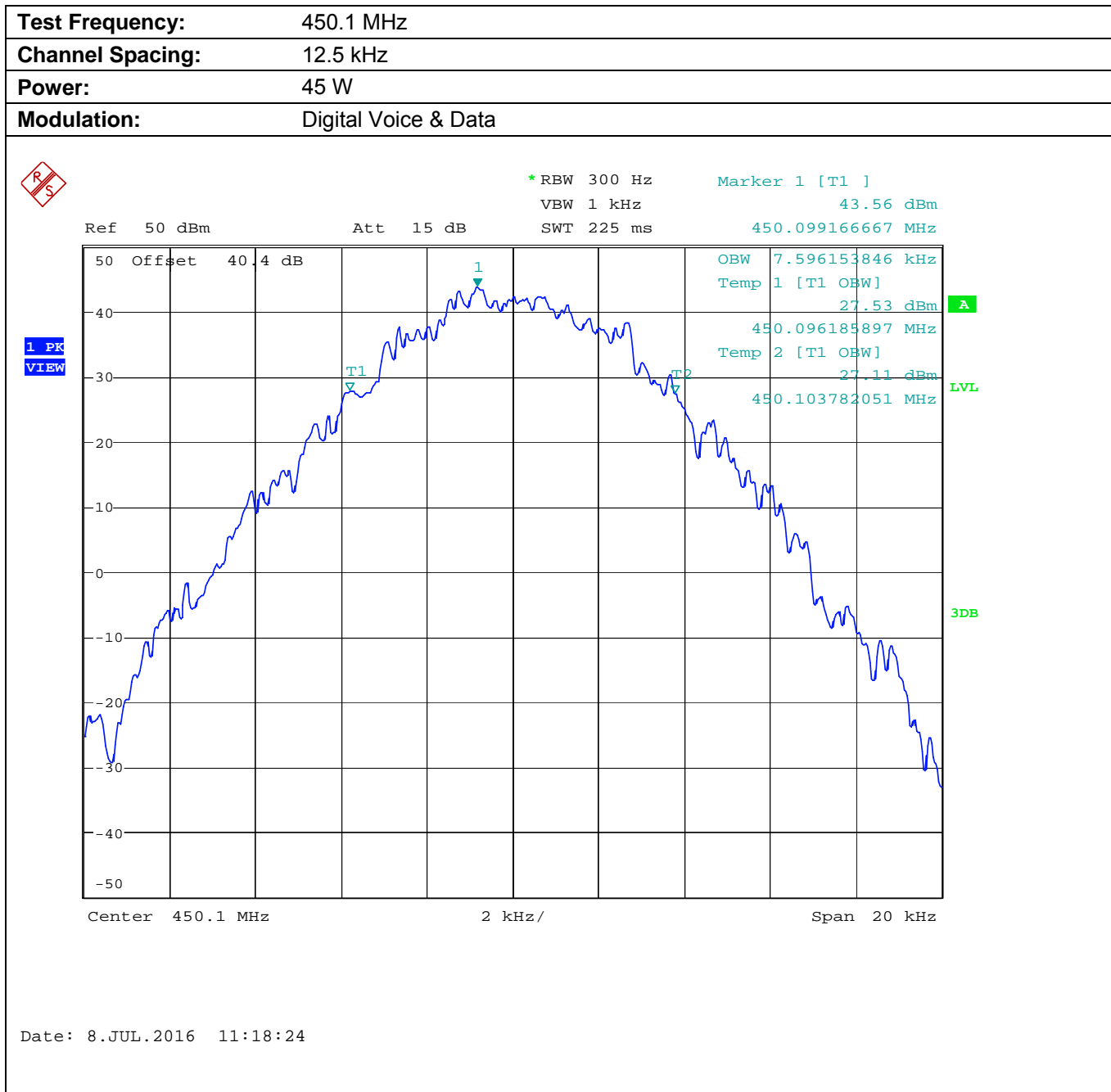
Plot 5.8.4.1.8. Occupied Bandwidth
