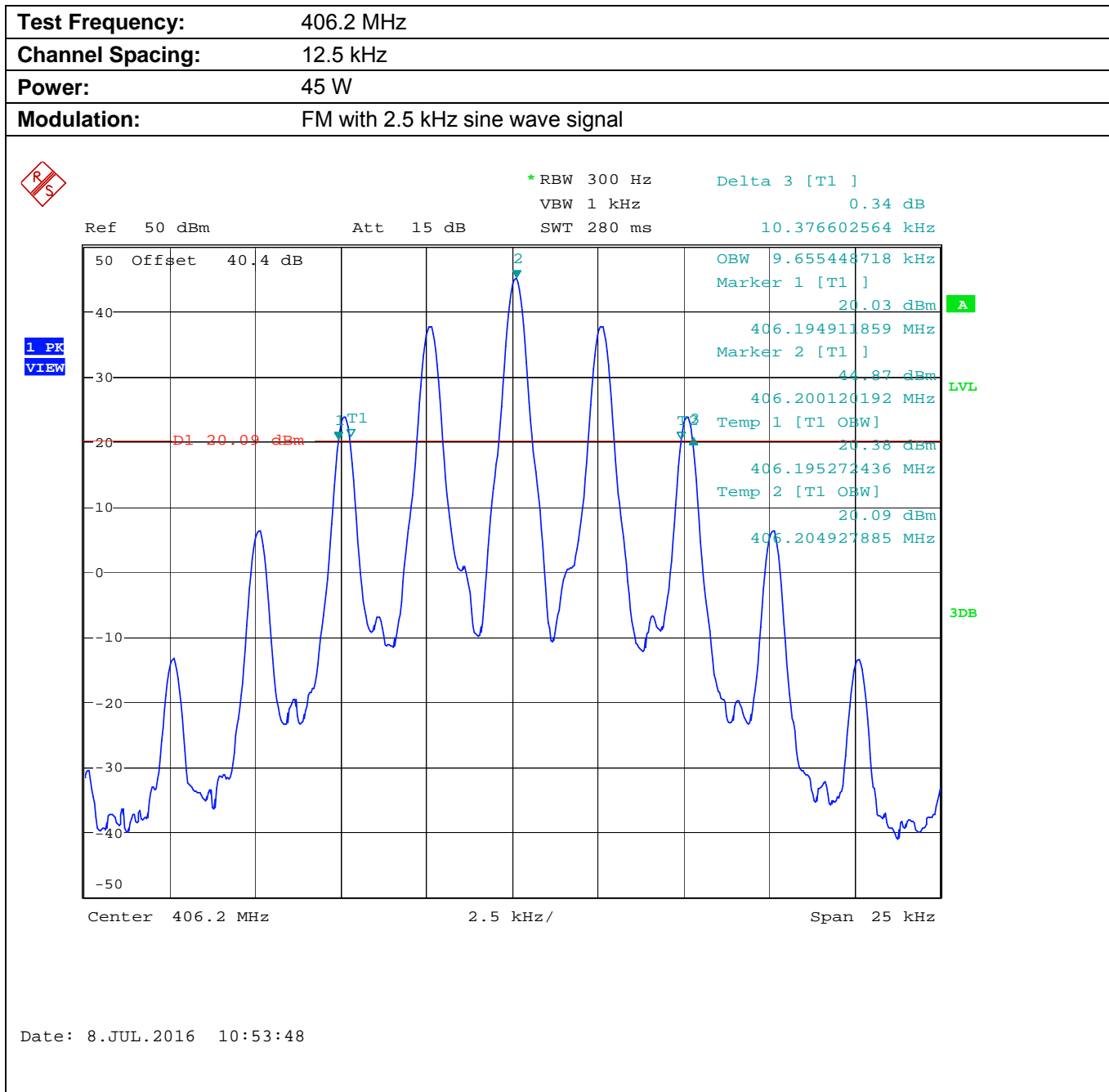
Plot 5.8.4.1.4. Occupied Bandwidth
