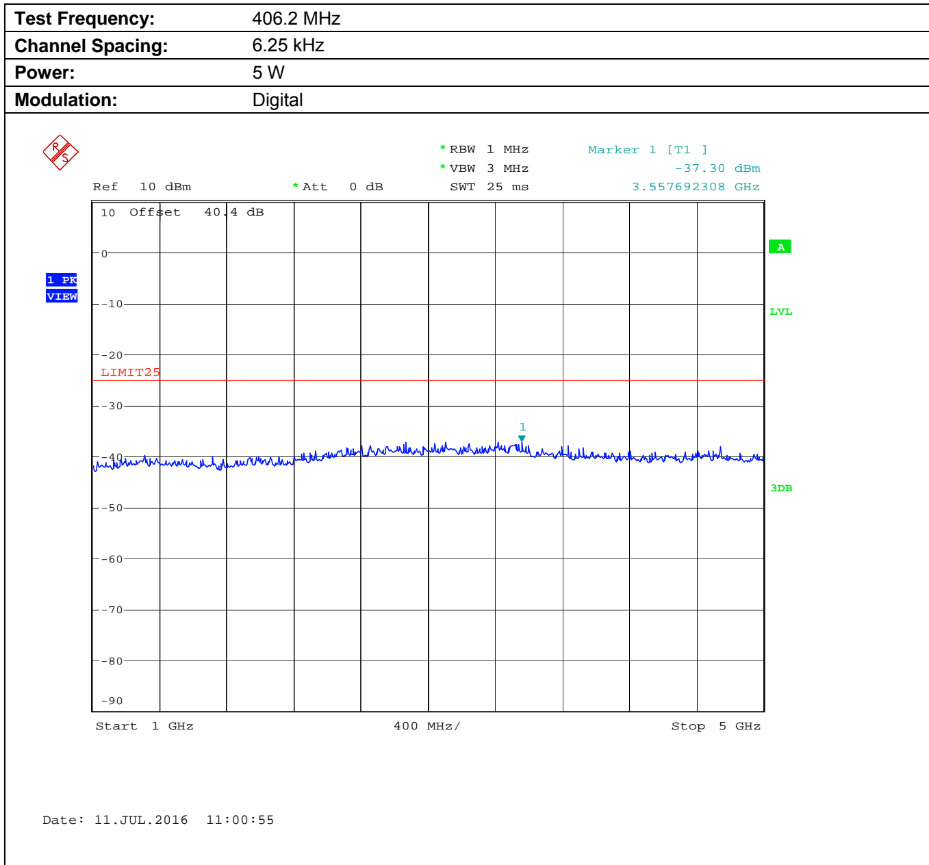
Plot 5.9.4.1.6. Conducted Transmitter Spurious Emissions for 406.2 MHz, Low Power, 1 - 5 GHz
