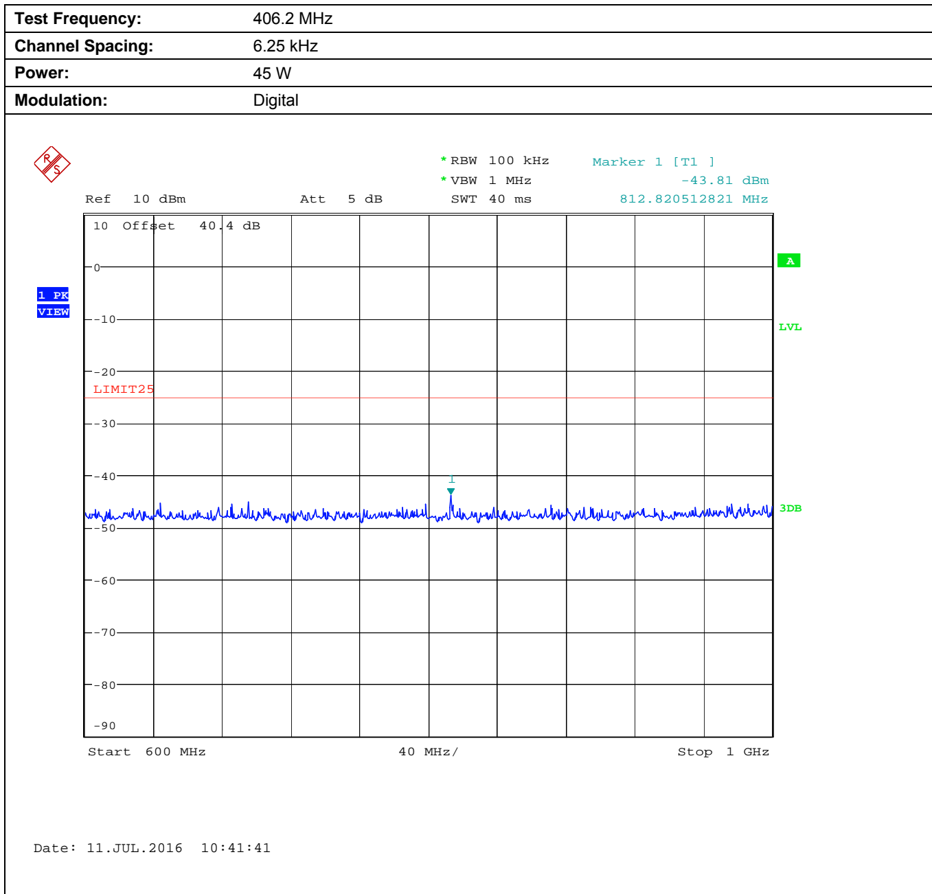
Plot 5.9.4.1.2. Conducted Transmitter Spurious Emissions for 406.2 MHz, High Power, 600 MHz - 1 GHz
