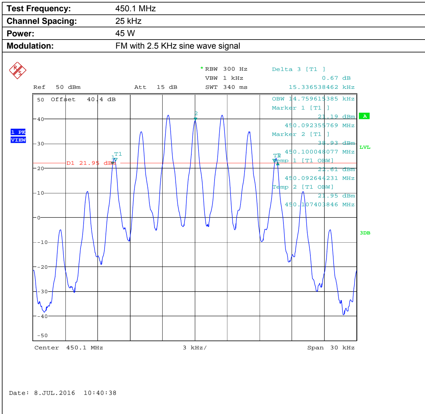
Plot 5.8.4.1.2. Occupied Bandwidth
