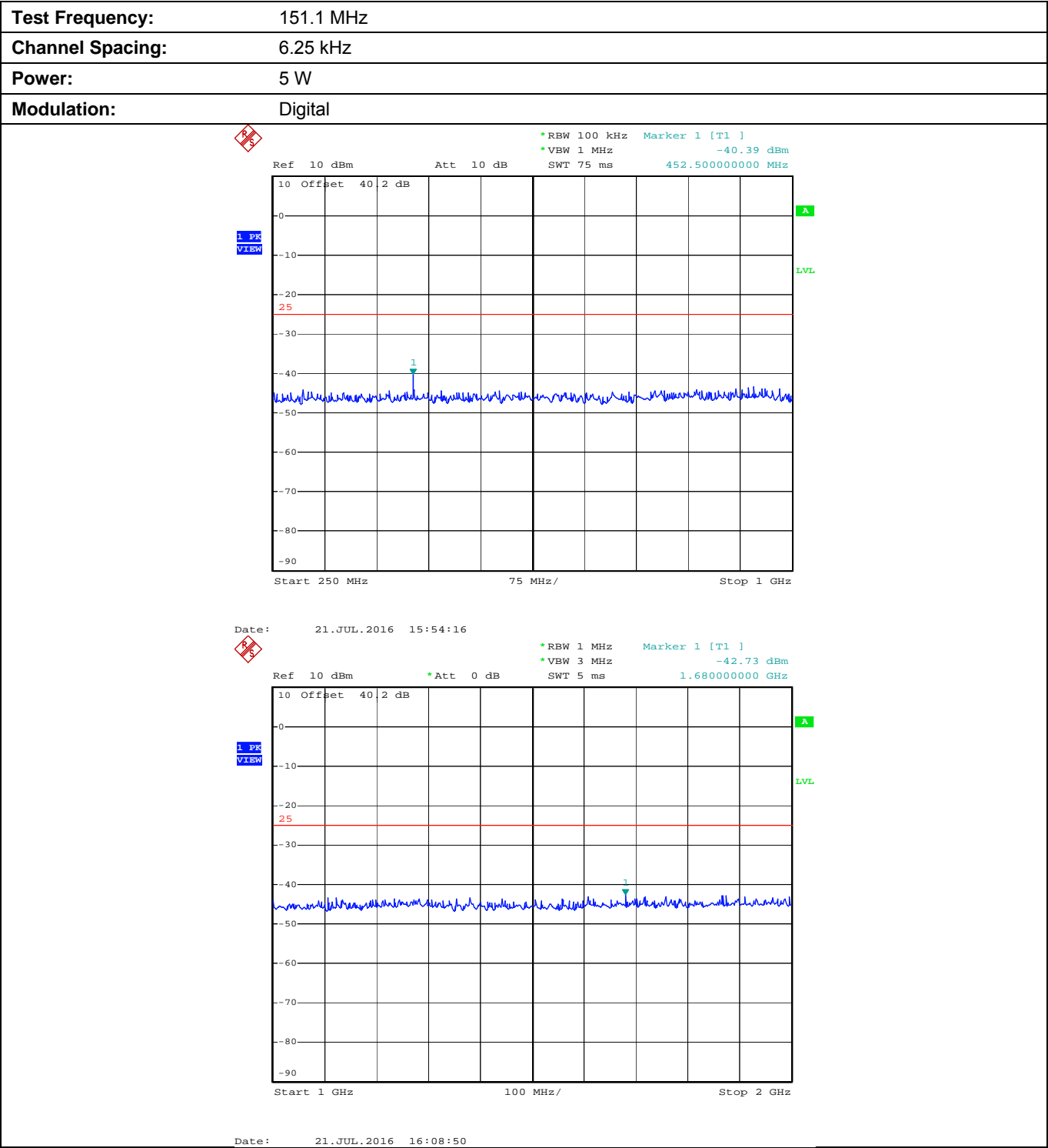
Plot 5.9.4.2.4. Conducted Transmitter Spurious Emissions for 151.1 MHz, Low Power, 250 MHz - 2 GHz
