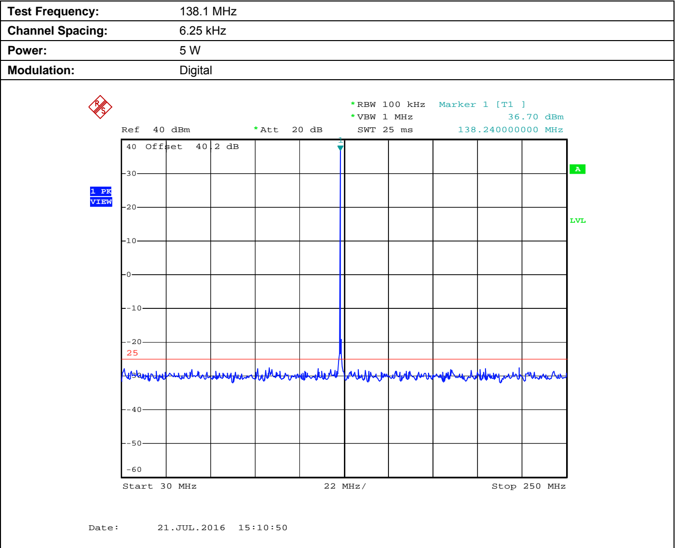
Plot 5.9.4.1.3. Conducted Transmitter Spurious Emissions for 138.1 MHz, Low Power, 30 MHz - 250 MHz
