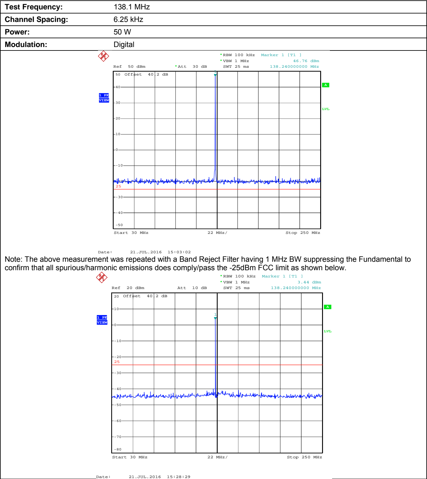
Plot 5.9.4.1.1. Conducted Transmitter Spurious Emissions for 138.1 MHz, High Power, 30 MHz - 250 MHz
