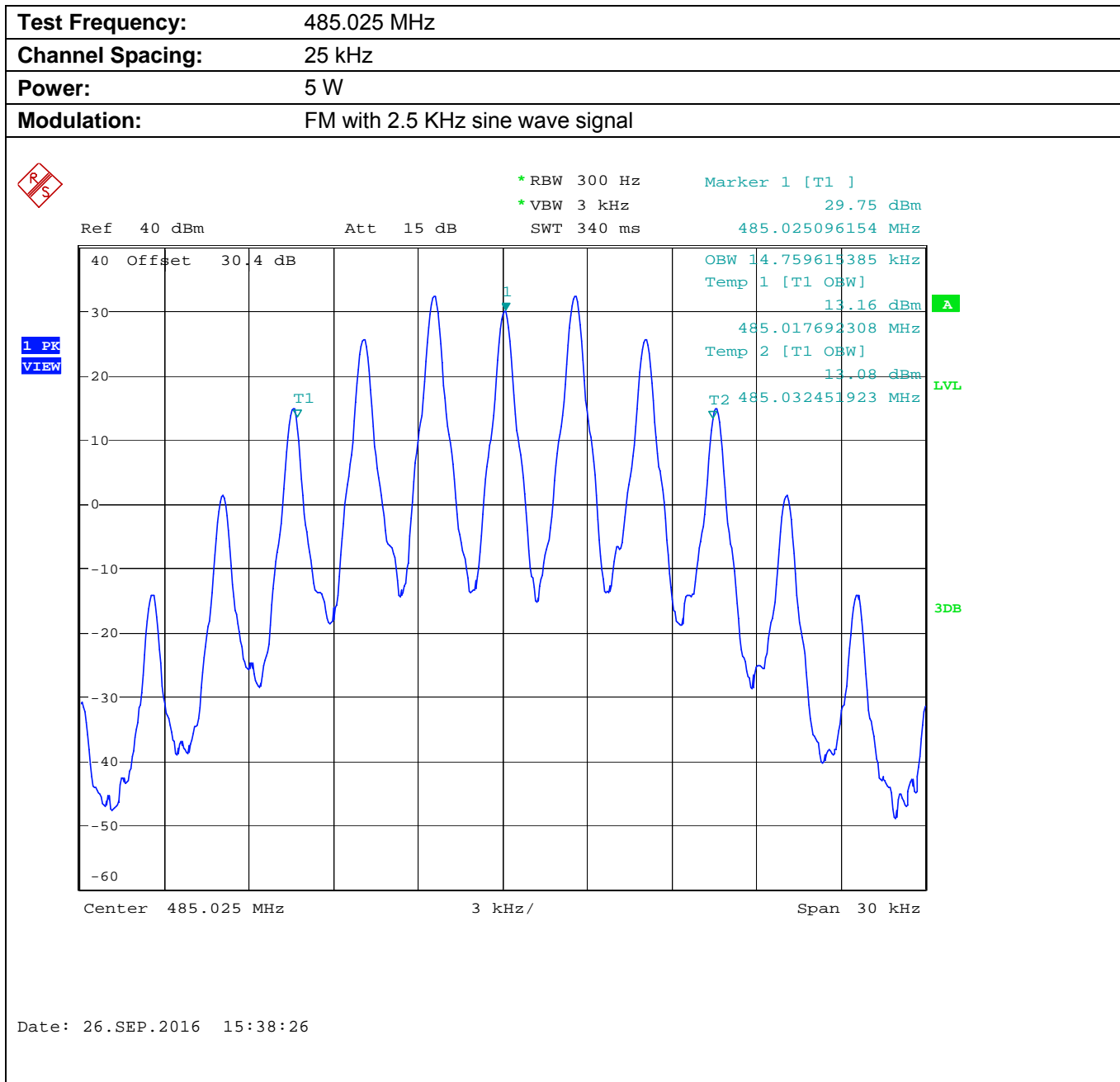
Plot 5.8.4.1.5. Occupied Bandwidth
