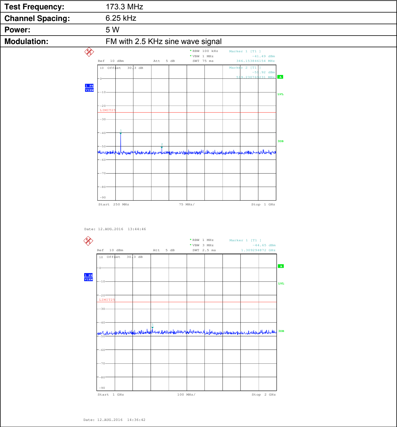
Plot 5.9.4.3.2. Conducted Transmitter Spurious Emissions for 173.3 MHz, High Power, 250 MHz - 2 GHz
