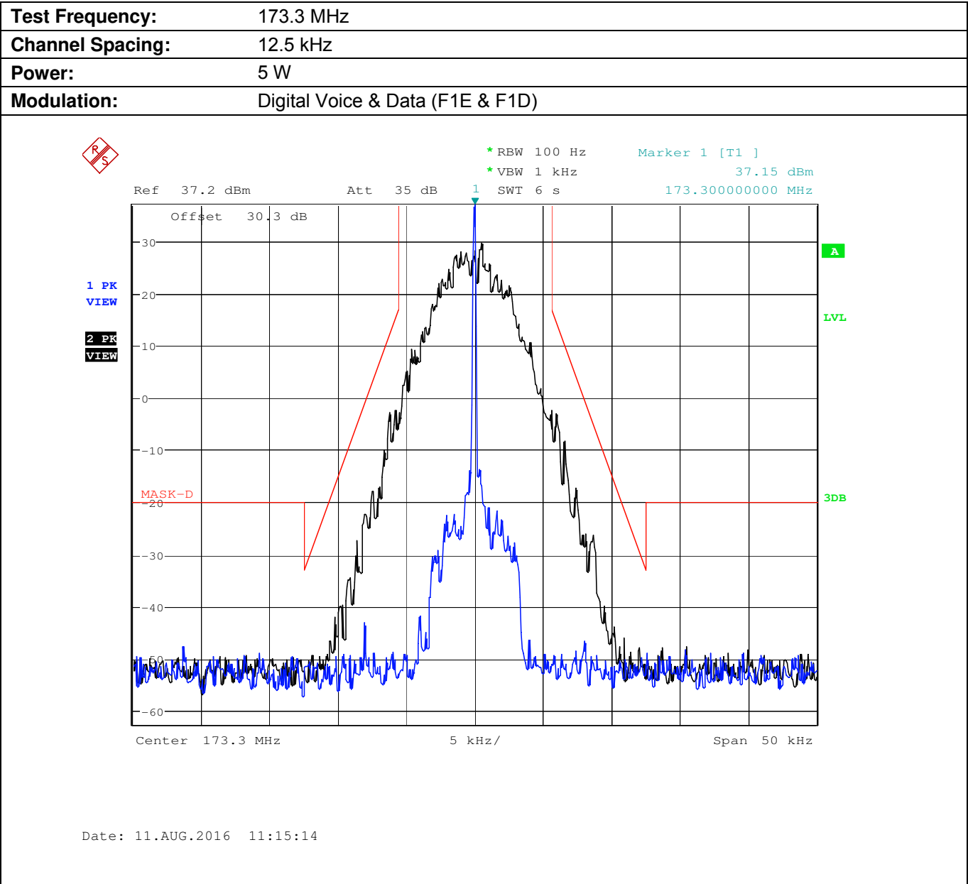
Plot 5.8.4.2.9. Emission Mask D, High Power
