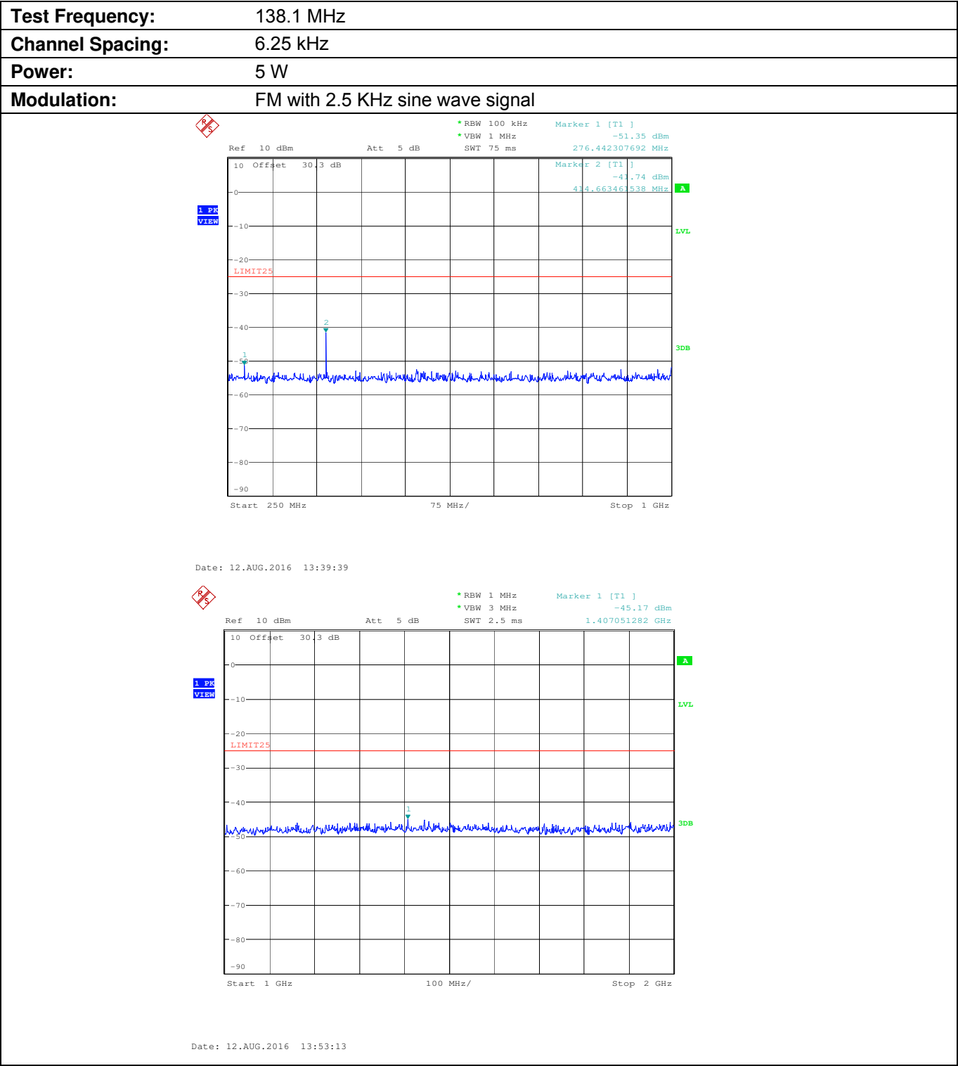
Plot 5.9.4.1.2. Conducted Transmitter Spurious Emissions for 138.1 MHz, High Power, 250 MHz - 2 GHz
