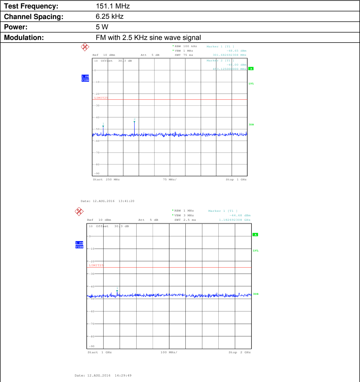
Plot 5.9.4.2.2. Conducted Transmitter Spurious Emissions for 151.1 MHz, High Power, 250 MHz - 2 GHz
