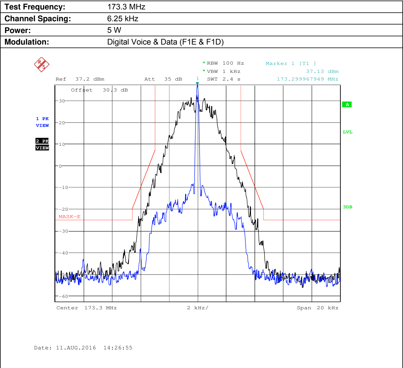
Plot 5.8.4.4.3. Emission Mask E, High Power
