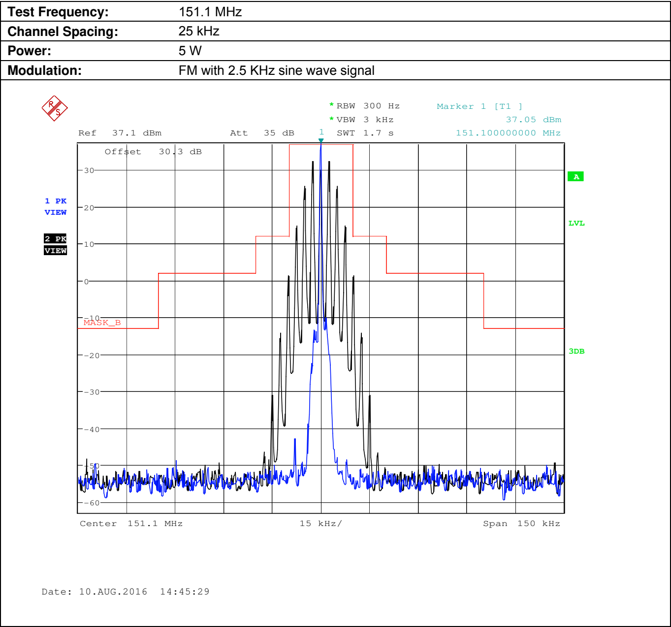
Plot 5.8.4.3.2. Emission Mask B, High Power
