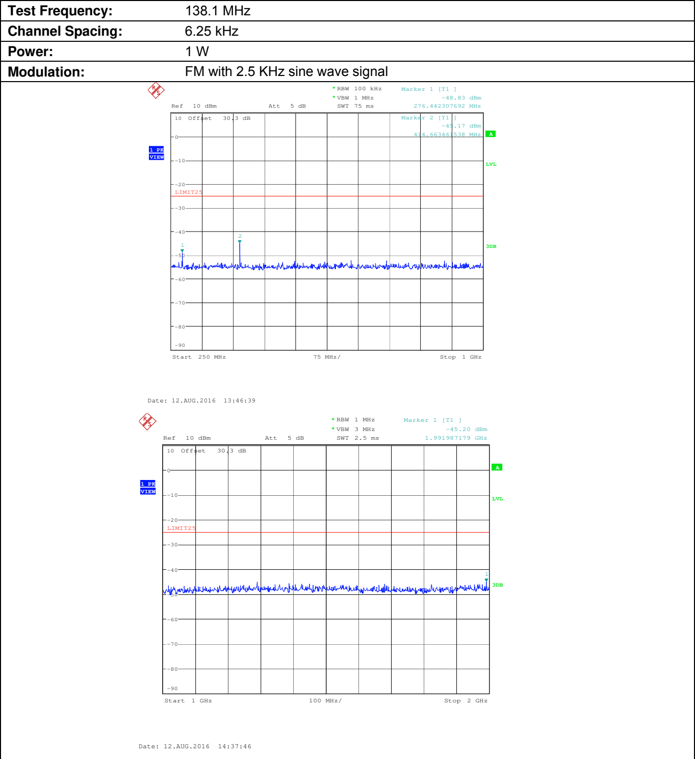
Plot 5.9.4.1.4. Conducted Transmitter Spurious Emissions for 138.1 MHz, Low Power, 250 MHz - 2 GHz
