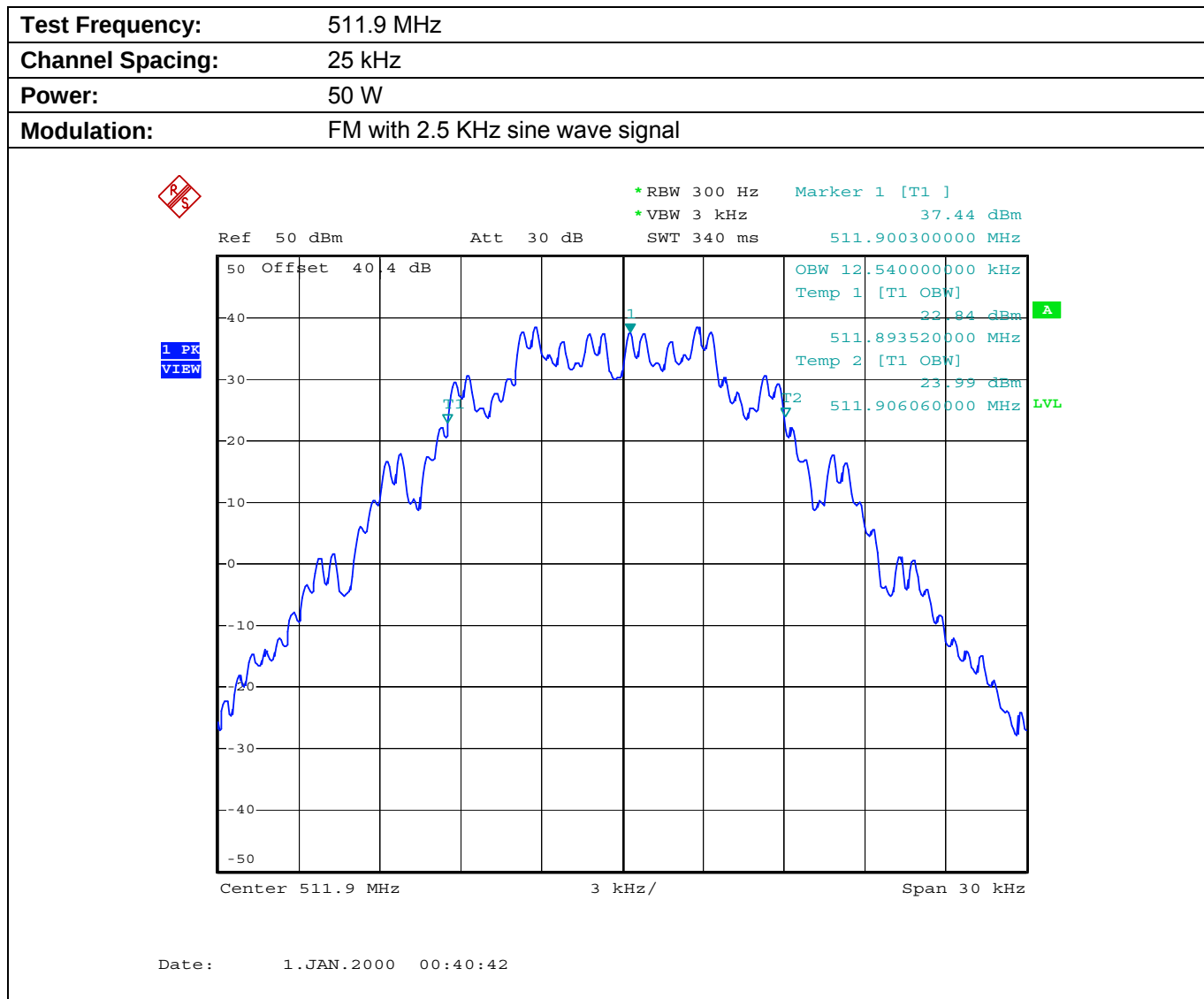
Plot 5.8.4.1.3. Occupied Bandwidth
