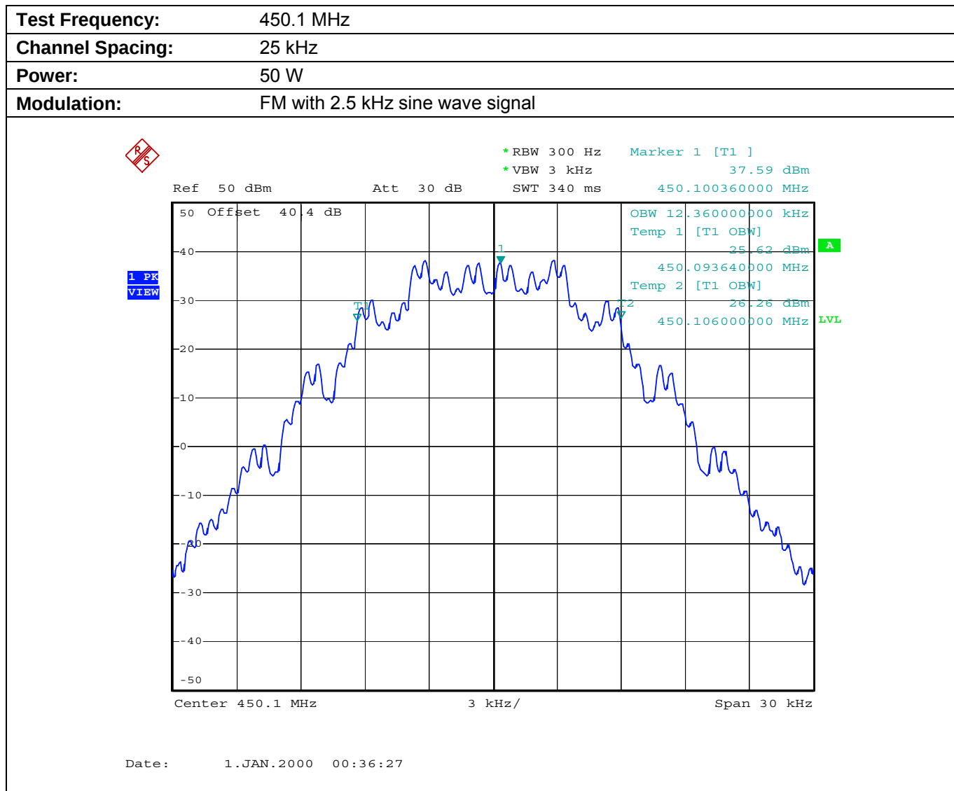
Plot 5.8.4.1.1. Occupied Bandwidth
