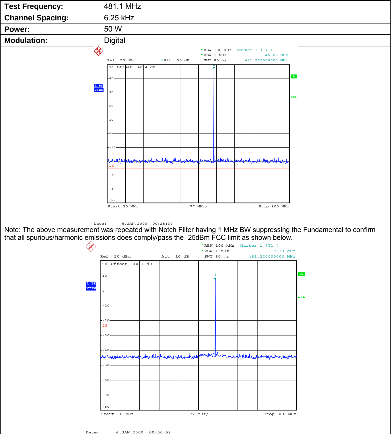
Plot 5.9.4.2.1. Conducted Transmitter Spurious Emissions for 481.1 MHz, High Power, 30 MHz - 800 MHz
