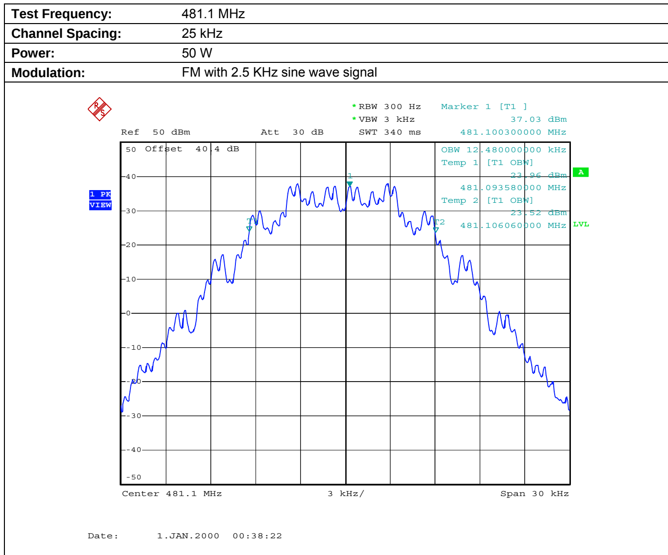
Plot 5.8.4.1.2. Occupied Bandwidth
