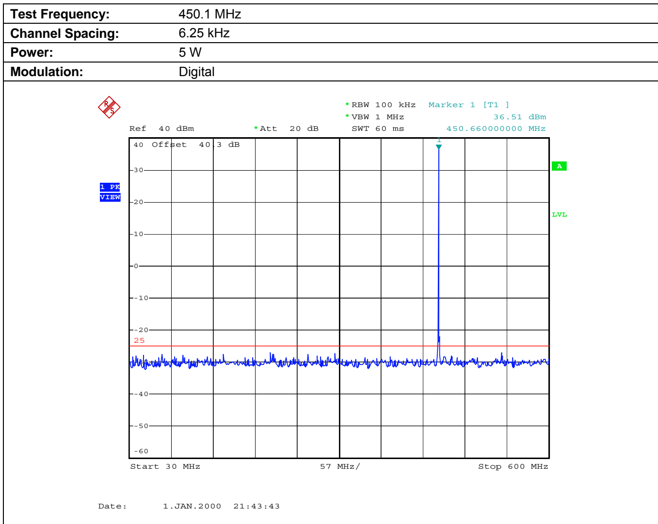
Plot 5.9.4.2.3. Conducted Transmitter Spurious Emissions for 450.1 MHz, Low Power, 30 MHz - 600 MHz
