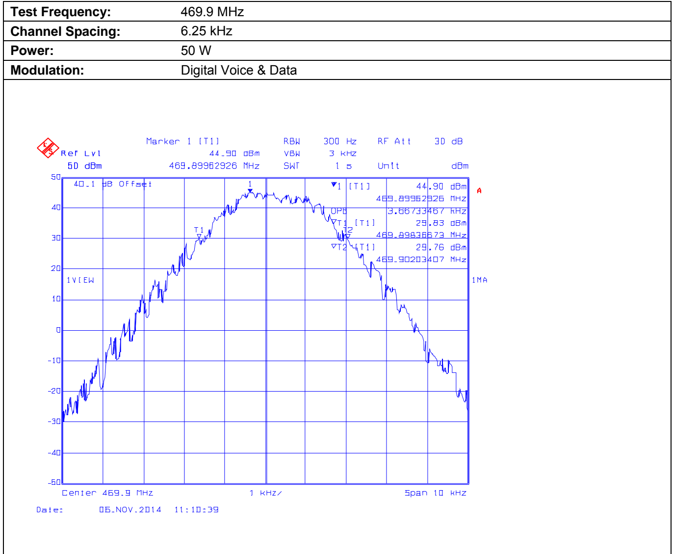
Plot 5.8.4.1.9. Occupied Bandwidth
