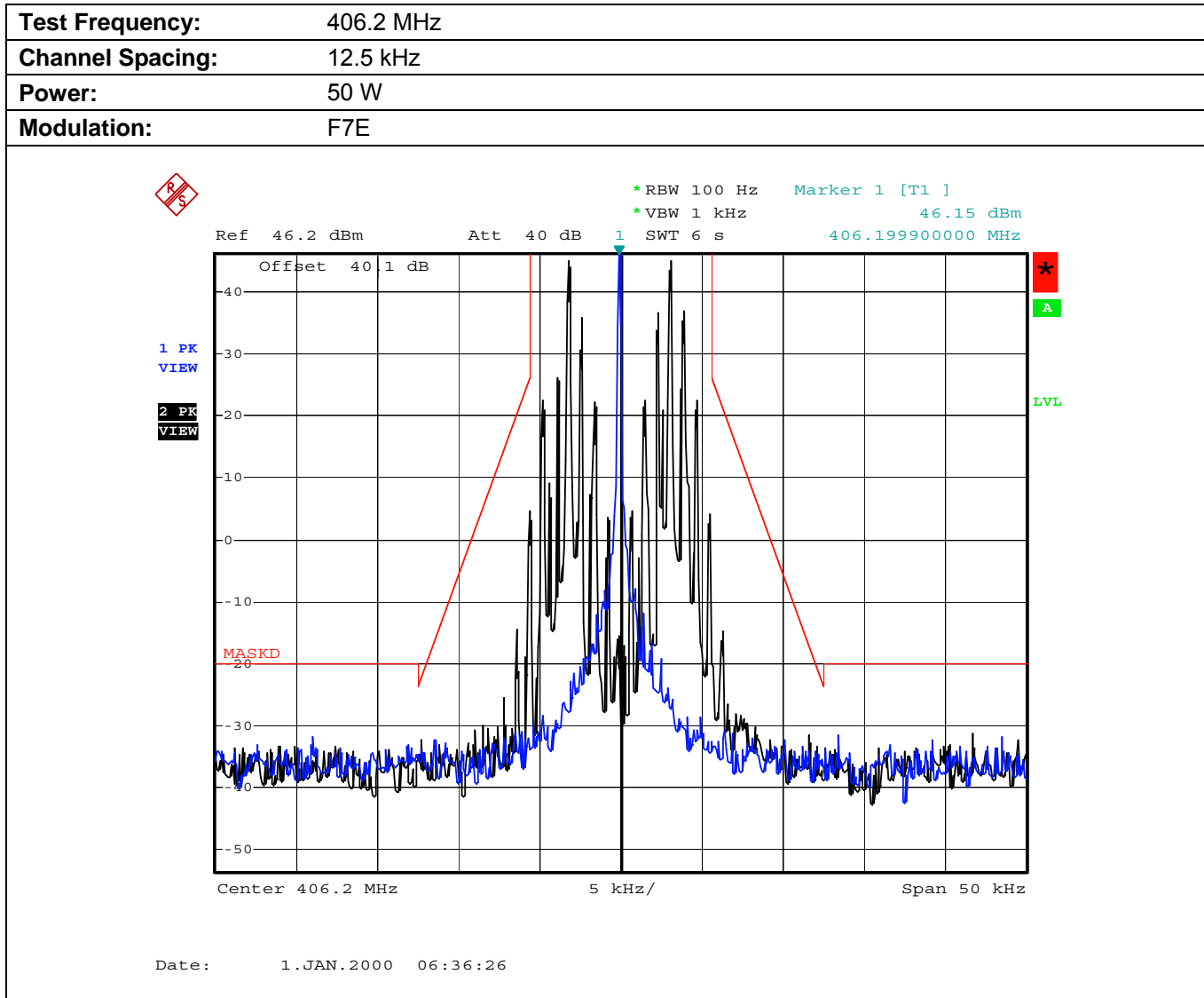
Plot 5.8.4.2.13. Emission Mask D, High Power
