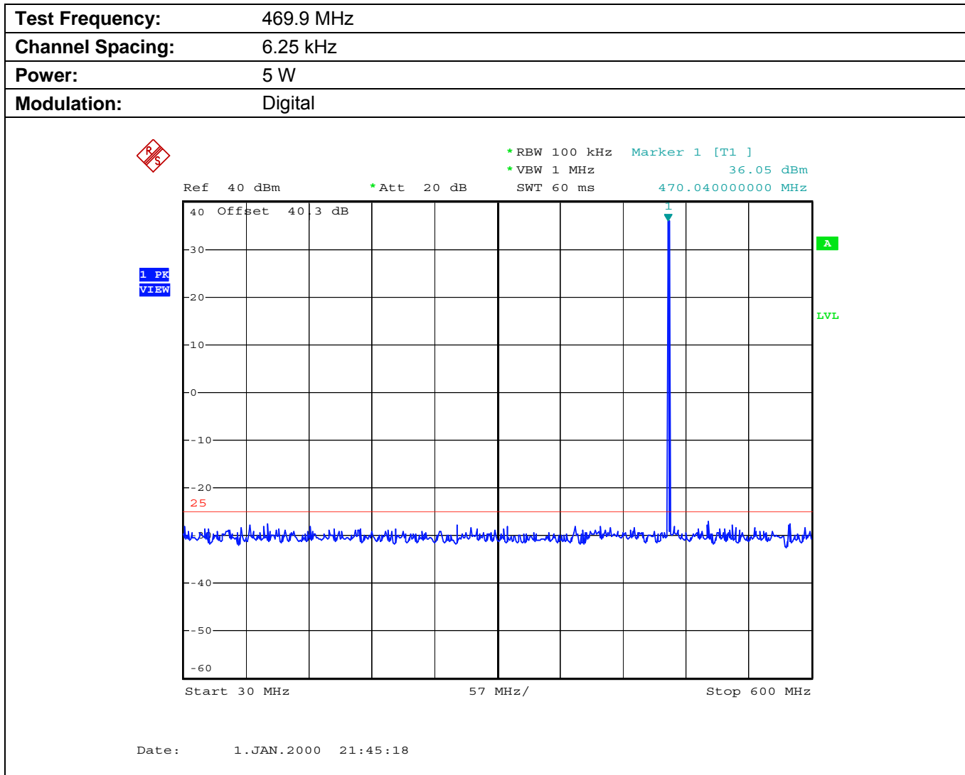
Plot 5.9.4.3.3. Conducted Transmitter Spurious Emissions for 469.9 MHz, Low Power, 30 MHz - 600 MHz
