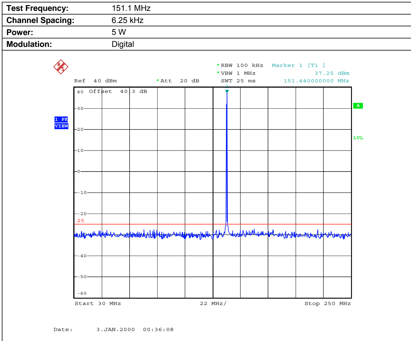
Plot 5.9.4.2.3. Conducted Transmitter Spurious Emissions for 151.1 MHz, Low Power, 30 MHz - 250 MHz
