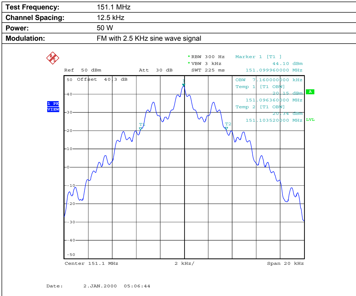
Plot 5.8.4.1.5. Occupied Bandwidth
