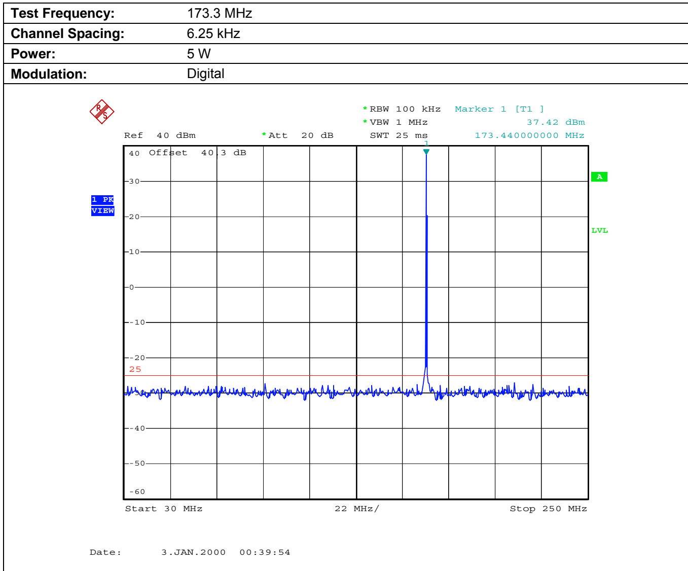
Plot 5.9.4.3.3. Conducted Transmitter Spurious Emissions for 173.3 MHz, Low Power, 30 MHz - 250 MHz
