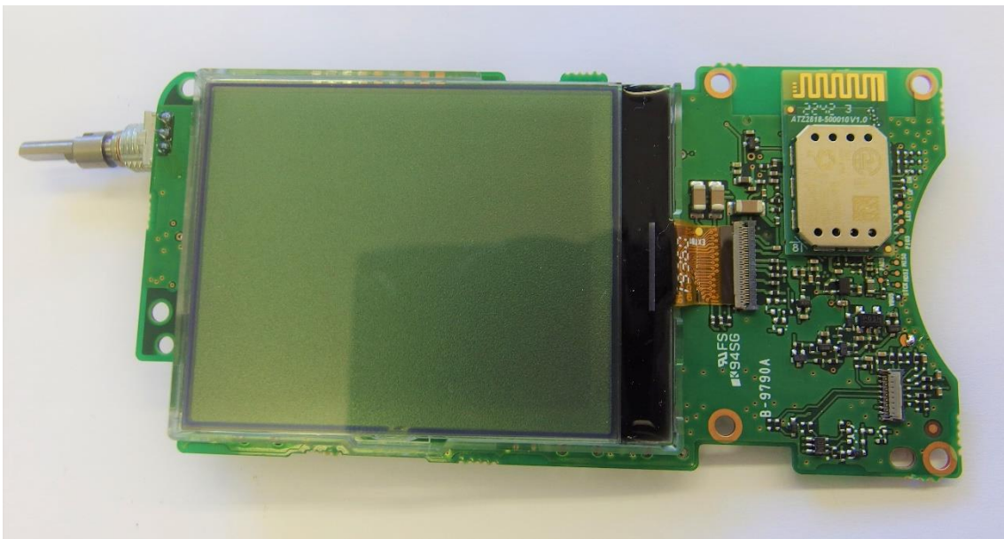
LOGIC_A_LCD
