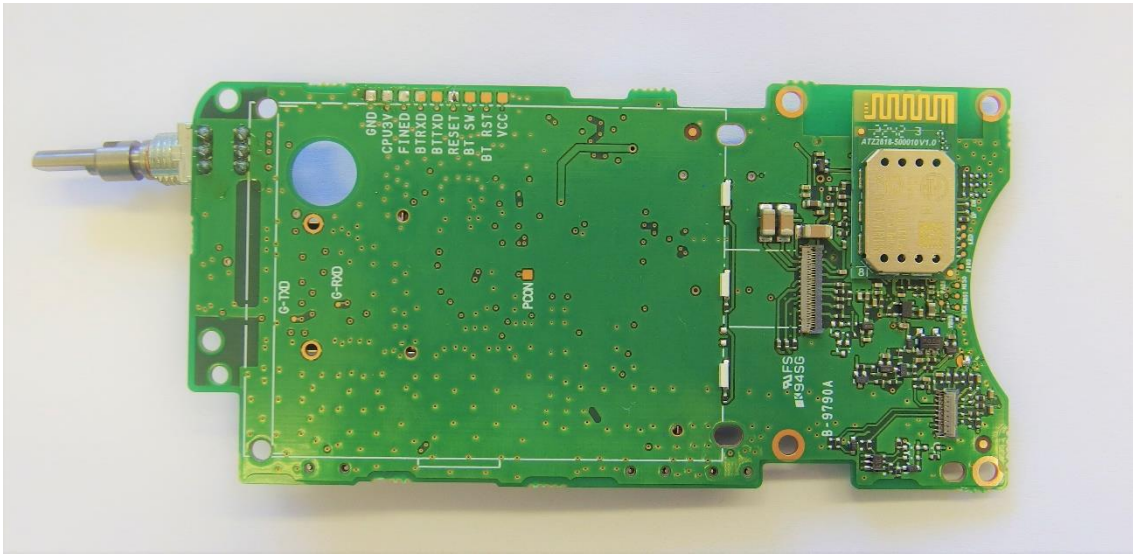
LOGIC_A
