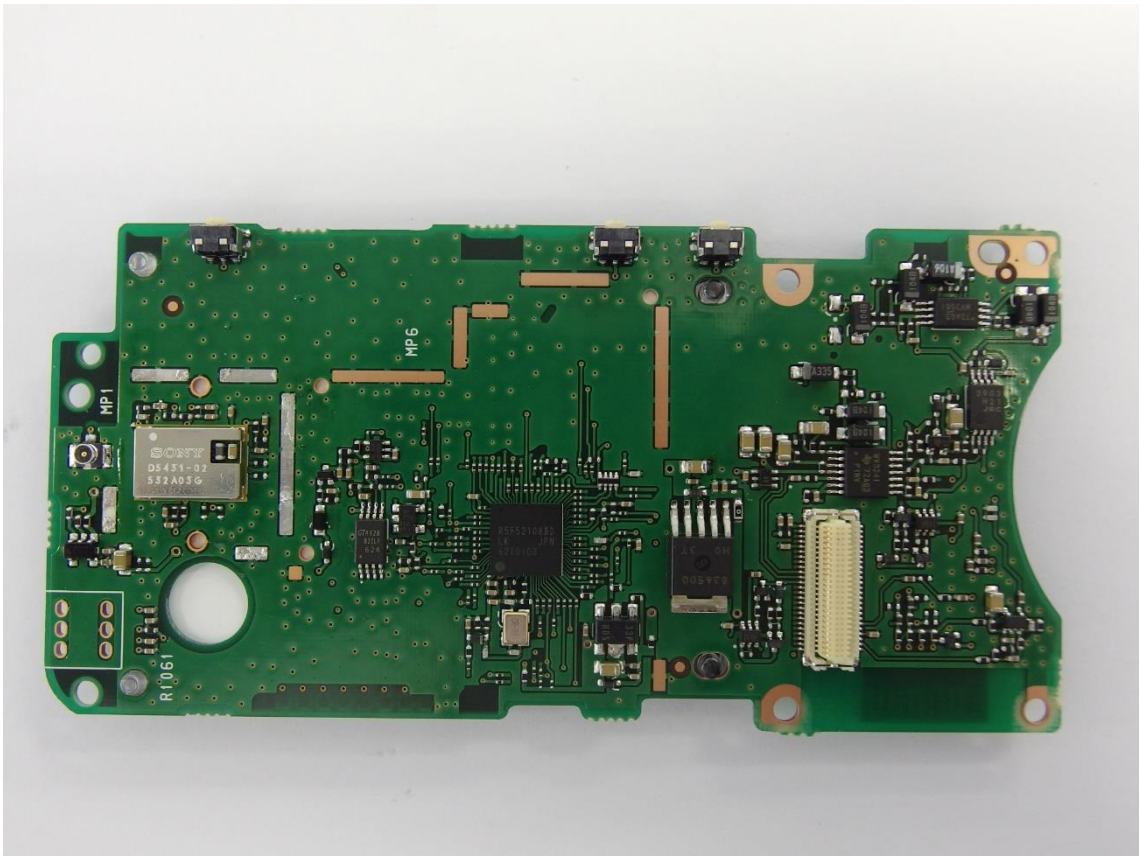
LOGIC_B
