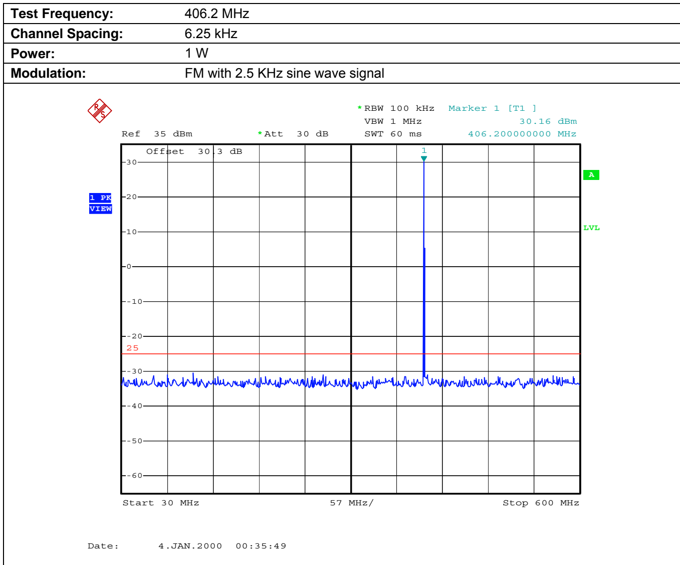
Plot 5.9.4.1.3. Conducted Transmitter Spurious Emissions for 406.2 MHz, Low Power, 30 MHz - 600 MHz
