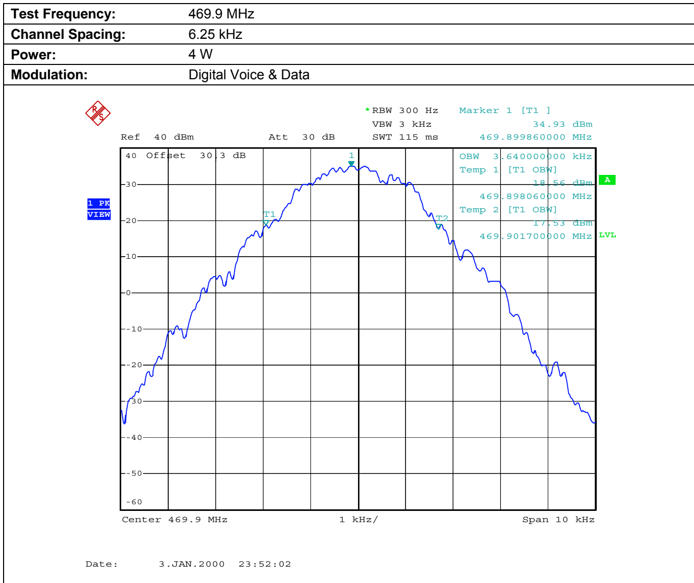
Plot 5.8.4.1.9. Occupied Bandwidth
