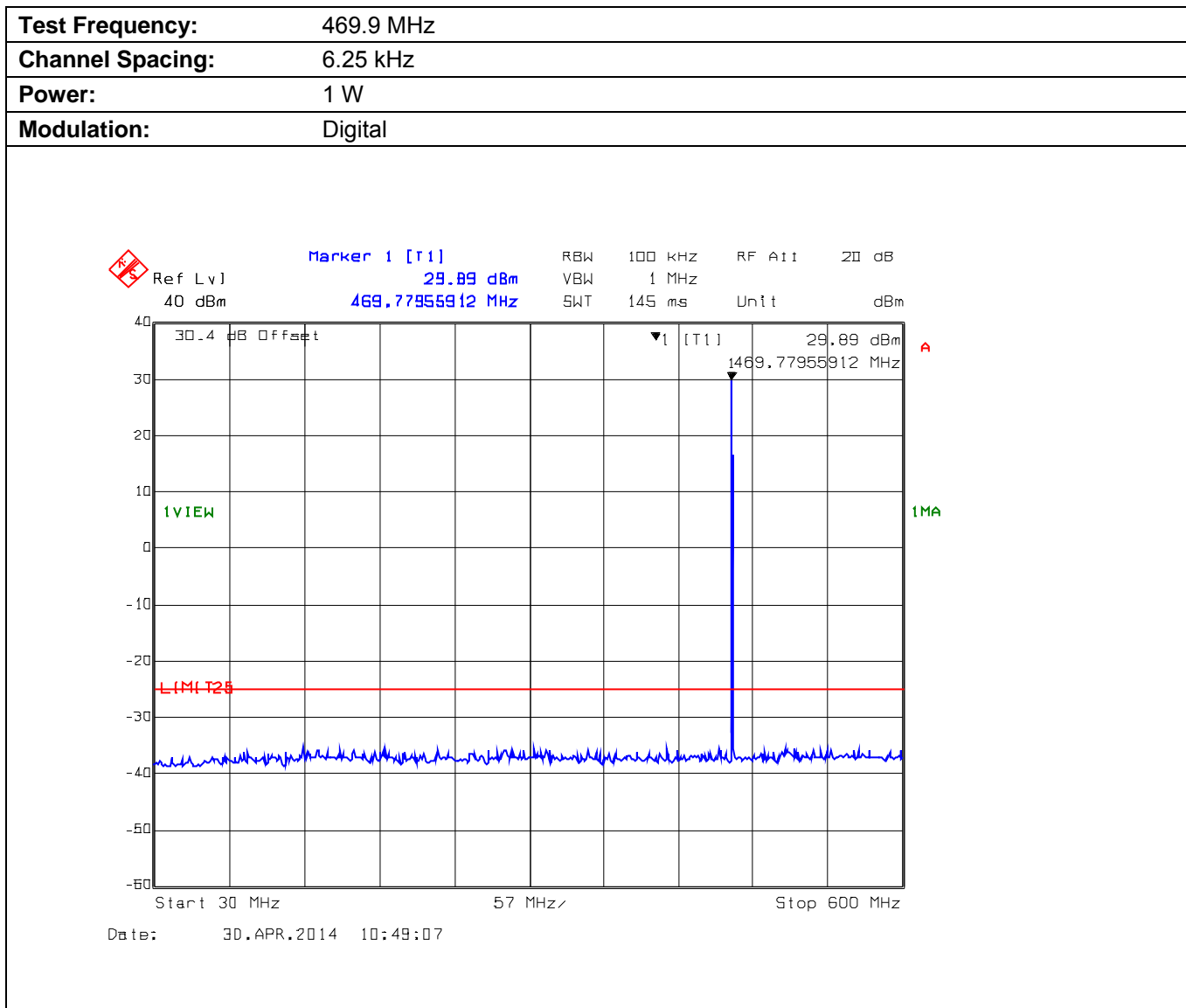
Plot 5.9.4.3.3. Conducted Transmitter Spurious Emissions for 469.9 MHz, Low Power, 30 MHz - 600 MHz
