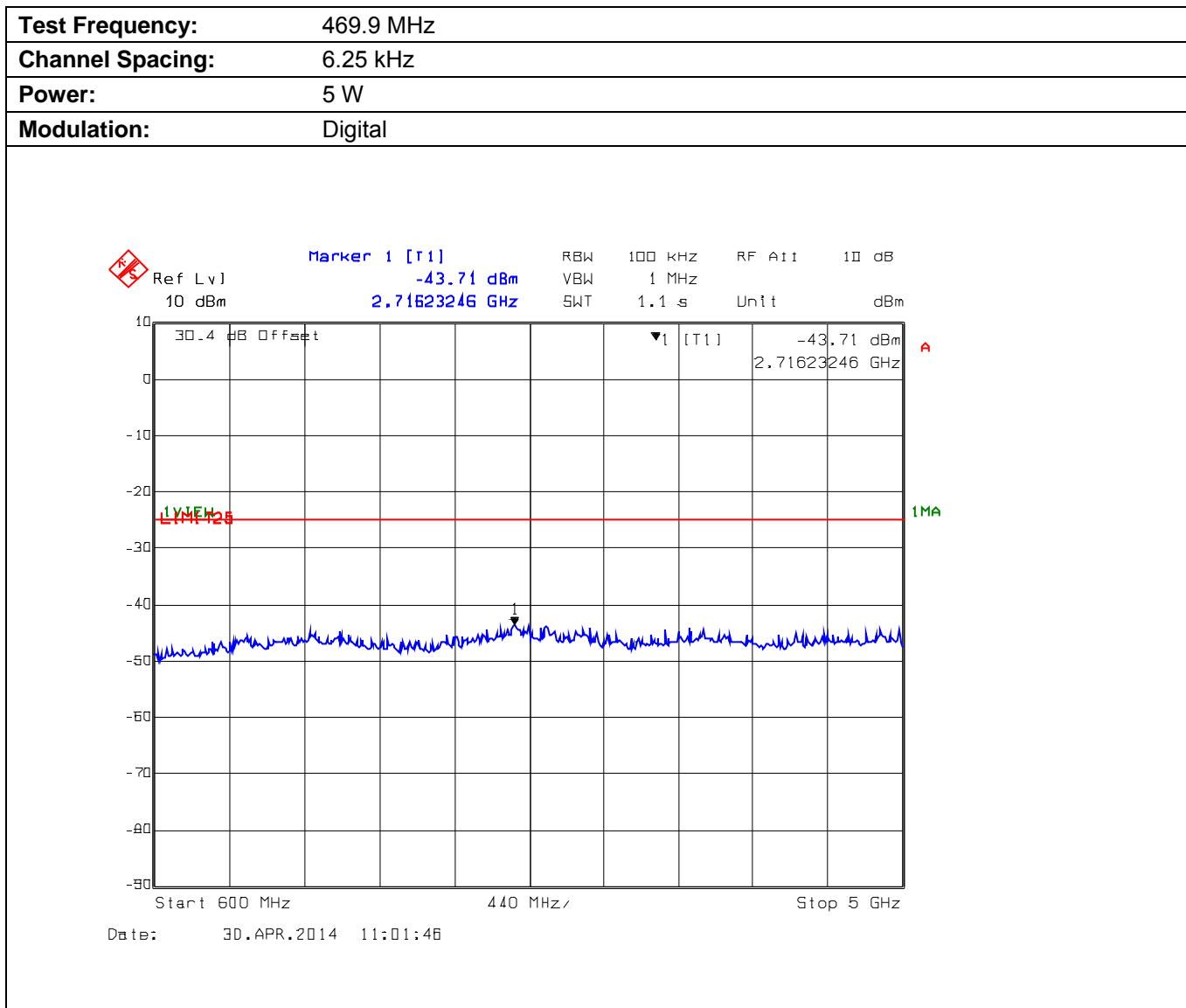
Plot 5.9.4.3.2. Conducted Transmitter Spurious Emissions for 469.9 MHz, High Power, 600 MHz - 5 GHz
