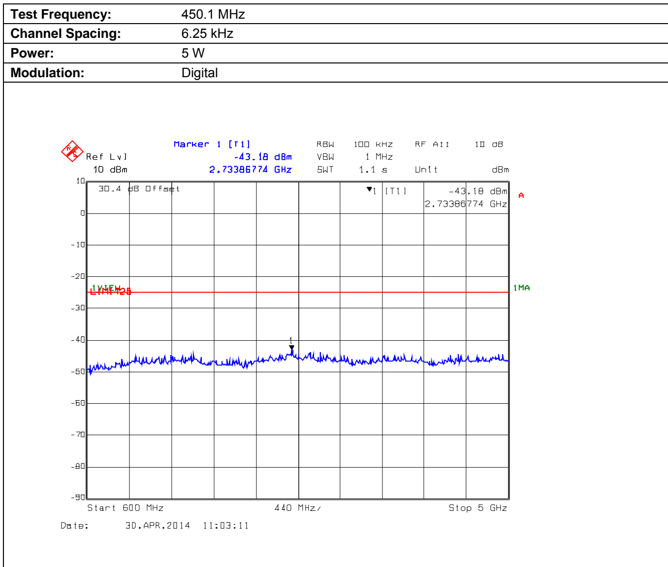
Plot 5.9.4.2.2. Conducted Transmitter Spurious Emissions for 450.1 MHz, High Power, 600 MHz - 5 GHz
