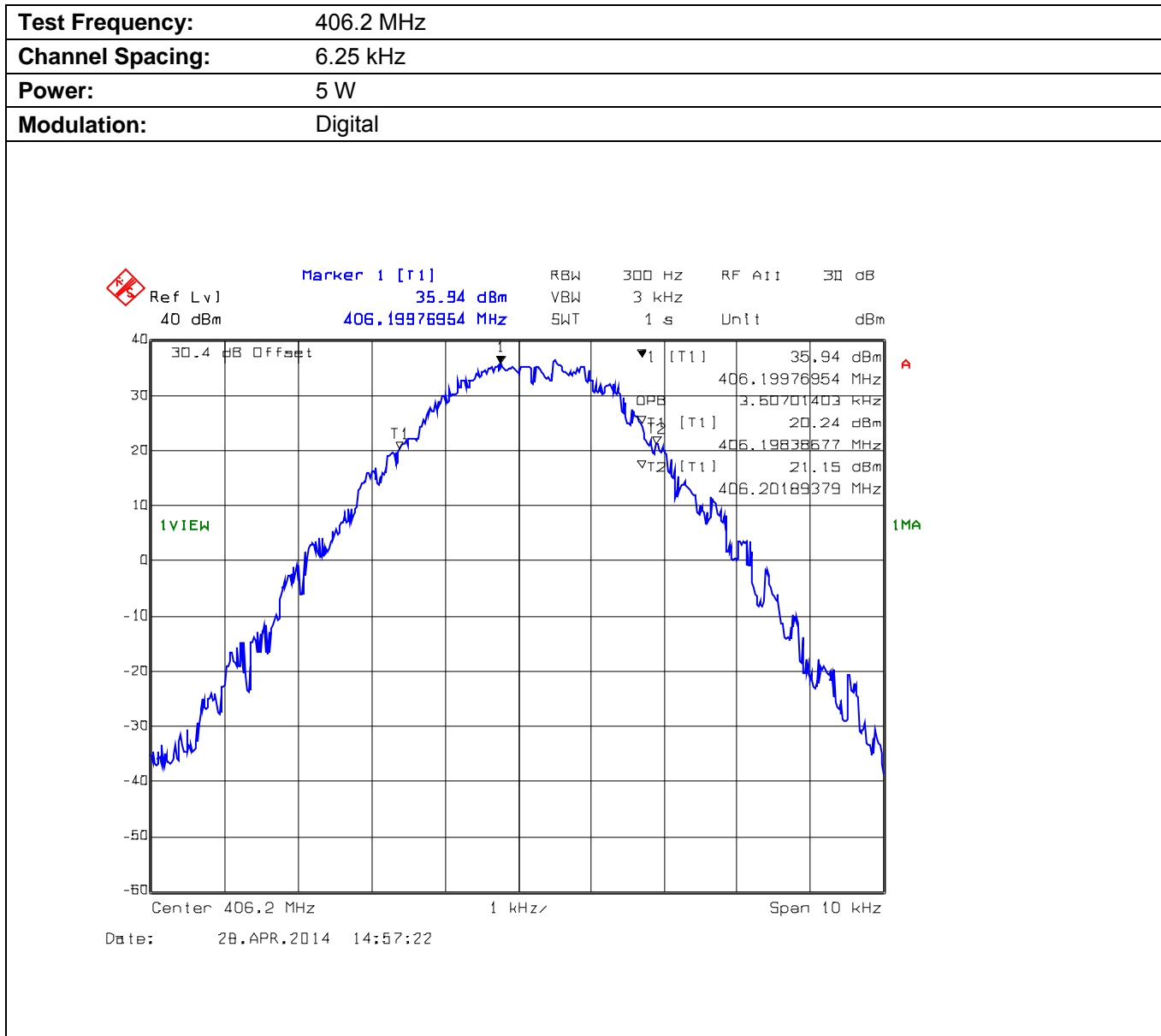
Plot 5.8.4.1.10. Occupied Bandwidth
