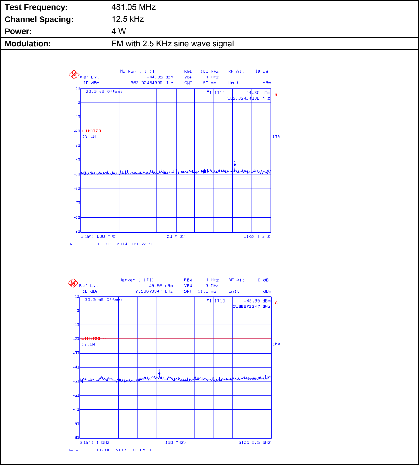
Plot 5.9.4.2.2. Conducted Transmitter Spurious Emissions for 481.05 MHz, High Power, 800 MHz - 5.5 GHz
