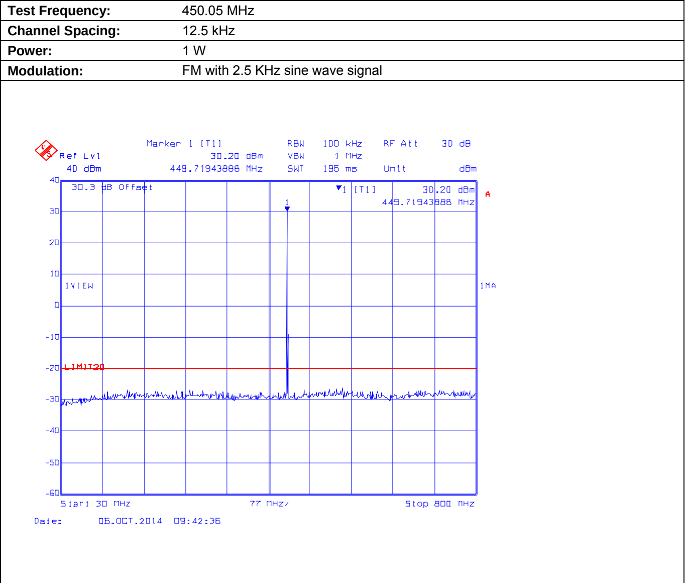
Plot 5.9.4.1.3. Conducted Transmitter Spurious Emissions for 450.05 MHz, Low Power, 30 MHz - 800 MHz
