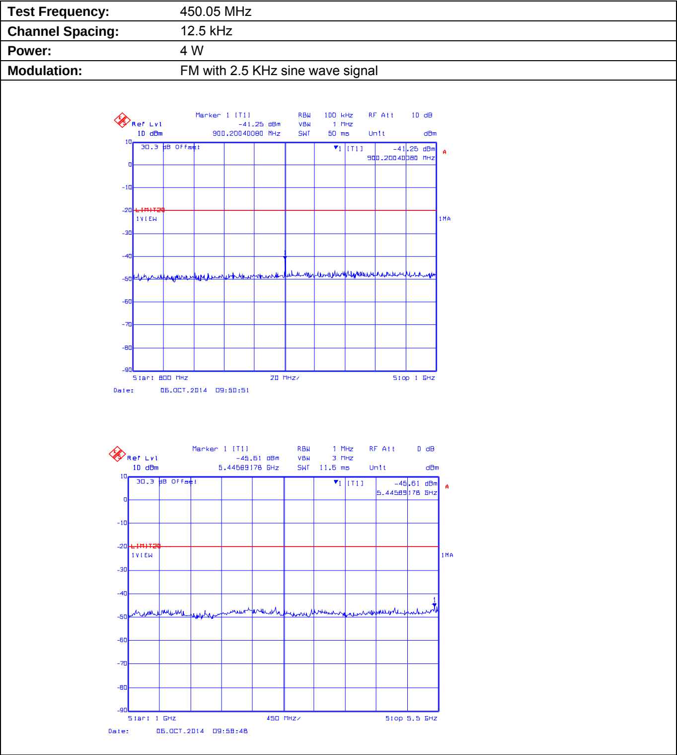
Plot 5.9.4.1.2. Conducted Transmitter Spurious Emissions for 450.05 MHz, High Power, 800 MHz - 5.5 GHz
