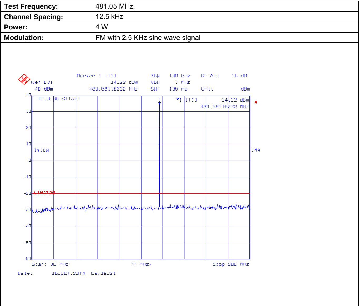
Plot 5.9.4.2.1. Conducted Transmitter Spurious Emissions for 481.05 MHz, High Power, 30 MHz - 800 MHz
