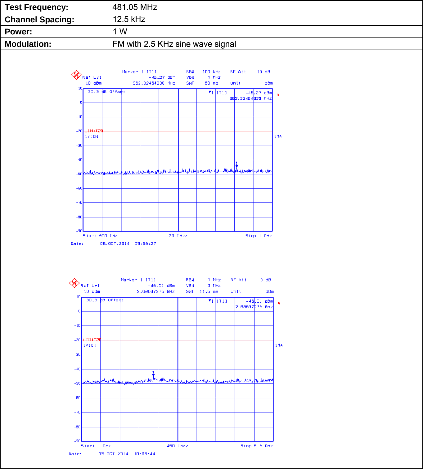
Plot 5.9.4.2.4. Conducted Transmitter Spurious Emissions for 481.05 MHz, Low Power, 800 MHz - 5.5 GHz
