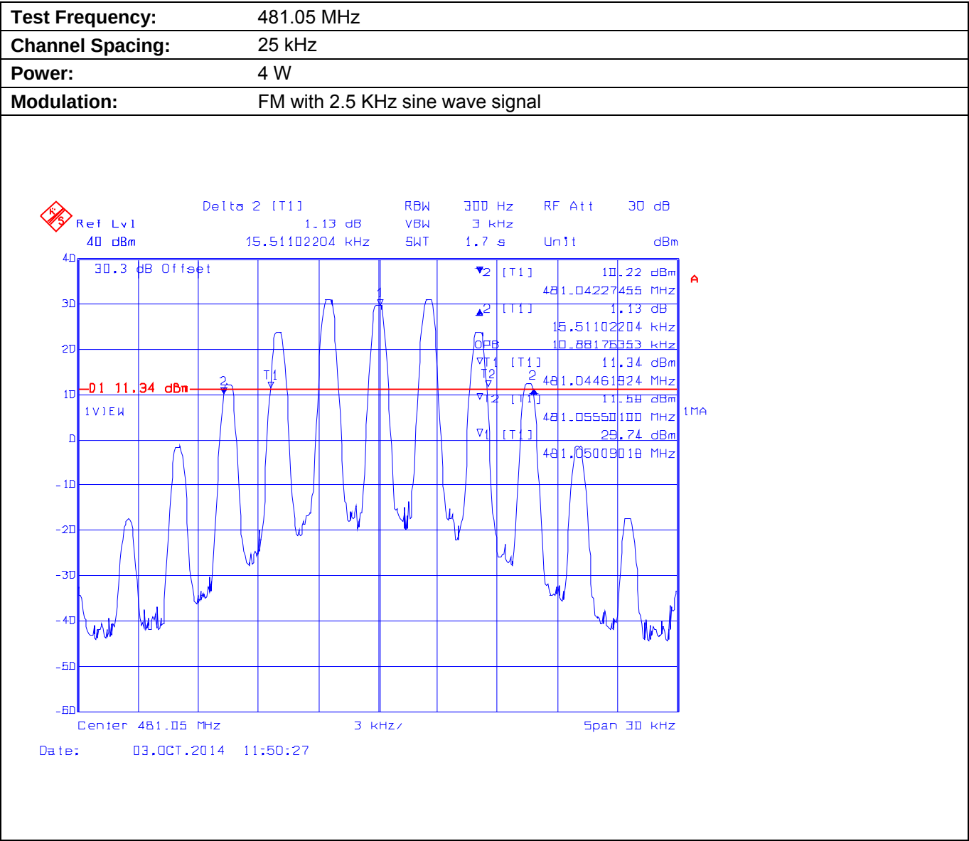
Plot 5.8.4.1.5. Occupied Bandwidth
