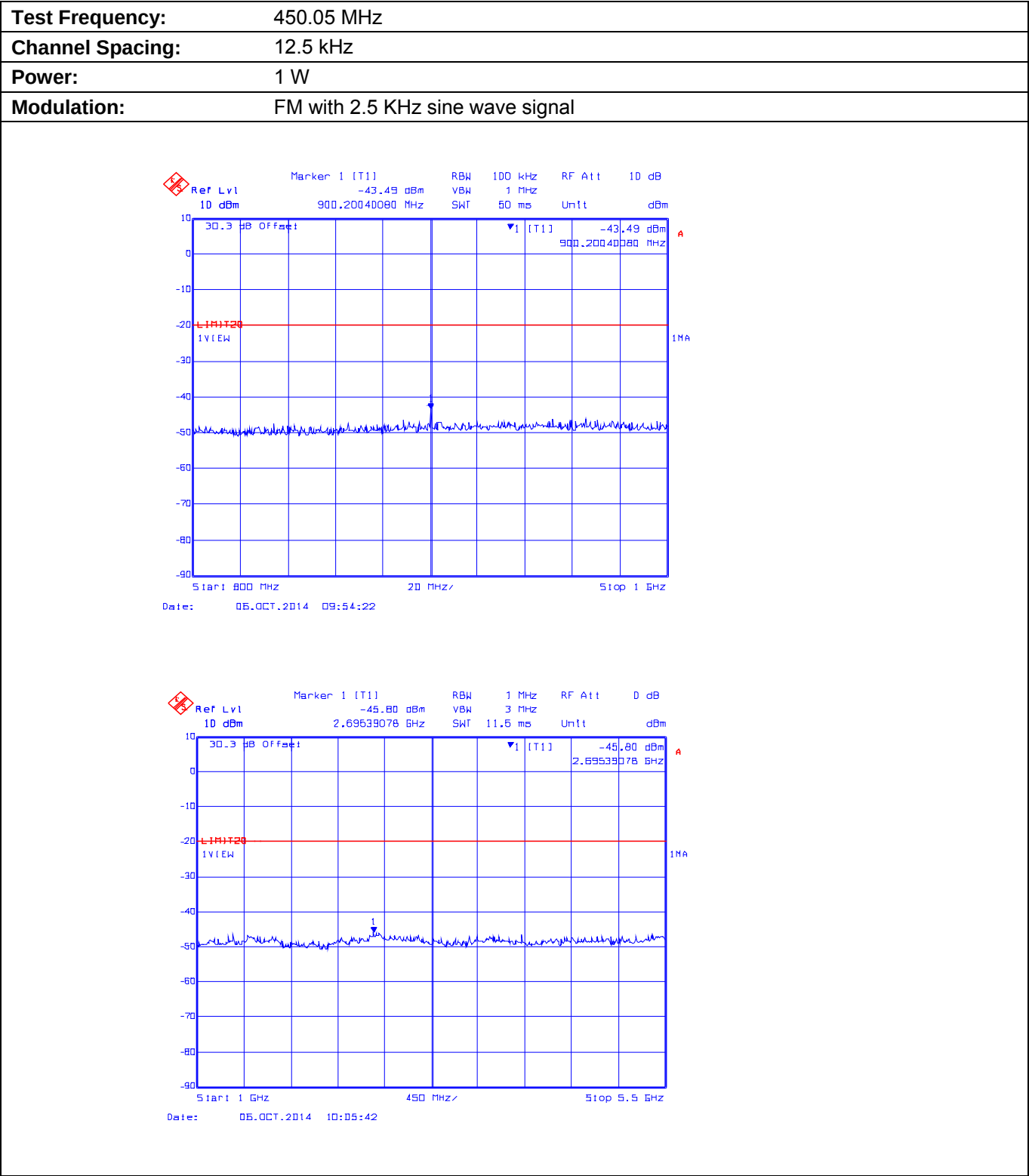
Plot 5.9.4.1.4. Conducted Transmitter Spurious Emissions for 450.05 MHz, Low Power, 800 MHz - 5.5 GHz
