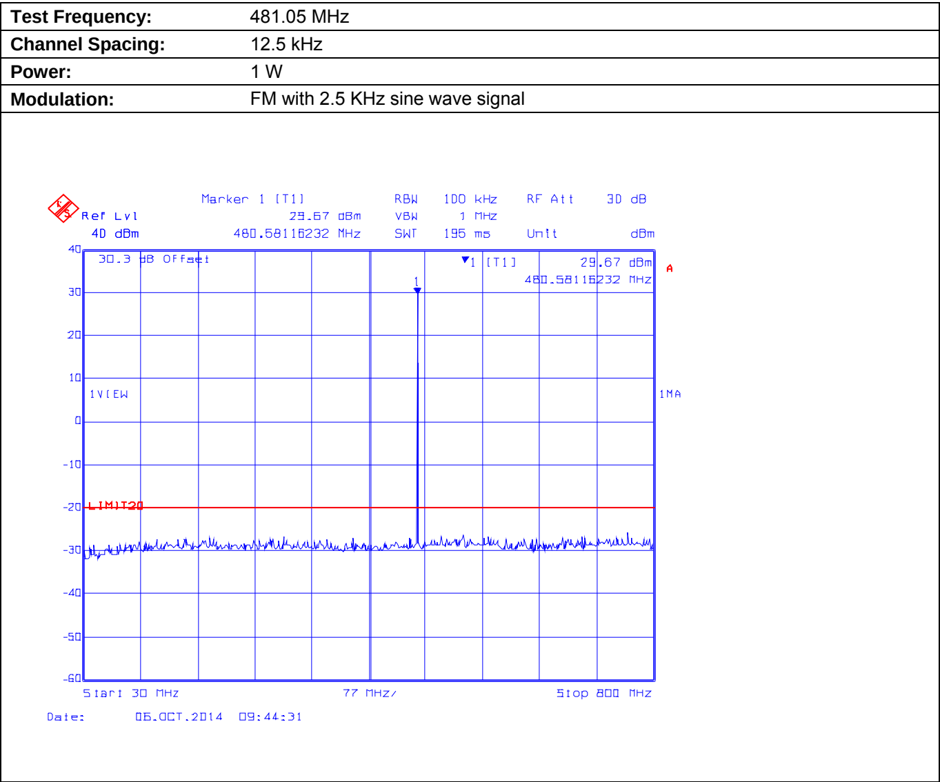
Plot 5.9.4.2.3. Conducted Transmitter Spurious Emissions for 481.05 MHz, Low Power, 30 MHz - 800 MHz
