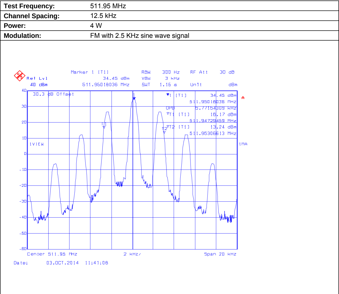
Plot 5.8.4.1.3. Occupied Bandwidth
