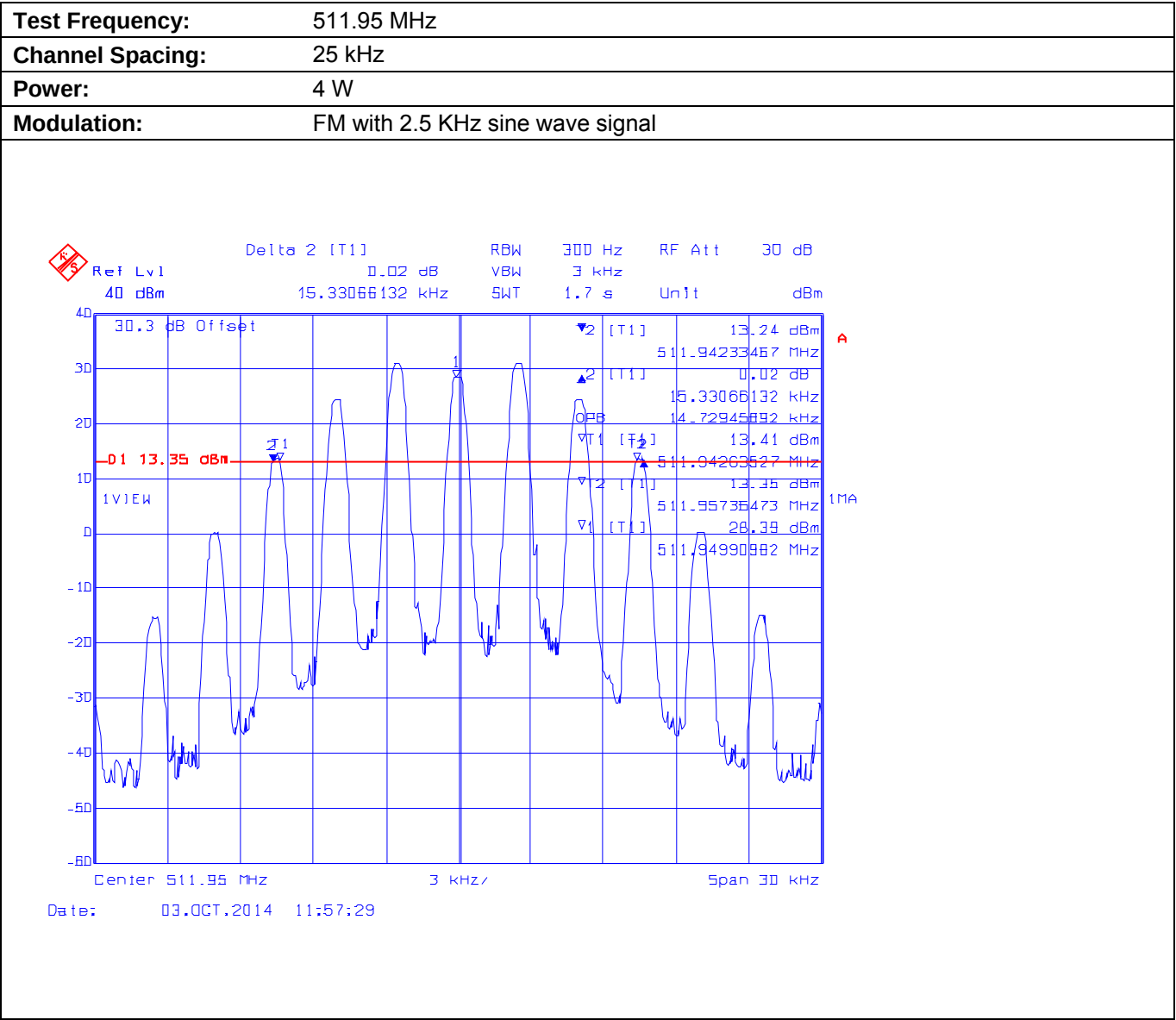
Plot 5.8.4.1.6. Occupied Bandwidth
