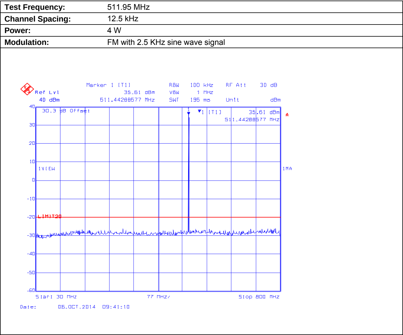
Plot 5.9.4.3.1. Conducted Transmitter Spurious Emissions for 511.95 MHz, High Power, 30 MHz - 800 MHz
