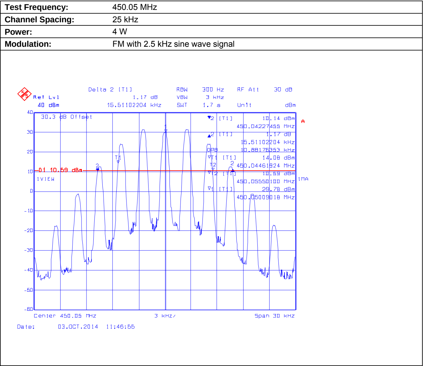
Plot 5.8.4.1.4. Occupied Bandwidth
