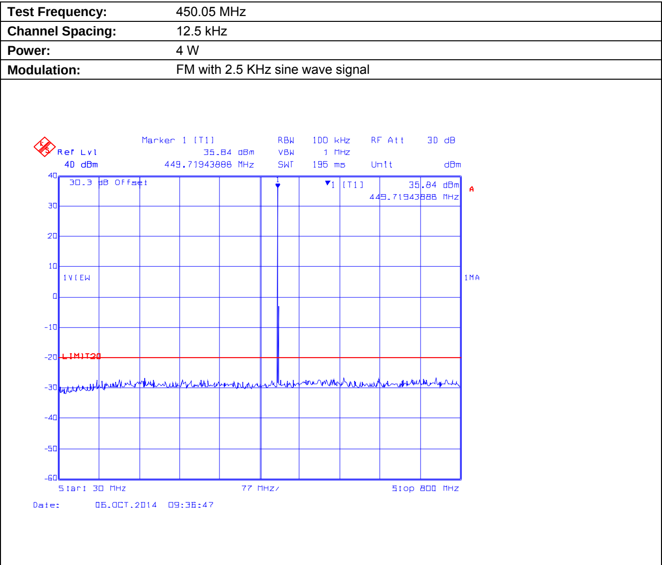
Plot 5.9.4.1.1. Conducted Transmitter Spurious Emissions for 450.05 MHz, High Power, 30 MHz - 800 MHz
