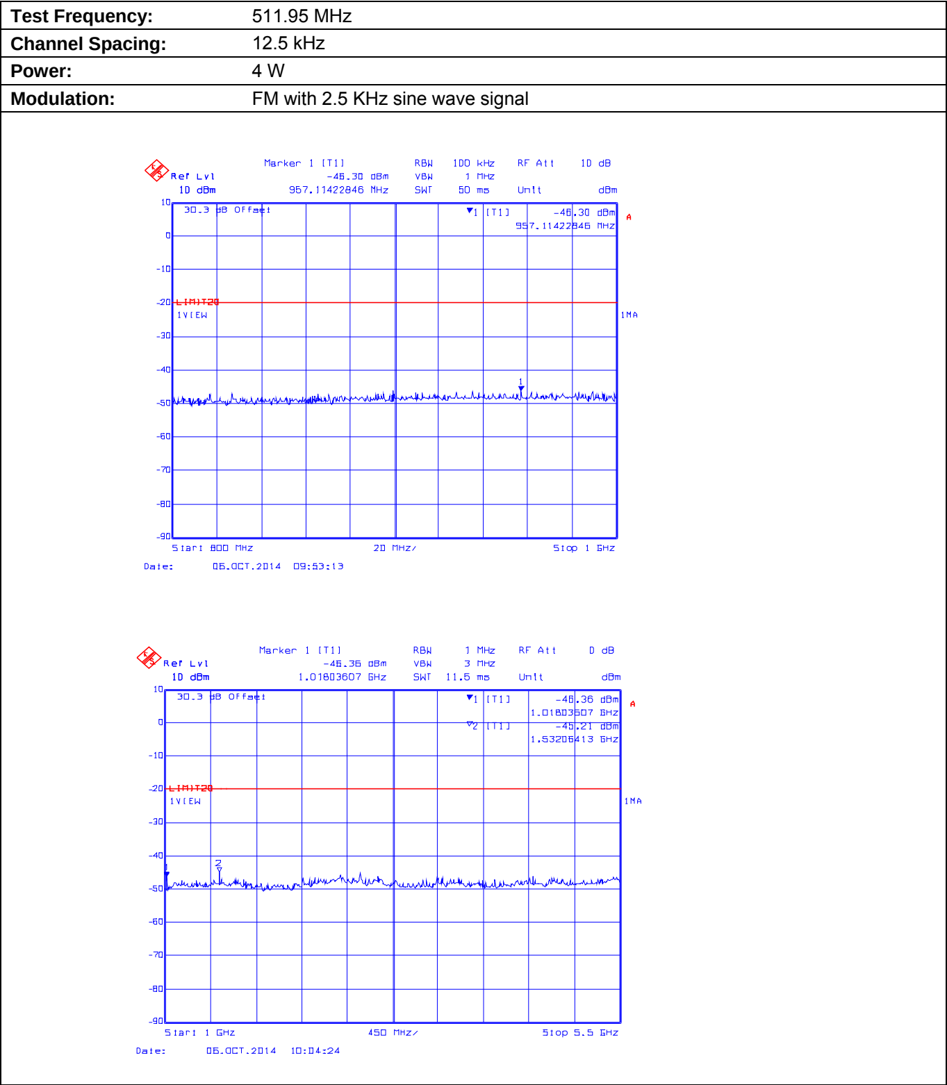
Plot 5.9.4.3.2. Conducted Transmitter Spurious Emissions for 511.95 MHz, High Power, 800 MHz - 5.5 GHz
