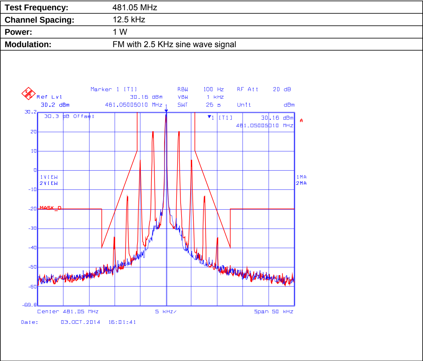
Plot 5.8.4.2.5. Emission Mask D, Low Power
