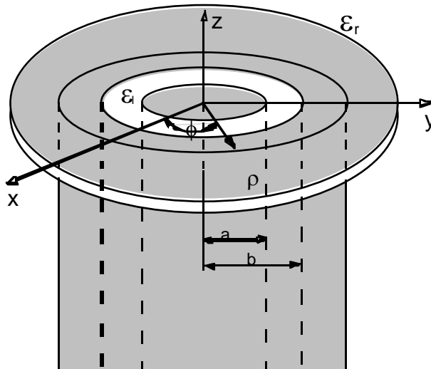
Figure 1.1.23. An open-ended coaxial probe with inner and outer radii a and b , respectively
