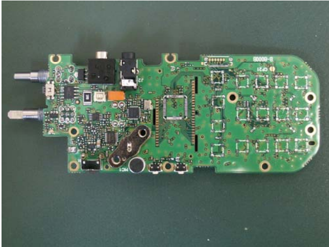
IC-F2000T - Front -
