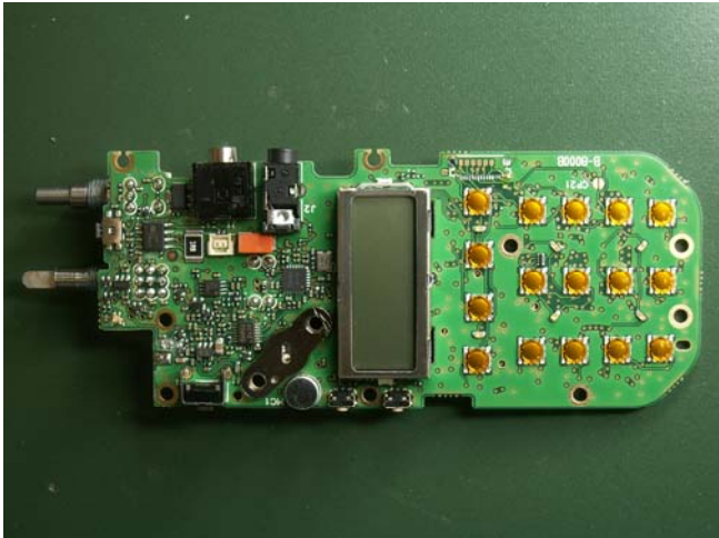
IC-F2000T - Front -
