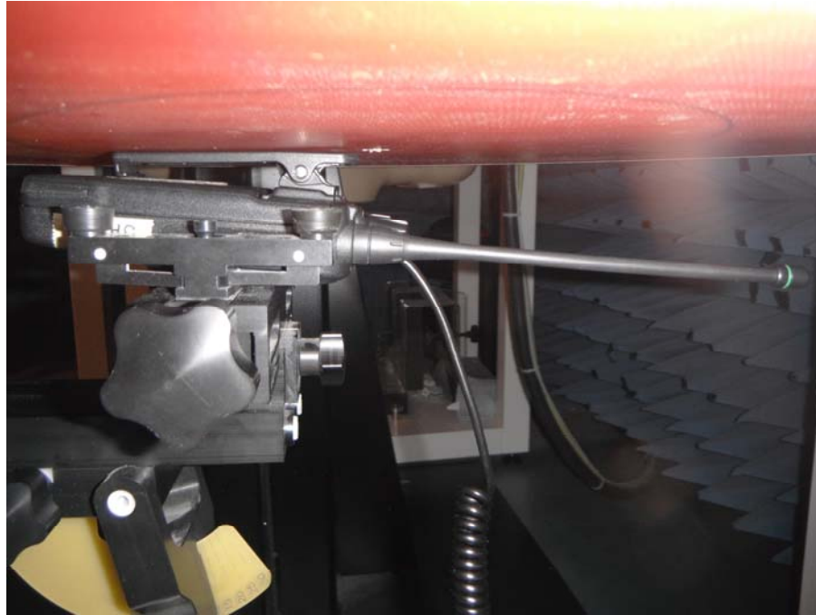
Back side of EUT in parallel to the phantom with the belt-clip (M/N: MB-133) in contact, attached HS-158LA Speaker Microphone
