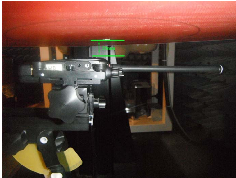
< FA-SC61VC cut antenna with the length of 174mm >
