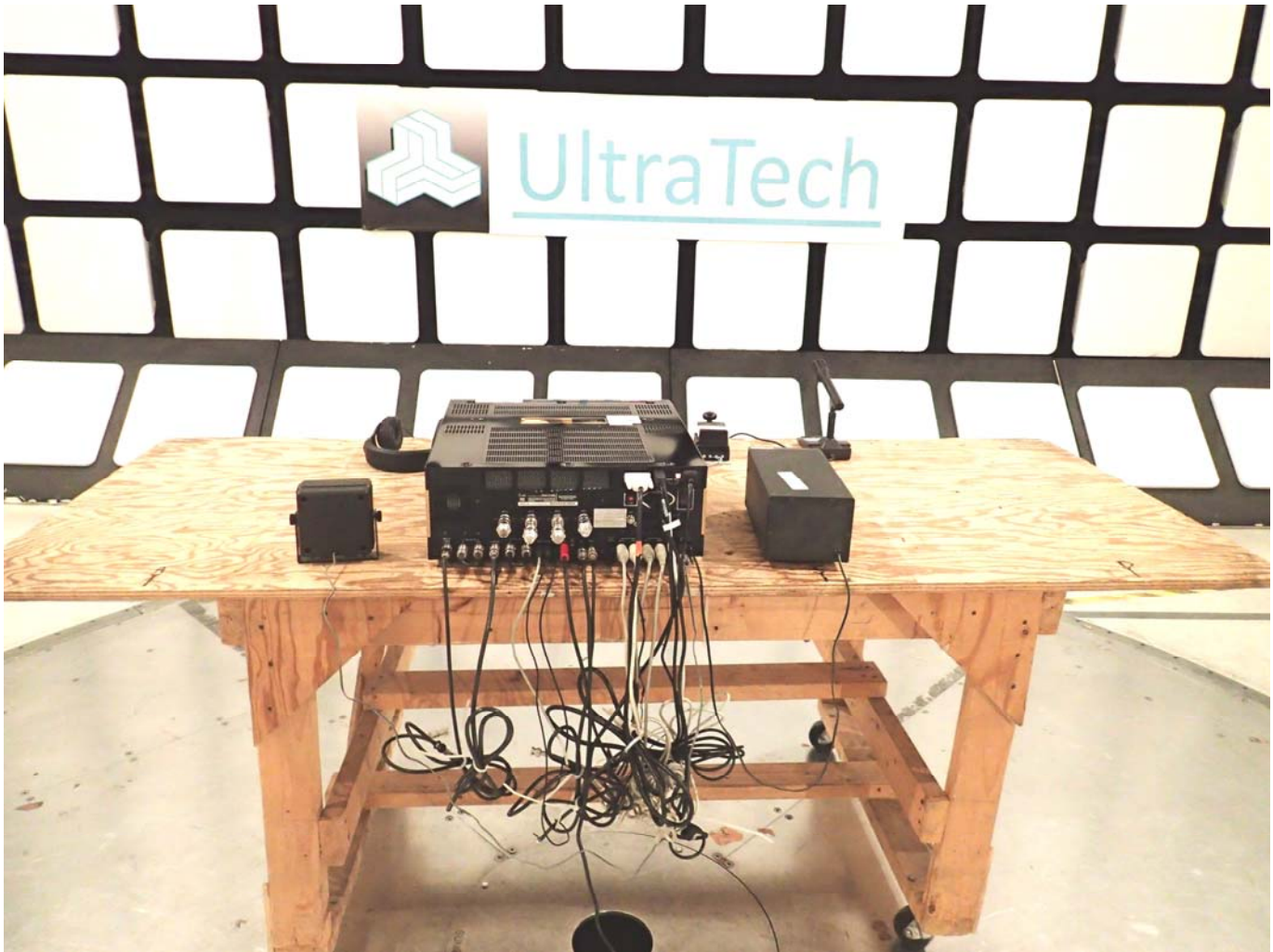
Radiated Emission at 3m Distance
