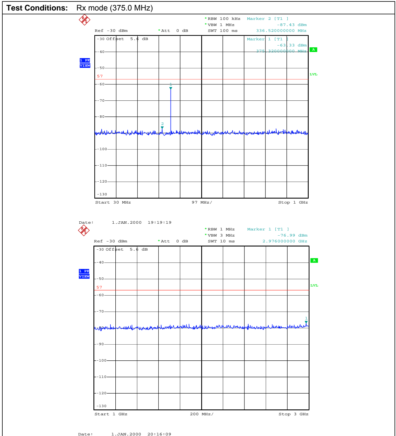
Plot 6: Conducted Receiver Spurious Emissions, 30 MHz – 3.0 GHz
