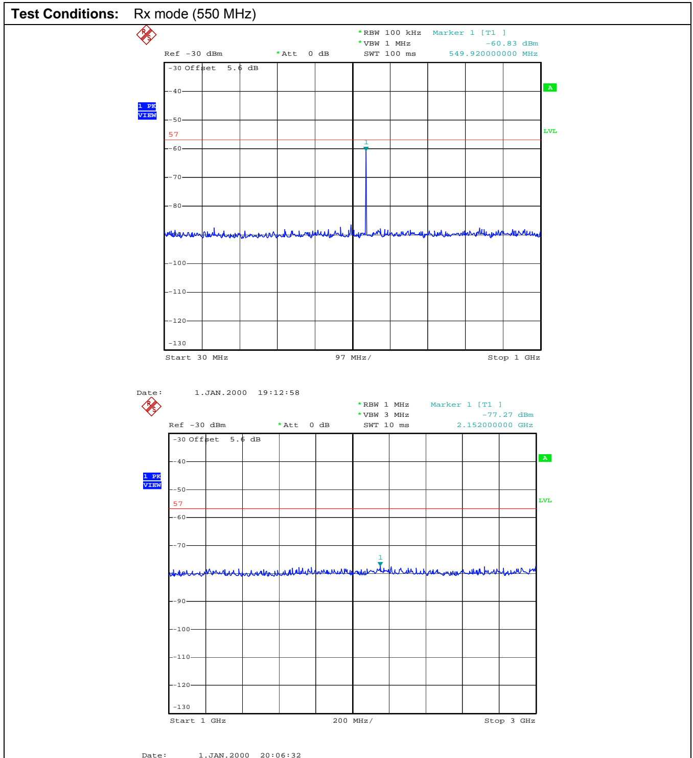
Plot 8: Conducted Receiver Spurious Emissions, 30 MHz – 3.0 GHz
