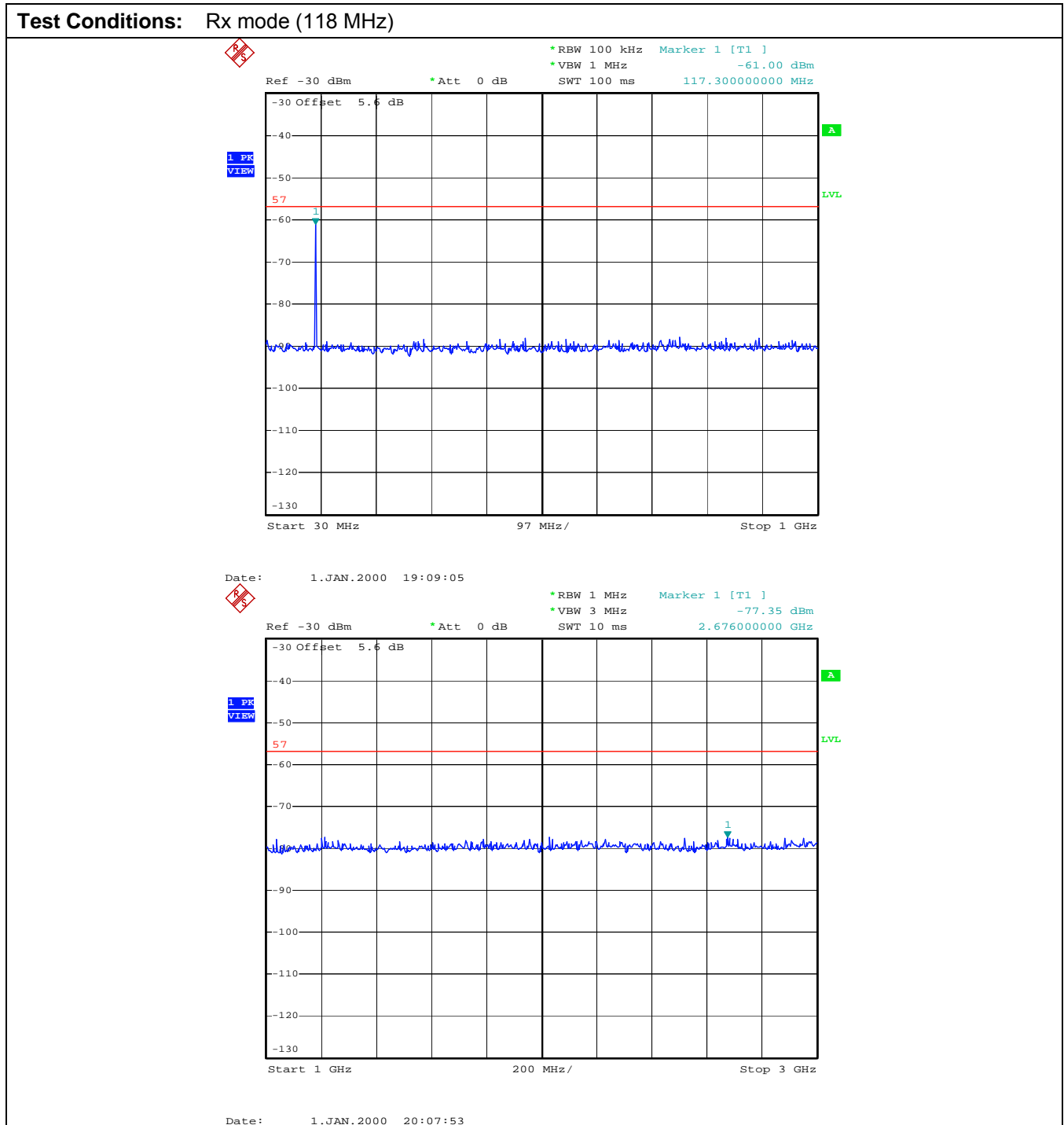
Plot 3: Conducted Receiver Spurious Emissions, 30 MHz – 3.0 GHz
