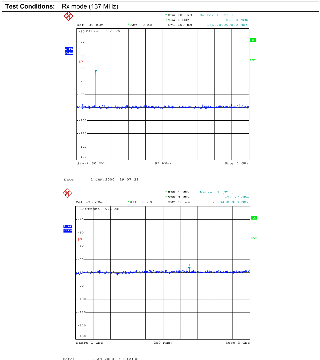
Plot 4: Conducted Receiver Spurious Emissions, 30 MHz – 3.0 GHz
