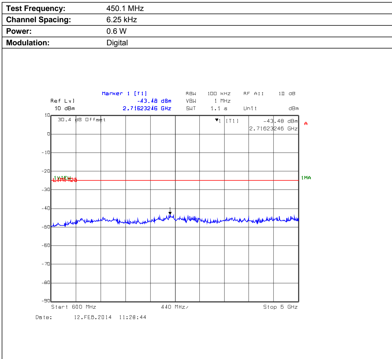
Plot 5.9.4.2.4. Conducted Transmitter Spurious Emissions for 450.1 MHz, Low Power, 600 MHz – 5 GHz
