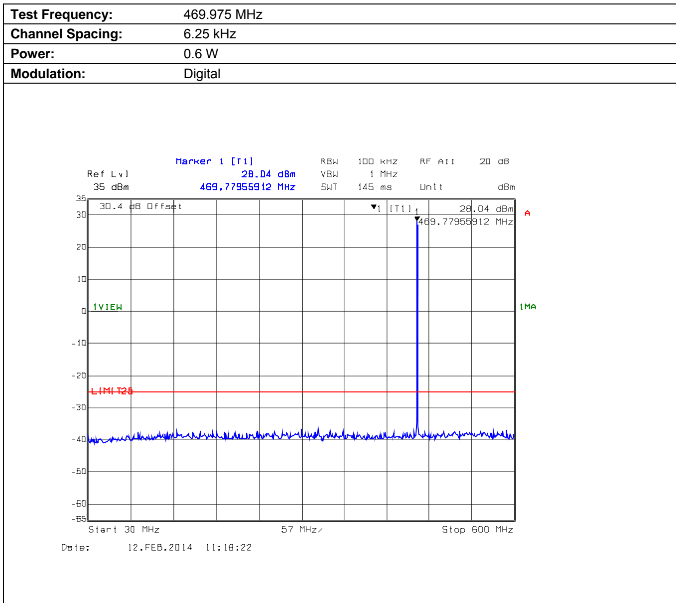
Plot 5.9.4.3.3. Conducted Transmitter Spurious Emissions for 469.975 MHz, Low Power, 30 MHz - 600 MHz
