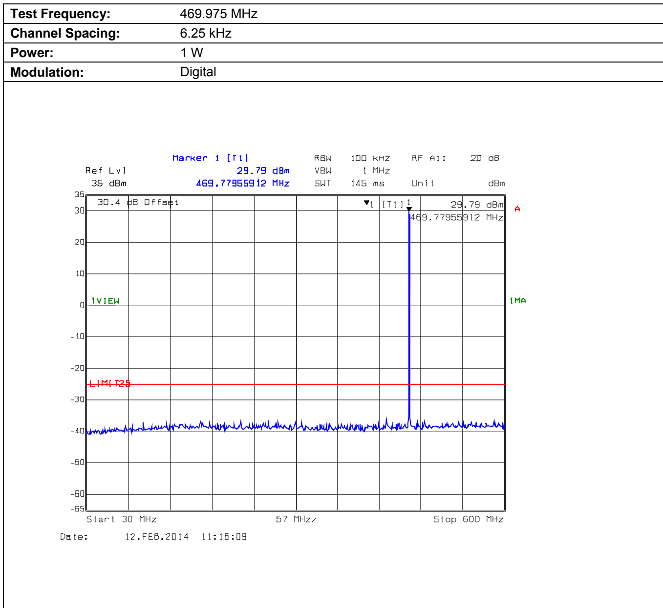
Plot 5.9.4.3.1. Conducted Transmitter Spurious Emissions for 469.975 MHz, High Power, 30 MHz - 600 MHz
