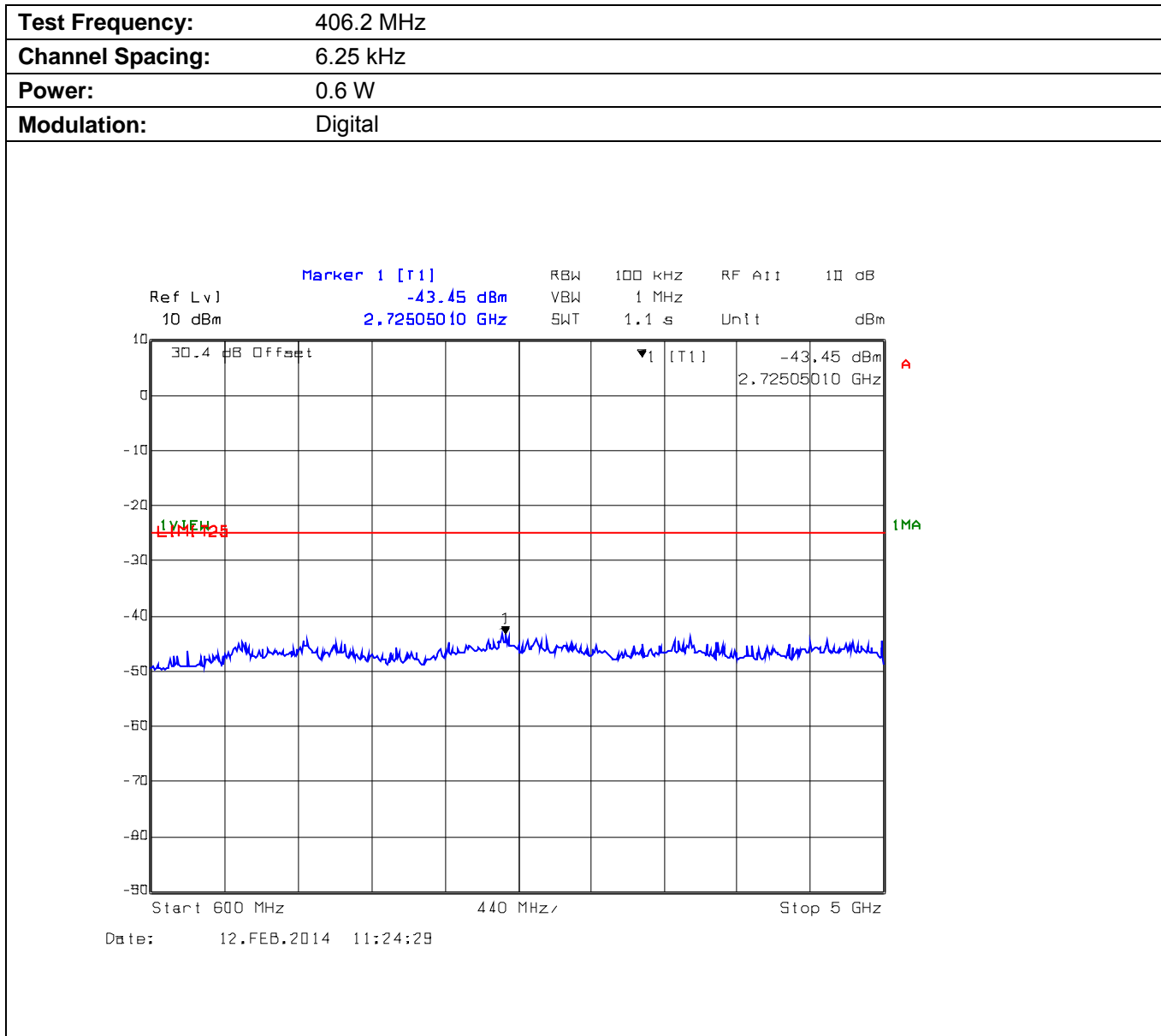
Plot 5.9.4.1.4. Conducted Transmitter Spurious Emissions for 406.2 MHz, Low Power, 600 MHz - 5 GHz
