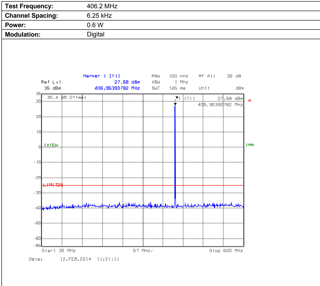
Plot 5.9.4.1.3. Conducted Transmitter Spurious Emissions for 406.2 MHz, Low Power, 30 MHz - 600 MHz
