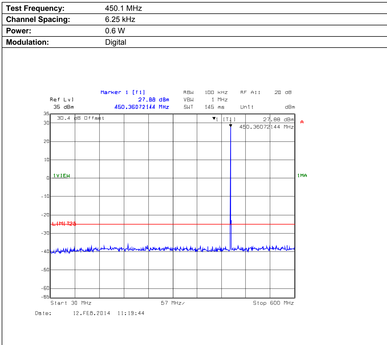
Plot 5.9.4.2.3. Conducted Transmitter Spurious Emissions for 450.1 MHz, Low Power, 30 MHz - 600 MHz
