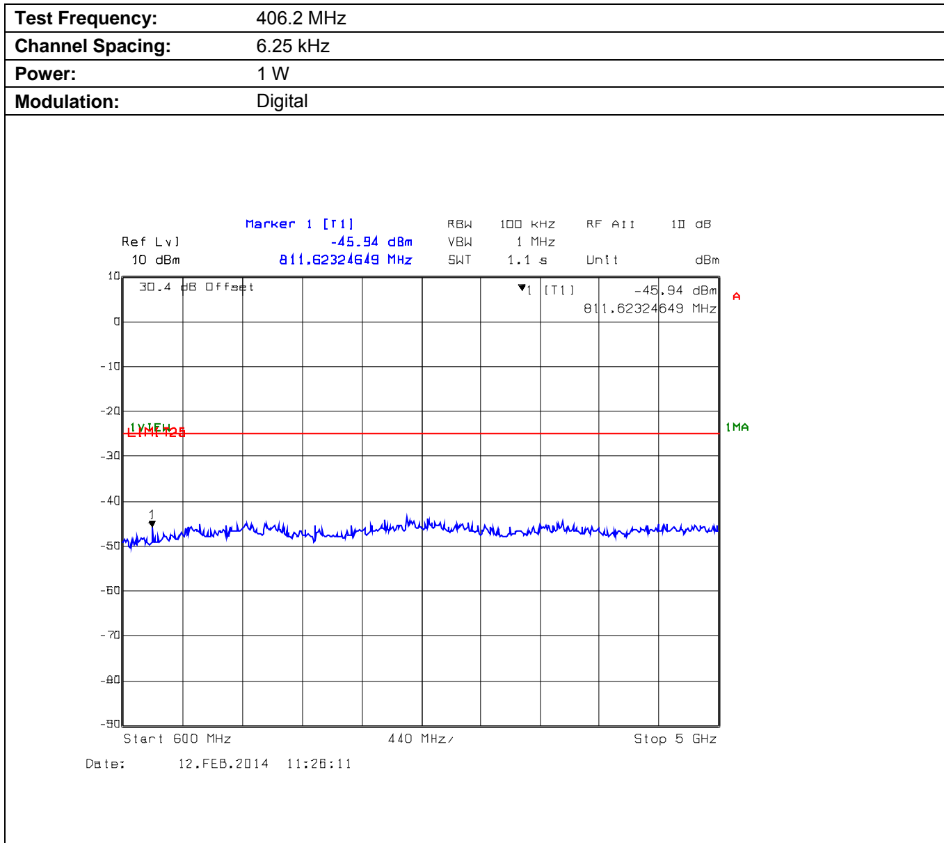
Plot 5.9.4.1.2. Conducted Transmitter Spurious Emissions for 406.2 MHz, High Power, 600 MHz - 5 GHz
