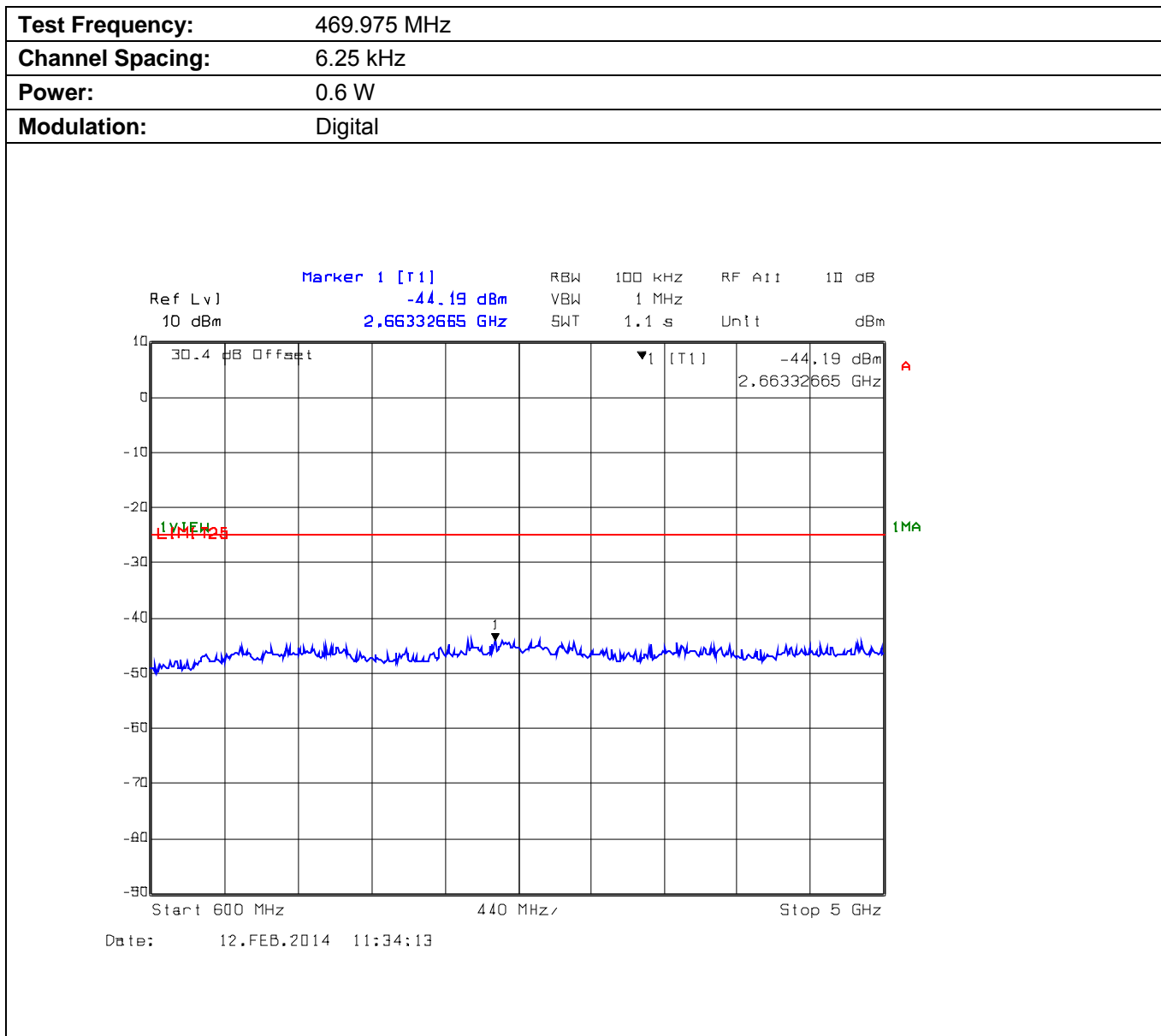
Plot 5.9.4.3.4. Conducted Transmitter Spurious Emissions for 469.975 MHz, Low Power, 600 MHz - 5 GHz
