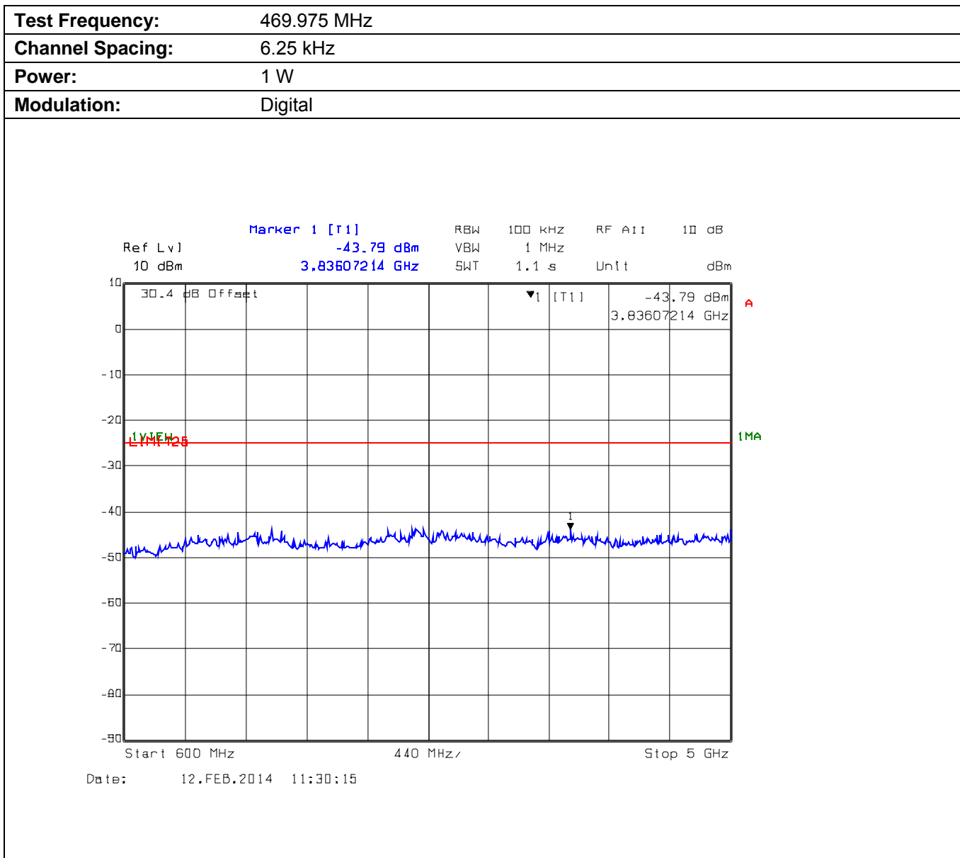
Plot 5.9.4.3.2. Conducted Transmitter Spurious Emissions for 469.975 MHz, High Power, 600 MHz - 5 GHz
