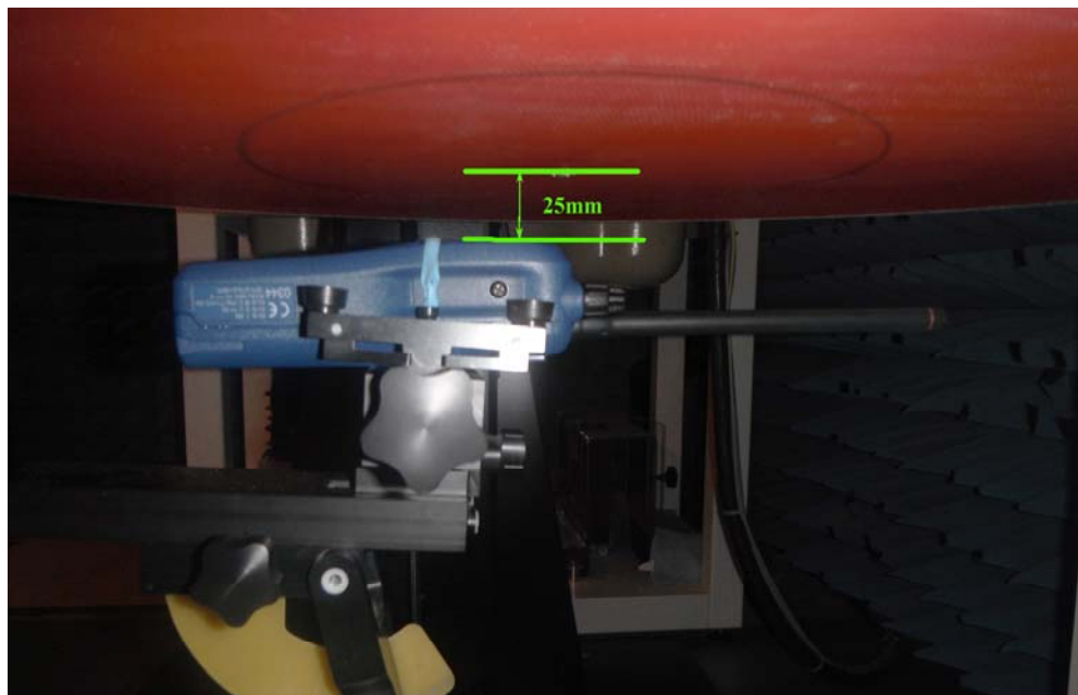
< FA-SC55V: 146MHz~174MHz; Red ring >
