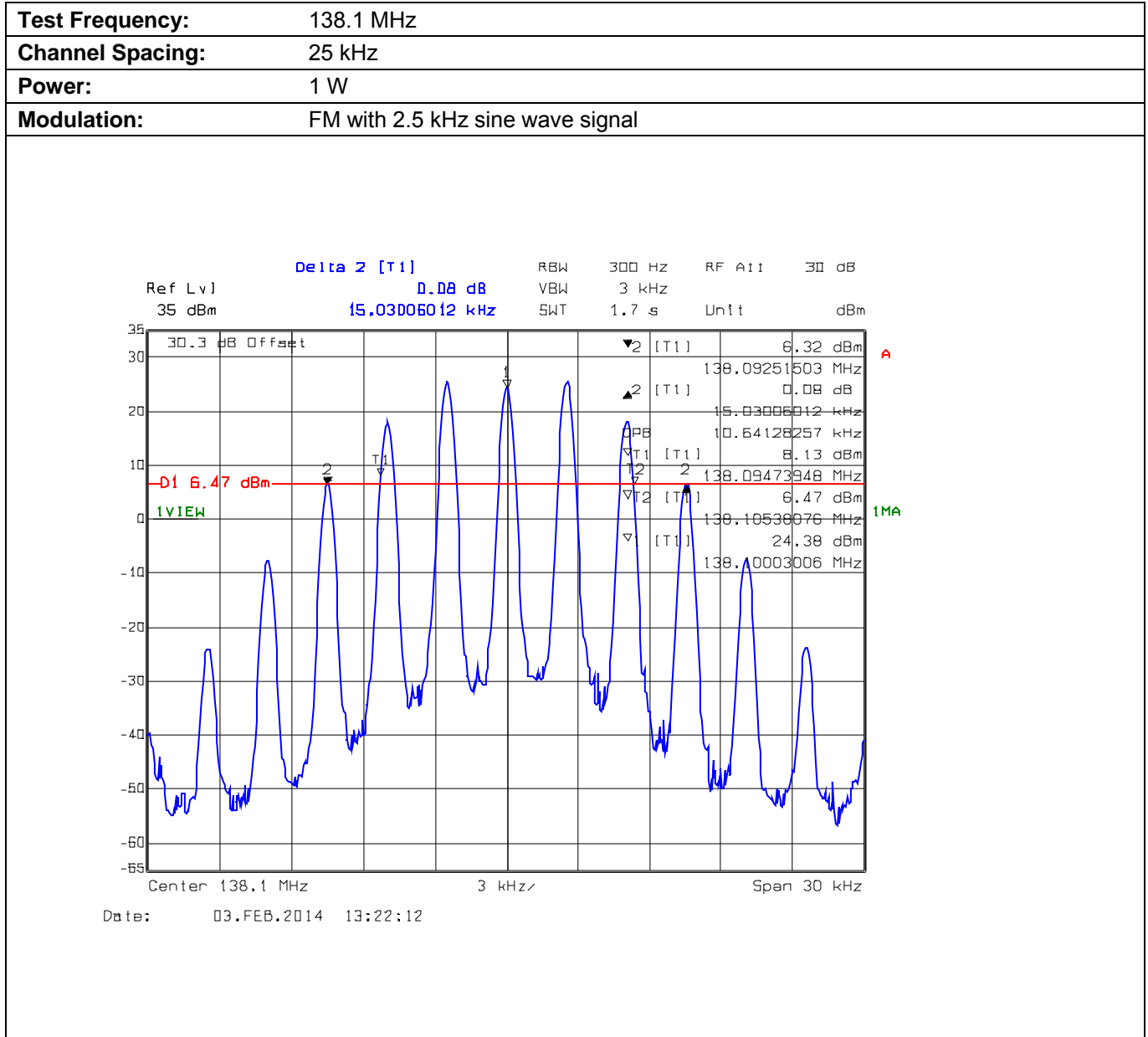
Plot 5.8.4.1.4. Occupied Bandwidth
