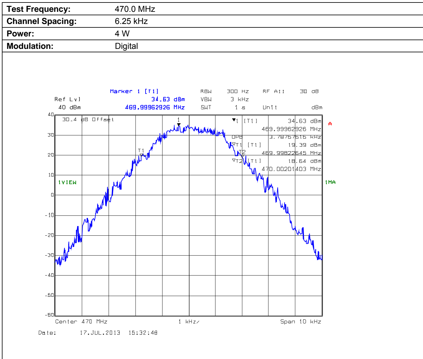
Plot 5.8.4.1.8. Occupied Bandwidth
