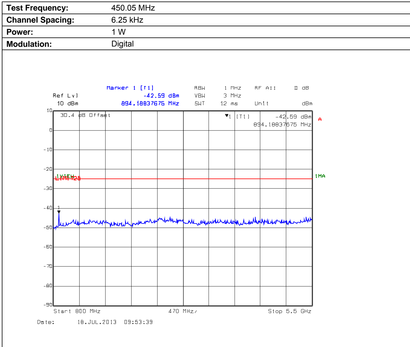
Plot 5.9.4.1.4. Conducted Transmitter Spurious Emissions for 450.05 MHz, Low Power, 800 MHz - 5.5 GHz
