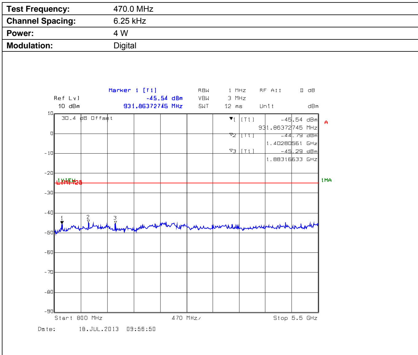
Plot 5.9.4.2.2. Conducted Transmitter Spurious Emissions for 470.0 MHz, High Power, 800 MHz - 5.5 GHz
