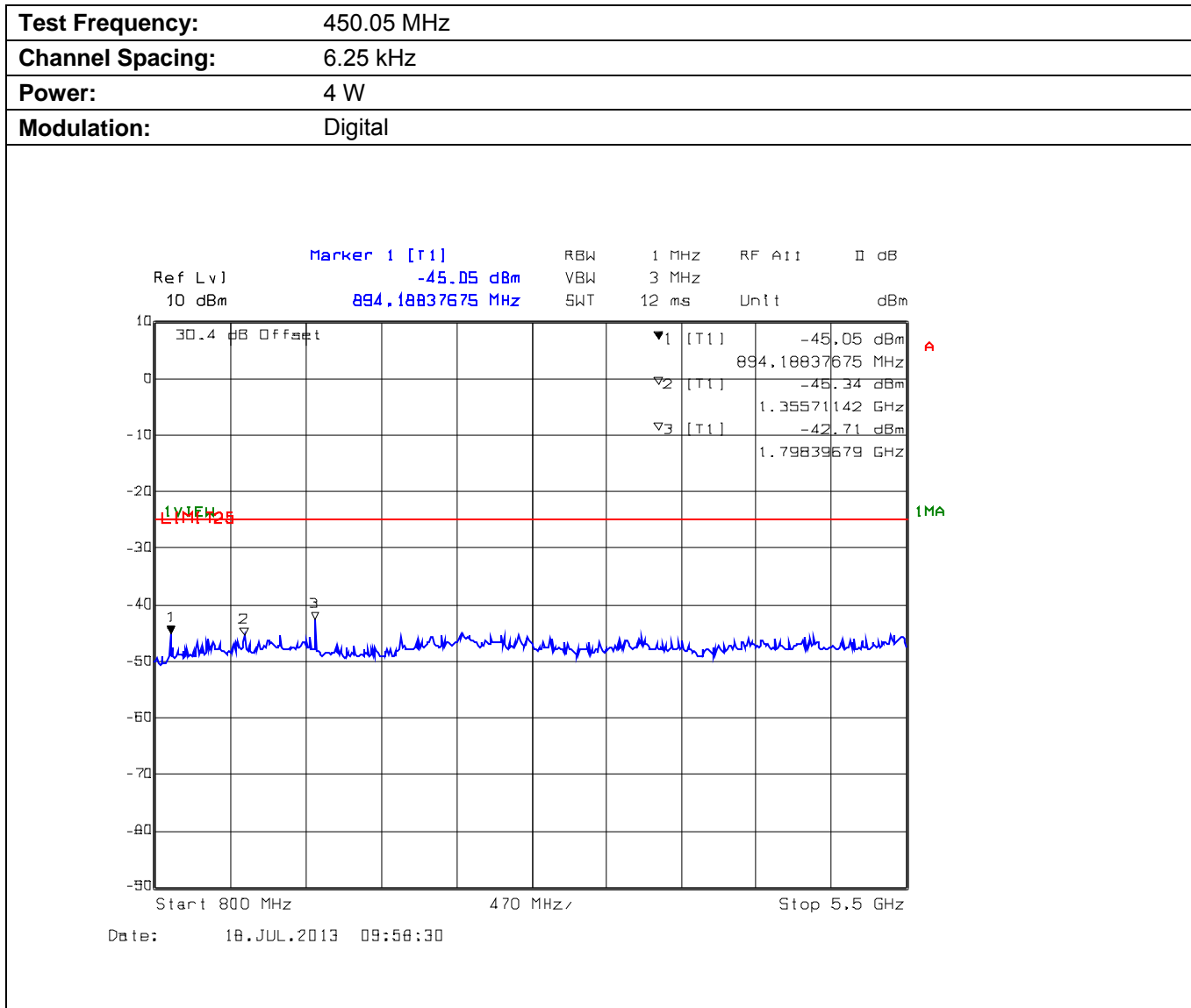
Plot 5.9.4.1.2. Conducted Transmitter Spurious Emissions for 450.05 MHz, High Power, 800 MHz - 5.5 GHz
