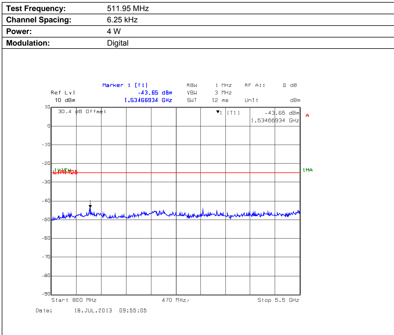
Plot 5.9.4.3.2. Conducted Transmitter Spurious Emissions for 511.95 MHz, High Power, 800 MHz - 5.5 GHz
