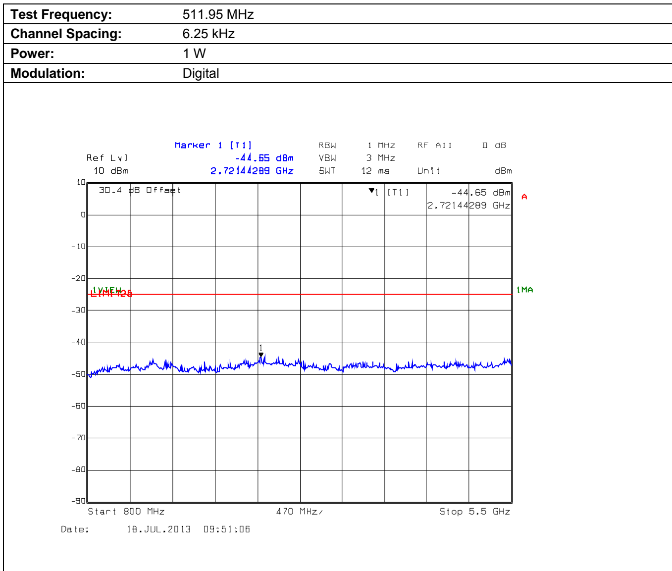
Plot 5.9.4.3.4. Conducted Transmitter Spurious Emissions for 511.95 MHz, Low Power, 800 MHz - 5.5 GHz
