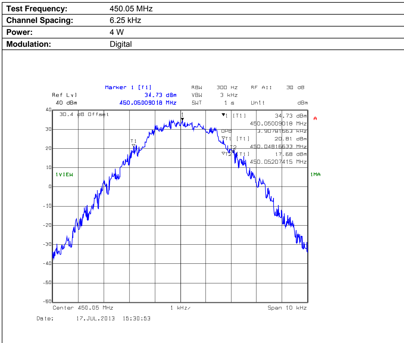
Plot 5.8.4.1.7. Occupied Bandwidth
