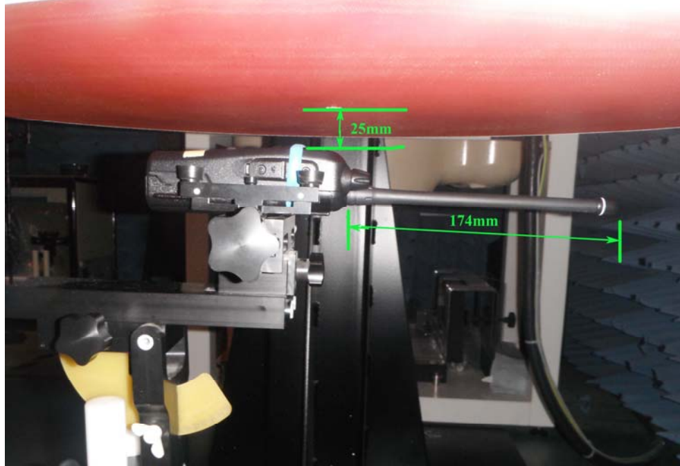
< FA-SC61VC cut antenna with the length of 174mm >
