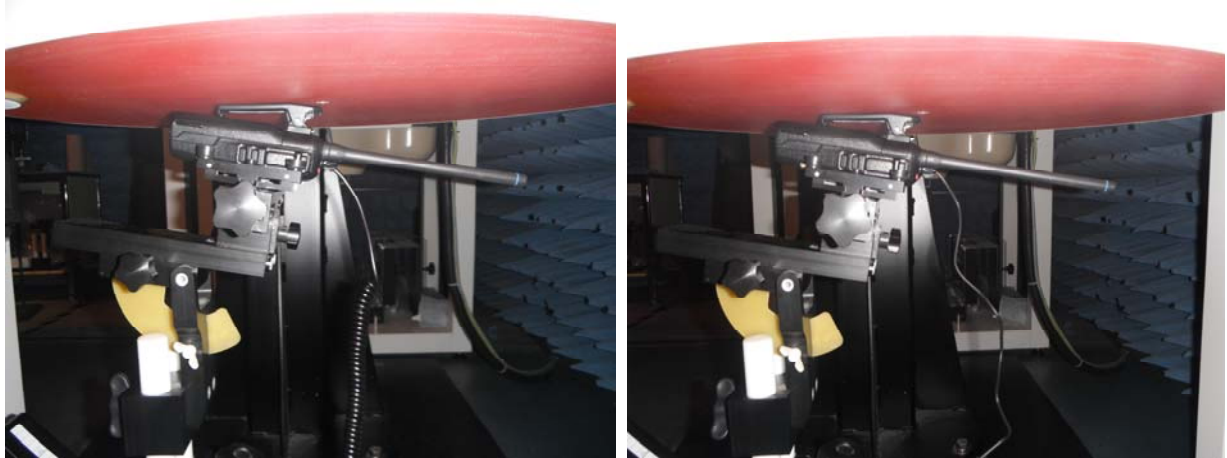
Back side of EUT in parallel to the phantom with the belt-clip (M/N: MB-94R) in contact, attached HM-158LA Speaker Microphone and HM-166LA Earphone Microphone
