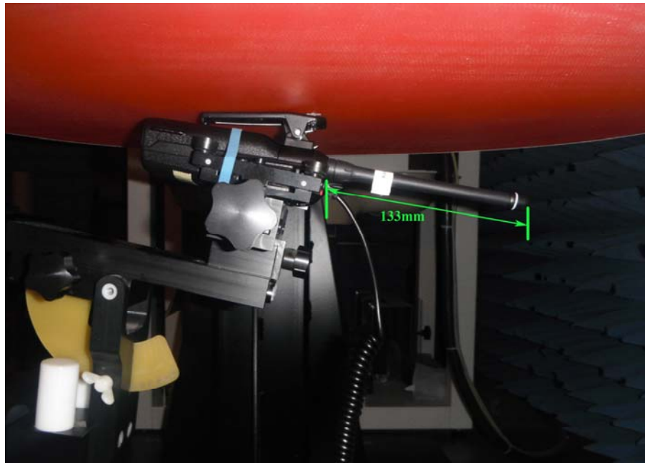
< FA-SC61VC cut antenna with the length of 133mm >
