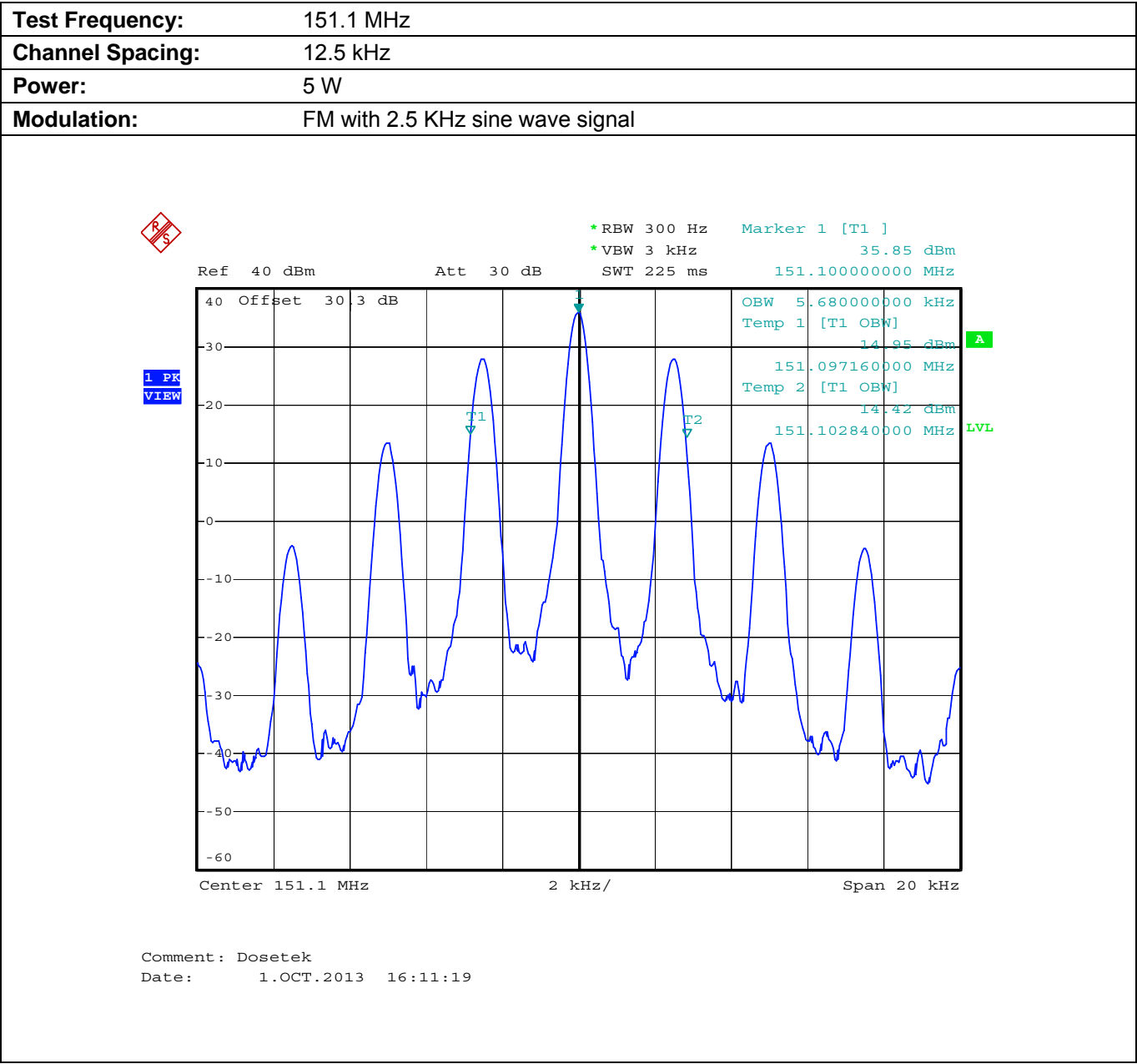
Plot 5.8.4.1.2. Occupied Bandwidth
