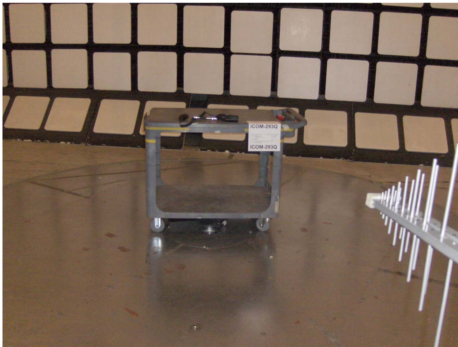
Radiated Transmitter Emission Test at 3m (Orthogonal Position 2)
