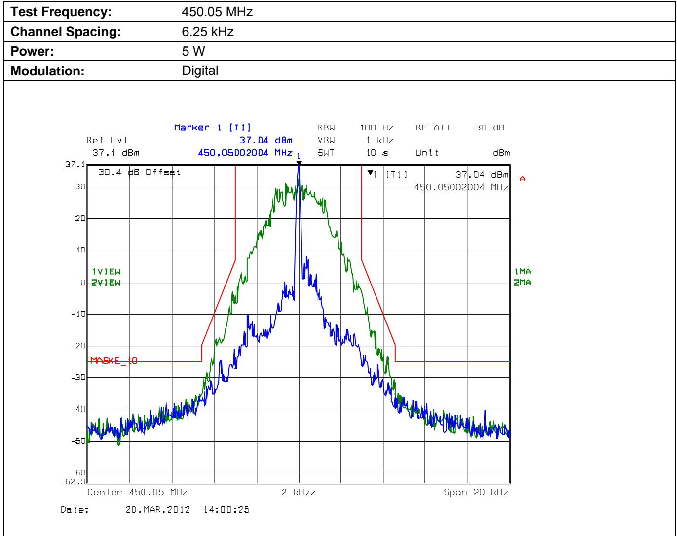
Plot 5.4.4.4.1. Emission Mask E, High Power
