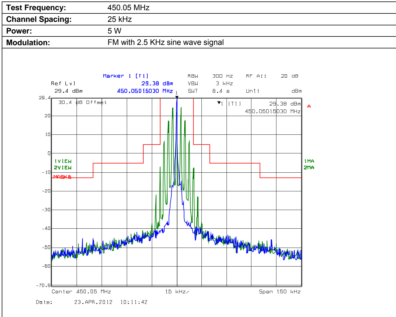
Plot 5.4.4.2.4. Emission Mask B (not for FCC Certification purpose), Low Power
