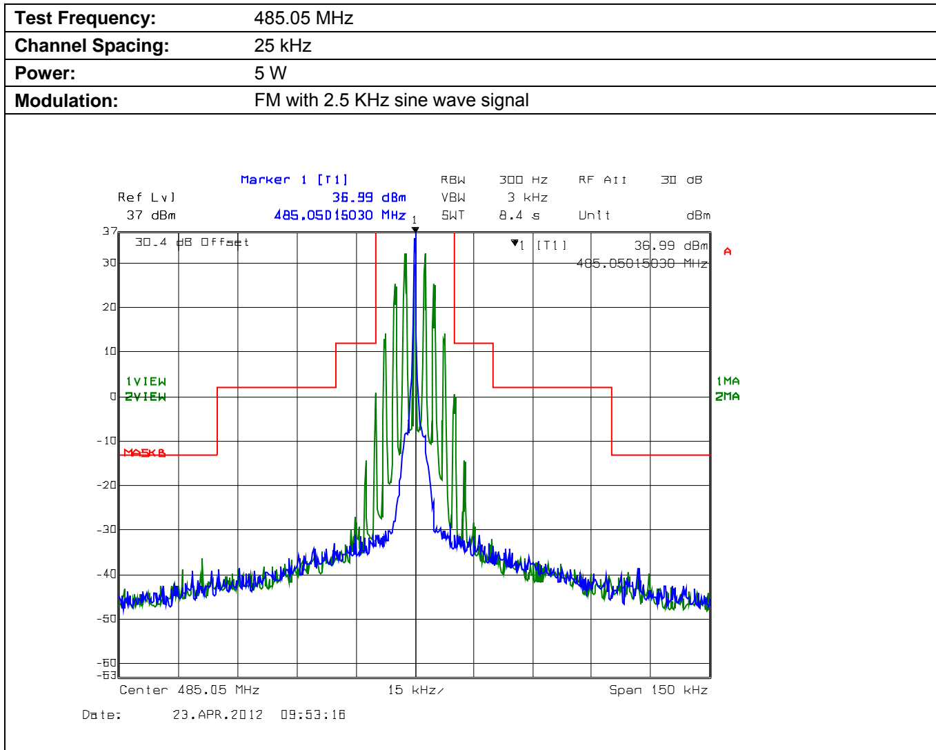
Plot 5.4.4.2. Emission Mask B (not for FCC Certification purpose), High Power
