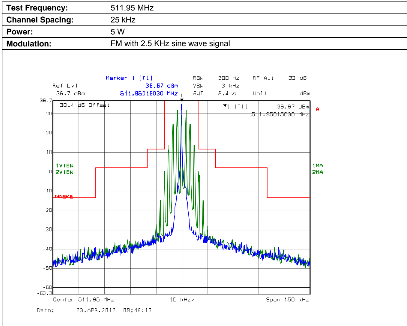
Plot 5.4.4.2.3. Emission Mask B (not for FCC Certification purpose), High Power
