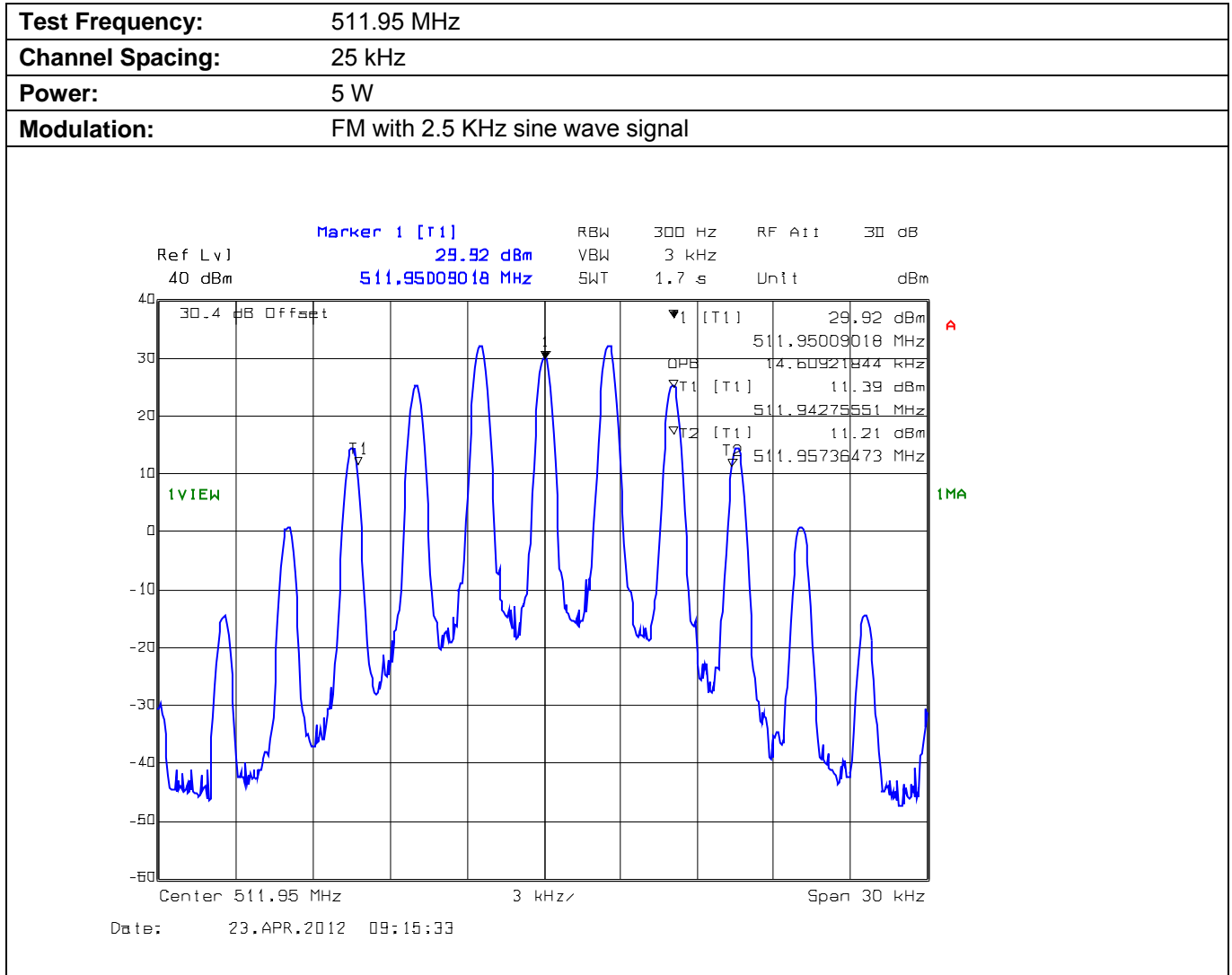
Plot 5.4.4.1.3. Occupied Bandwidth
