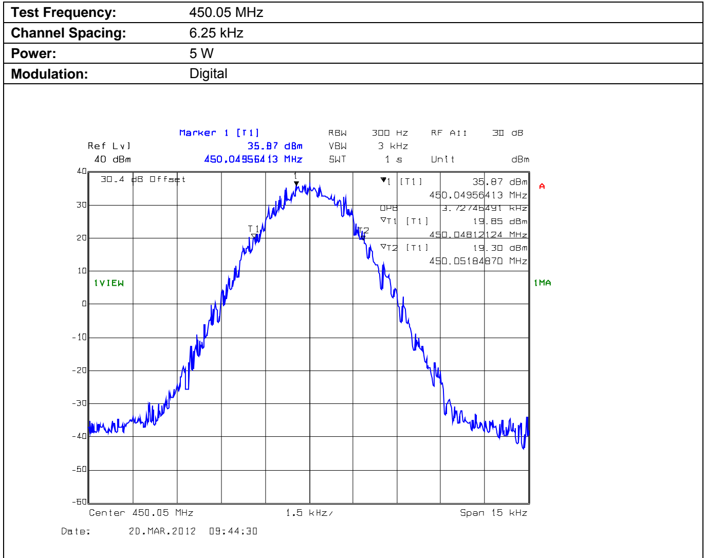
Plot 5.4.4.1.7. Occupied Bandwidth
