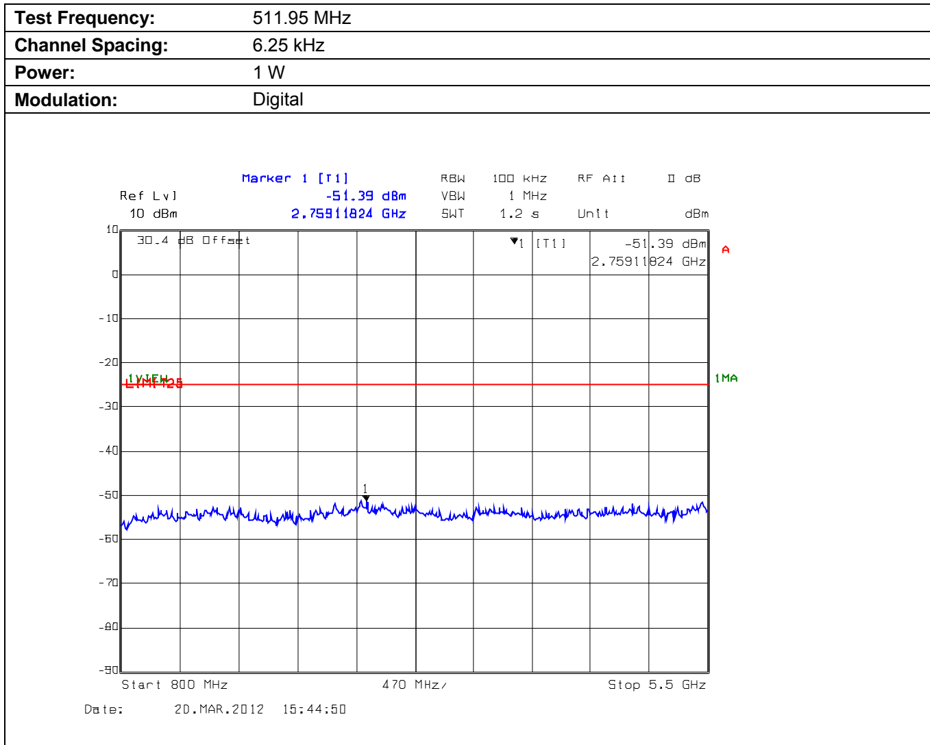
Plot 5.5.4.3.4. Conducted Transmitter Spurious Emissions for 511.95 MHz, Low Power, 800 MHz - 5.5 GHz
