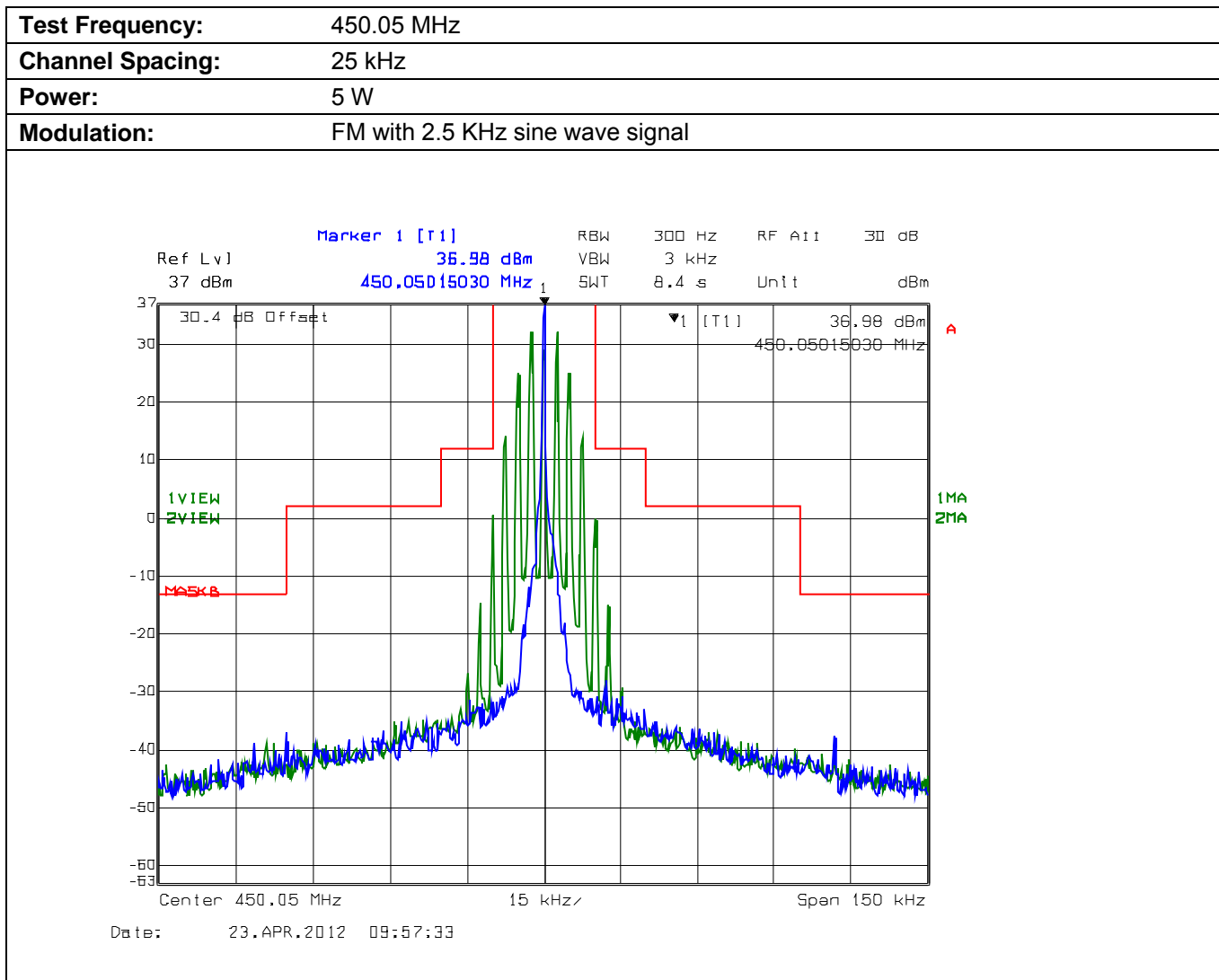
Plot 5.4.4.2.1. Emission Mask B (not for FCC Certification purpose), High Power
