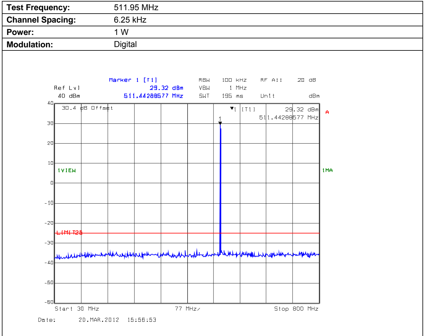
Plot 5.5.4.3.3. Conducted Transmitter Spurious Emissions for 511.95 MHz, Low Power, 30 - 800 MHz
