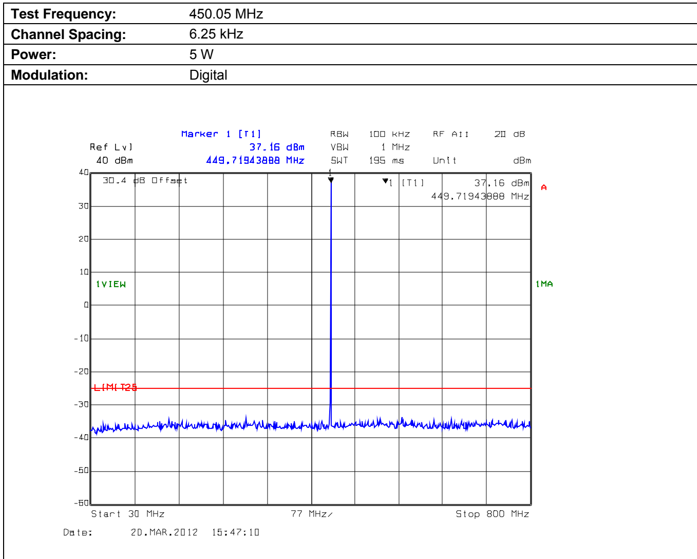
Plot 5.5.4.1.1. Conducted Transmitter Spurious Emissions for 450.05 MHz, High Power, 30 - 800 MHz
