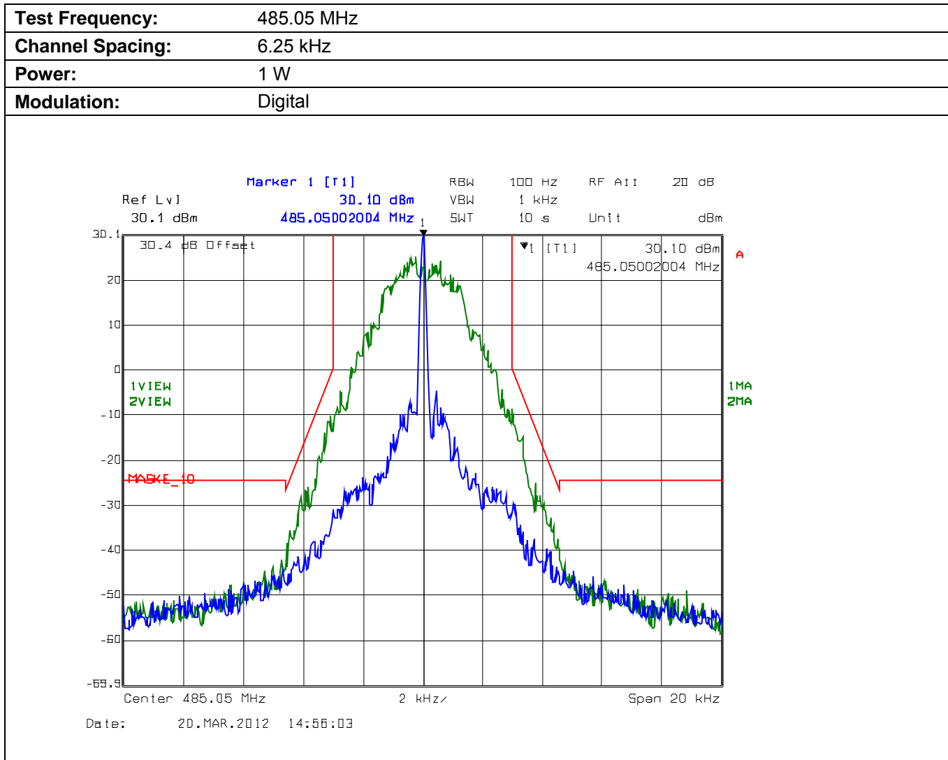
Plot 5.4.4.4.5. Emission Mask E, Low Power
