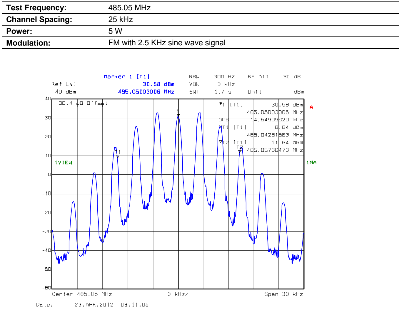
Plot 5.4.4.1.2. Occupied Bandwidth
