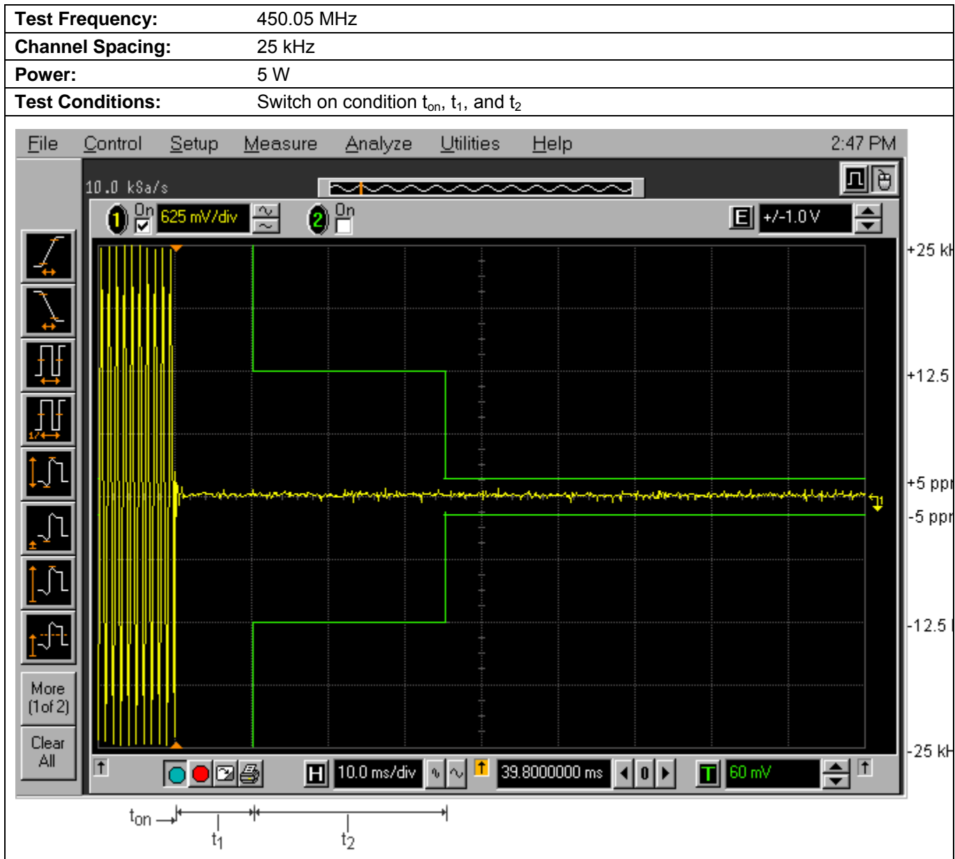
Plot 5.8.4.1. Transient Frequency Behavior for 25 kHz Channel Spacing (Not for FCC Certification purpose)
