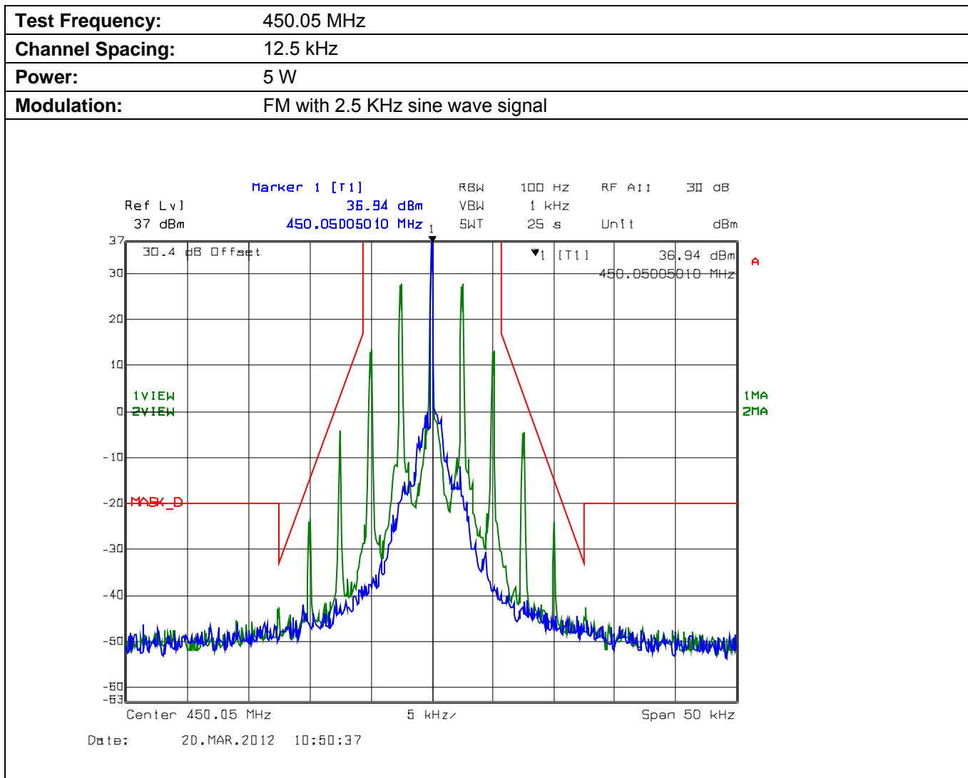
Plot 5.4.4.3.1. Emission Mask D, High Power
