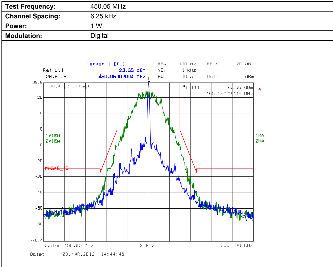
Plot 5.4.4.4. Emission Mask E, Low Power
