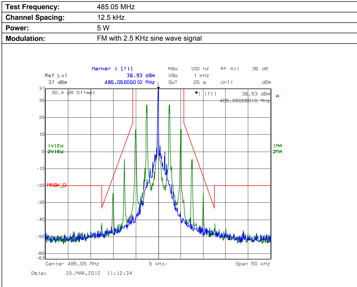
Plot 5.4.4.3.2. Emission Mask D, High Power
