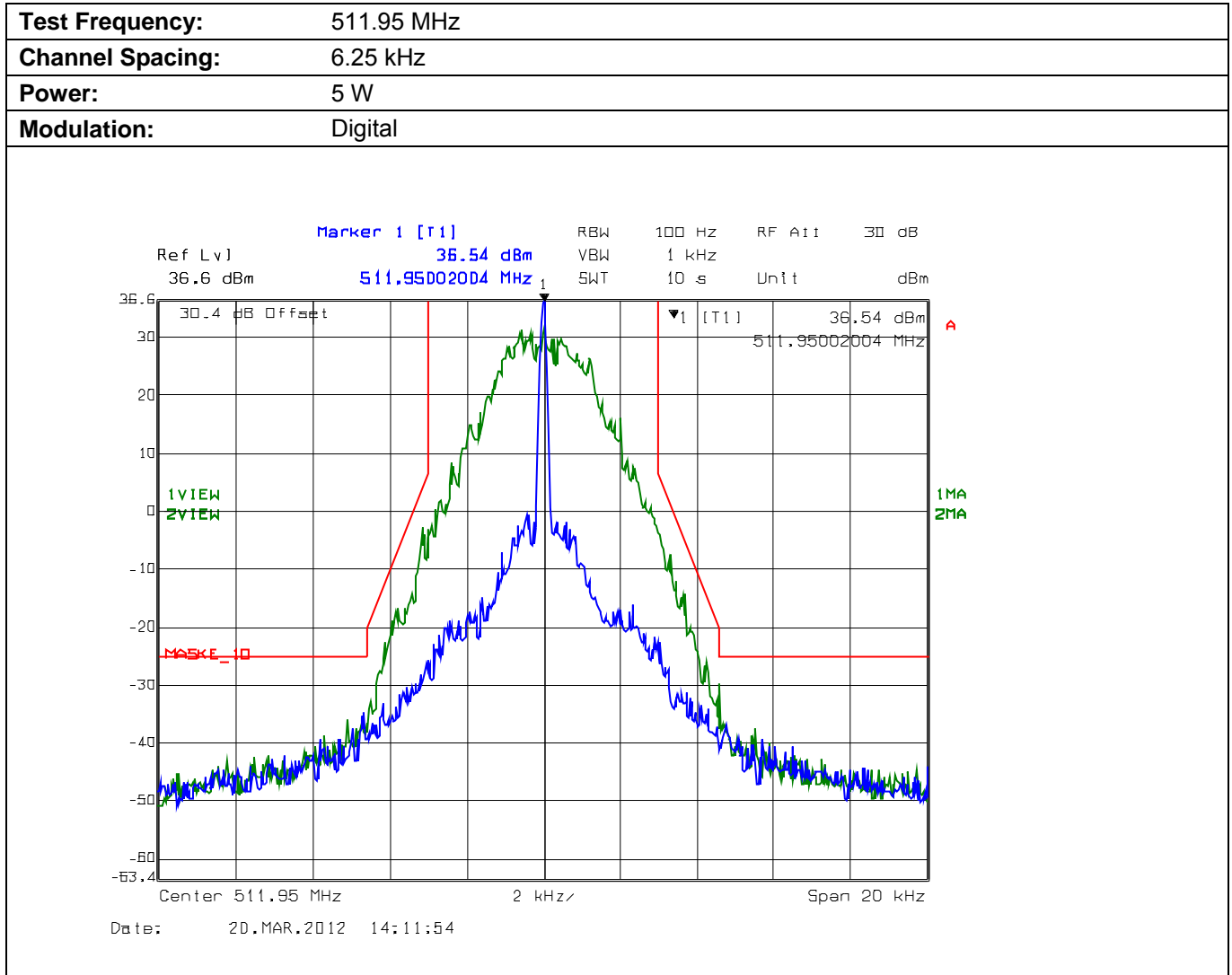
Plot 5.4.4.3. Emission Mask E, High Power
