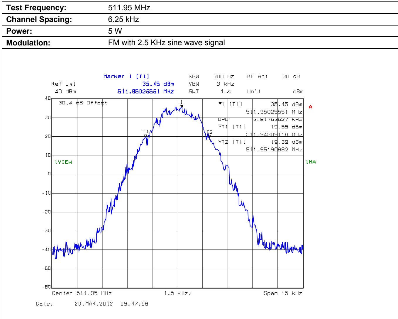
Plot 5.4.4.1.9. Occupied Bandwidth
