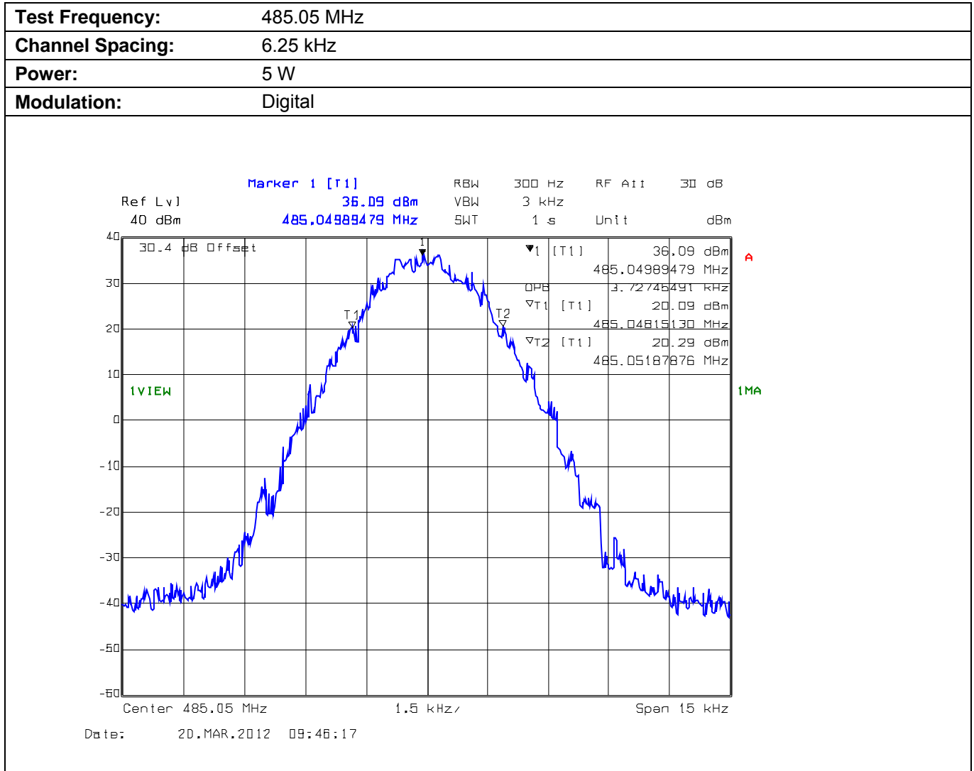
Plot 5.4.4.1.8. Occupied Bandwidth
