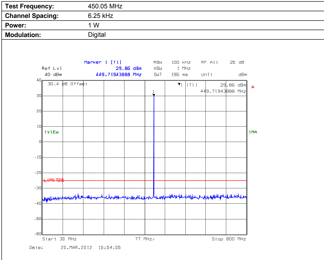
Plot 5.5.4.1.3. Conducted Transmitter Spurious Emissions for 450.05 MHz, Low Power, 30 - 800 MHz
