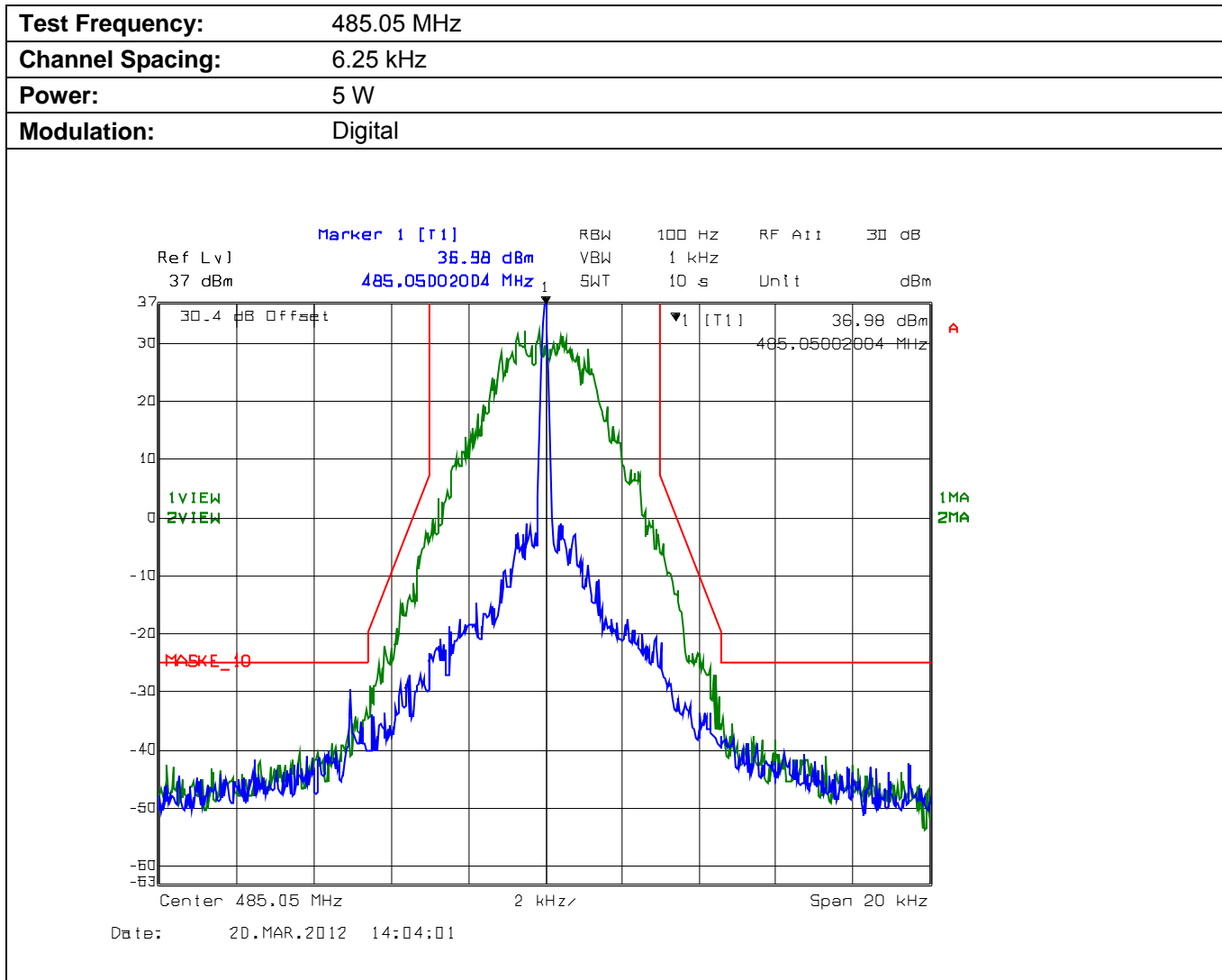
Plot 5.4.4.2. Emission Mask E, High Power
