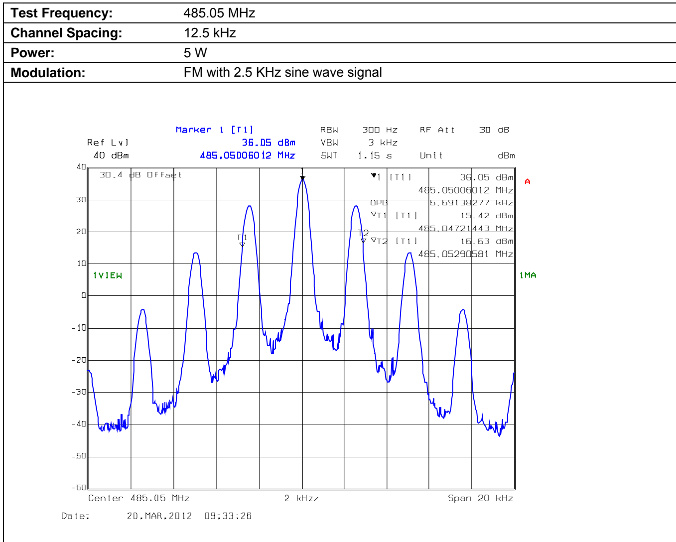
Plot 5.4.4.1.5. Occupied Bandwidth
