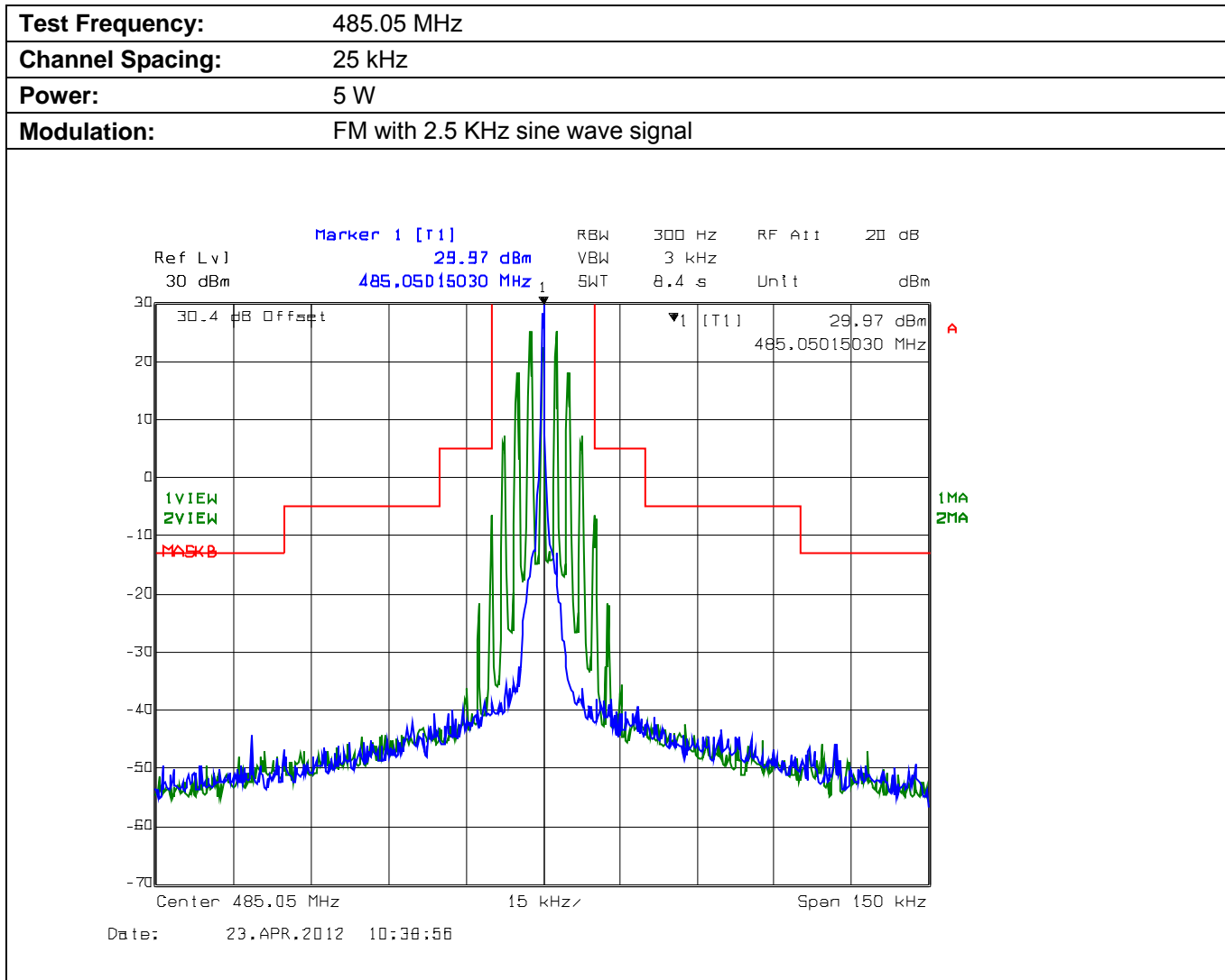
Plot 5.4.4.2.5. Emission Mask B (not for FCC Certification purpose), Low Power
