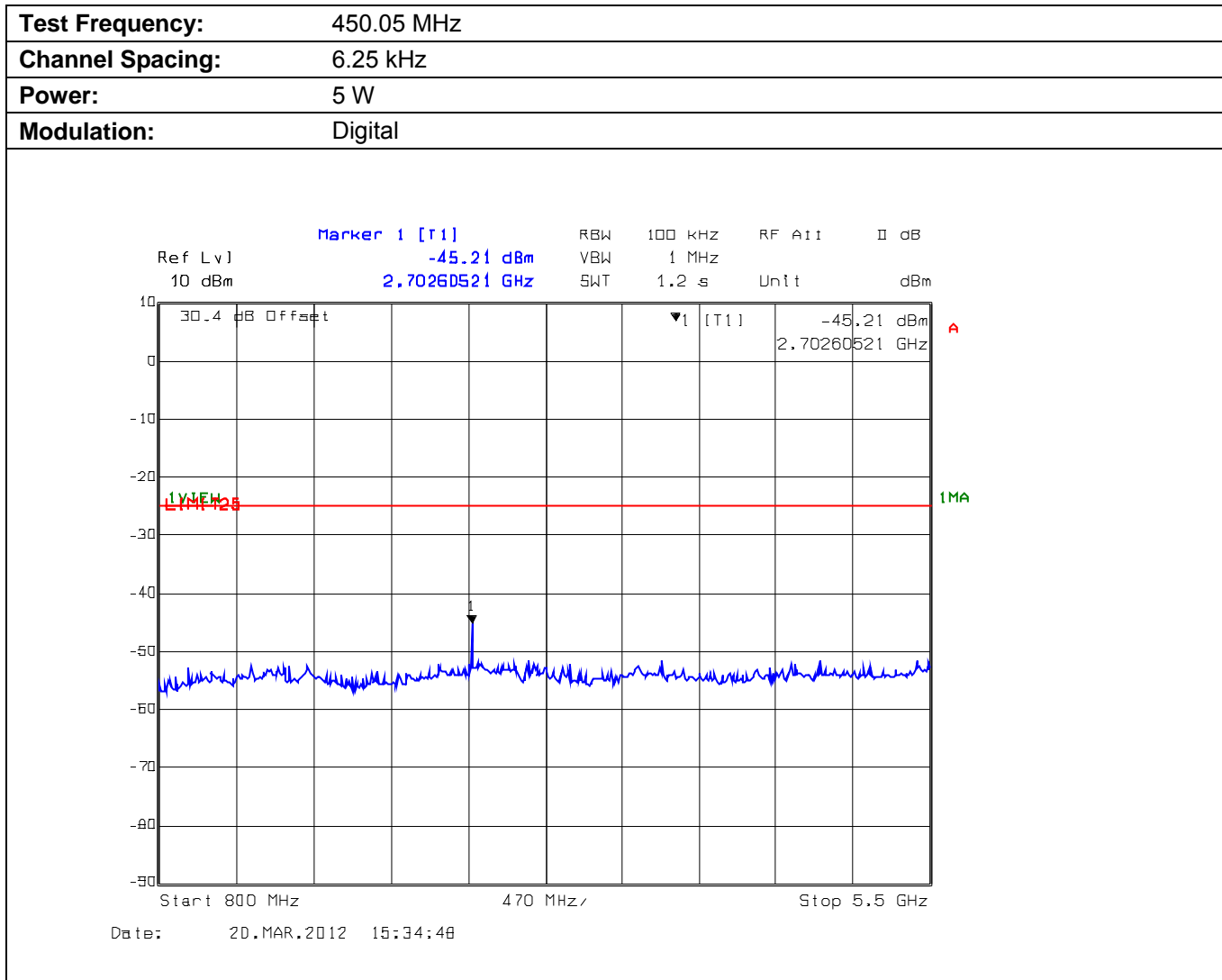
Plot 5.5.4.1.2. Conducted Transmitter Spurious Emissions for 450.05 MHz, High Power, 800 MHz - 5.5 GHz
