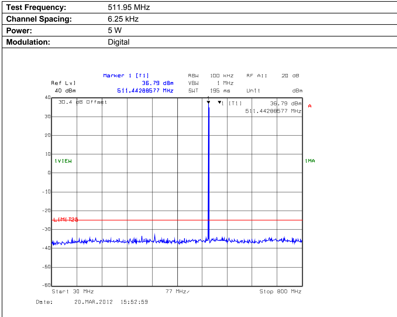
Plot 5.5.4.3.1. Conducted Transmitter Spurious Emissions for 511.95 MHz, High Power, 30 - 800 MHz
