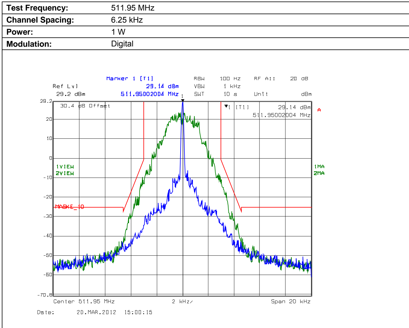
Plot 5.4.4.4.6. Emission Mask E, Low Power
