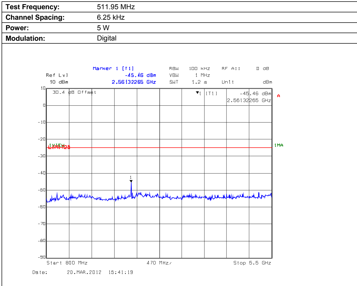
Plot 5.5.4.3.2. Conducted Transmitter Spurious Emissions for 511.95 MHz, High Power, 800 MHz - 5.5 GHz
