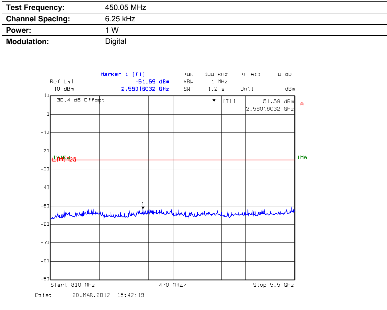
Plot 5.5.4.1.4. Conducted Transmitter Spurious Emissions for 450.05 MHz, Low Power, 800 MHz - 5.5 GHz
