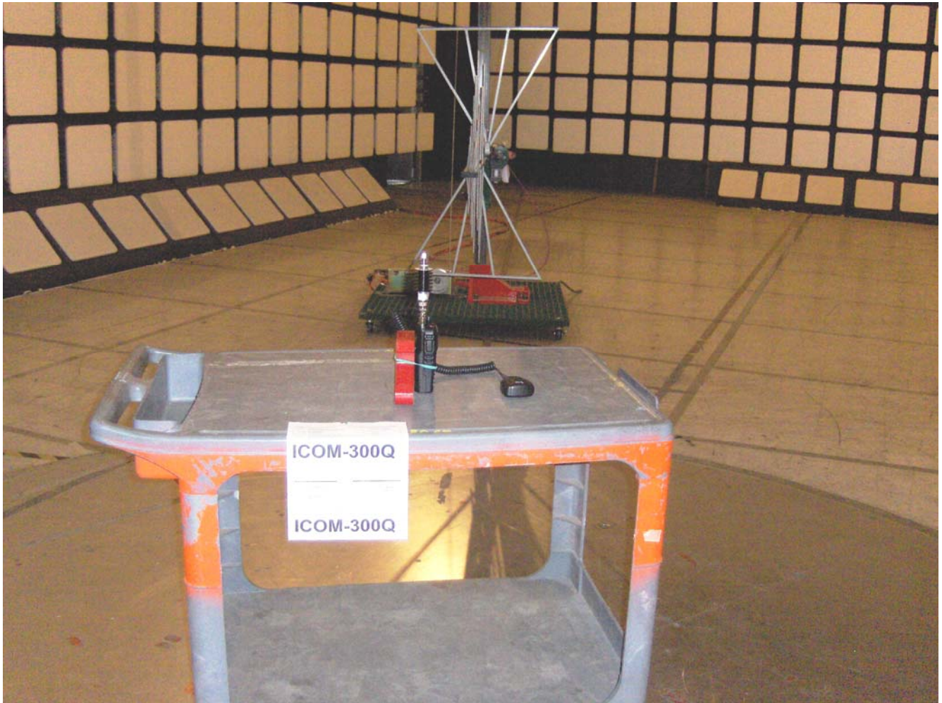
Plot #1: Tx Radiated Emission Test Setup
