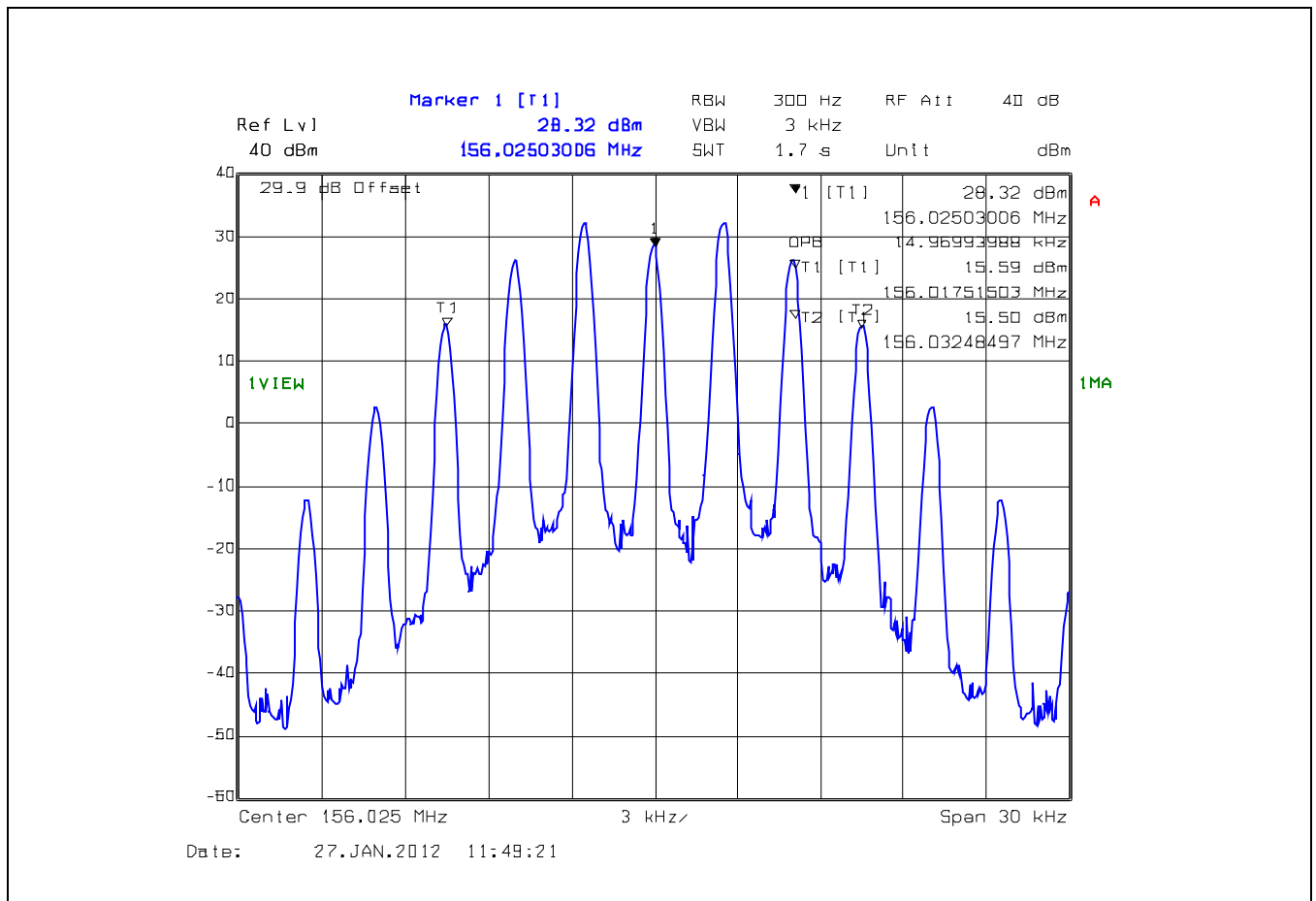
Plot 5.4.4.1.1. Occupied Bandwidth for 156.025 MHz, 25 kHz Channel Spacing, High Power (5 W), G3E
