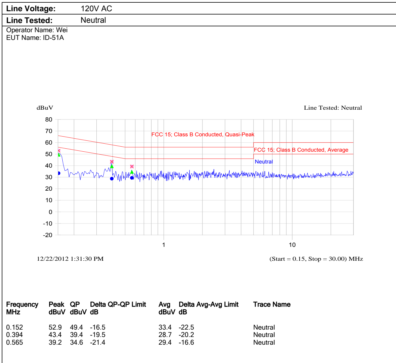
Plot 2: AC Power Line Conducted Emissions
