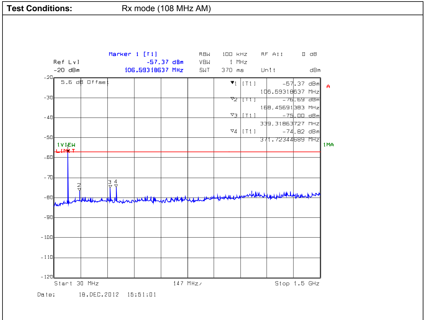
Plot 3: Conducted Receiver Spurious Emissions, 30 MHz – 1.5 GHz
