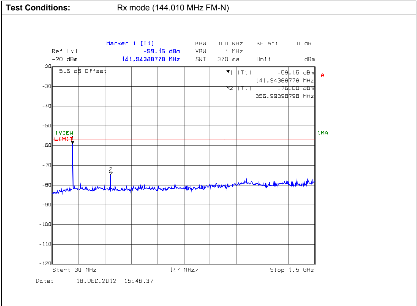
Plot 4: Conducted Receiver Spurious Emissions, 30 MHz – 1.5 GHz
