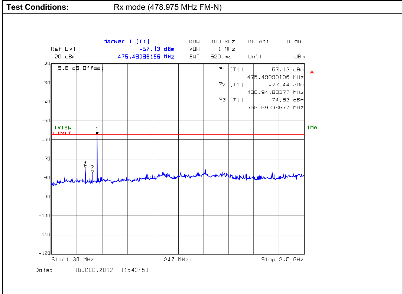
Plot 8: Conducted Receiver Spurious Emissions, 30 MHz – 2.5 GHz
