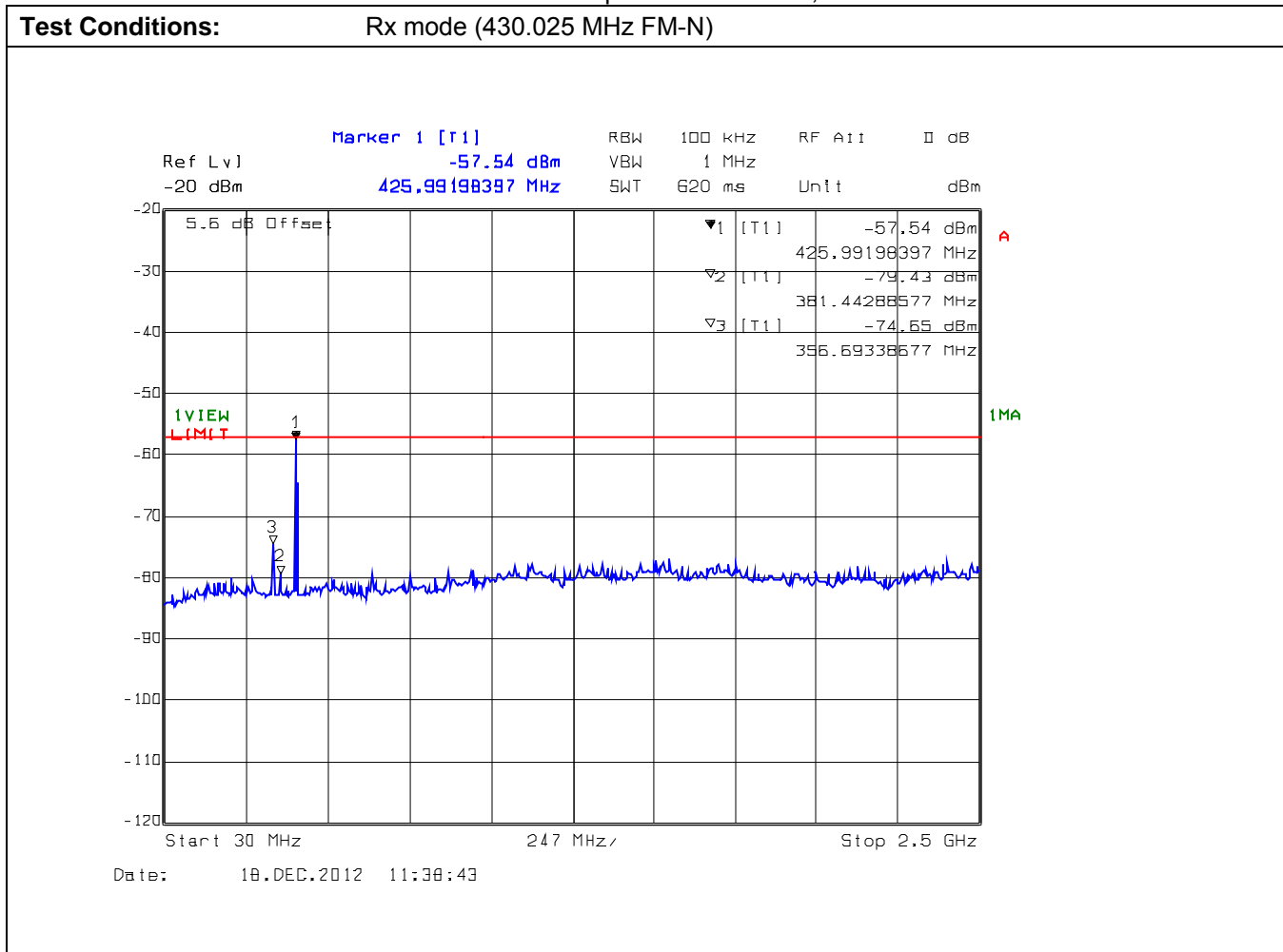
Plot 7: Conducted Receiver Spurious Emissions, 30 MHz – 2.5 GHz
