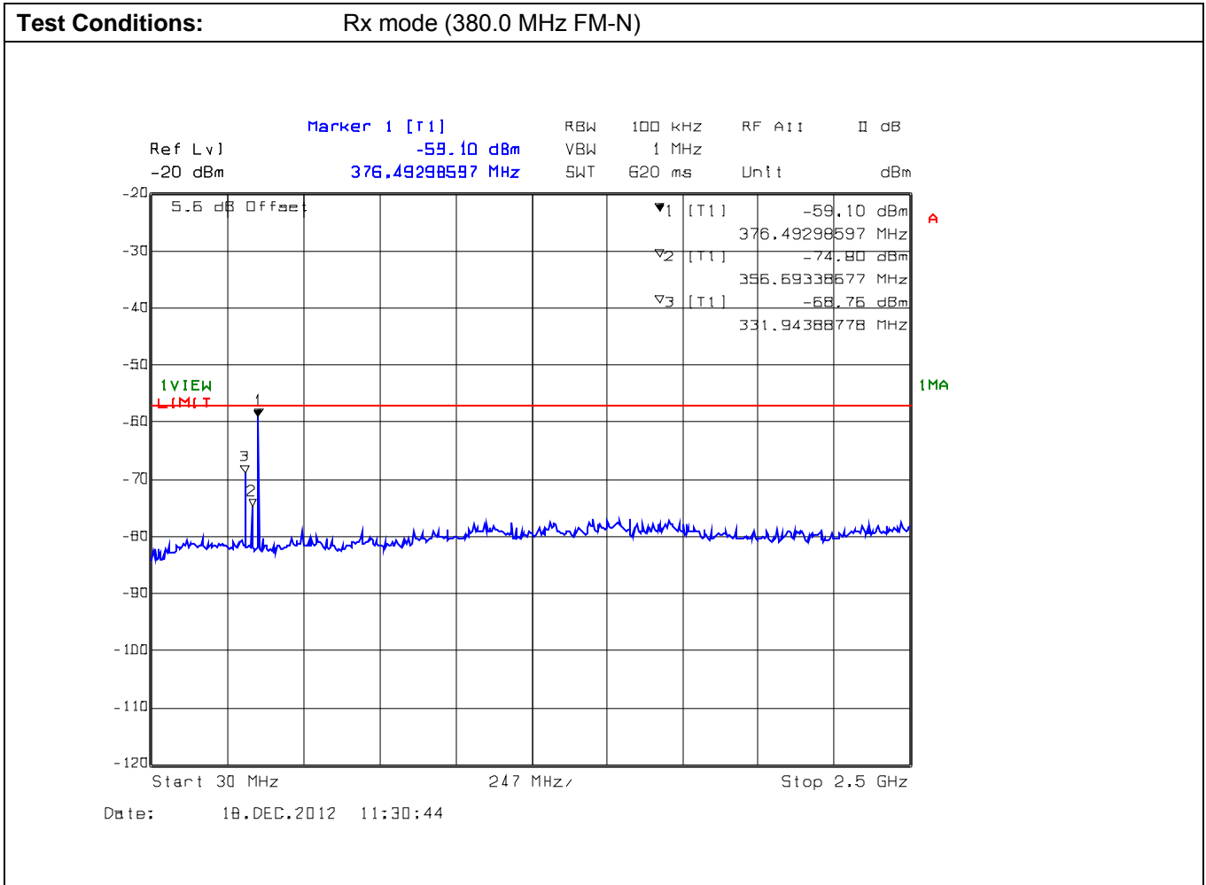
Plot 6: Conducted Receiver Spurious Emissions, 30 MHz – 2.5 GHz
