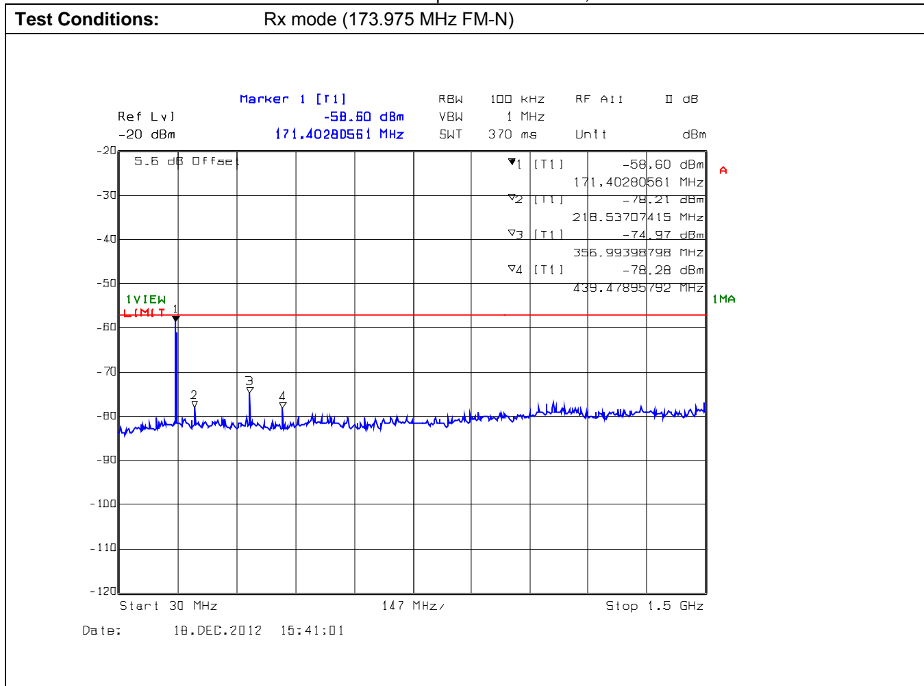
Plot 5: Conducted Receiver Spurious Emissions, 30 MHz – 1.5 GHz
