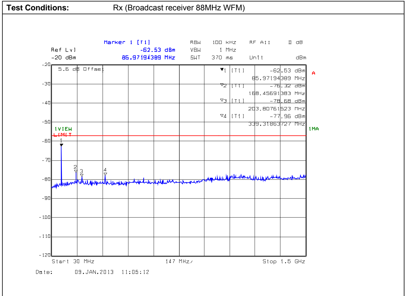
Plot 9: Conducted Receiver Spurious Emissions, 30 MHz – 1.5 GHz
