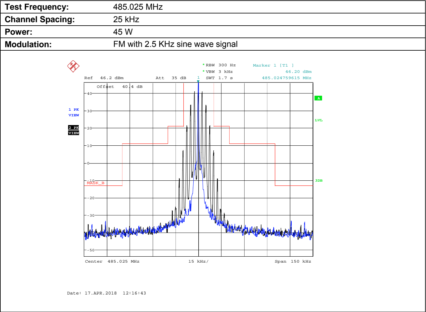
Plot 5.8.4.3.3. Emission Mask B, High Power
