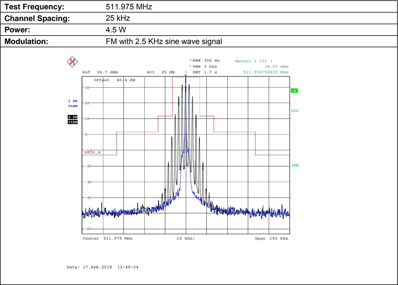
Plot 5.8.4.3.6. Emission Mask B, Low Power
