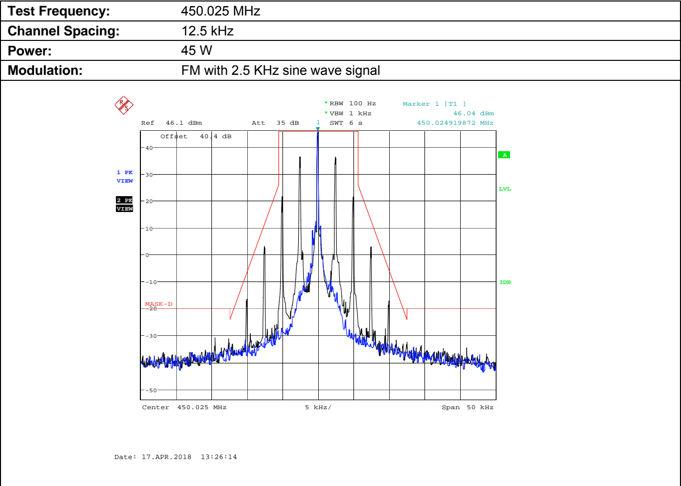
Plot 5.8.4.2.1. Emission Mask D, High Power
