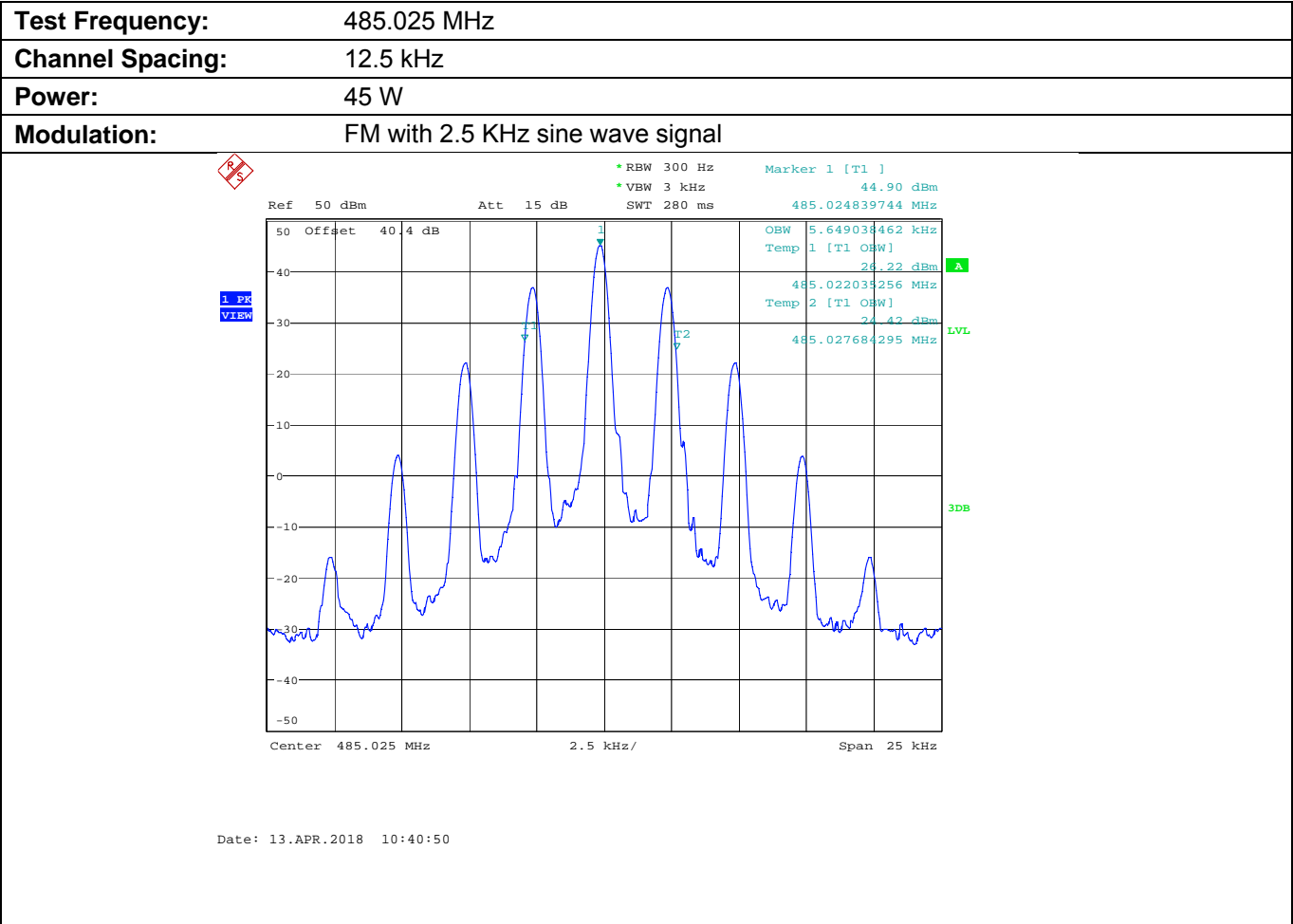
Plot 5.8.4.1.5. Occupied Bandwidth
