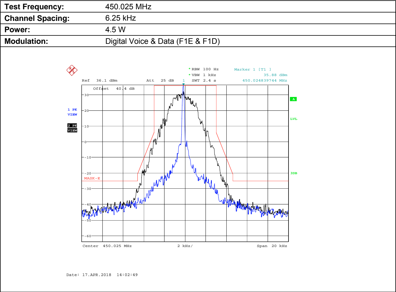
Plot 5.8.4.4.2. Emission Mask E, Low Power
