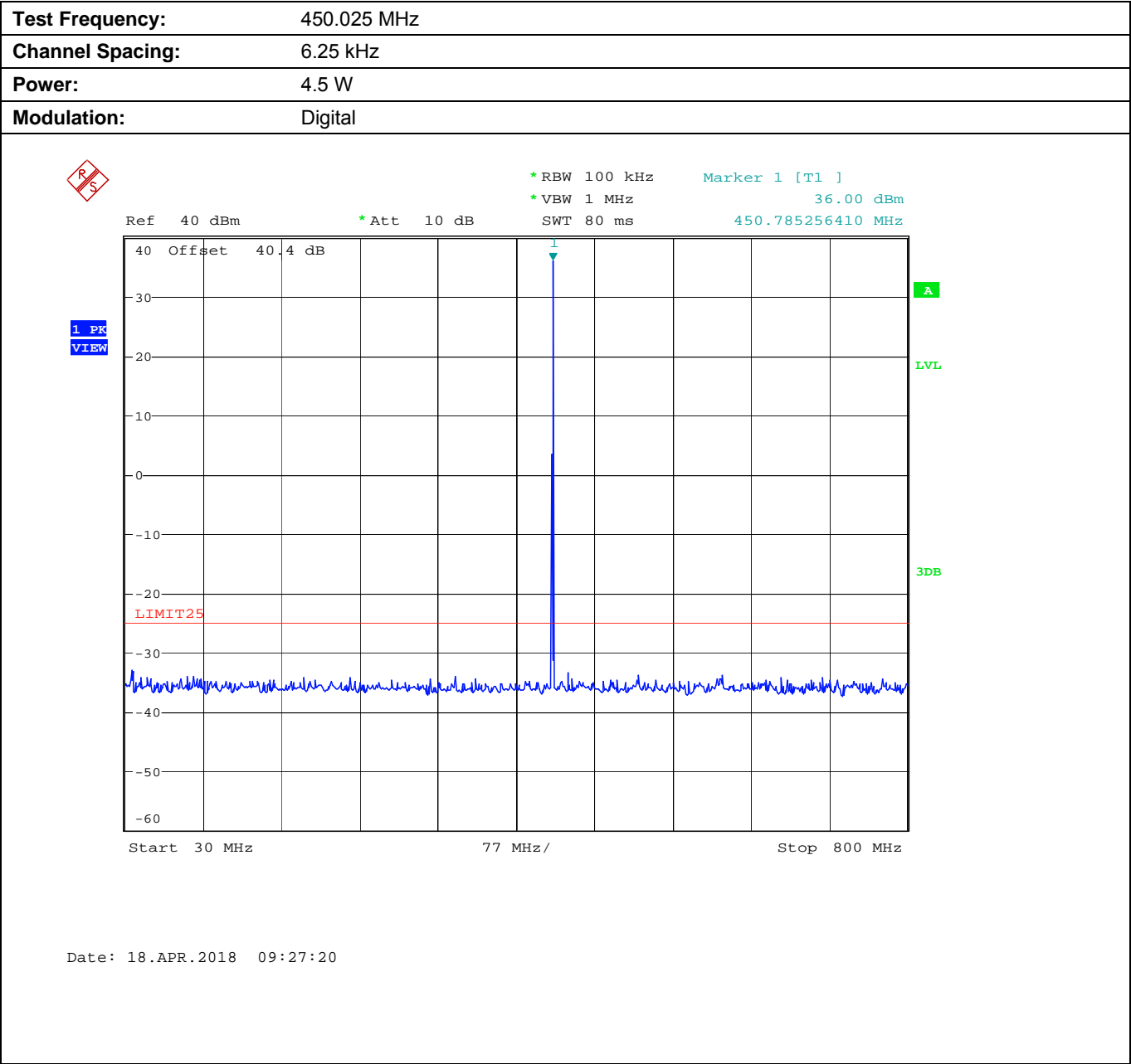
Plot 5.9.4.1.3. Conducted Transmitter Spurious Emissions for 450.025 MHz, Low Power, 30 - 800 MHz
