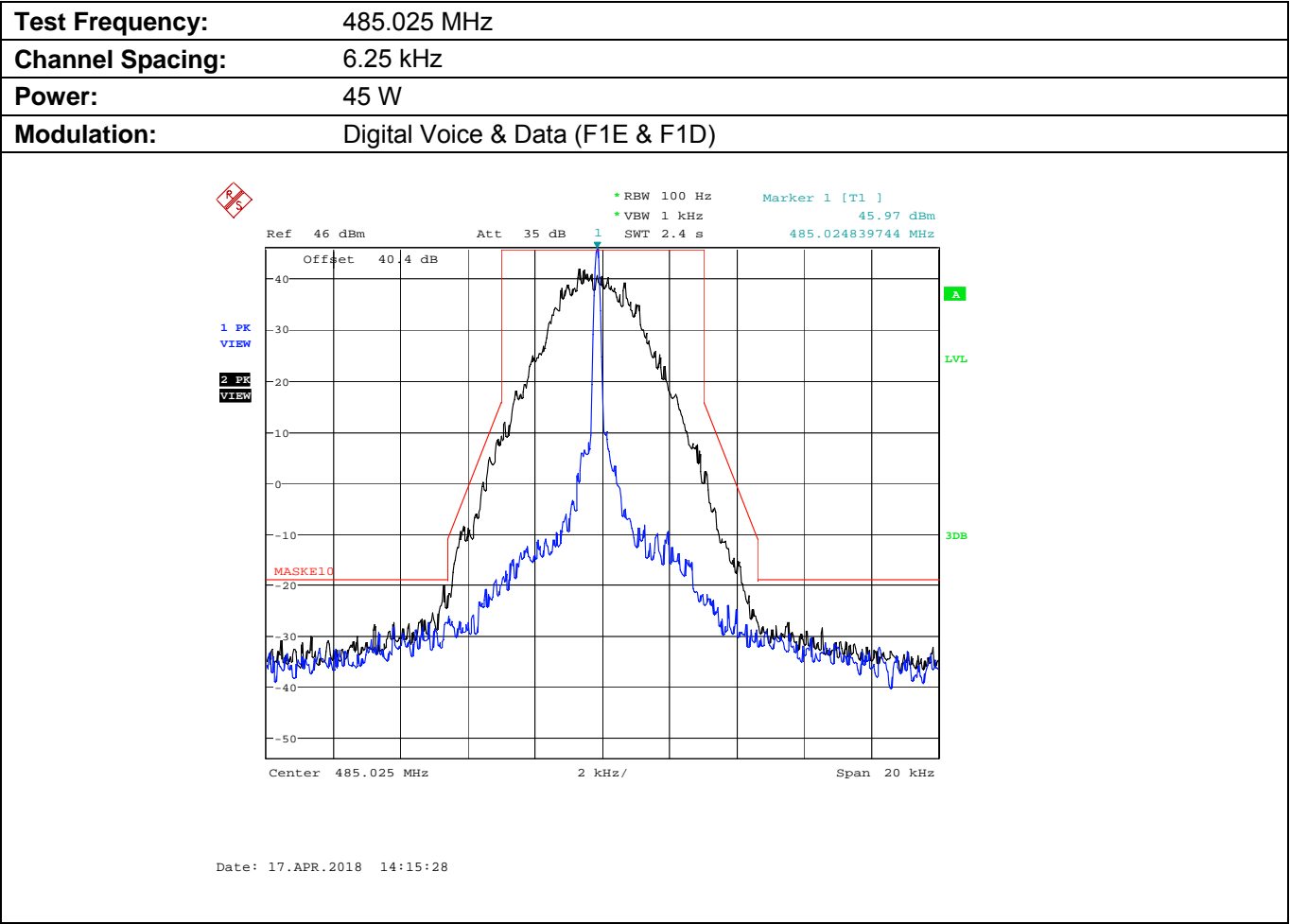
Plot 5.8.4.4.3. Emission Mask E, High Power
