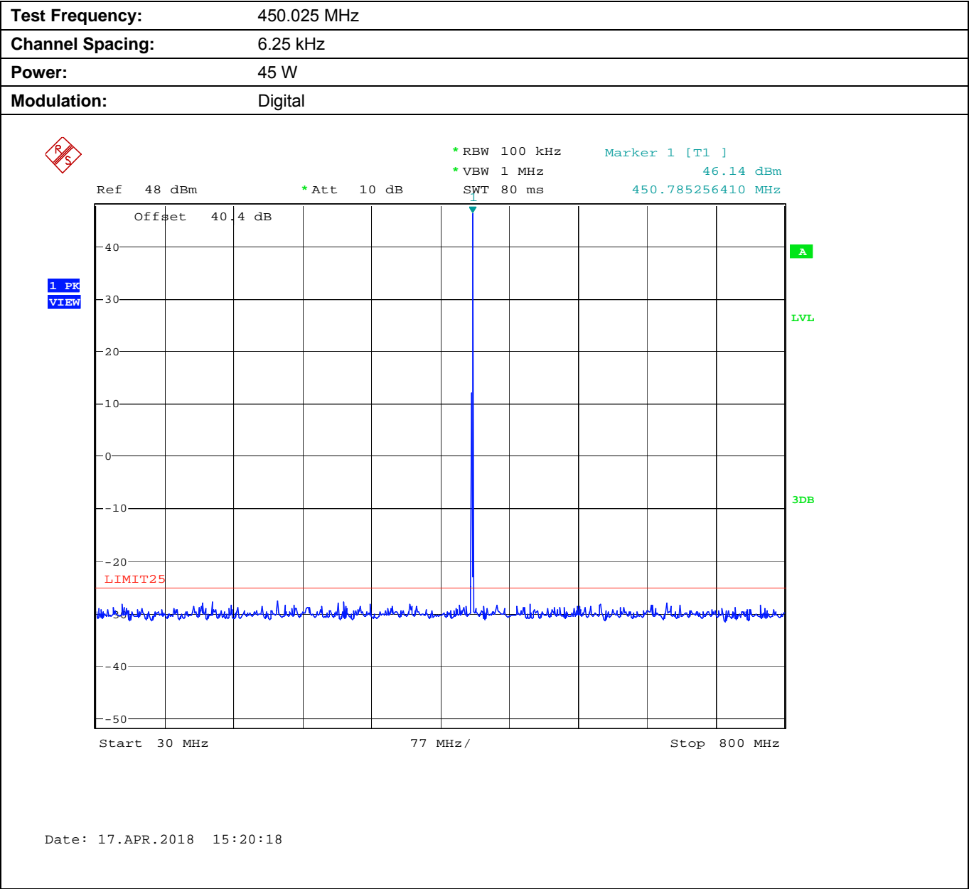
Plot 5.9.4.1.1. Conducted Transmitter Spurious Emissions for 450.025 MHz, High Power, 30 - 800 MHz
