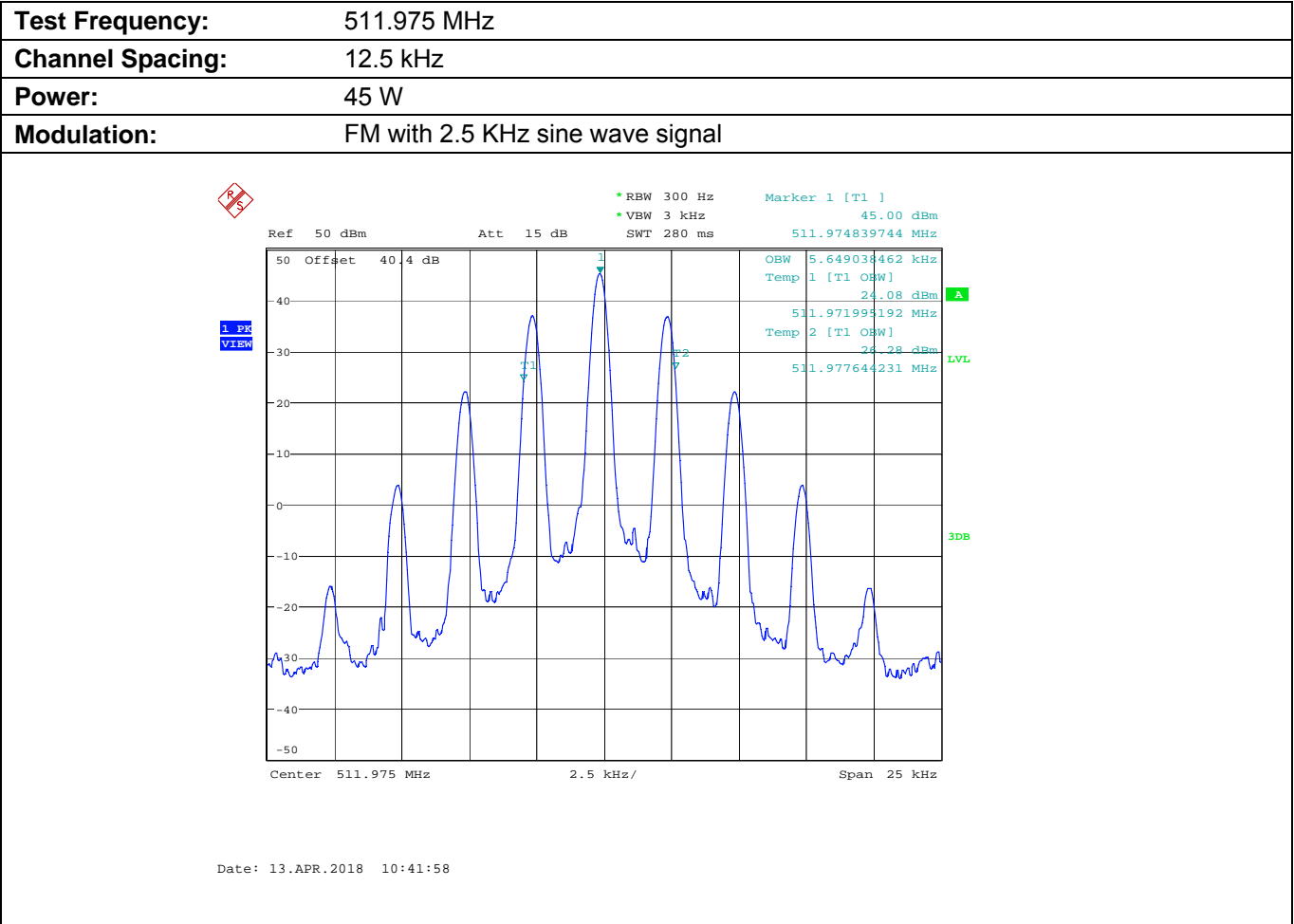
Plot 5.8.4.1.6. Occupied Bandwidth
