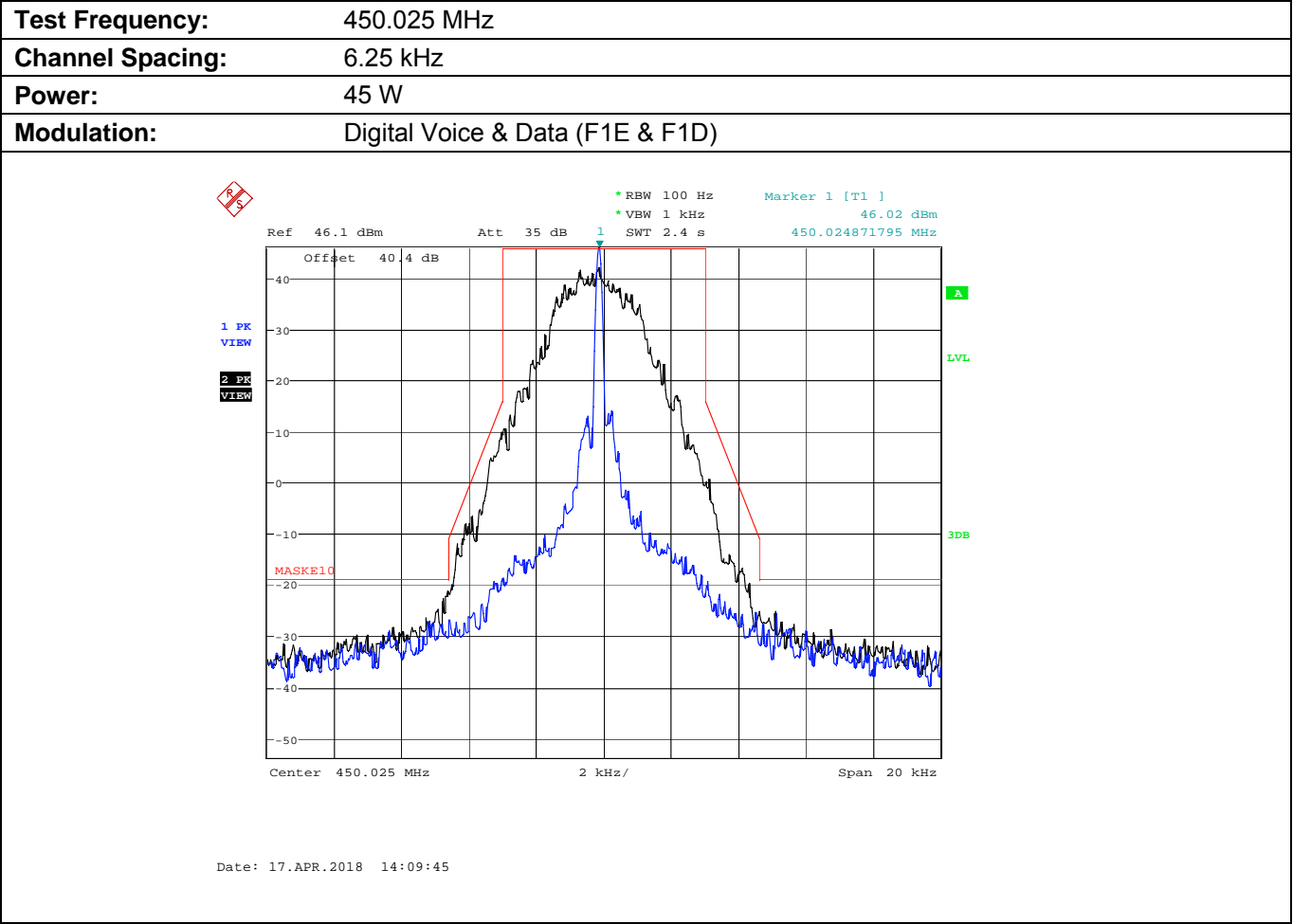
Plot 5.8.4.4.1. Emission Mask E, High Power
