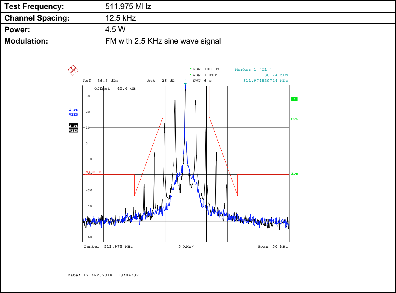
Plot 5.8.4.2.6. Emission Mask D, Low Power
