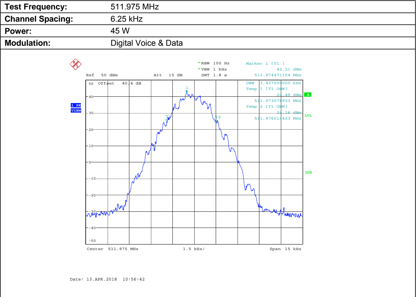
Plot 5.8.4.1.9. Occupied Bandwidth
