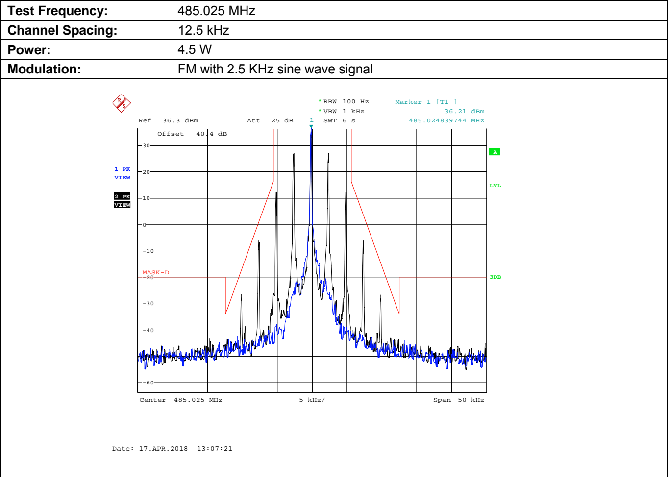
Plot 5.8.4.2.4. Emission Mask D, Low Power
