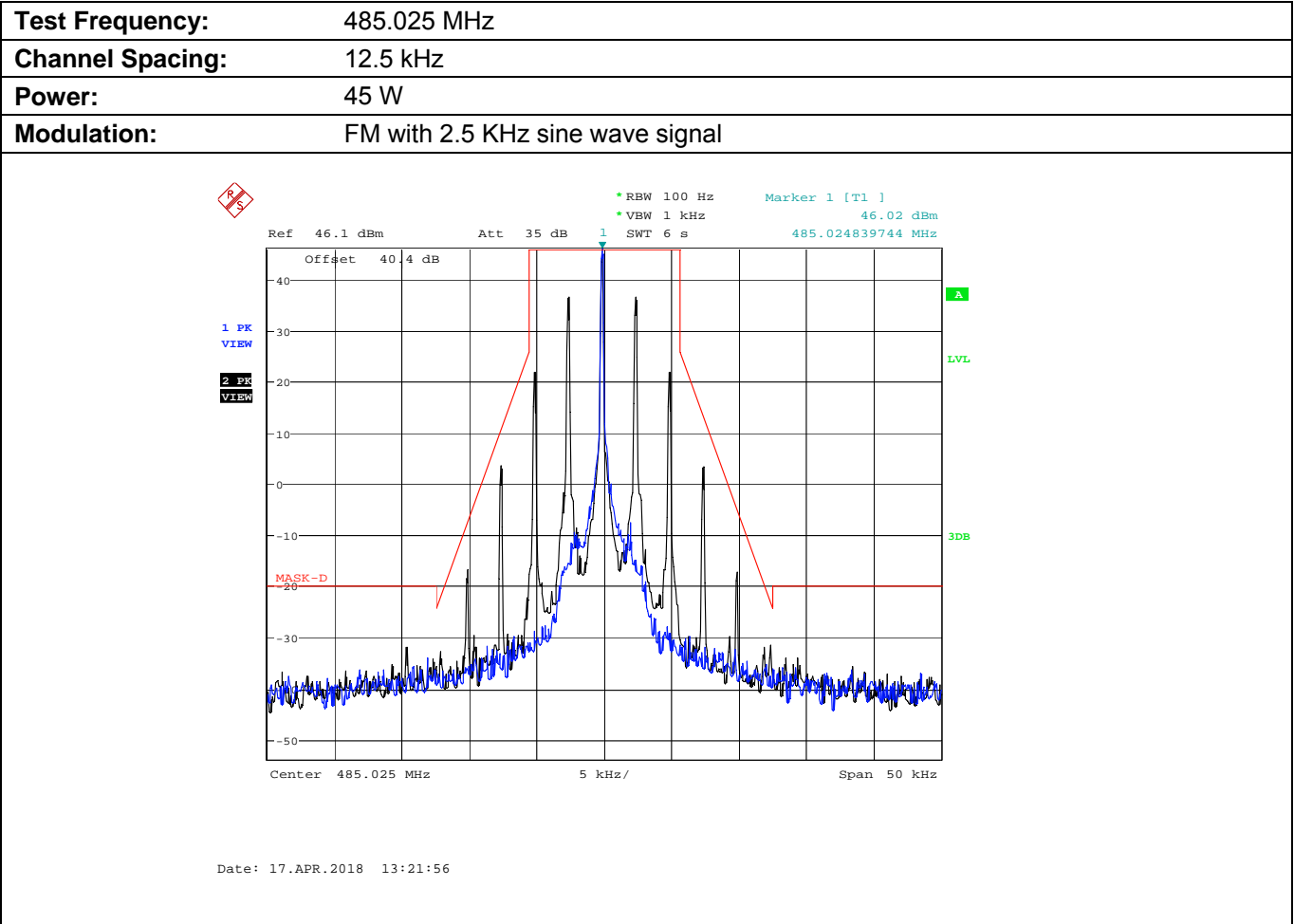
Plot 5.8.4.2.3. Emission Mask D, High Power
