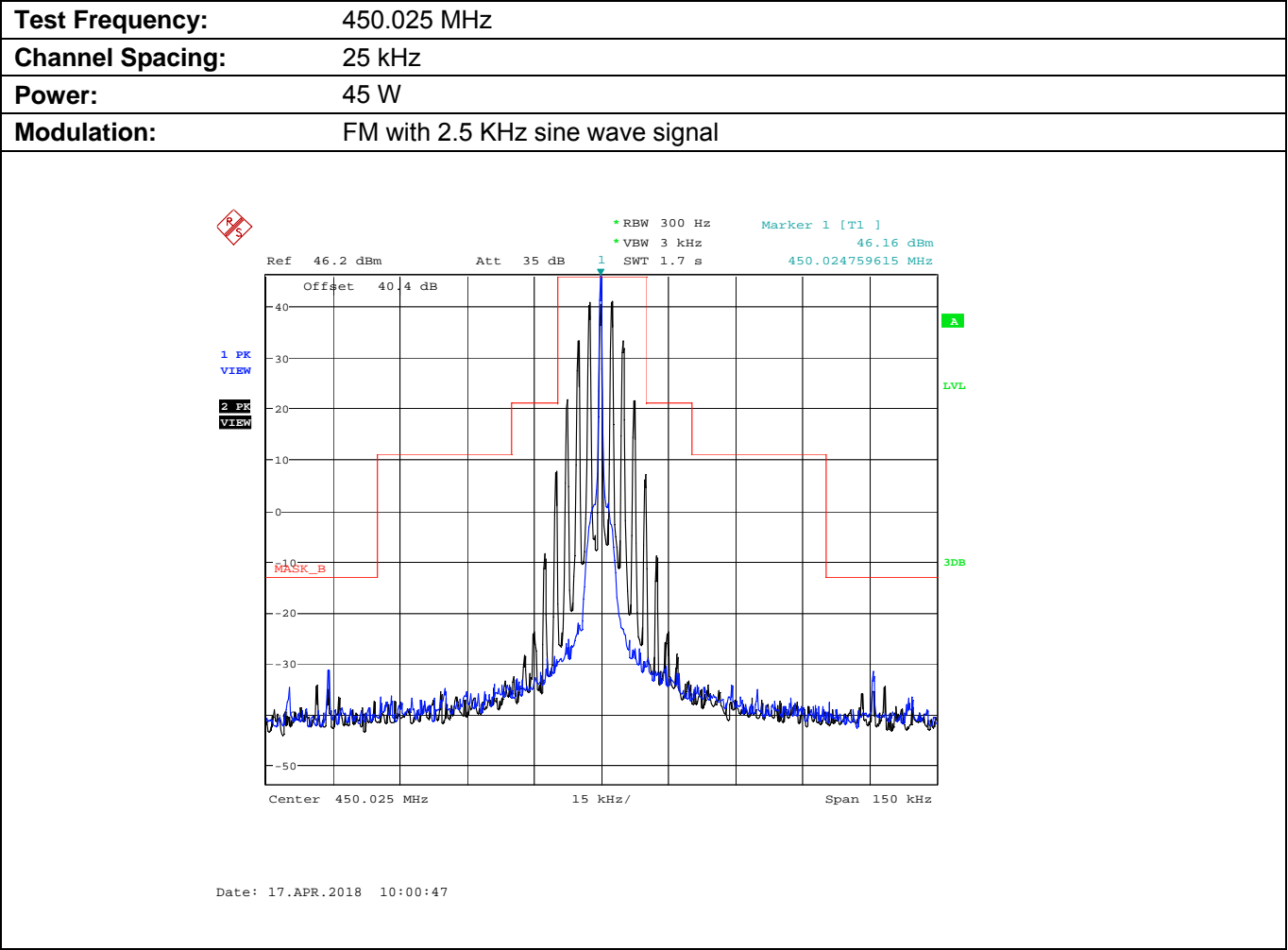
Plot 5.8.4.3.1. Emission Mask B, High Power
