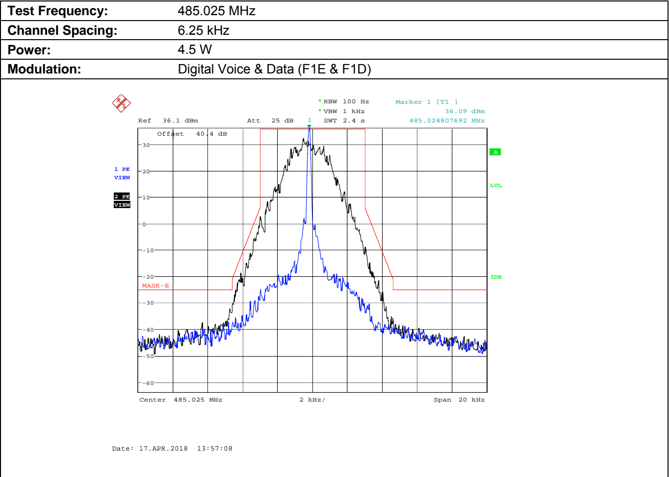
Plot 5.8.4.4.4. Emission Mask E, Low Power
