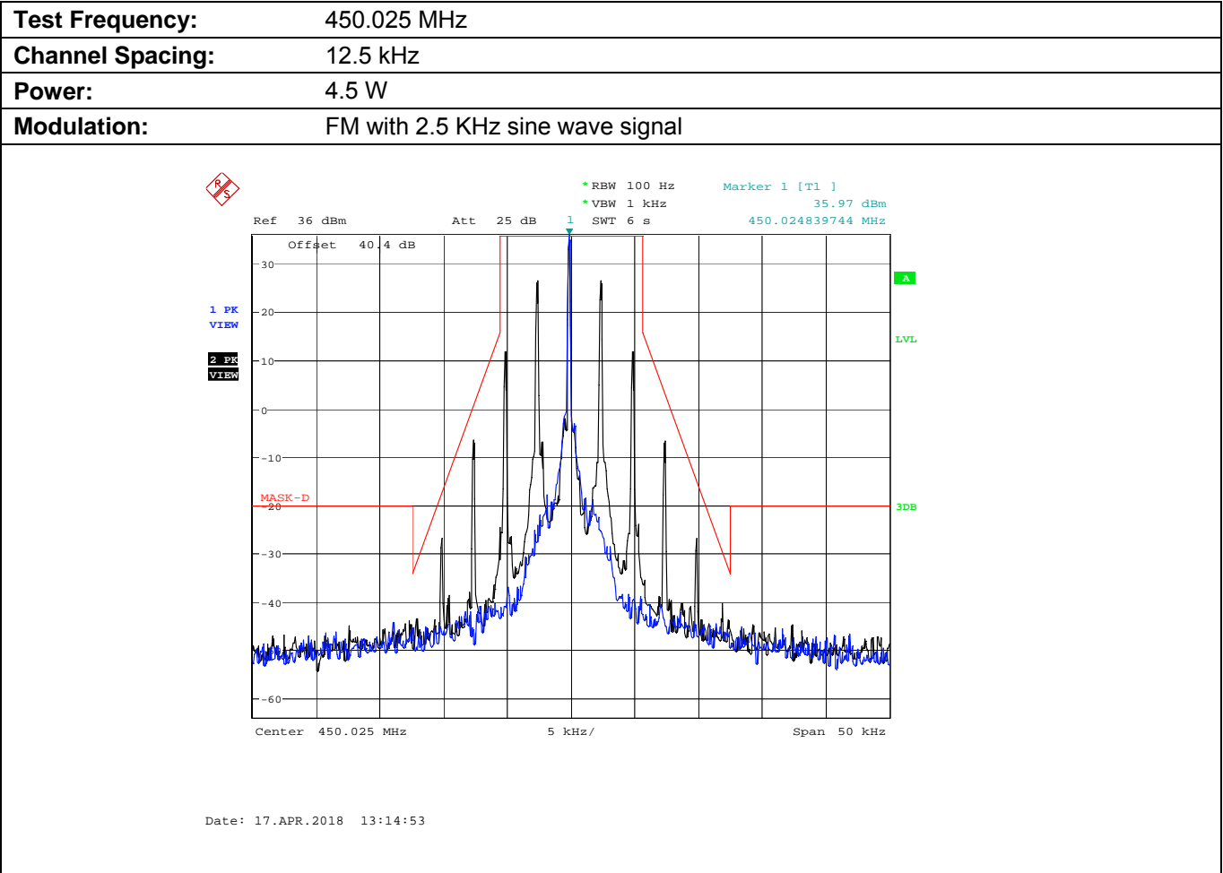
Plot 5.8.4.2.2. Emission Mask D, Low Power
