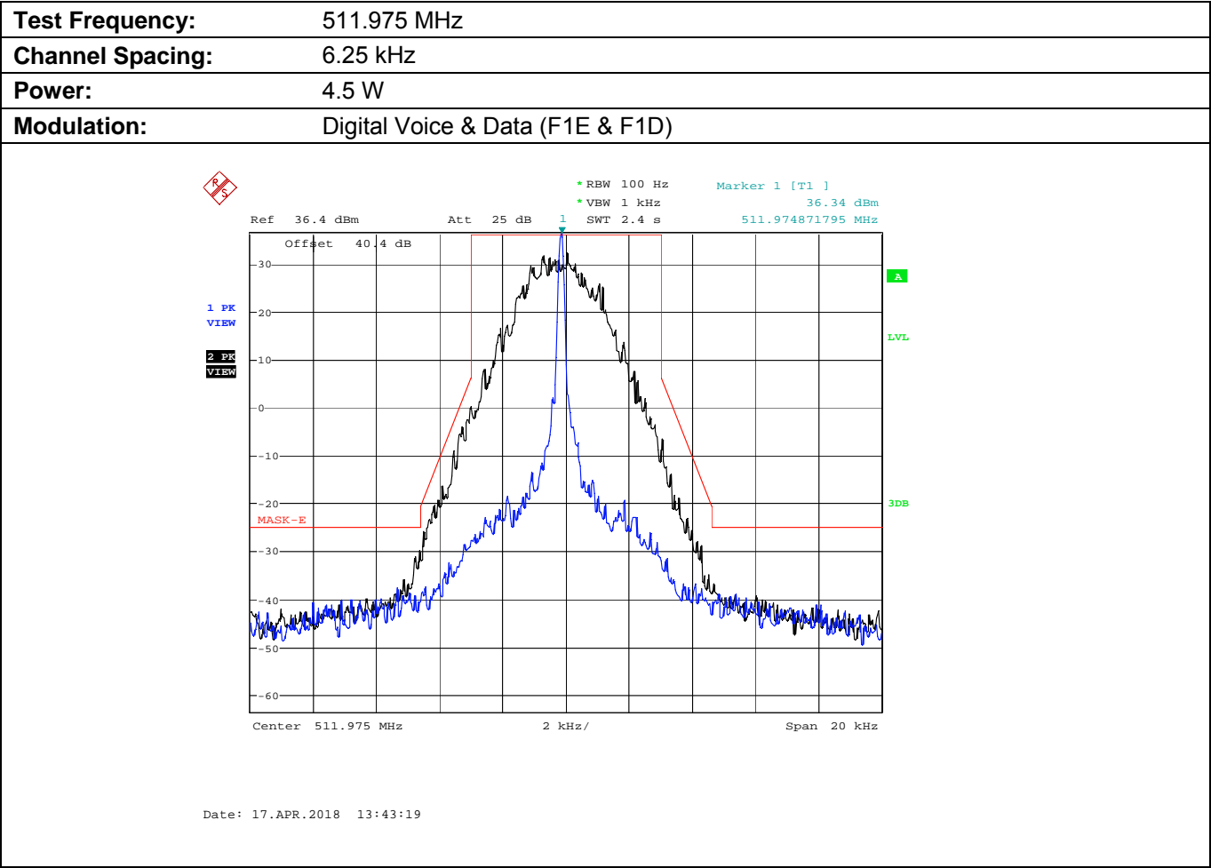
Plot 5.8.4.4.6. Emission Mask E, Low Power
