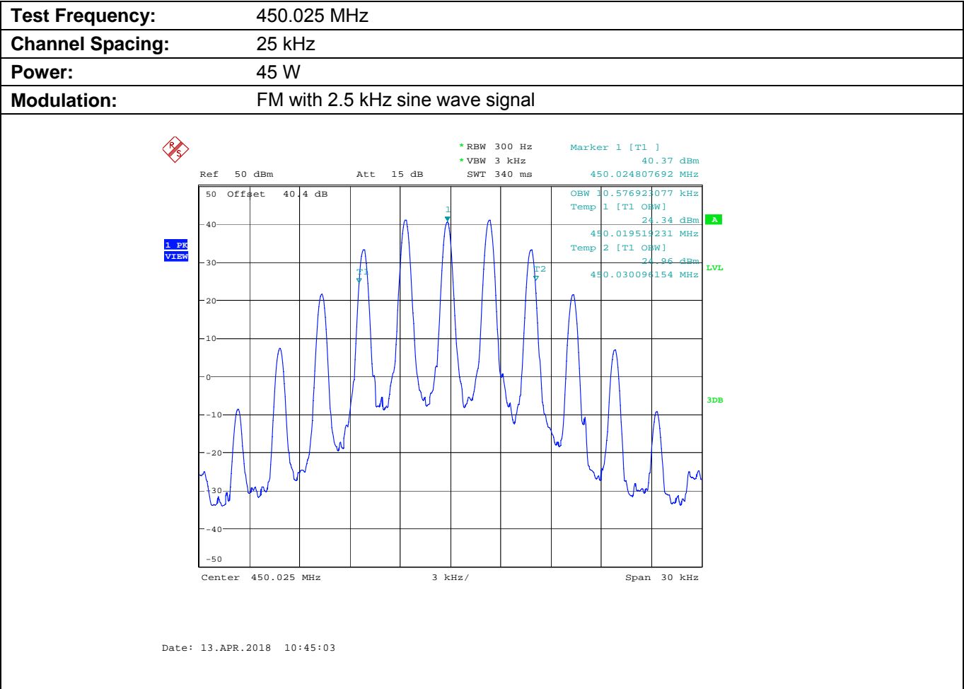
Plot 5.8.4.1.1. Occupied Bandwidth
