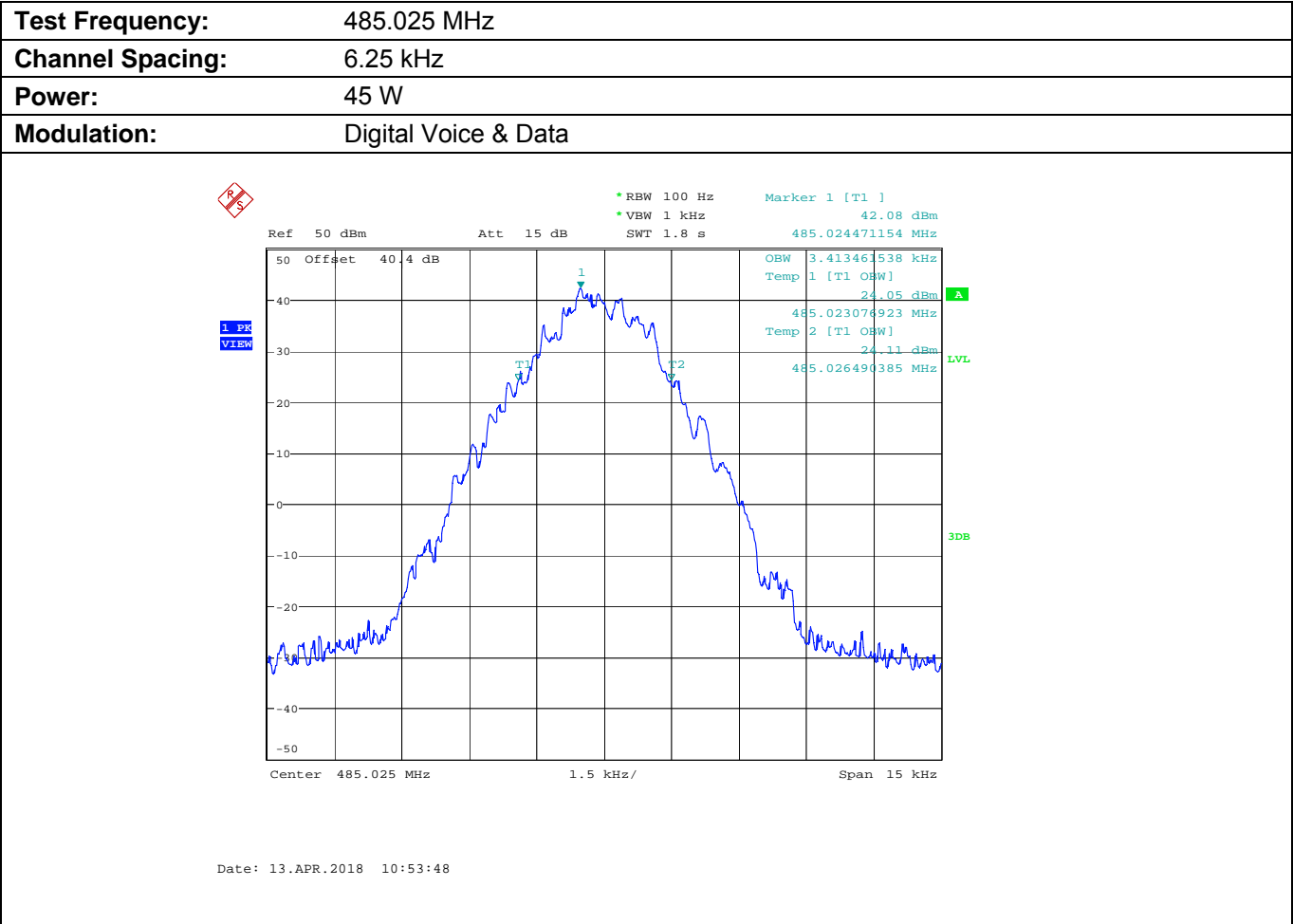
Plot 5.8.4.1.8. Occupied Bandwidth
