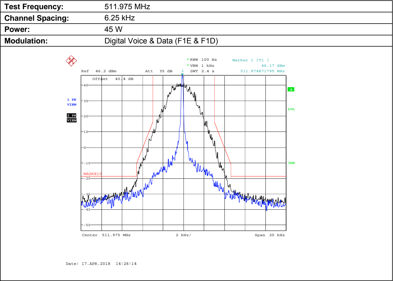
Plot 5.8.4.4.5. Emission Mask E, High Power
