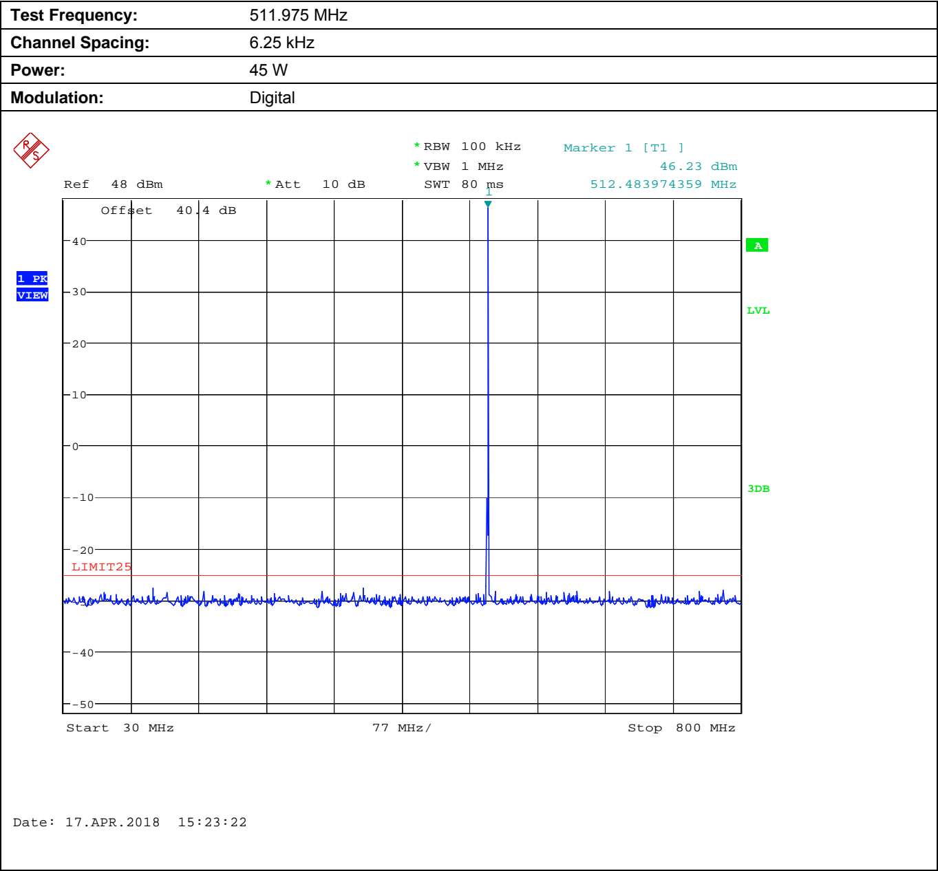
Plot 5.9.4.3.1. Conducted Transmitter Spurious Emissions for 511.975 MHz, High Power, 30 - 800 MHz
