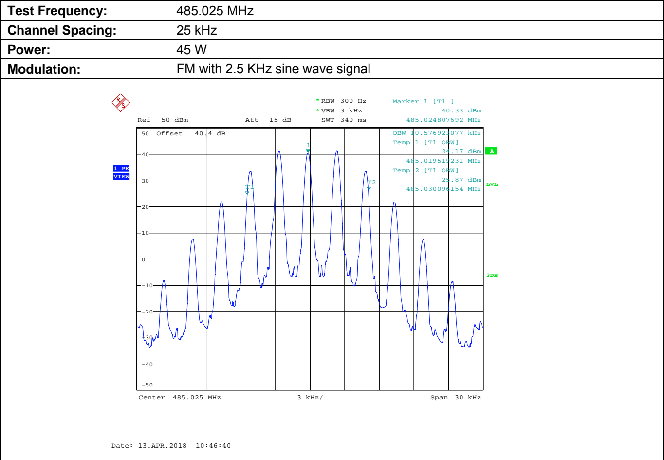
Plot 5.8.4.1.2. Occupied Bandwidth
