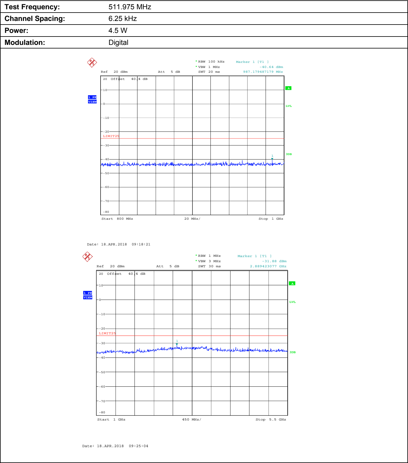
Plot 5.9.4.3.4. Conducted Transmitter Spurious Emissions for 511.975 MHz, Low Power, 0.8 - 5.5 GHz
