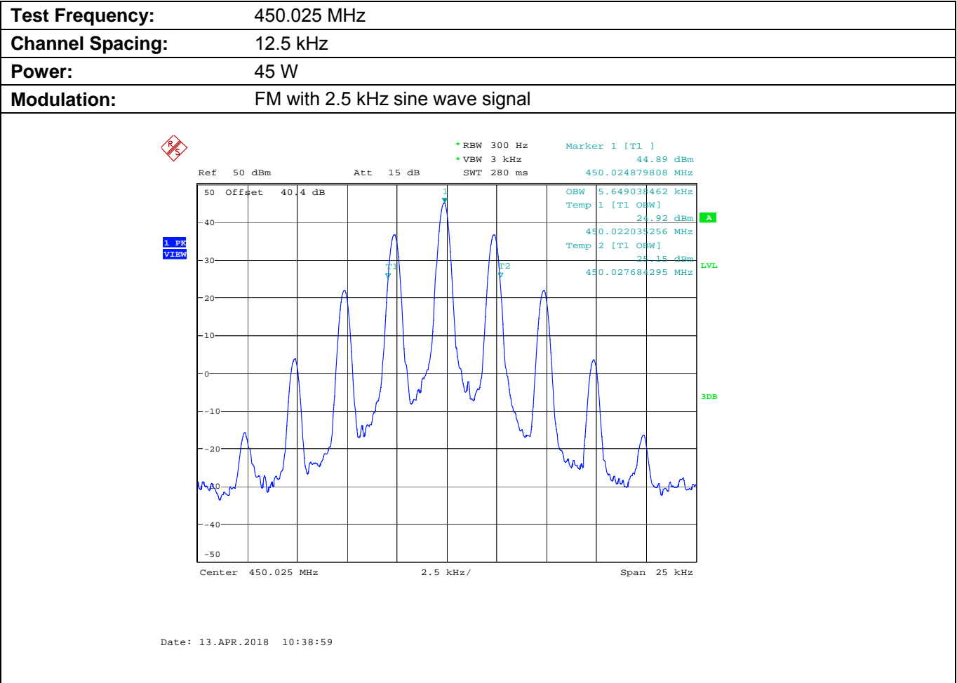
Plot 5.8.4.1.4. Occupied Bandwidth
