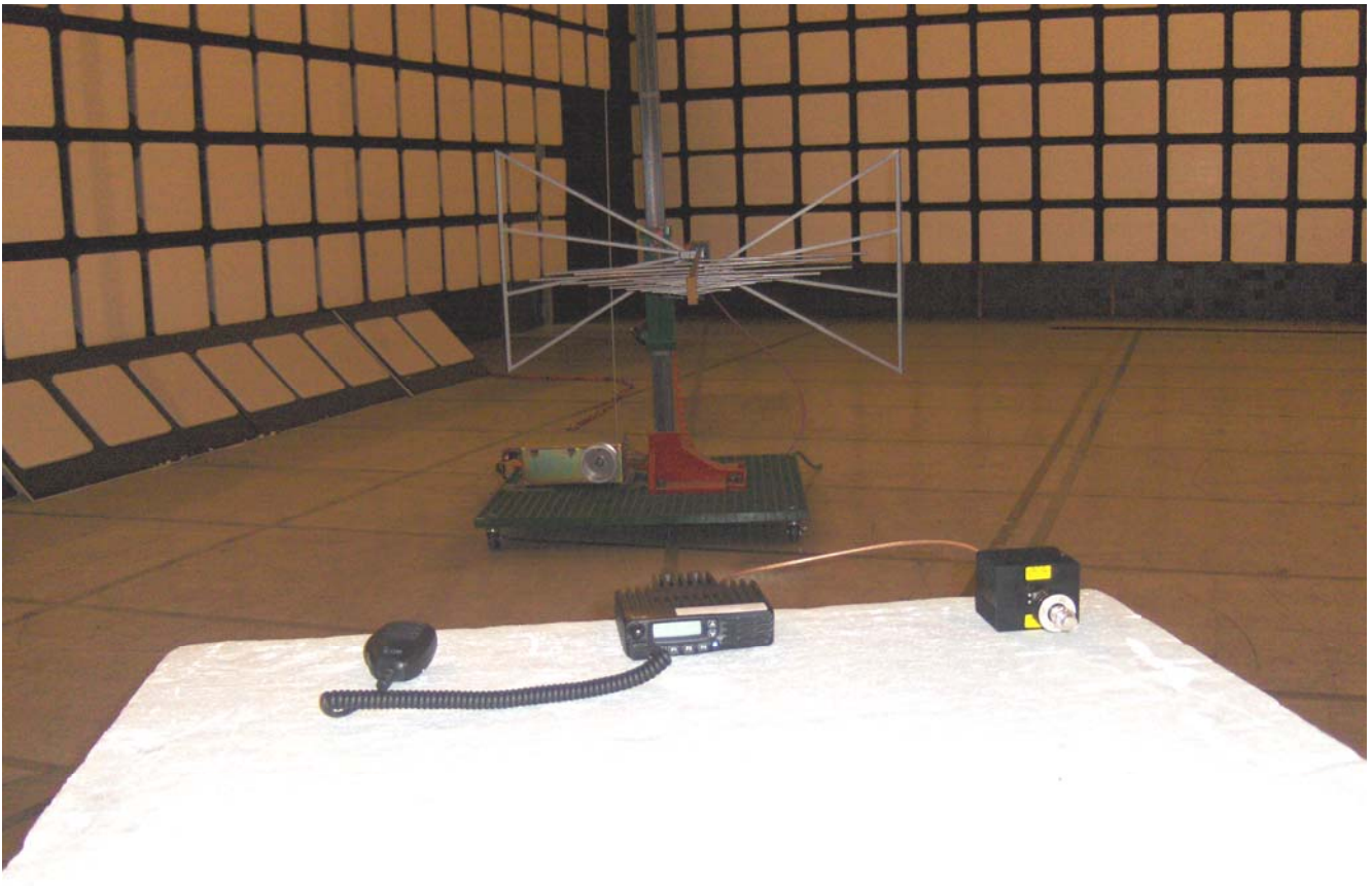
Radiated Transmitter Emission Test at 3m, 30 MHz to 1GHz
