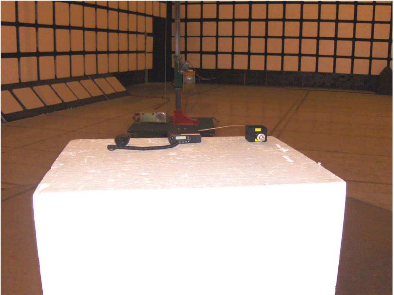
Radiated Transmitter Emission Test at 3m, Above 1GHz
