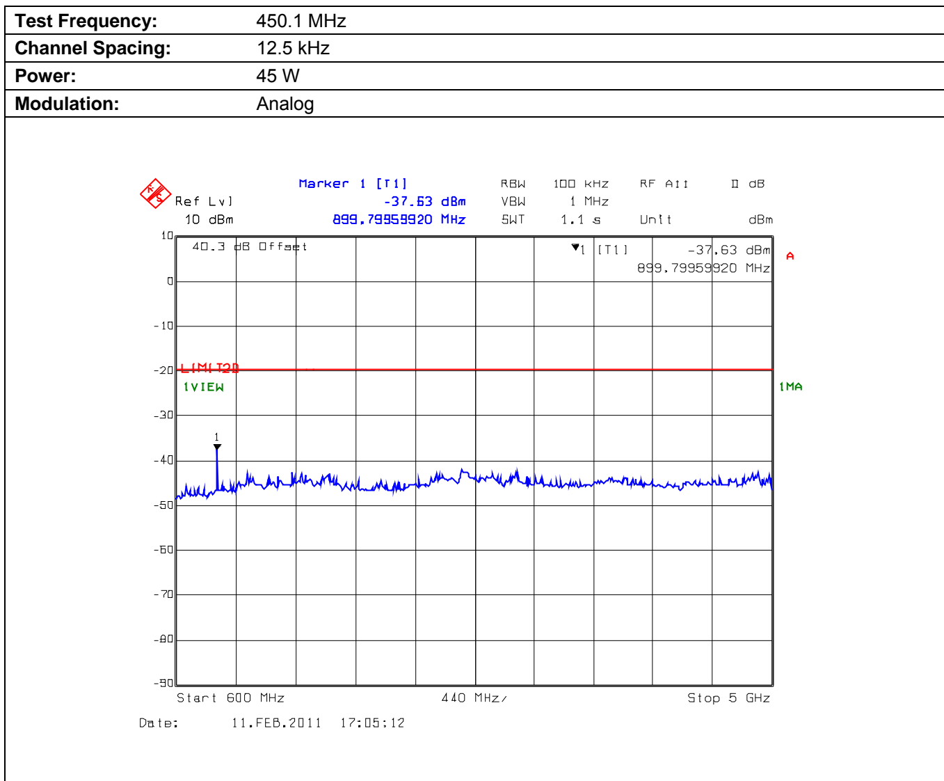
Plot 5.10.4.3.2. Conducted Transmitter Spurious Emissions for 450.1 MHz, High Power, 600 MHz - 5 GHz
