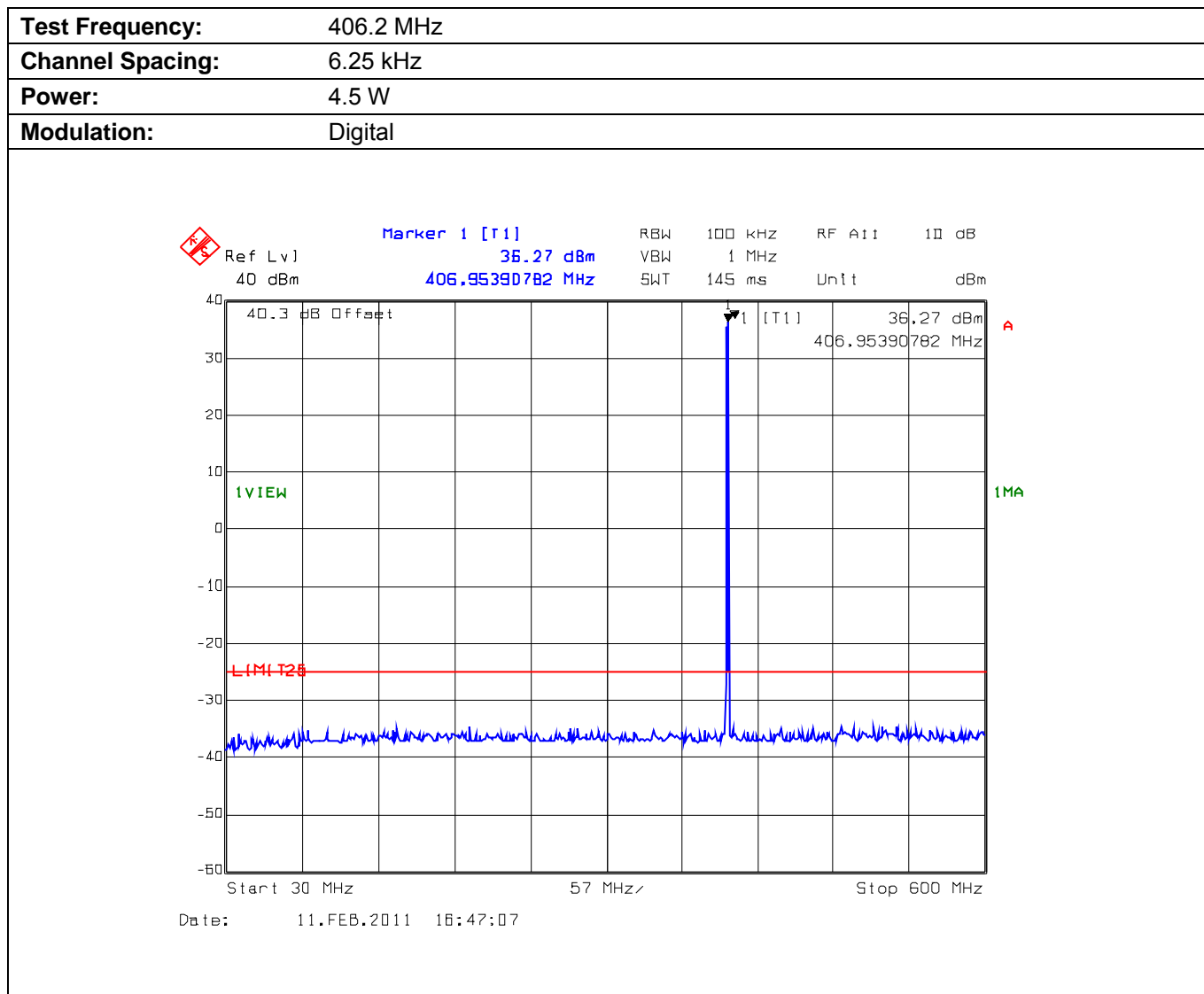
Plot 5.10.4.2.3. Conducted Transmitter Spurious Emissions for 406.2 MHz, Low Power, 30 MHz - 600 MHz
