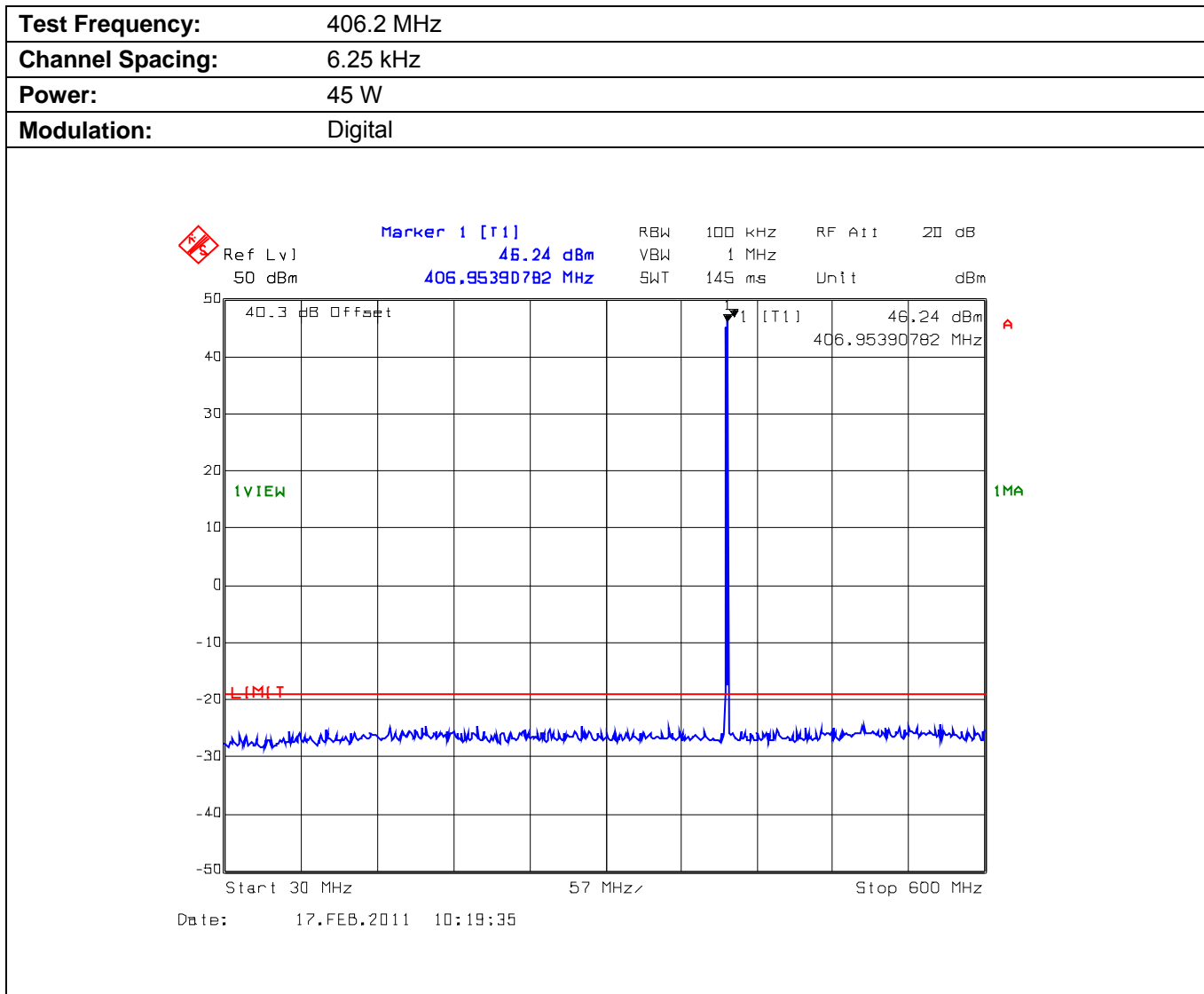
Plot 5.10.4.2.1. Conducted Transmitter Spurious Emissions for 406.2 MHz, High Power, 30 MHz - 600 MHz
