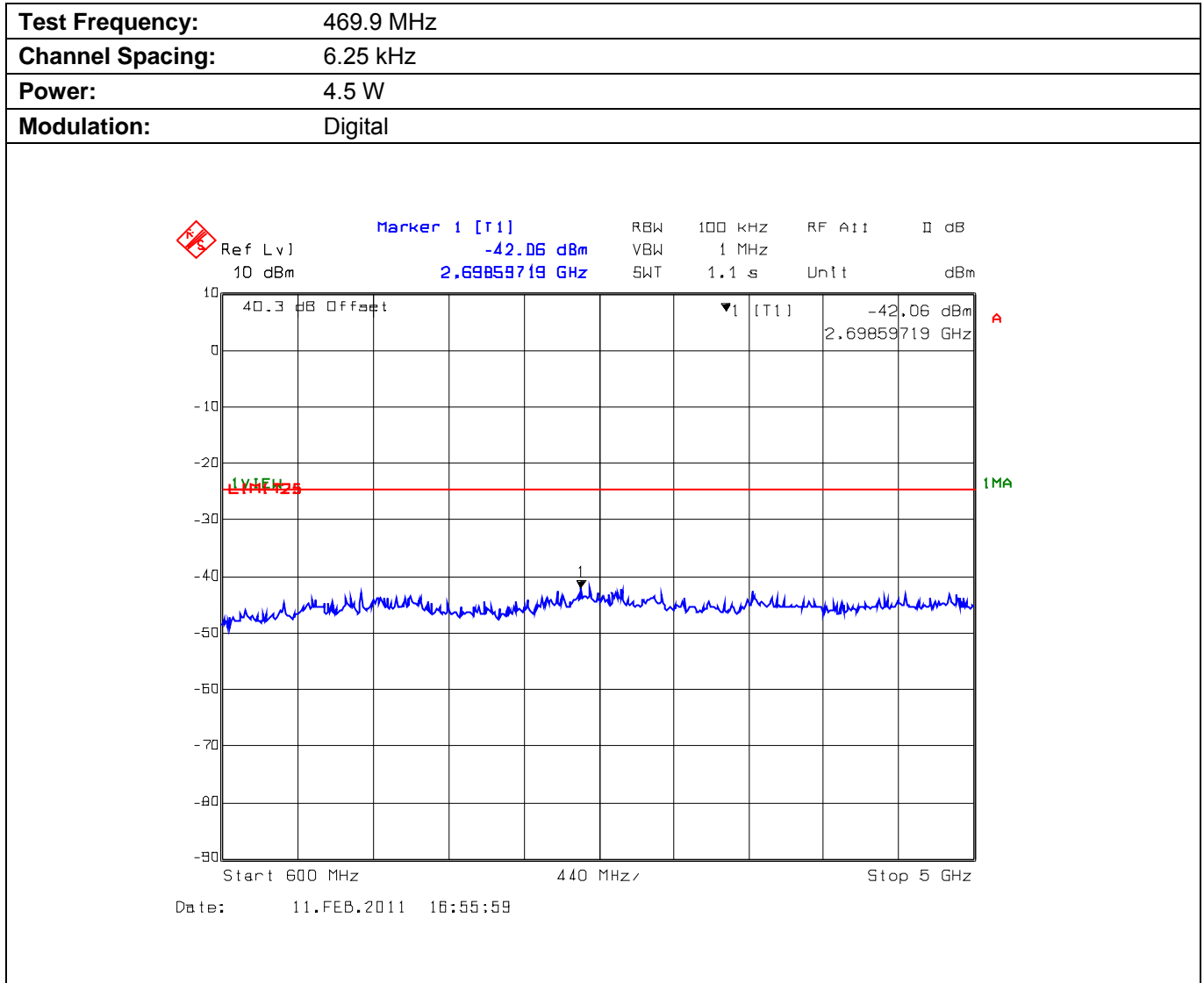
Plot 5.10.4.6.4. Conducted Transmitter Spurious Emissions for 469.9 MHz, Low Power, 600 MHz - 5 GHz
