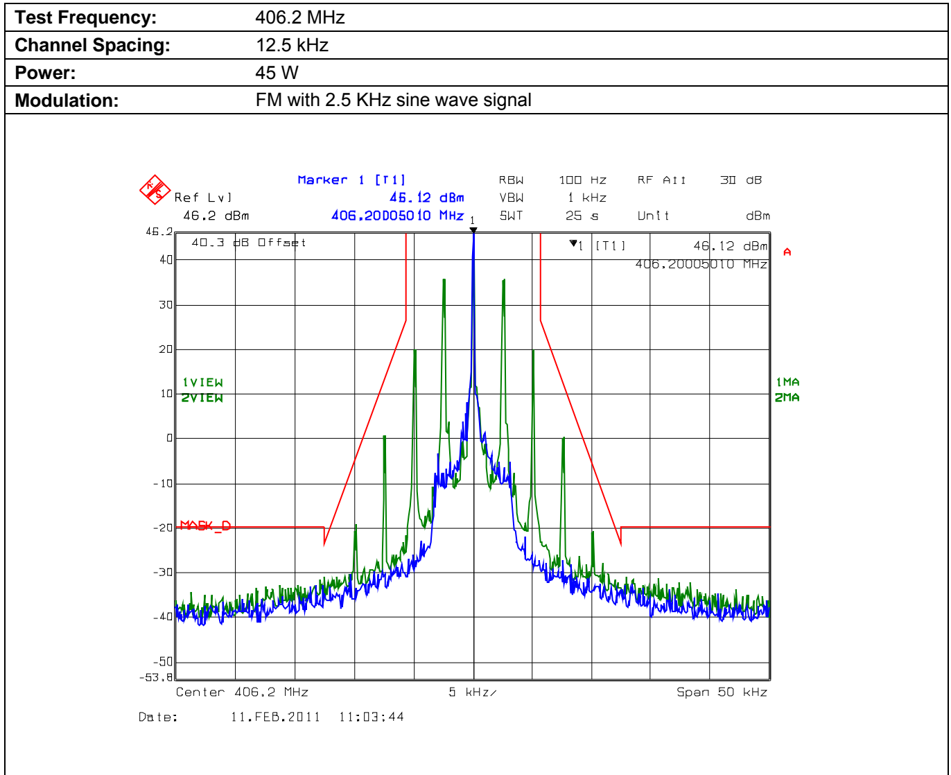
Plot 5.9.4.2.1. Emission Mask D, High Power
