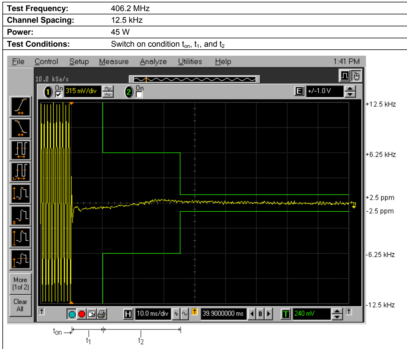
Plot 5.13.4.1. Transient Frequency Behavior for 12.5 kHz Channel Spacing
