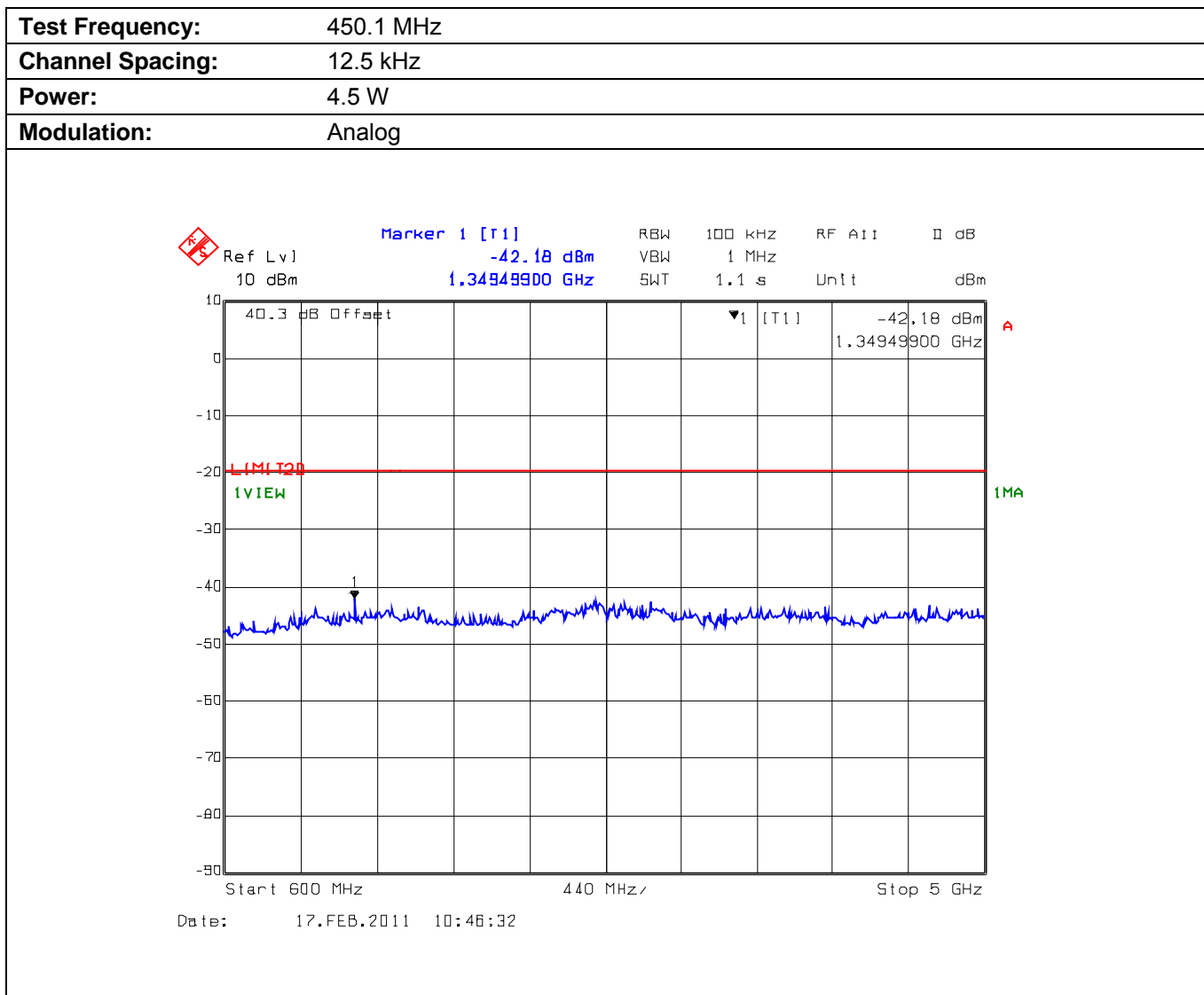
Plot 5.10.4.3.4. Conducted Transmitter Spurious Emissions for 450.1 MHz, Low Power, 600 MHz - 5 GHz
