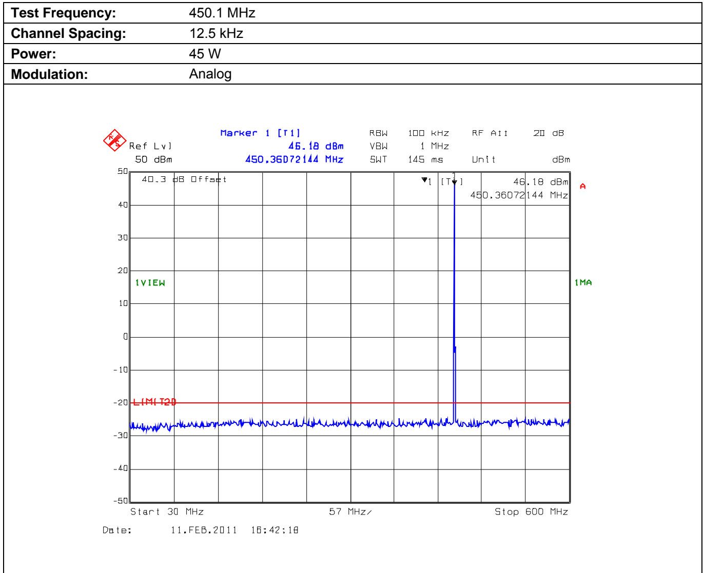
Plot 5.10.4.3.1. Conducted Transmitter Spurious Emissions for 450.1 MHz, High Power, 30 MHz - 600 MHz
