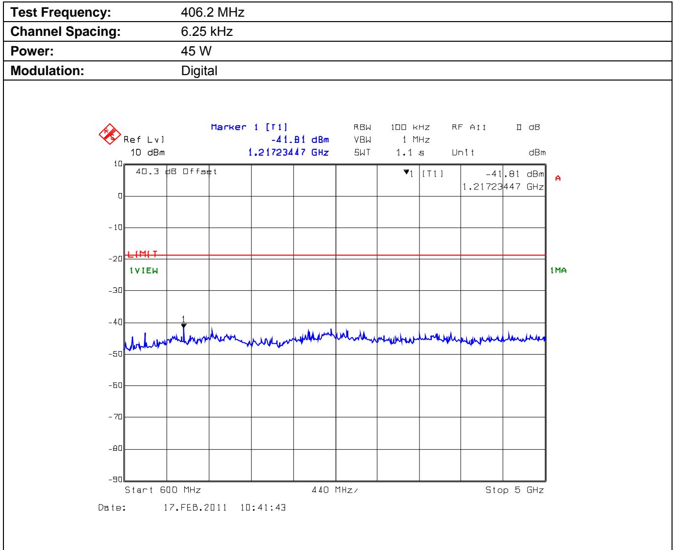
Plot 5.10.4.2.2. Conducted Transmitter Spurious Emissions for 406.2 MHz, High Power, 600 MHz - 5 GHz
