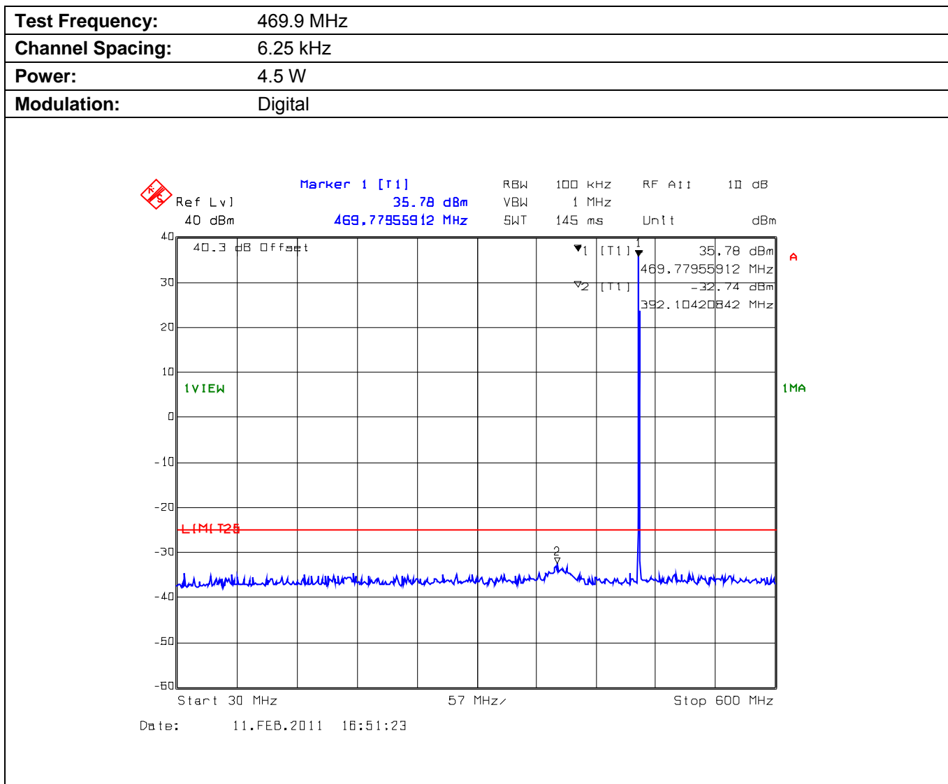
Plot 5.10.4.6.3. Conducted Transmitter Spurious Emissions for 469.9 MHz, Low Power, 30 MHz - 600 MHz
