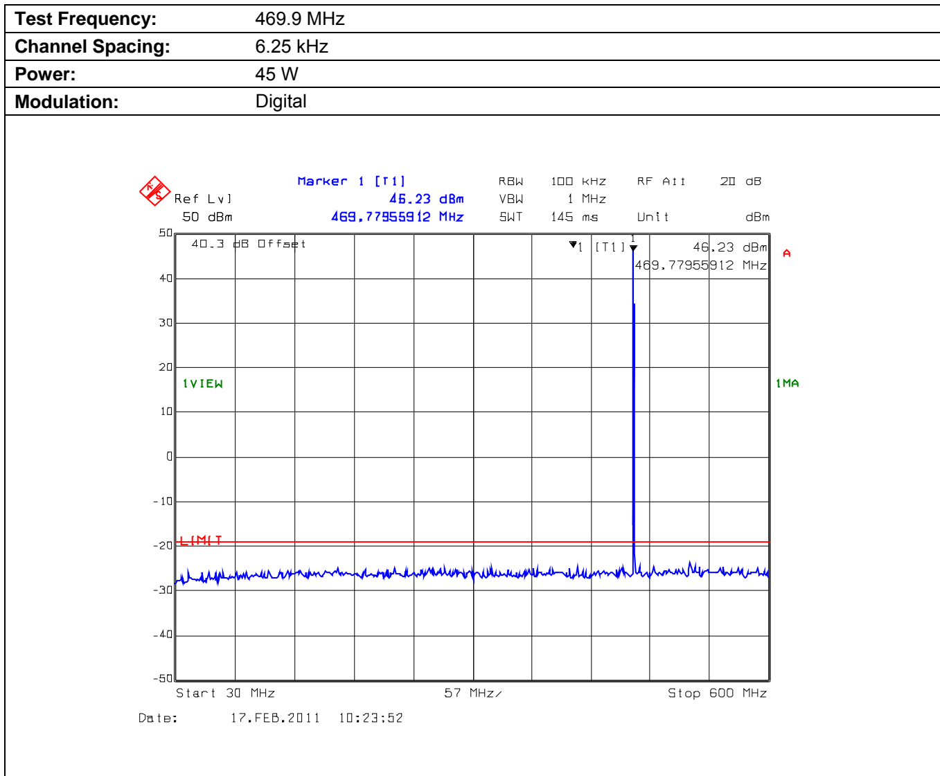
Plot 5.10.4.6.1. Conducted Transmitter Spurious Emissions for 469.9 MHz, High Power, 30 MHz - 600 MHz
