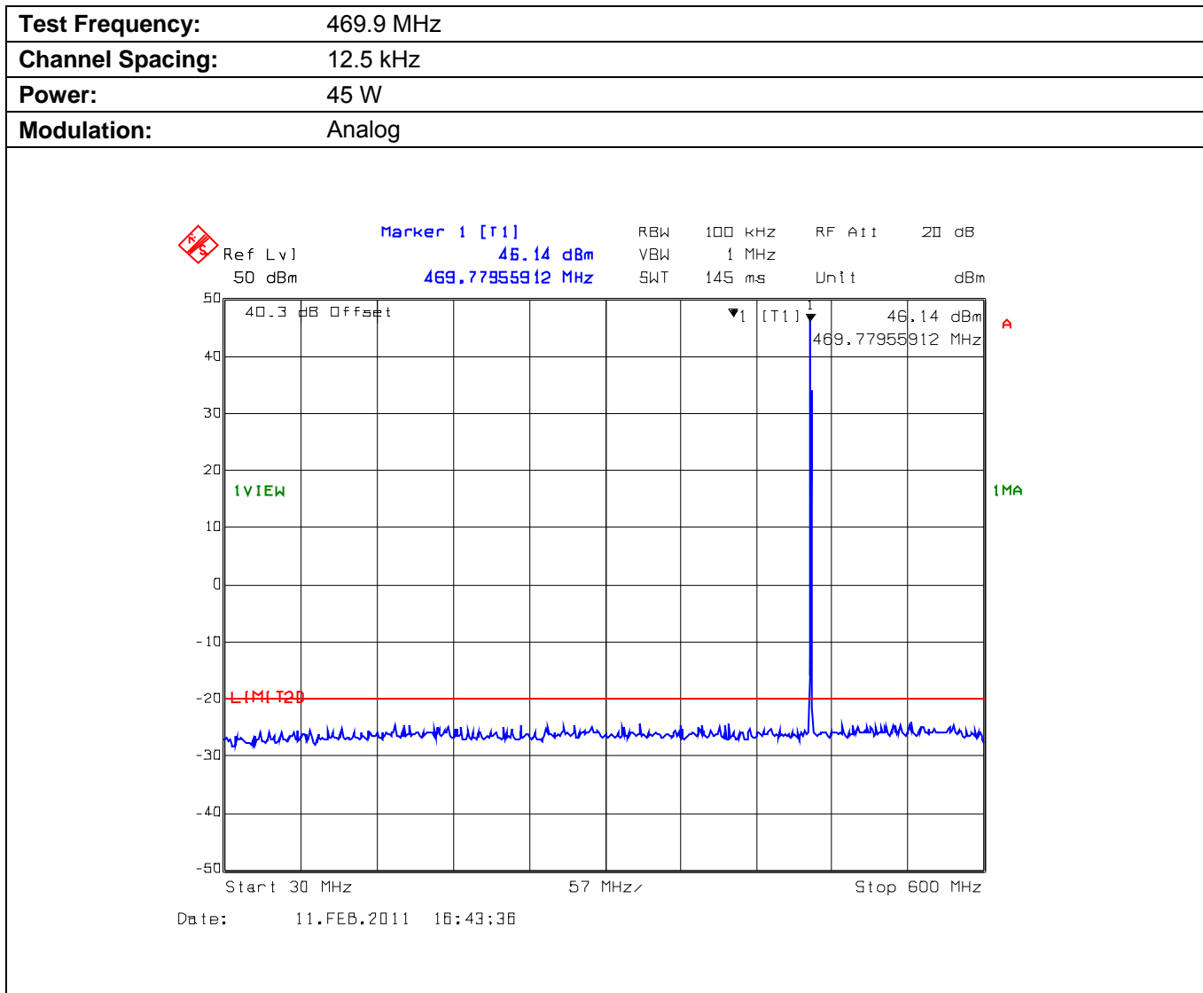
Plot 5.10.4.5.1. Conducted Transmitter Spurious Emissions for 469.9 MHz, High Power, 30 MHz - 600 MHz
