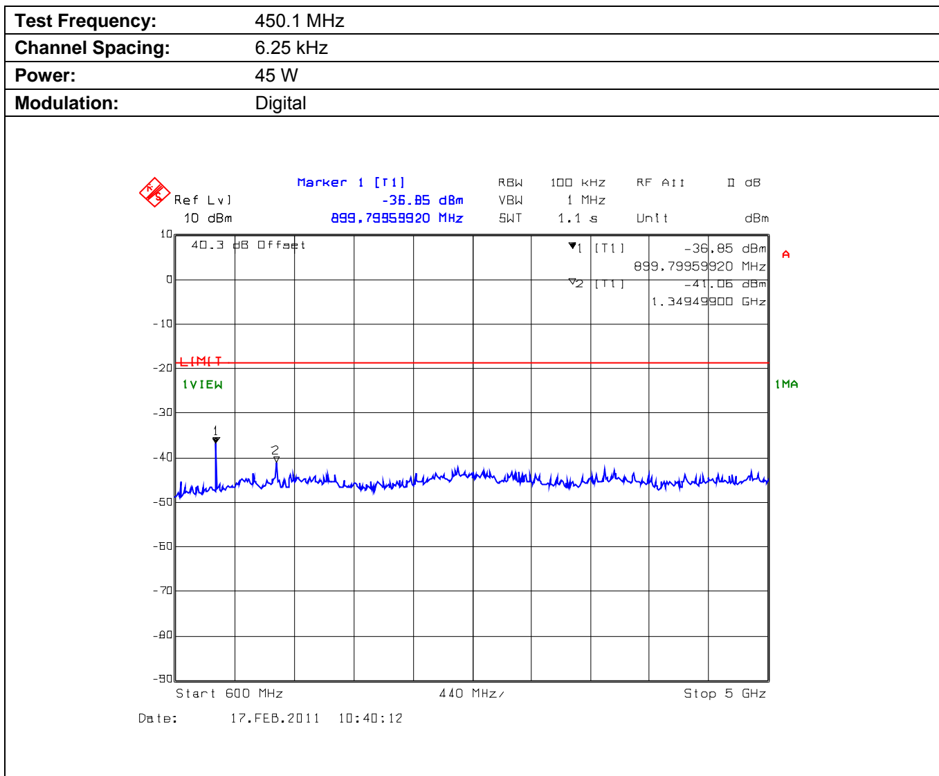
Plot 5.10.4.4.2. Conducted Transmitter Spurious Emissions for 450.1 MHz, High Power, 600 MHz - 5 GHz
