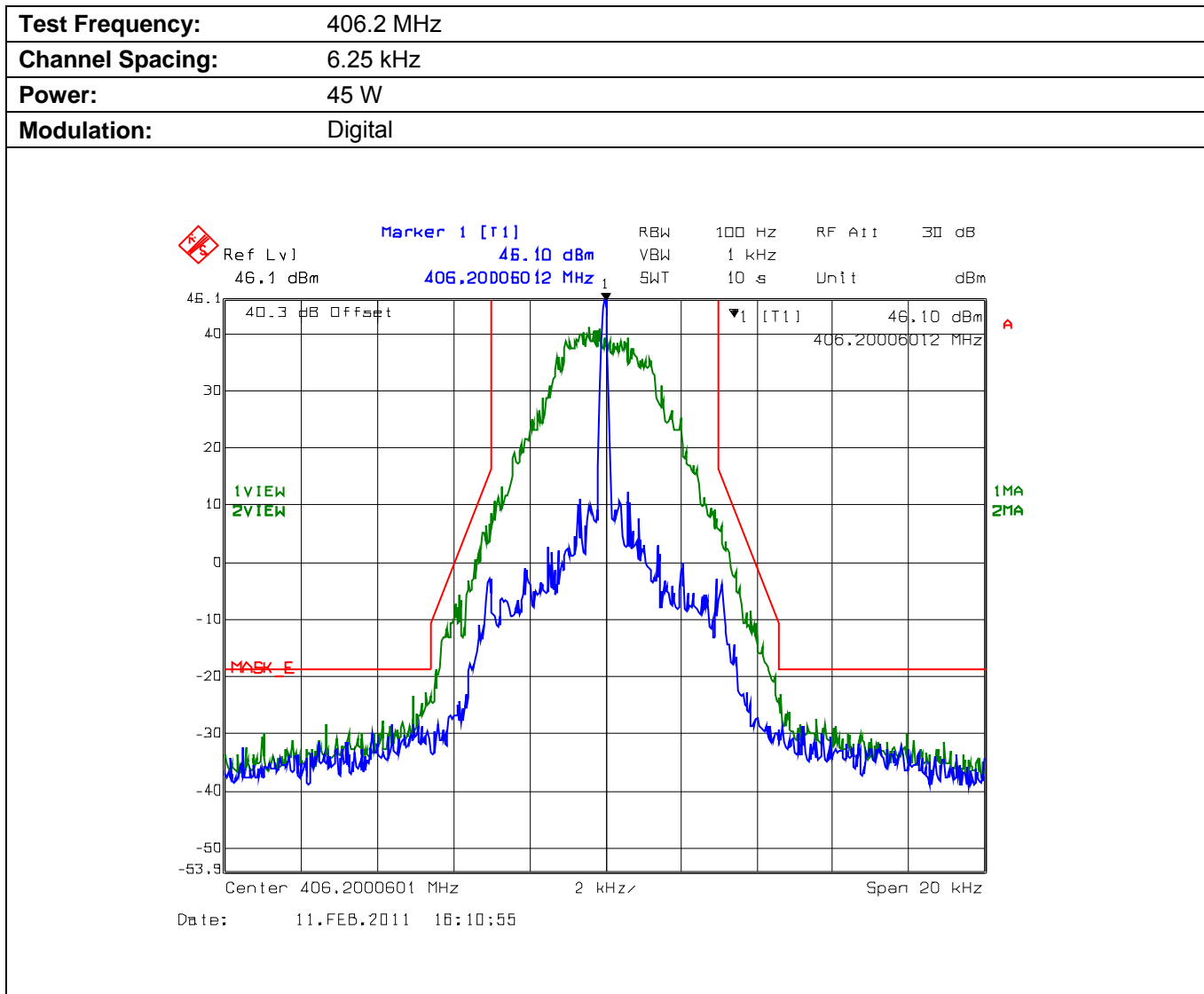
Plot 5.9.4.3.1. Emission Mask E, High Power
