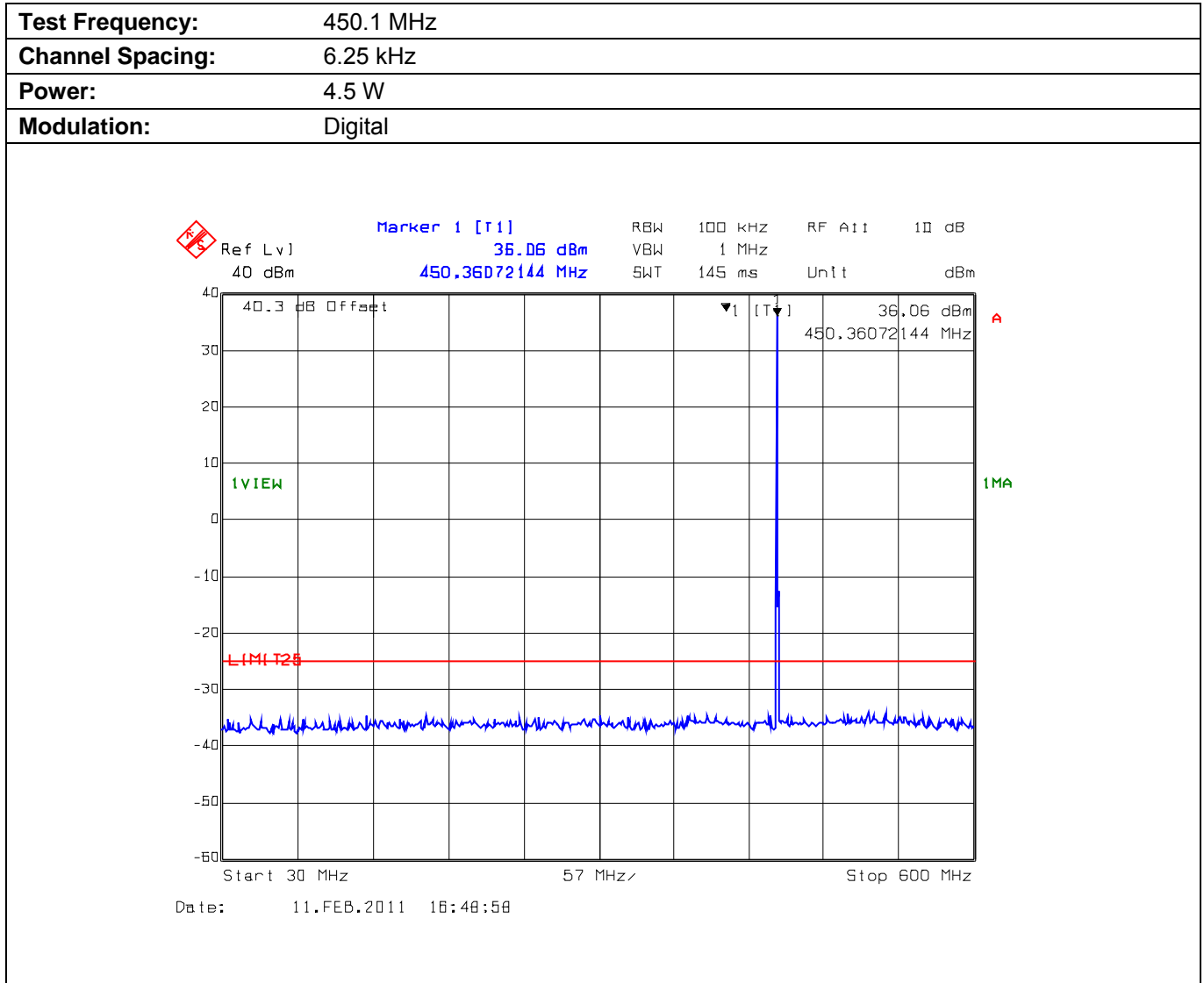
Plot 5.10.4.4.3. Conducted Transmitter Spurious Emissions for 450.1 MHz, Low Power, 30 MHz - 600 MHz
