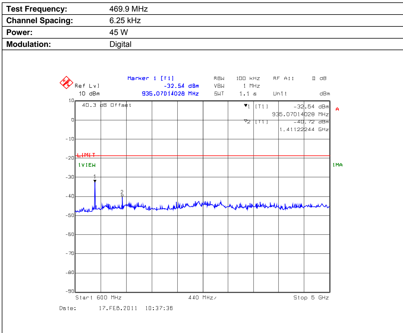
Plot 5.10.4.6.2. Conducted Transmitter Spurious Emissions for 469.9 MHz, High Power, 600 MHz - 5 GHz
