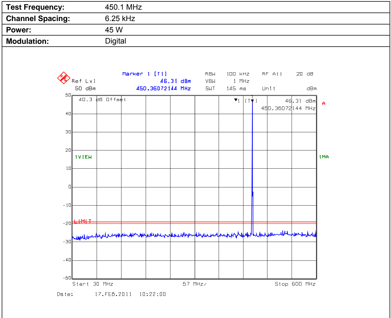
Plot 5.10.4.4.1. Conducted Transmitter Spurious Emissions for 450.1 MHz, High Power, 30 MHz - 600 MHz
