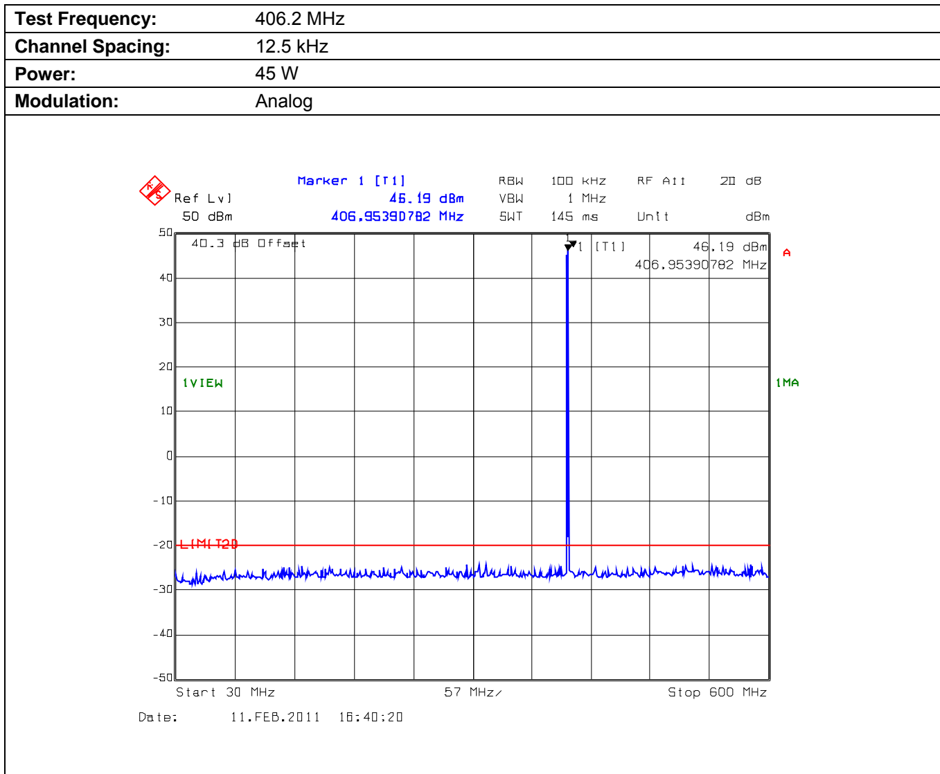
Plot 5.10.4.1.1. Conducted Transmitter Spurious Emissions for 406.2 MHz, High Power, 30 MHz - 600 MHz
