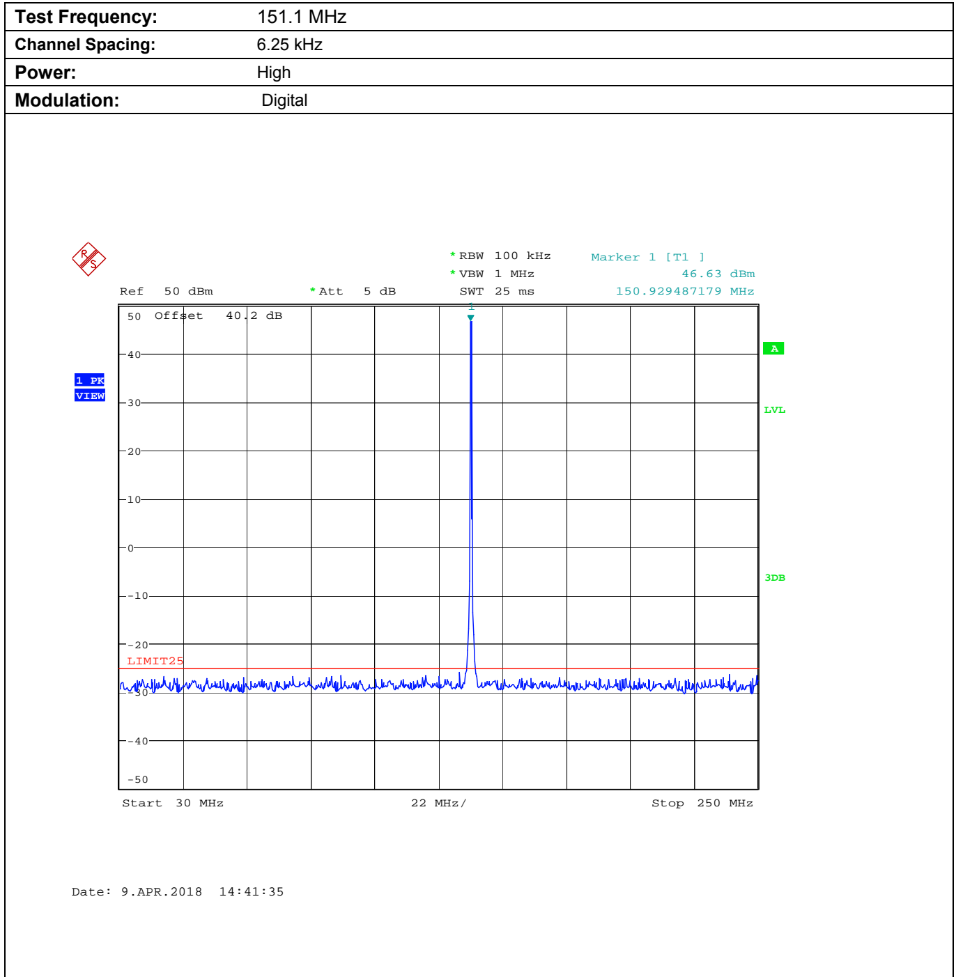
Plot 5.9.4.2.1. Conducted Transmitter Spurious Emissions for 151.1 MHz, High Power
