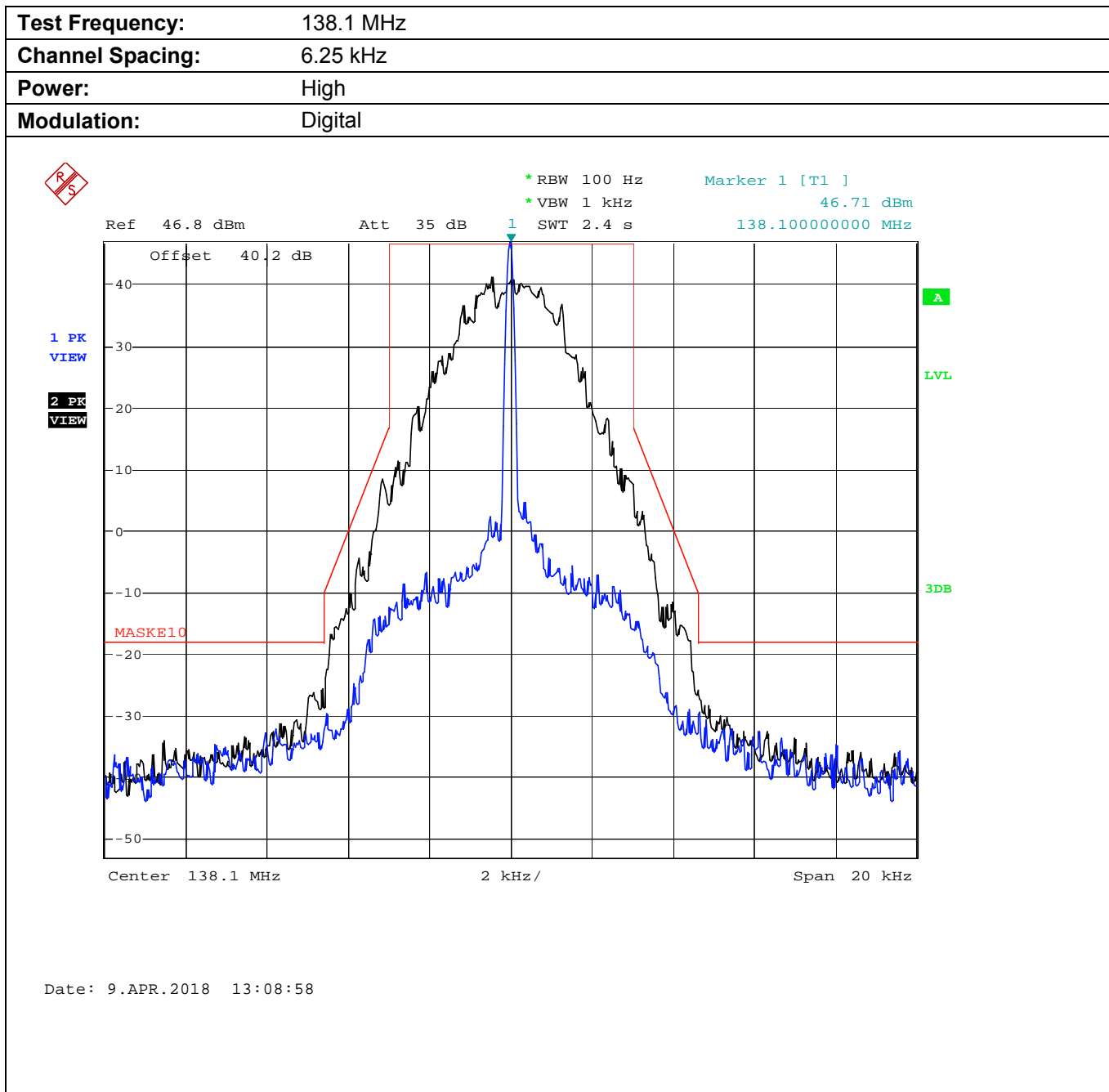
Plot 5.8.4.1.1. Emission Mask E, High Power
