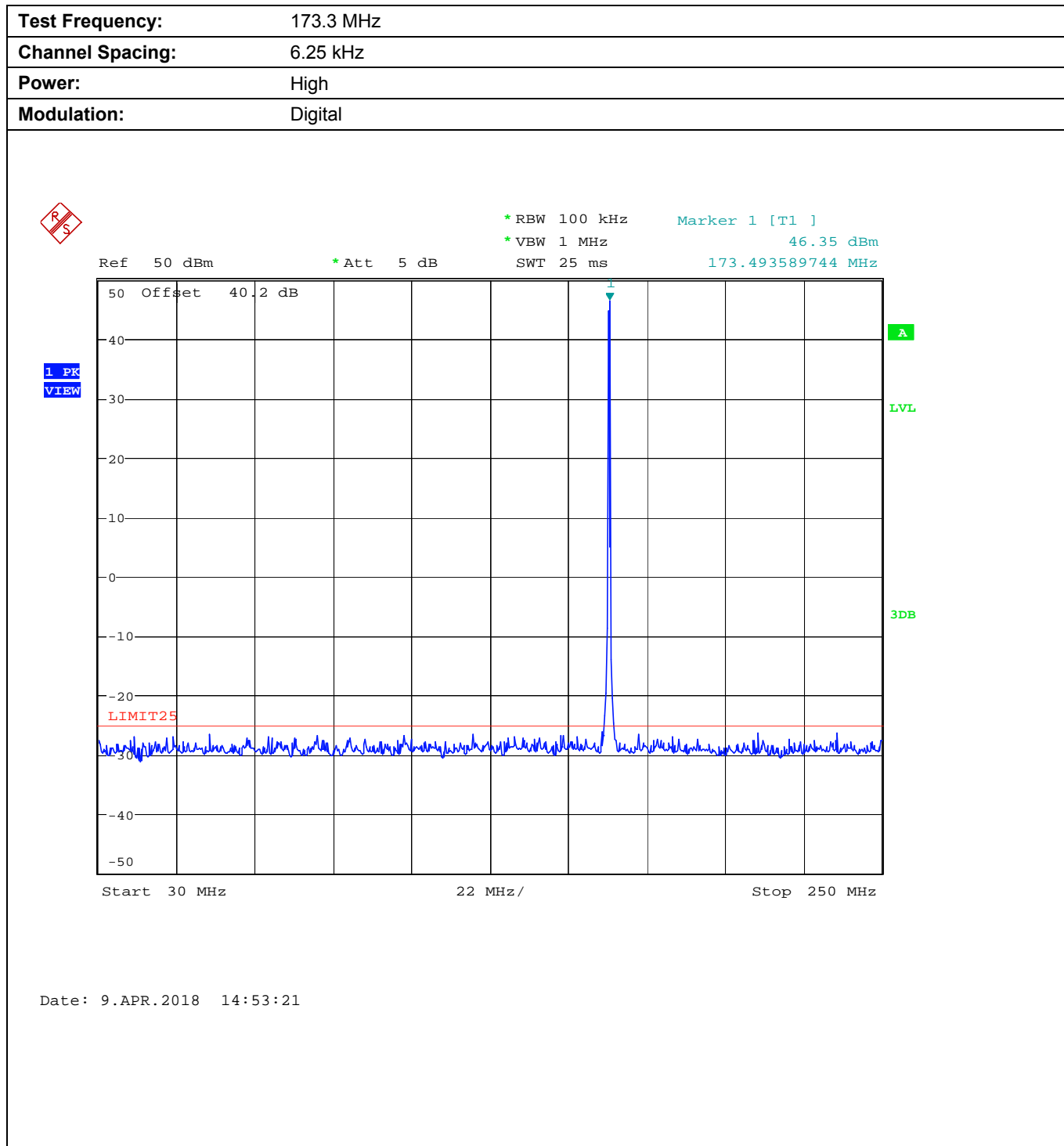
Plot 5.9.4.4.1. Conducted Transmitter Spurious Emissions for 173.3 MHz, High Power
