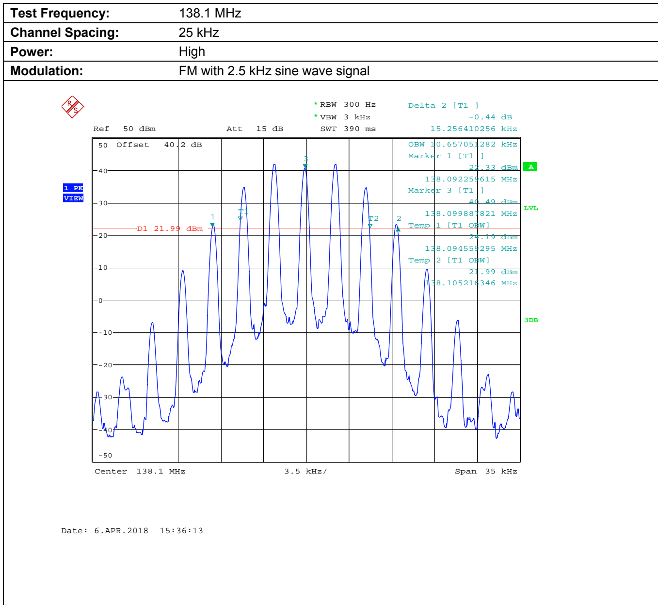
Plot 5.8.4.1.1. Occupied Bandwidth
