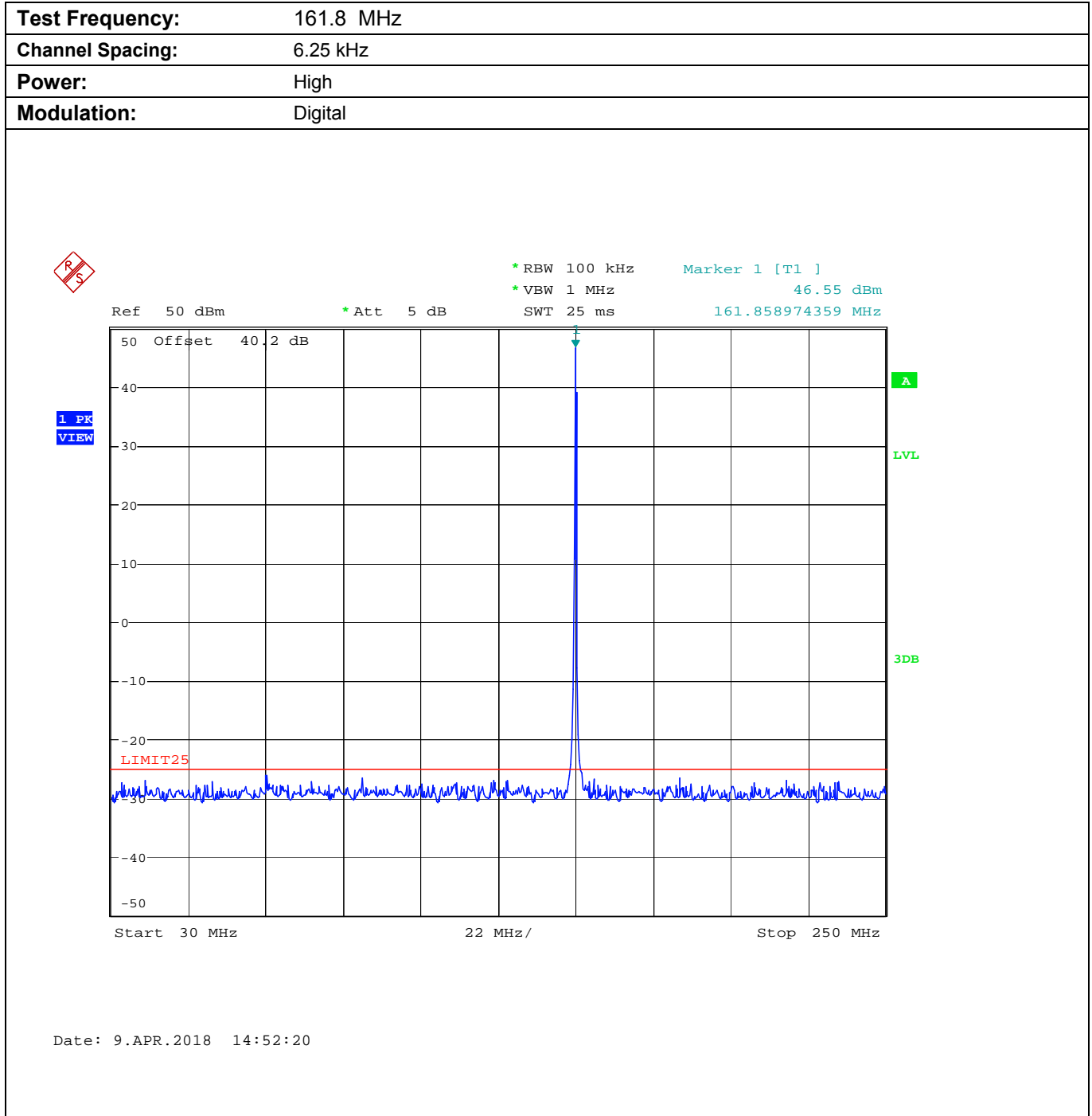
Plot 5.9.4.3.1. Conducted Transmitter Spurious Emissions for 161.8 MHz, High Power
