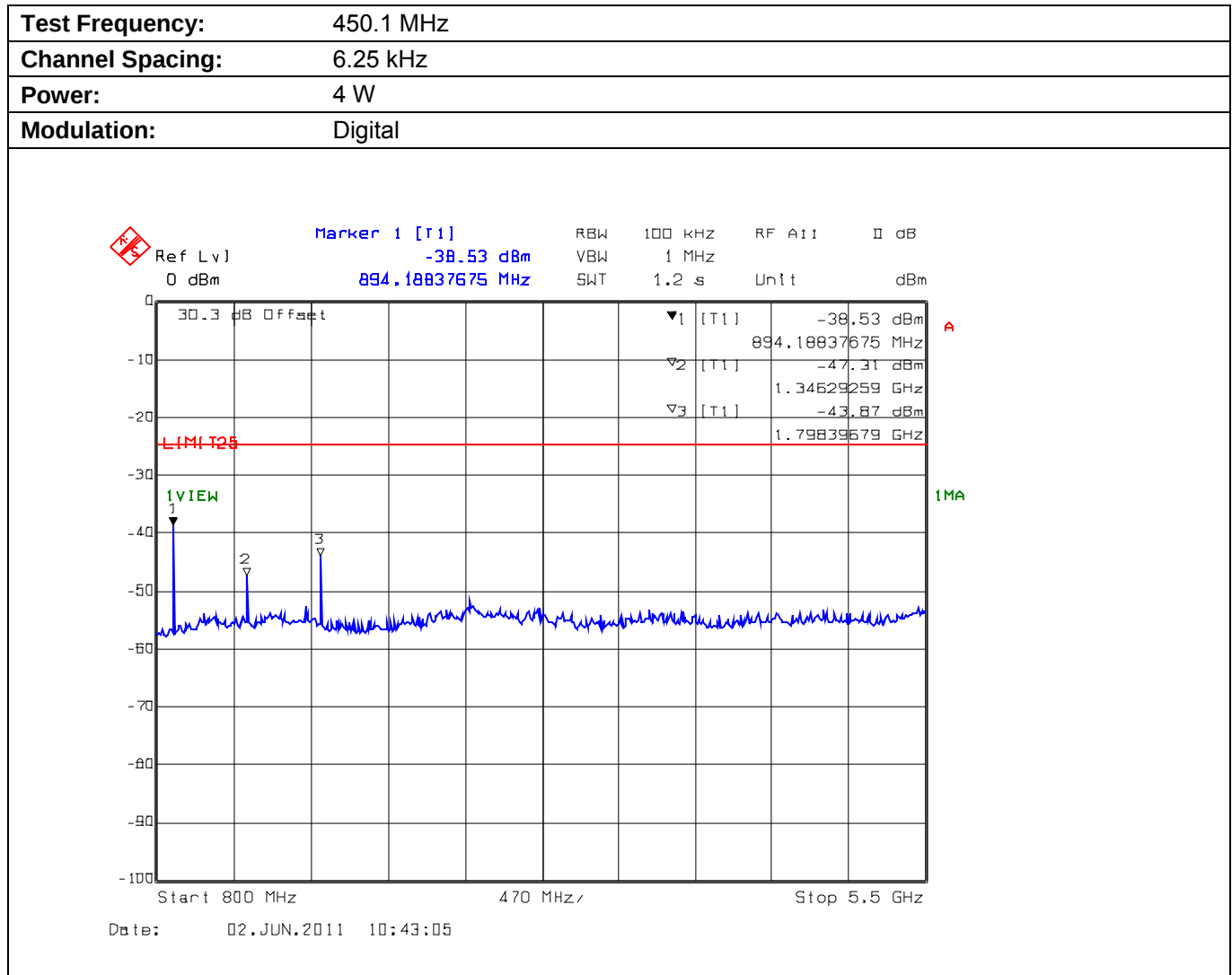
Plot 5.9.4.1.2. Conducted Transmitter Spurious Emissions for 450.1 MHz, High Power, 800 MHz - 5.5 GHz
