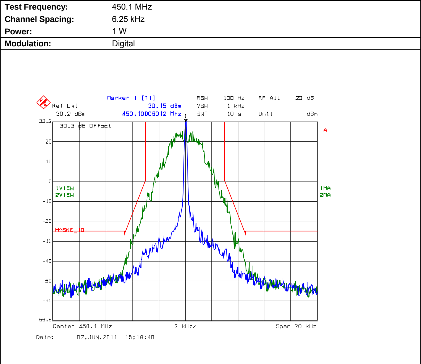
Plot 5.8.4.3.4. Emission Mask E, Low Power
