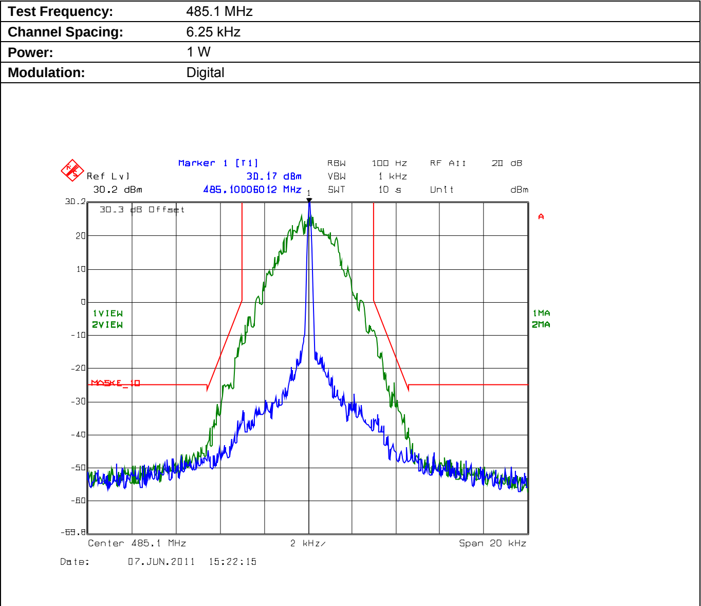
Plot 5.8.4.3.5. Emission Mask E, Low Power
