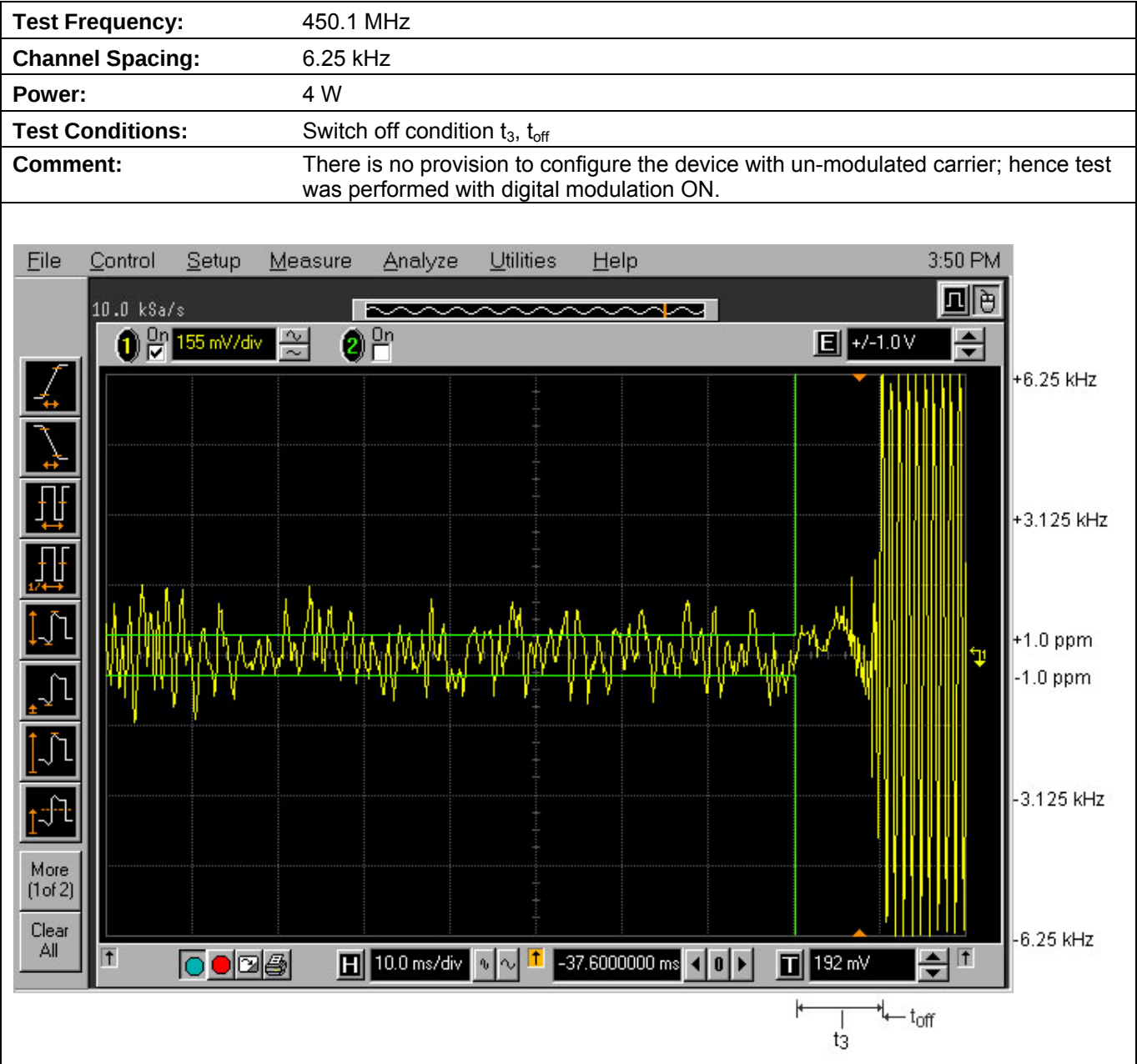
Plot 5.12.4.4. Transient Frequency Behavior for 6.25 kHz Channel Spacing
