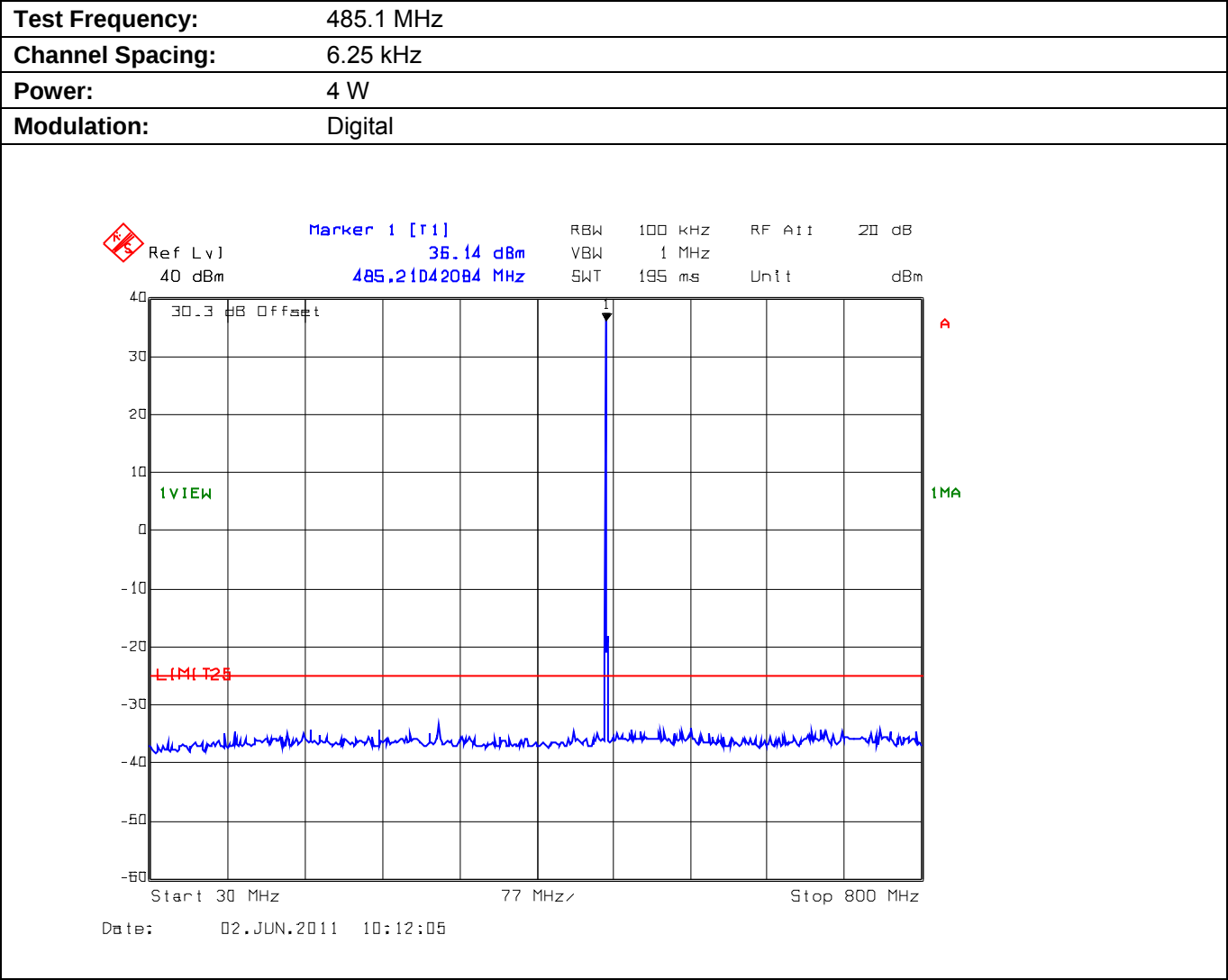
Plot 5.9.4.2.1. Conducted Transmitter Spurious Emissions for 485.1 MHz, High Power, 30 MHz - 800 MHz
