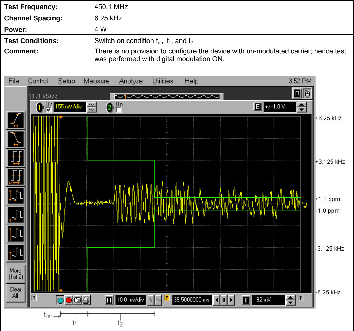
Plot 5.12.4.3. Transient Frequency Behavior for 6.25 kHz Channel Spacing
