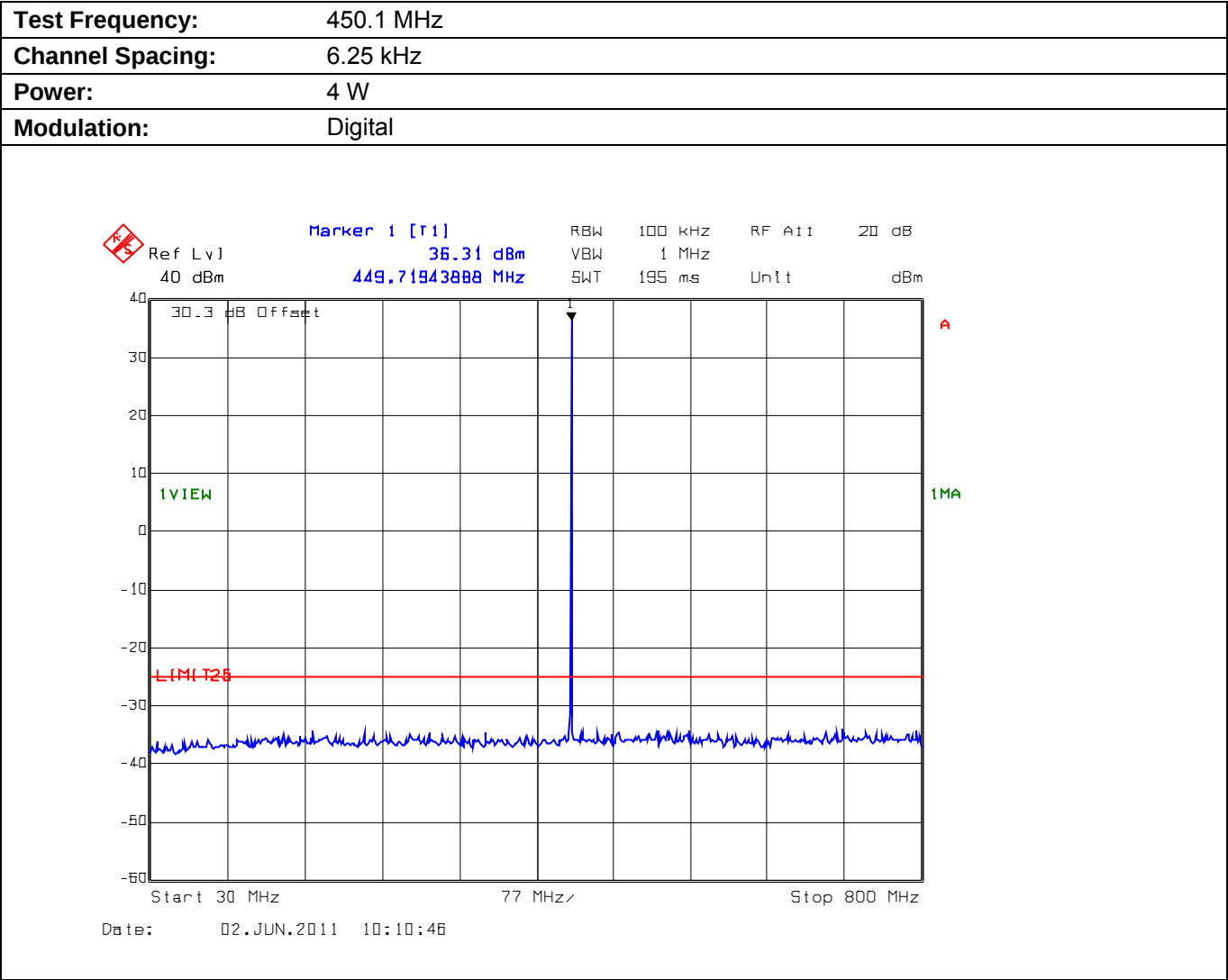
Plot 5.9.4.1.1. Conducted Transmitter Spurious Emissions for 450.1 MHz, High Power, 30 MHz - 800 MHz
