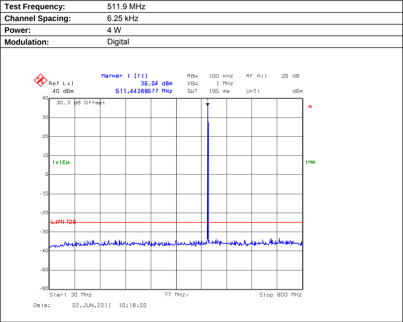
Plot 5.9.4.3.1. Conducted Transmitter Spurious Emissions for 511.9 MHz, High Power, 30 MHz - 800 MHz
