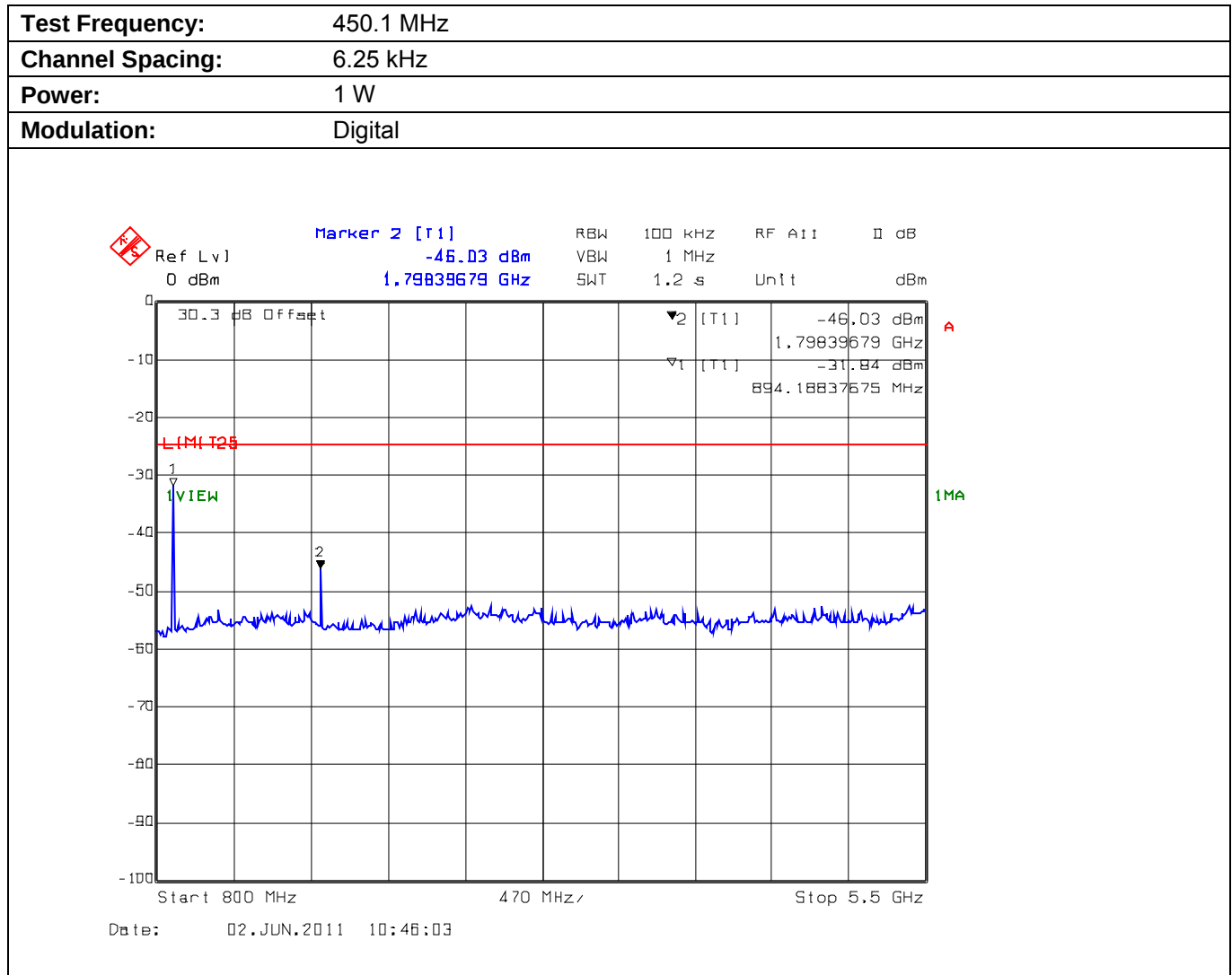
Plot 5.9.4.1.4. Conducted Transmitter Spurious Emissions for 450.1 MHz, Low Power, 800 MHz - 5.5 GHz
