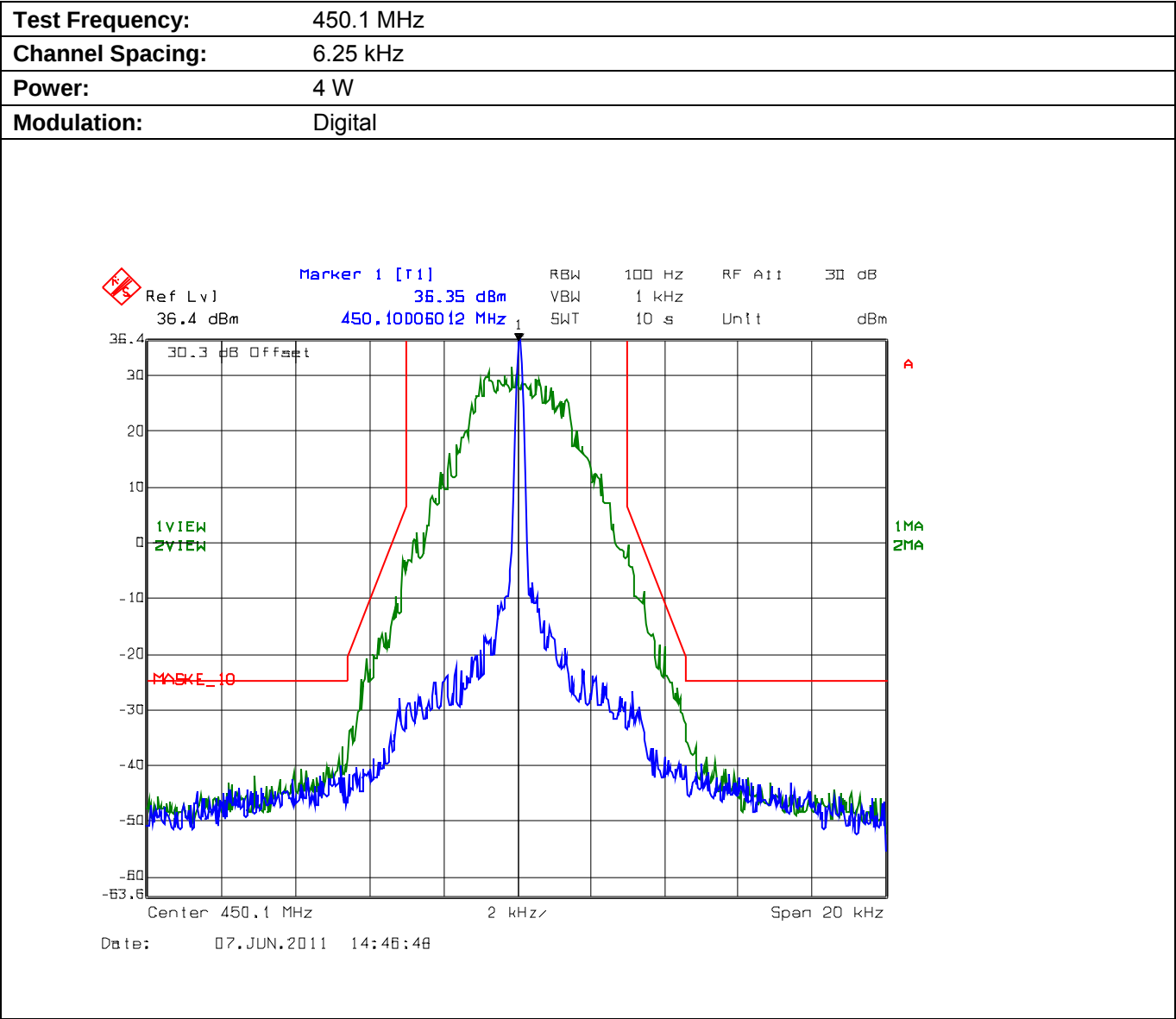
Plot 5.8.4.3.1. Emission Mask E, High Power
