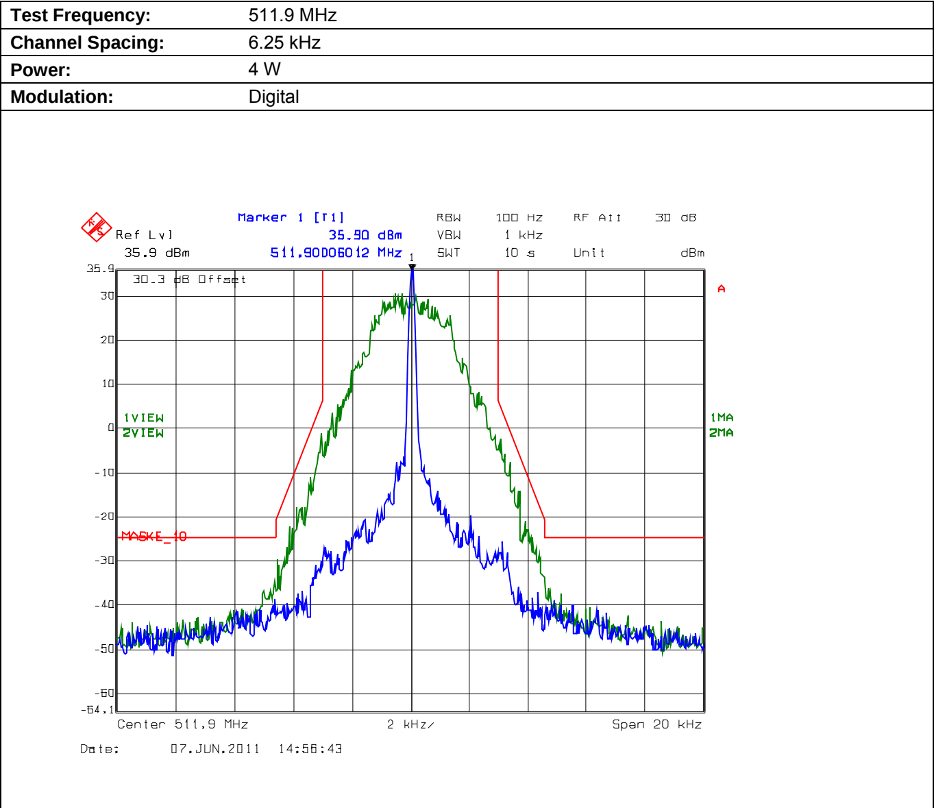
Plot 5.8.4.3.3. Emission Mask E, High Power
