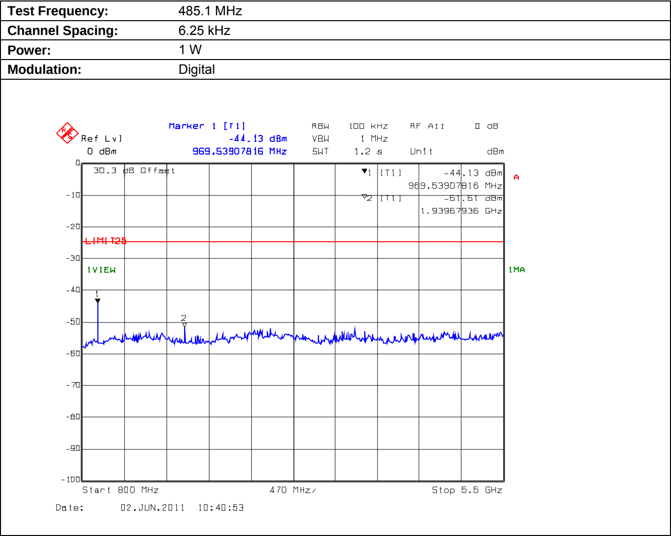
Plot 5.9.4.2.4. Conducted Transmitter Spurious Emissions for 485.1 MHz, Low Power, 800 MHz - 5.5 GHz
