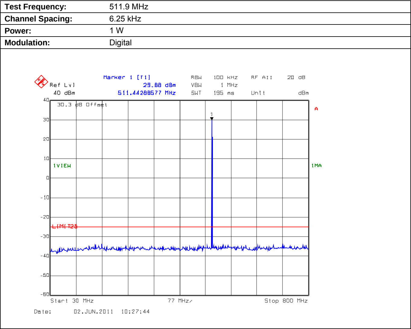
Plot 5.9.4.3.3. Conducted Transmitter Spurious Emissions for 511.9 MHz, Low Power, 30 MHz - 800 MHz
