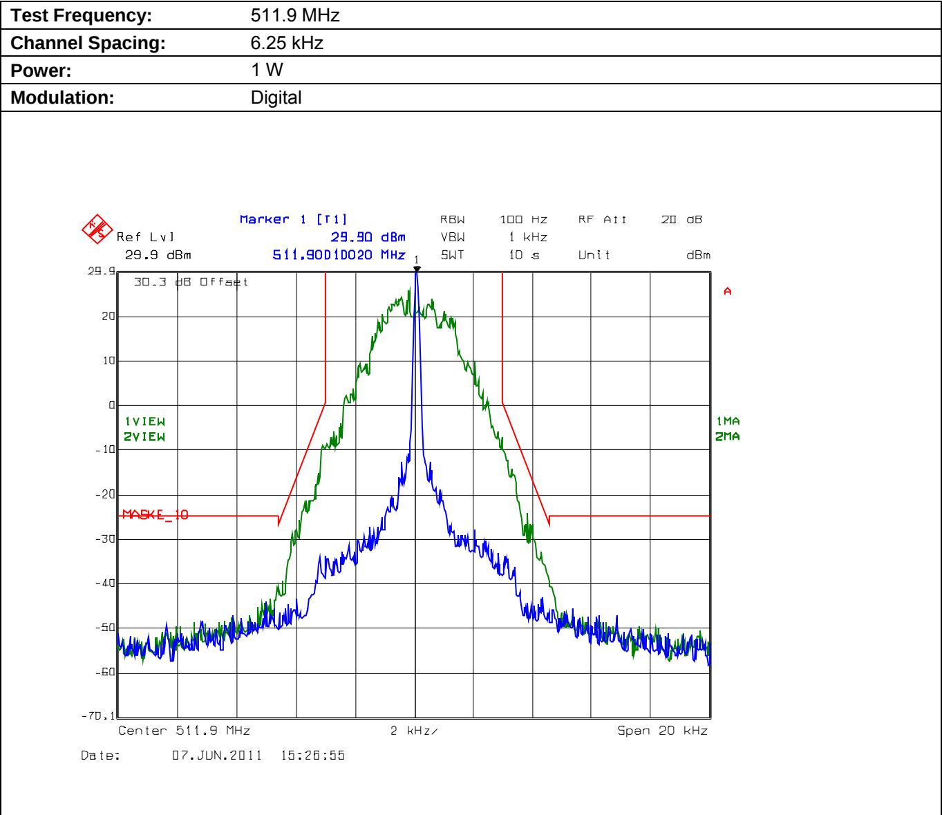
Plot 5.8.4.3.6. Emission Mask E, Low Power
