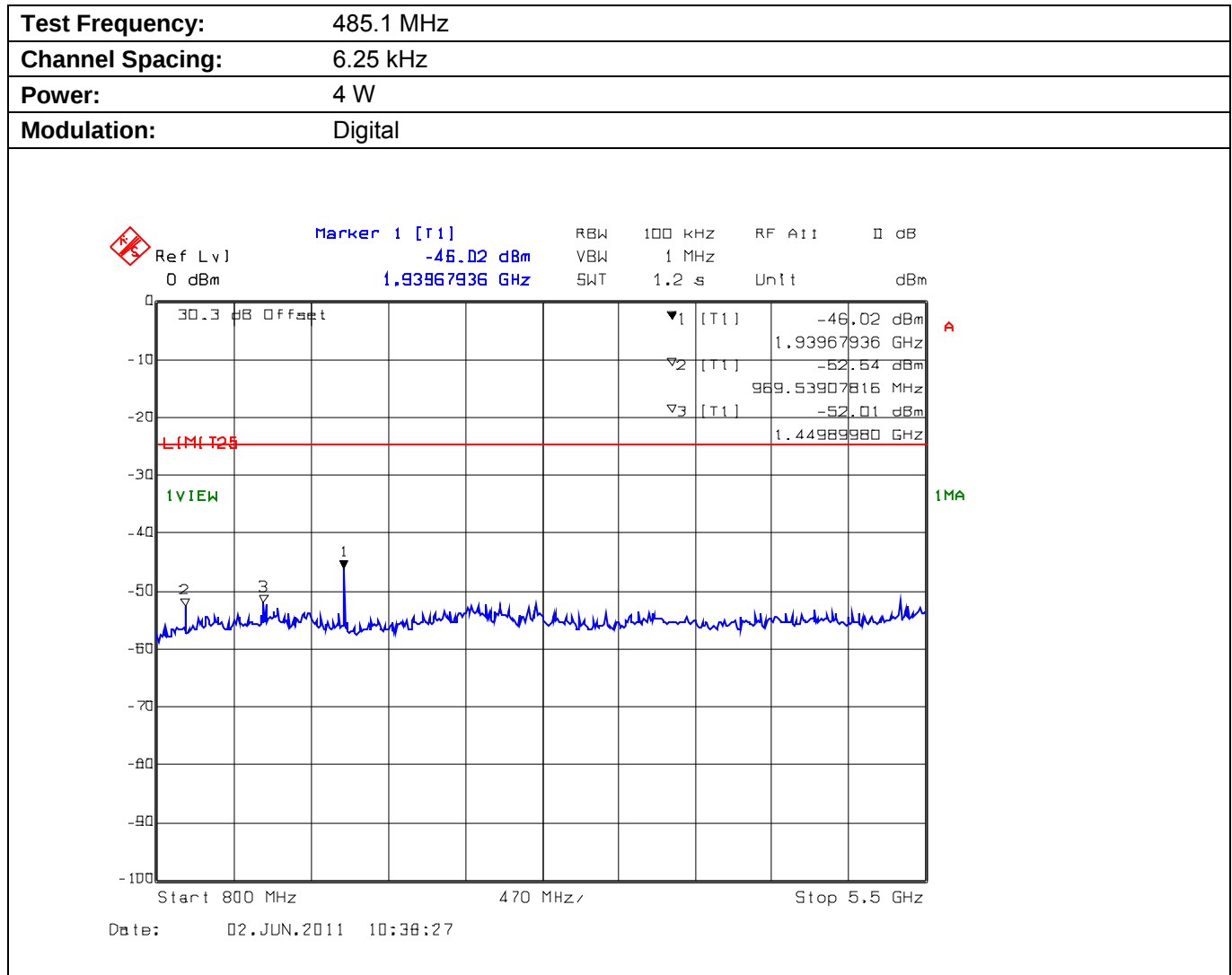
Plot 5.9.4.2.2. Conducted Transmitter Spurious Emissions for 485.1 MHz, High Power, 800 MHz - 5.5 GHz
