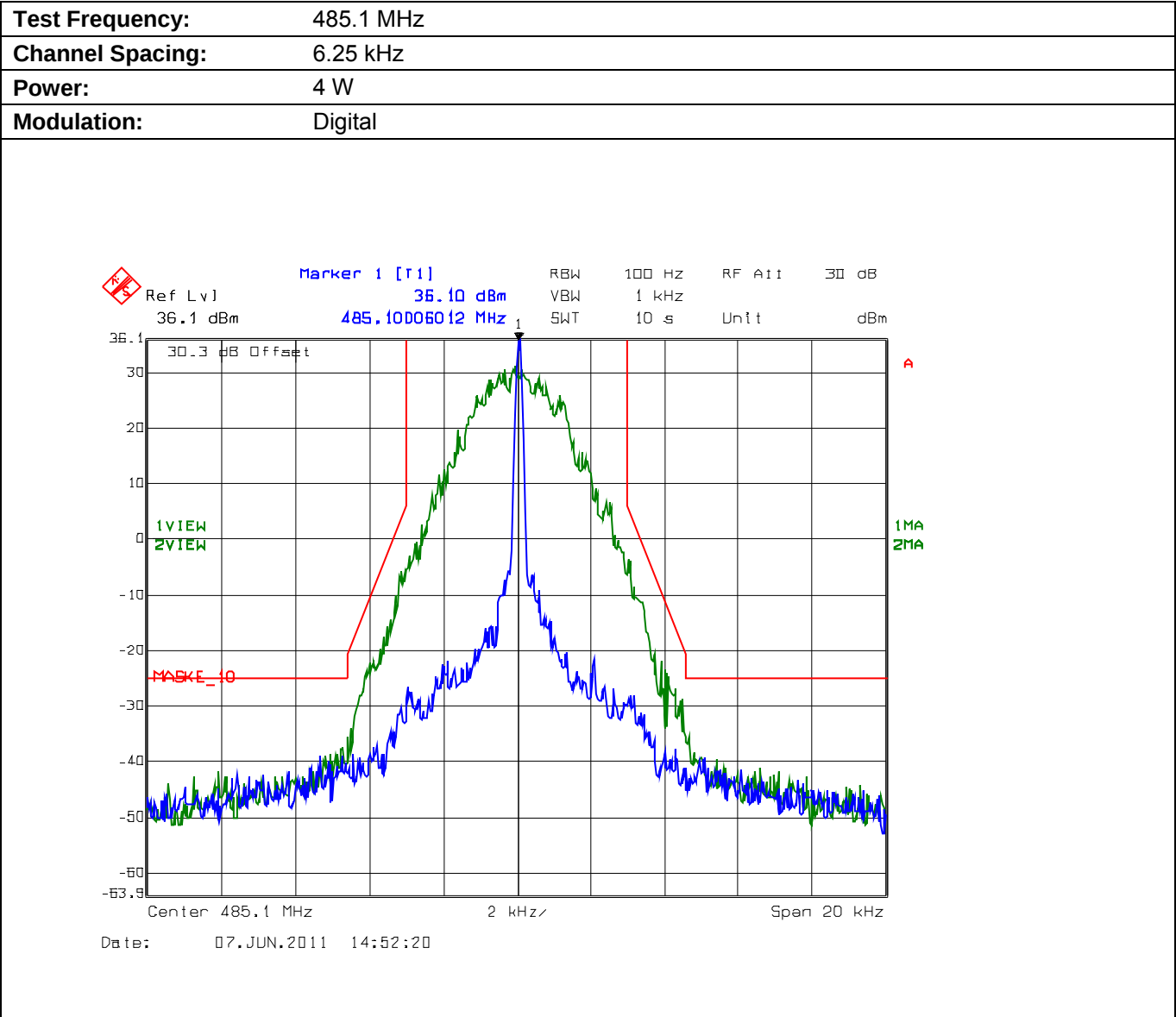
Plot 5.8.4.3.2. Emission Mask E, High Power
