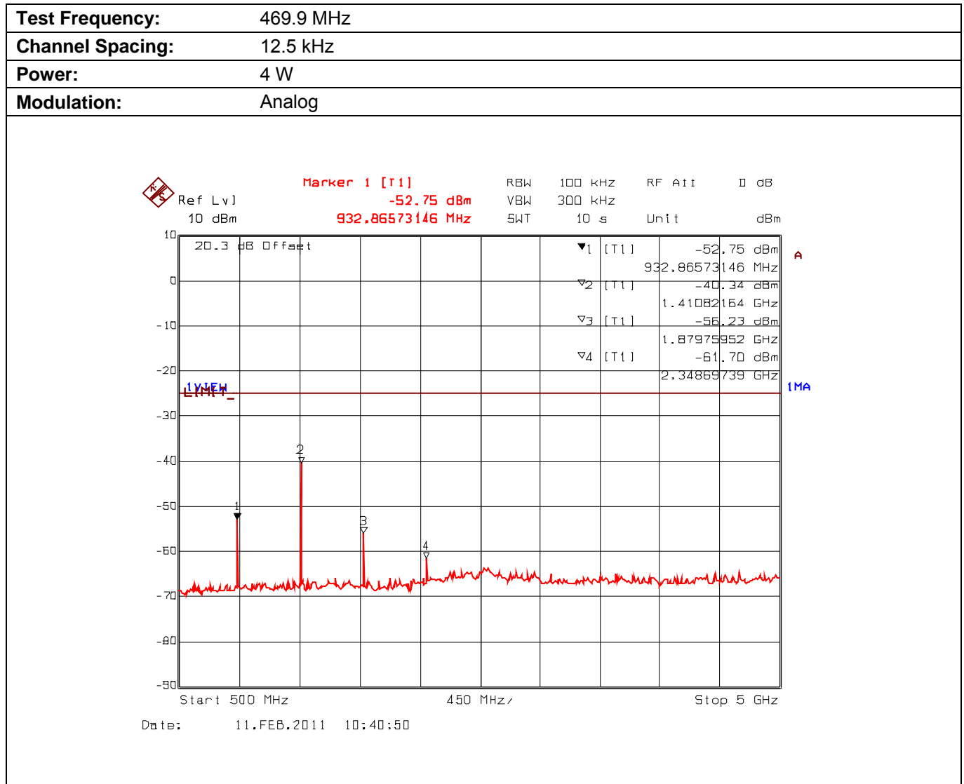
Plot 5.9.4.3.2. Conducted Transmitter Spurious Emissions for 469.9 MHz, High Power, 500 MHz - 5 GHz
