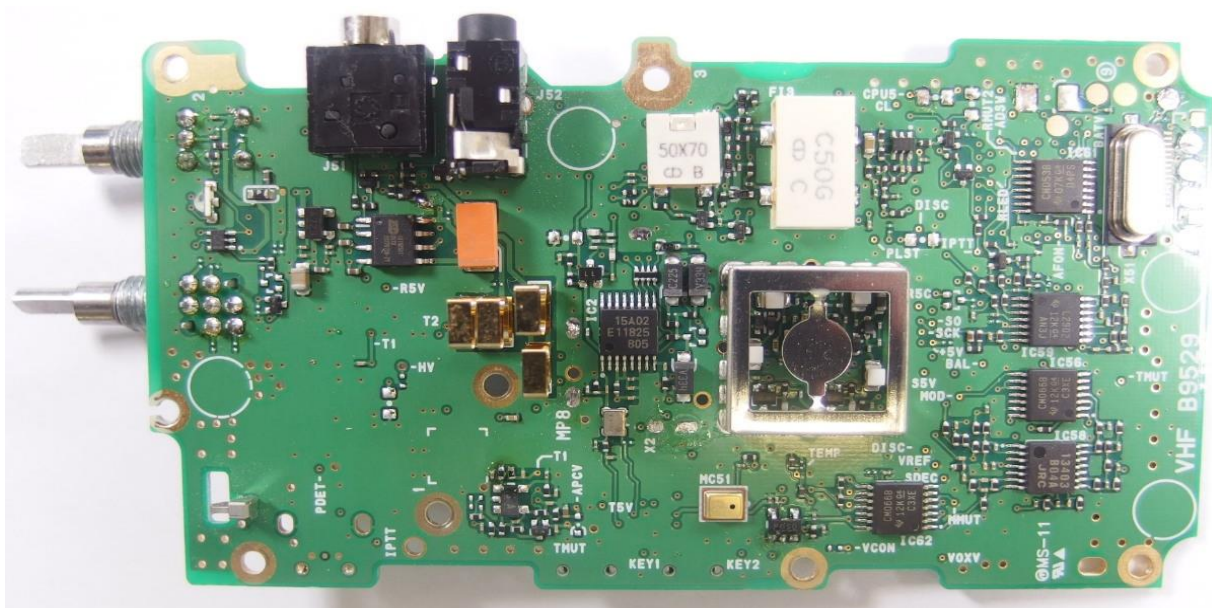
Main-B Board (side-A) view
