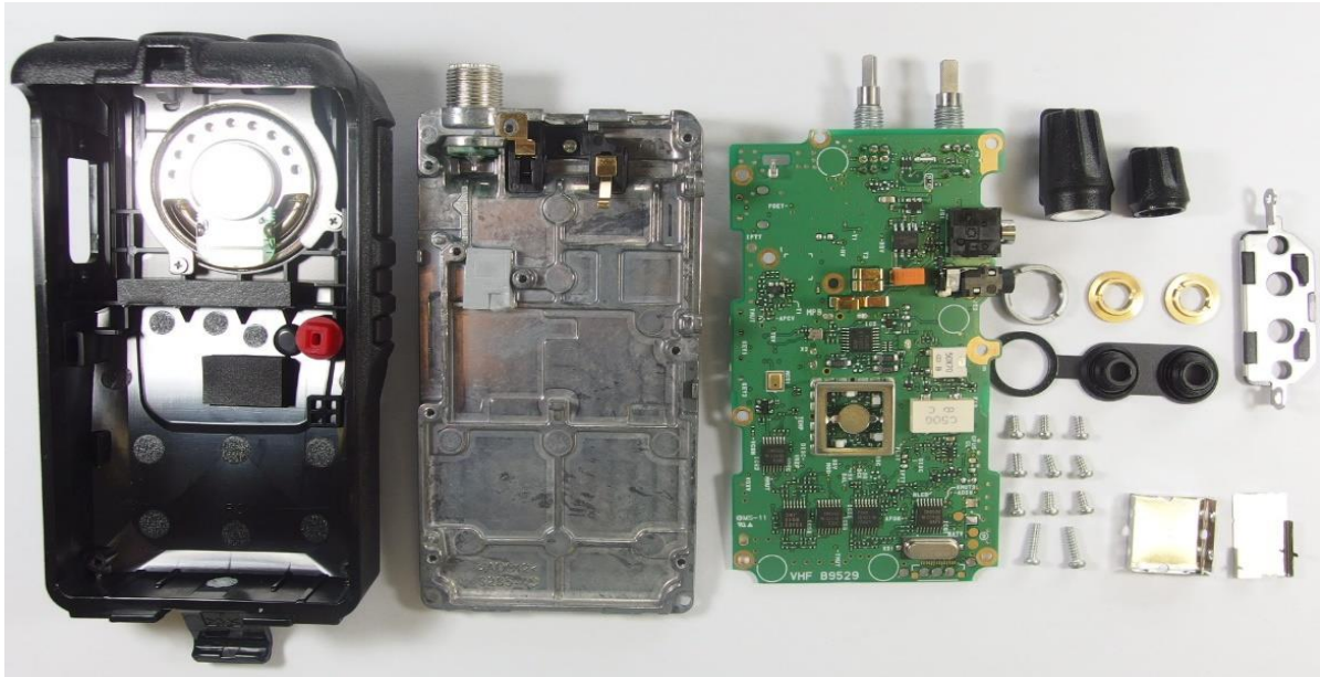
IC-V3MR CHASSIS
