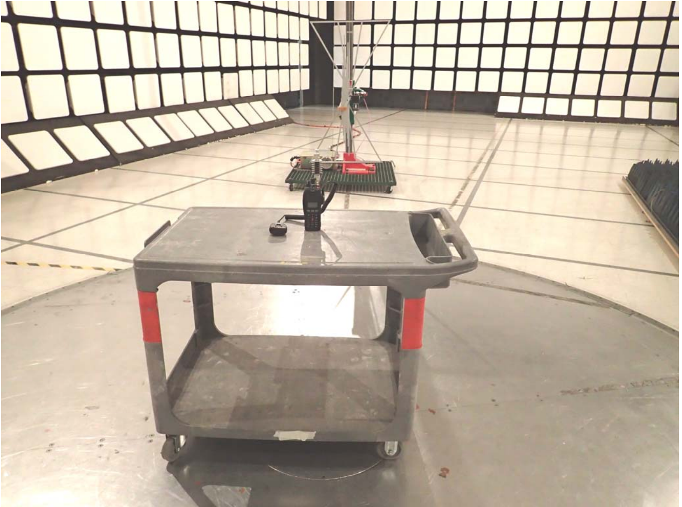
Transmitter Radiated Emission Test at 3m, 30 MHz to 1GHz - Position #1
