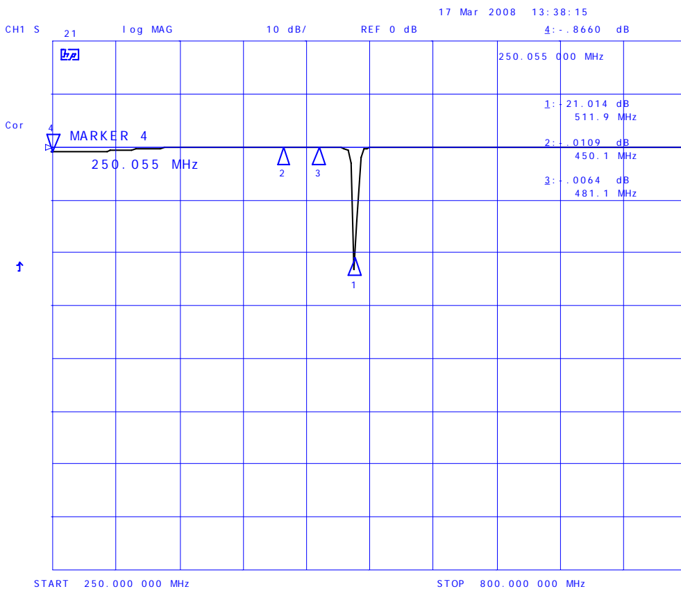
Plot # 54.: Notch Filter Characteristics 511.9MHz, K&L 500-1000MHz Tunable Bandreject Filter, P/N 3TNF-500/1000-N/N, S/N 470
