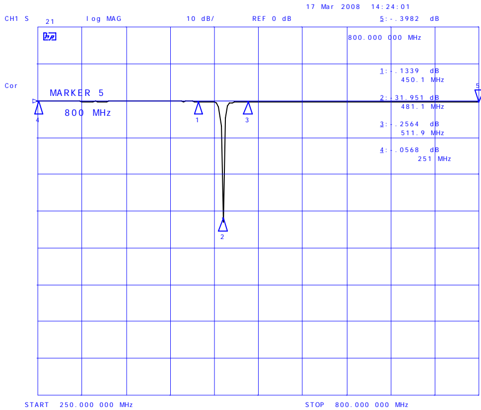
Plot # 53.: Notch Filter Characteristics 481.1MHz, K&L 250-500MHz Tunable Bandreject Filter, P/N 3TNF-250/500-N, S/N UU041-1
