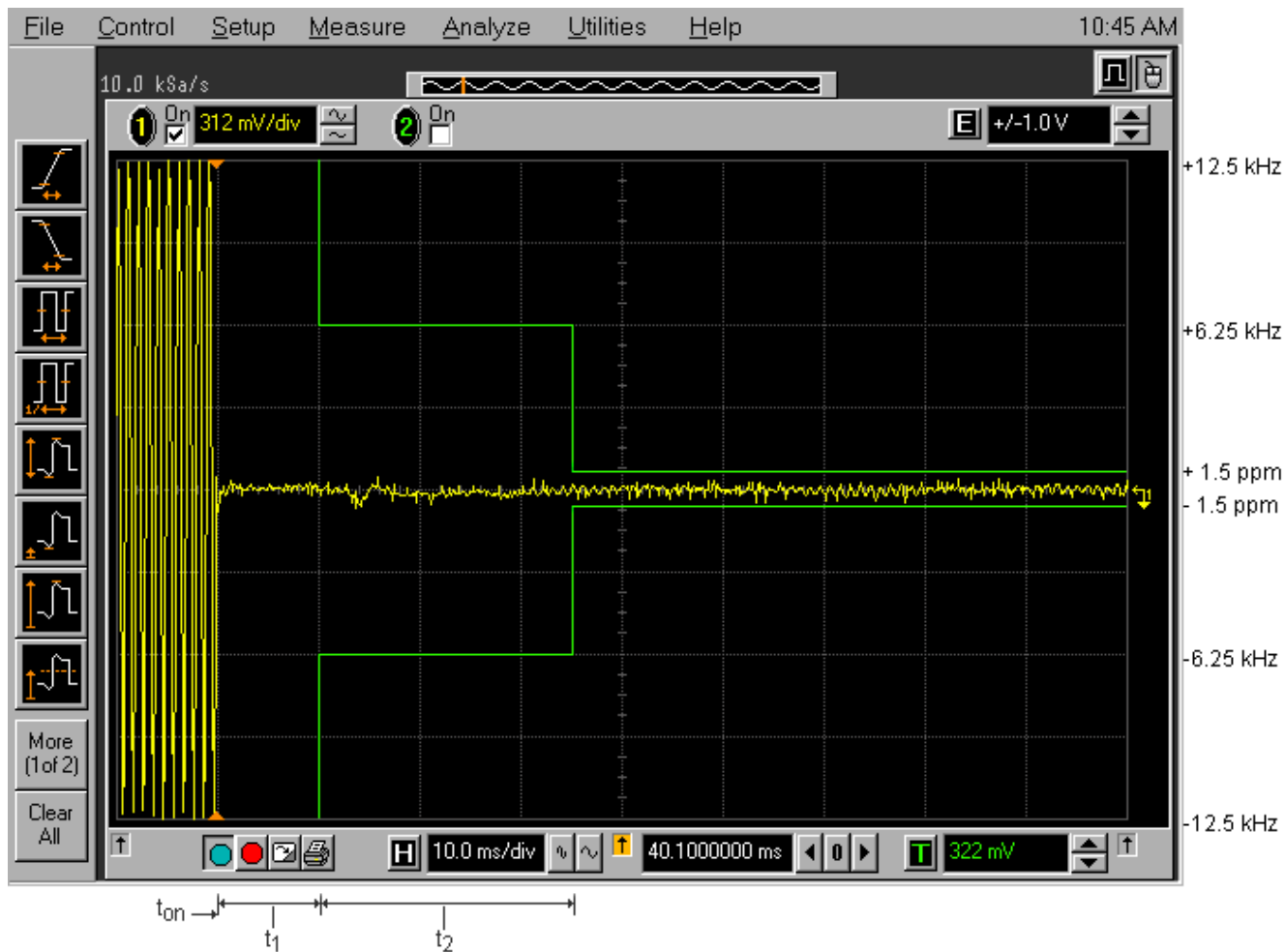
Plot 6.12.5.3 Transient Frequency Behavior Carrier Frequency: 406.2 MHz; Channel Spacing: 12.5 kHz; Power: 50 W Description: Switch on condition t_{on} , t_1 , and t_2
