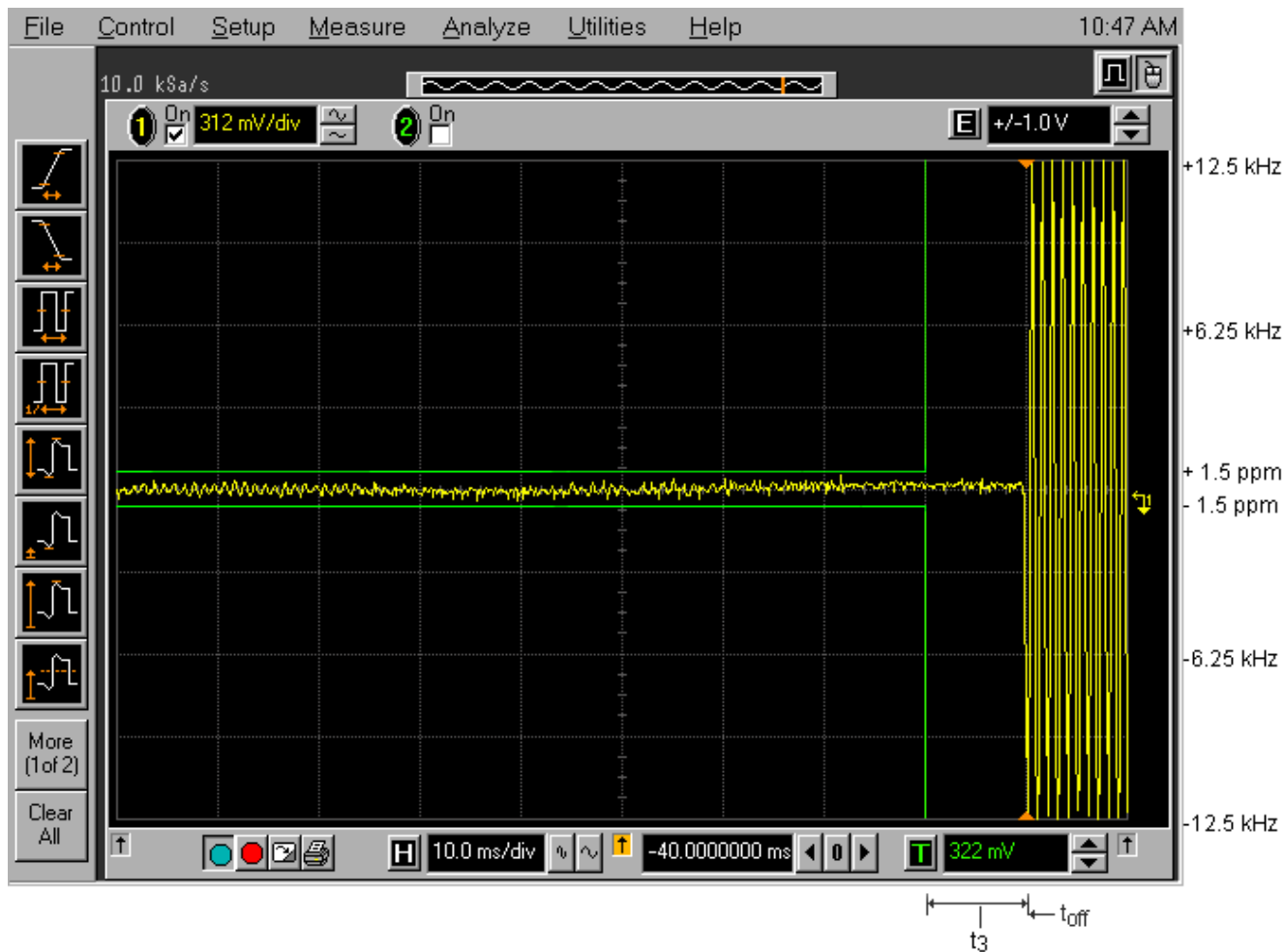
Plot 6.12.5.4 Transient Frequency Behavior Carrier Frequency: 406.2 MHz; Channel Spacing: 12.5 kHz; Power: 50 W Description: Switch off condition t_3 , t_{off}
