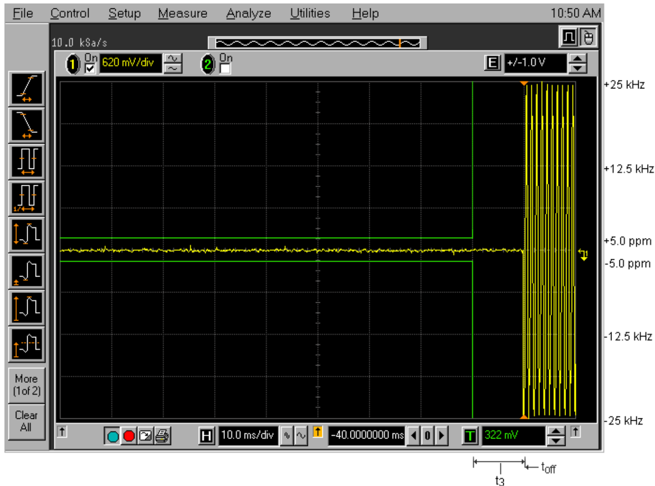
Plot 6.12.5.2 Transient Frequency Behavior Carrier Frequency: 406.2 MHz; Channel Spacing: 25 kHz; Power: 50 W Description: Switch off condition t_3 , t_{off}
