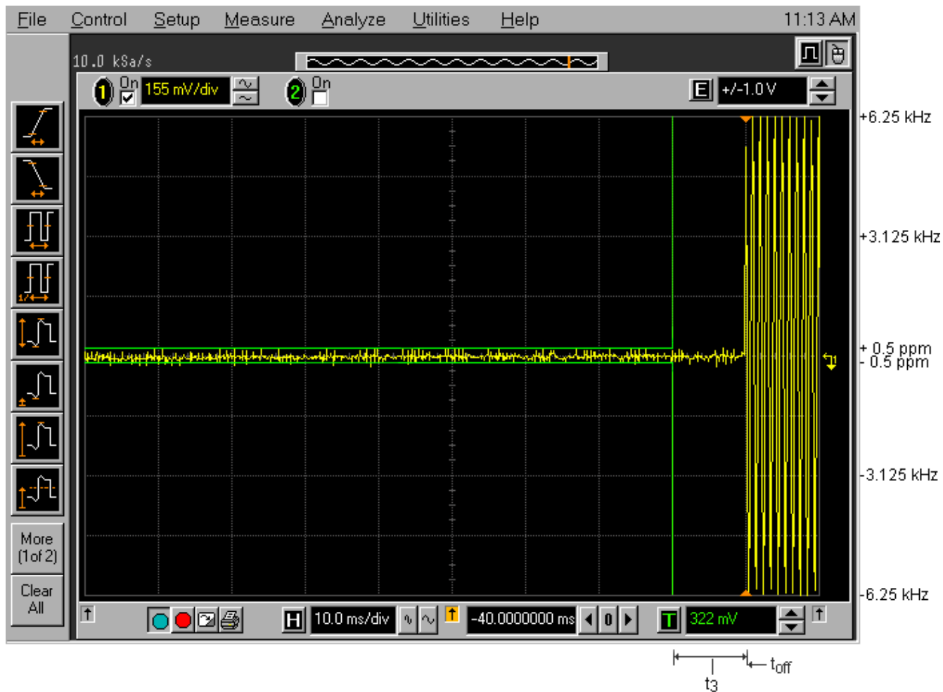
Plot 6.12.5.6 Transient Frequency Behavior Carrier Frequency: 406.2 MHz; Channel Spacing: 6.25 kHz; Power: 50 W Description: Switch off condition t_3 , t_{off}
