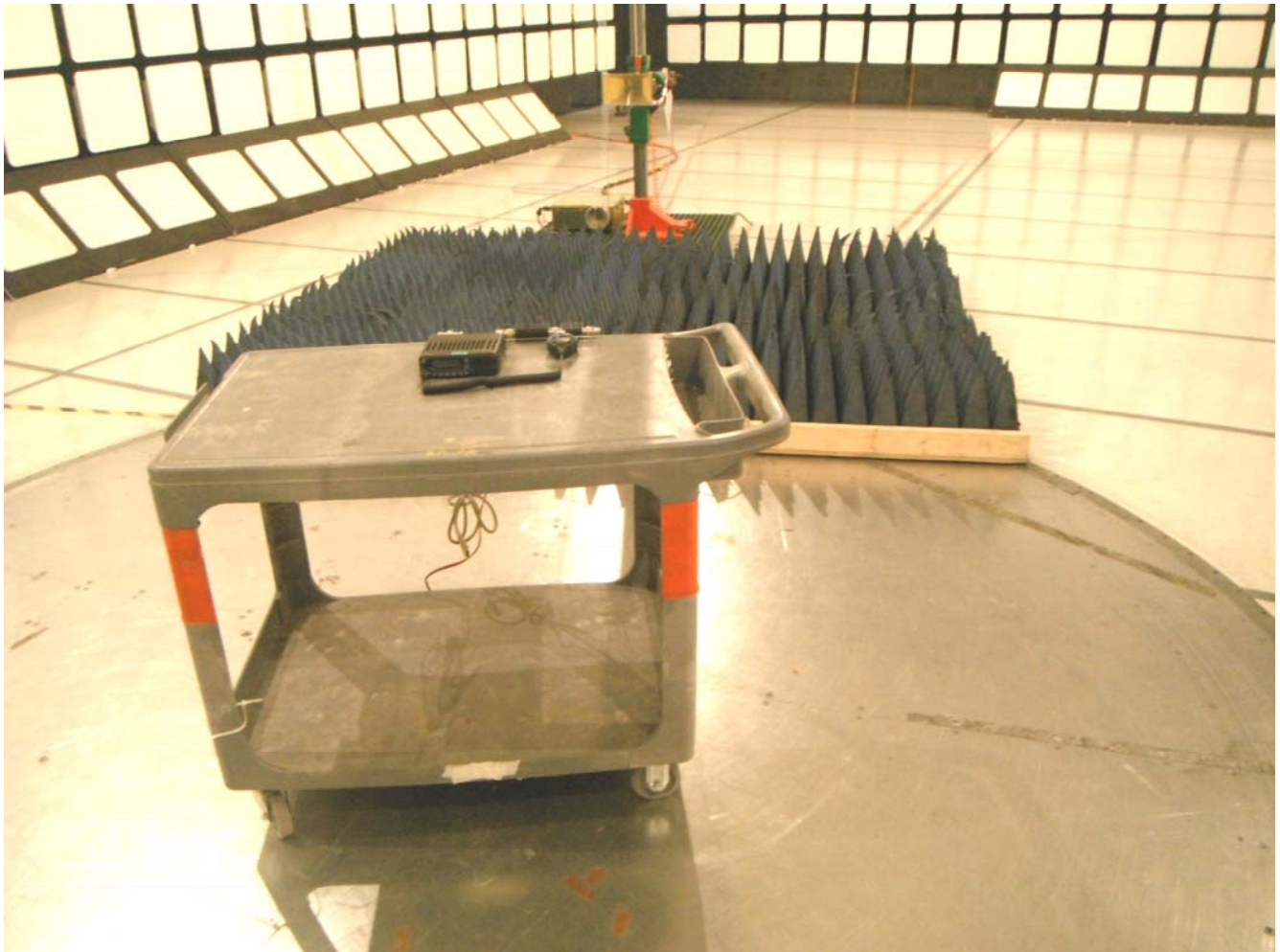
Transmitter Radiated Emission Test at 3m, Above 1GHz
