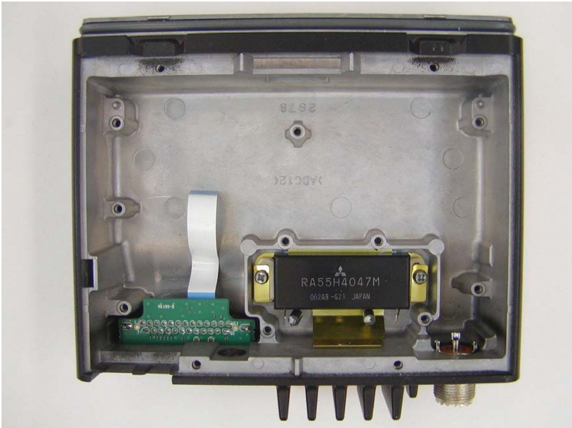
CHASSIS inside
