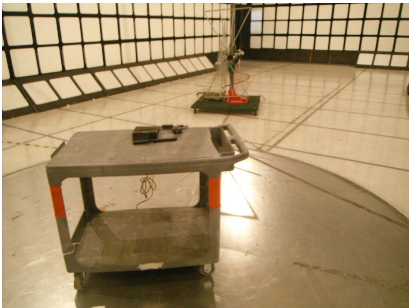
Transmitter Radiated Emission Test at 3m, 30 MHz to 1GHz
