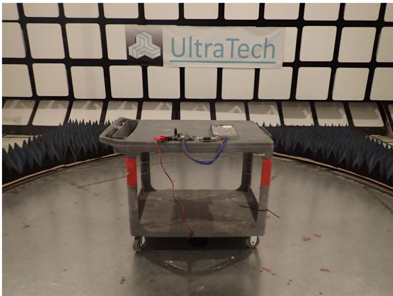
Radiated Emission at 3m Distance (30 – 1000 MHz)
