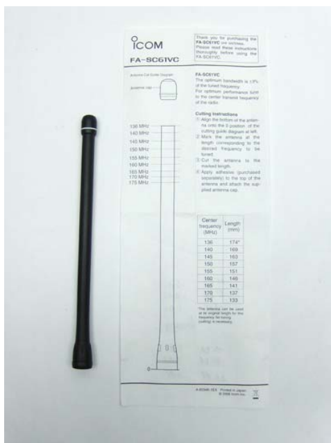
&lt; FA-SC61VC cut antenna (White Ring) &gt;
