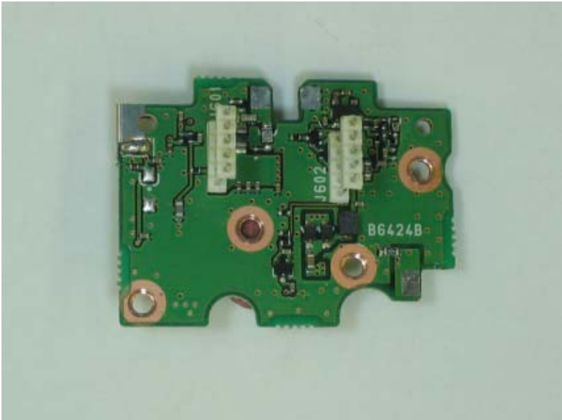
RF SIDE A
