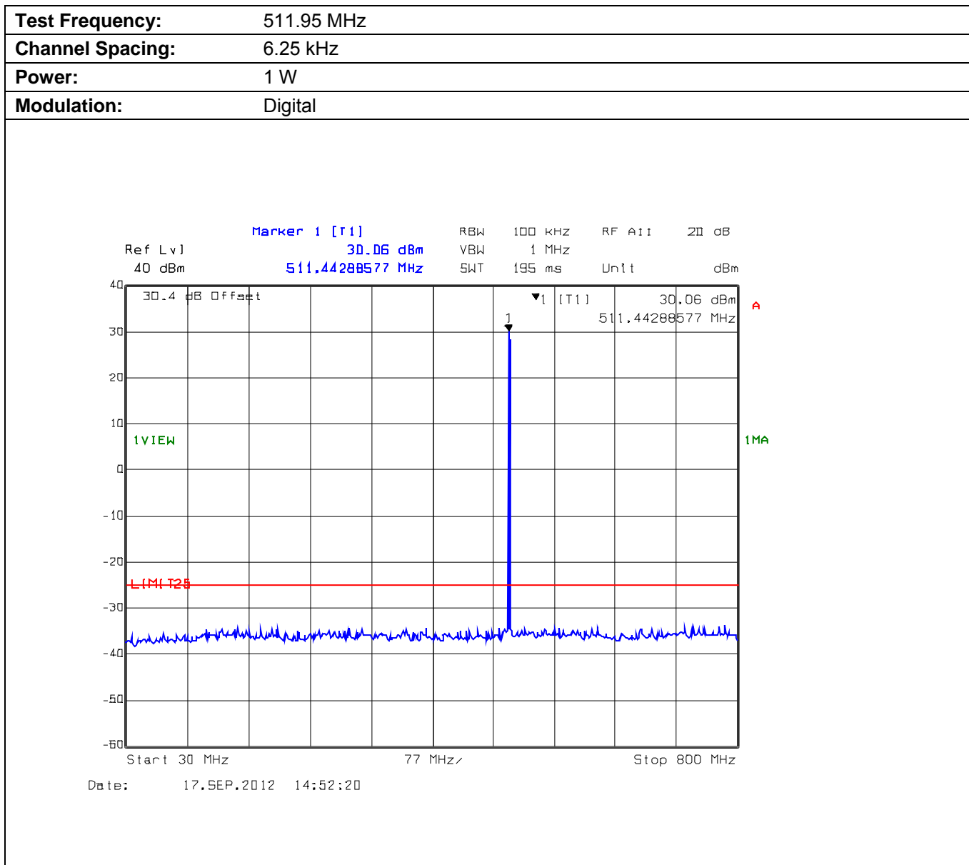
Plot 5.9.4.3.3. Conducted Transmitter Spurious Emissions for 511.95 MHz, Low Power, 30 MHz - 800 MHz
