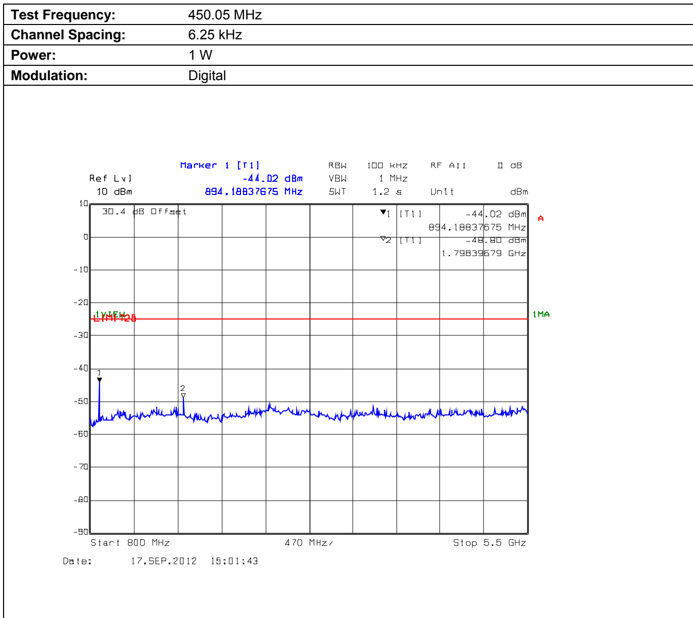
Plot 5.9.4.1.4. Conducted Transmitter Spurious Emissions for 450.05 MHz, Low Power, 800 MHz – 5.5 GHz
