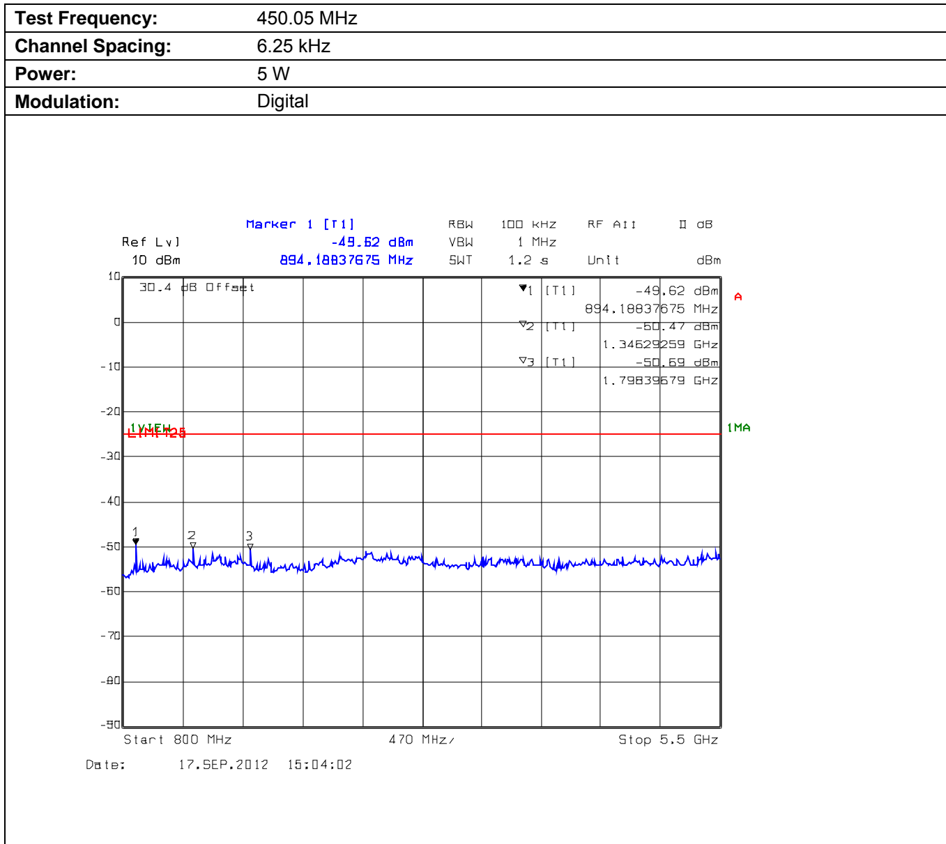
Plot 5.9.4.1.2. Conducted Transmitter Spurious Emissions for 450.05 MHz, High Power, 800 MHz - 5.5 GHz
