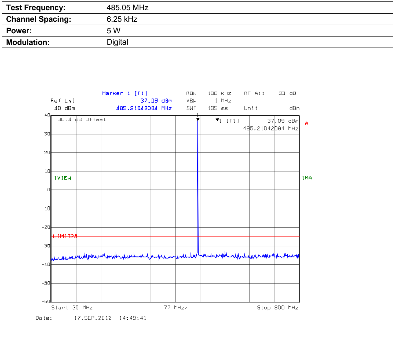
Plot 5.9.4.2.1. Conducted Transmitter Spurious Emissions for 485.05 MHz, High Power, 30 MHz - 800 MHz
