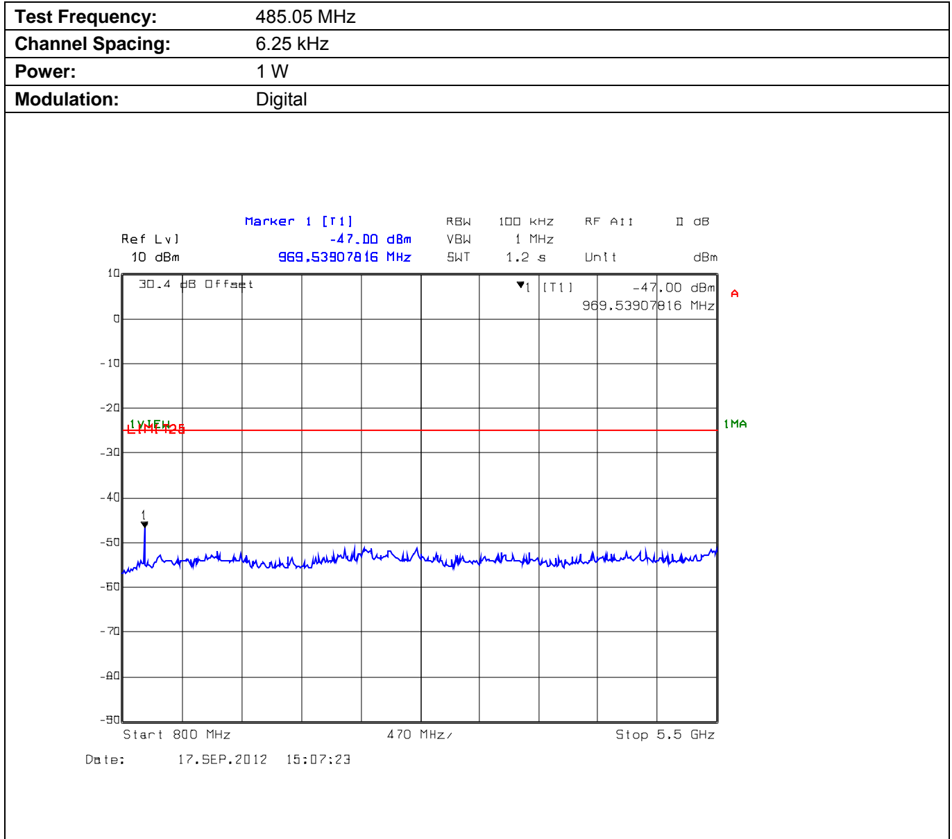
Plot 5.9.4.2.4. Conducted Transmitter Spurious Emissions for 485.05 MHz, Low Power, 800 MHz – 5.5 GHz
