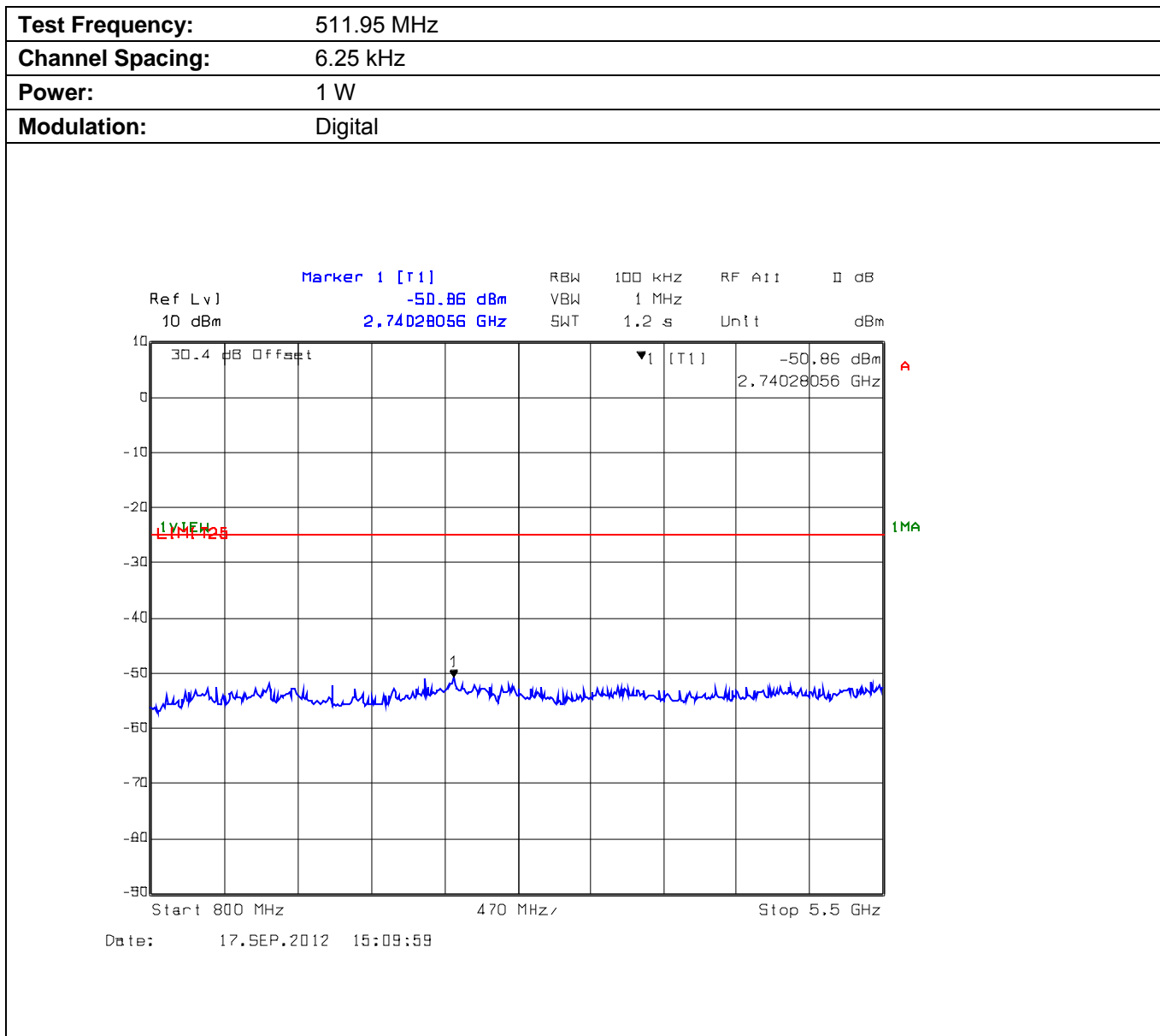
Plot 5.9.4.3.4. Conducted Transmitter Spurious Emissions for 511.95 MHz, Low Power, 800 MHz – 5.5 GHz
