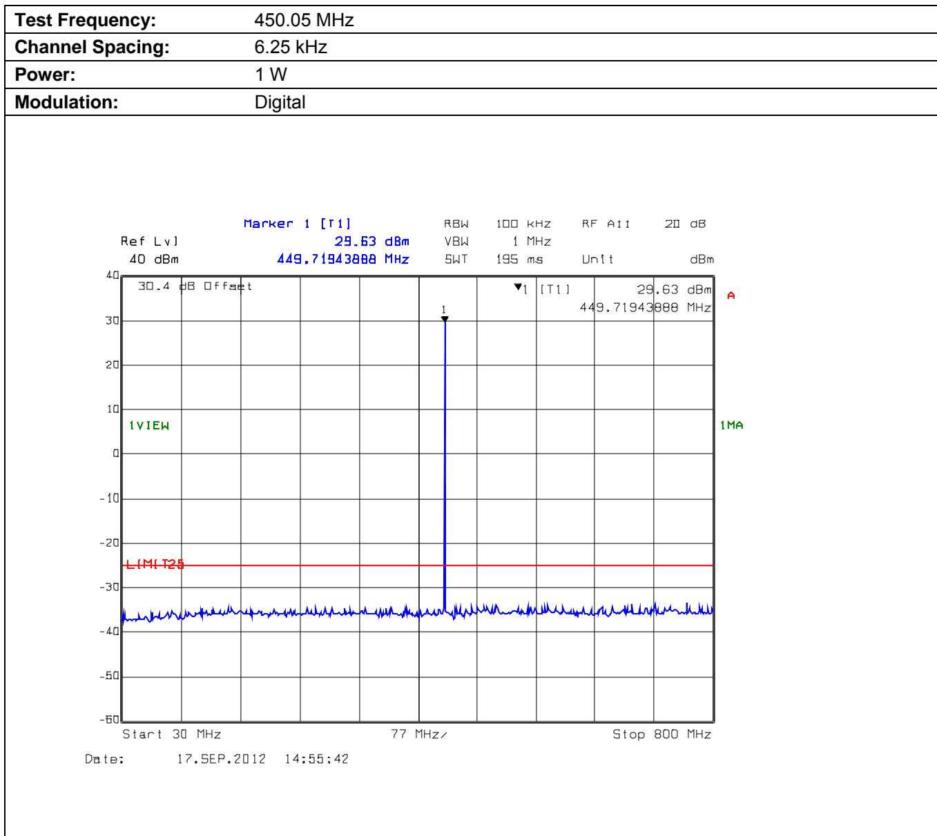
Plot 5.9.4.1.3. Conducted Transmitter Spurious Emissions for 450.05 MHz, Low Power, 30 MHz - 800 MHz
