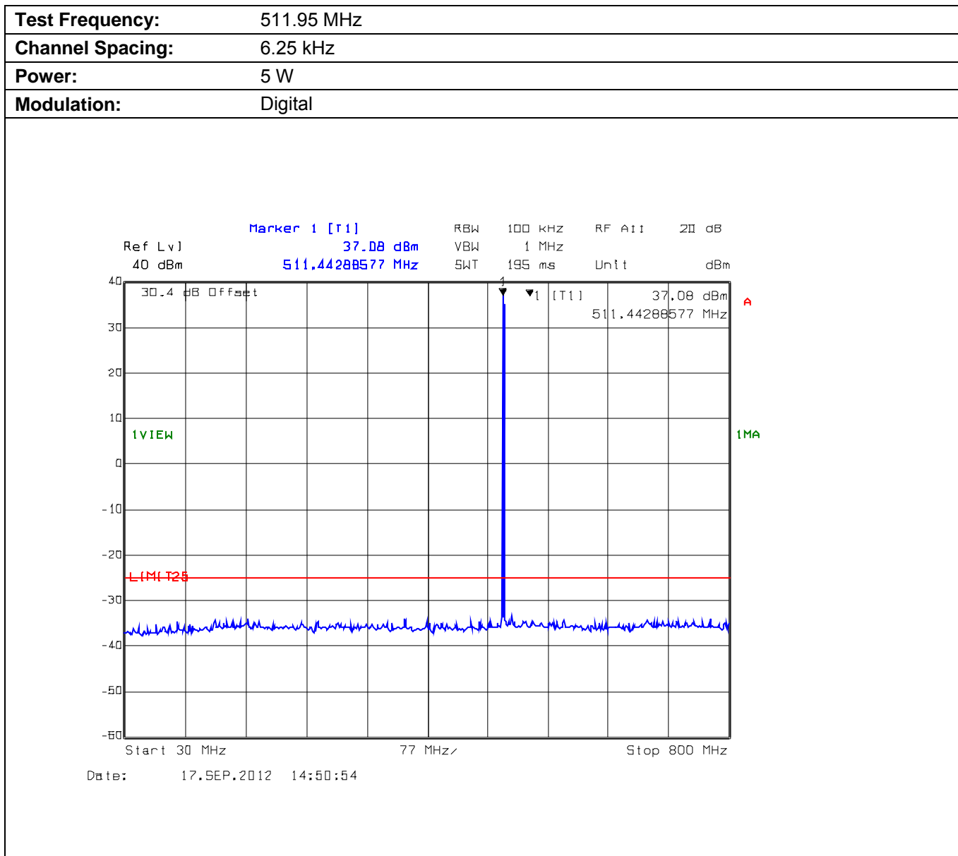
Plot 5.9.4.3.1. Conducted Transmitter Spurious Emissions for 511.95 MHz, High Power, 30 MHz - 800 MHz
