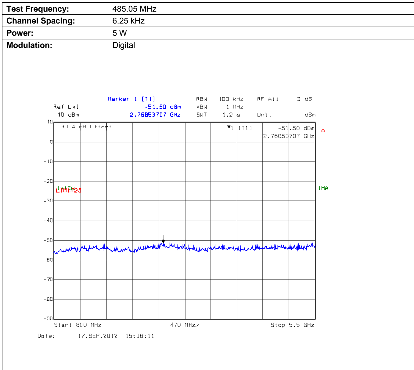
Plot 5.9.4.2.2. Conducted Transmitter Spurious Emissions for 485.05 MHz, High Power, 800 MHz – 5.5 GHz
