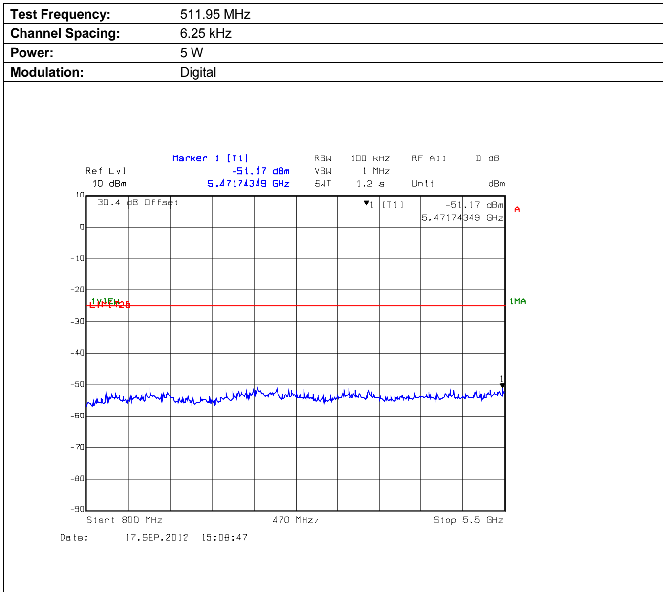
Plot 5.9.4.3.2. Conducted Transmitter Spurious Emissions for 511.95 MHz, High Power, 800 MHz – 5.5 GHz
