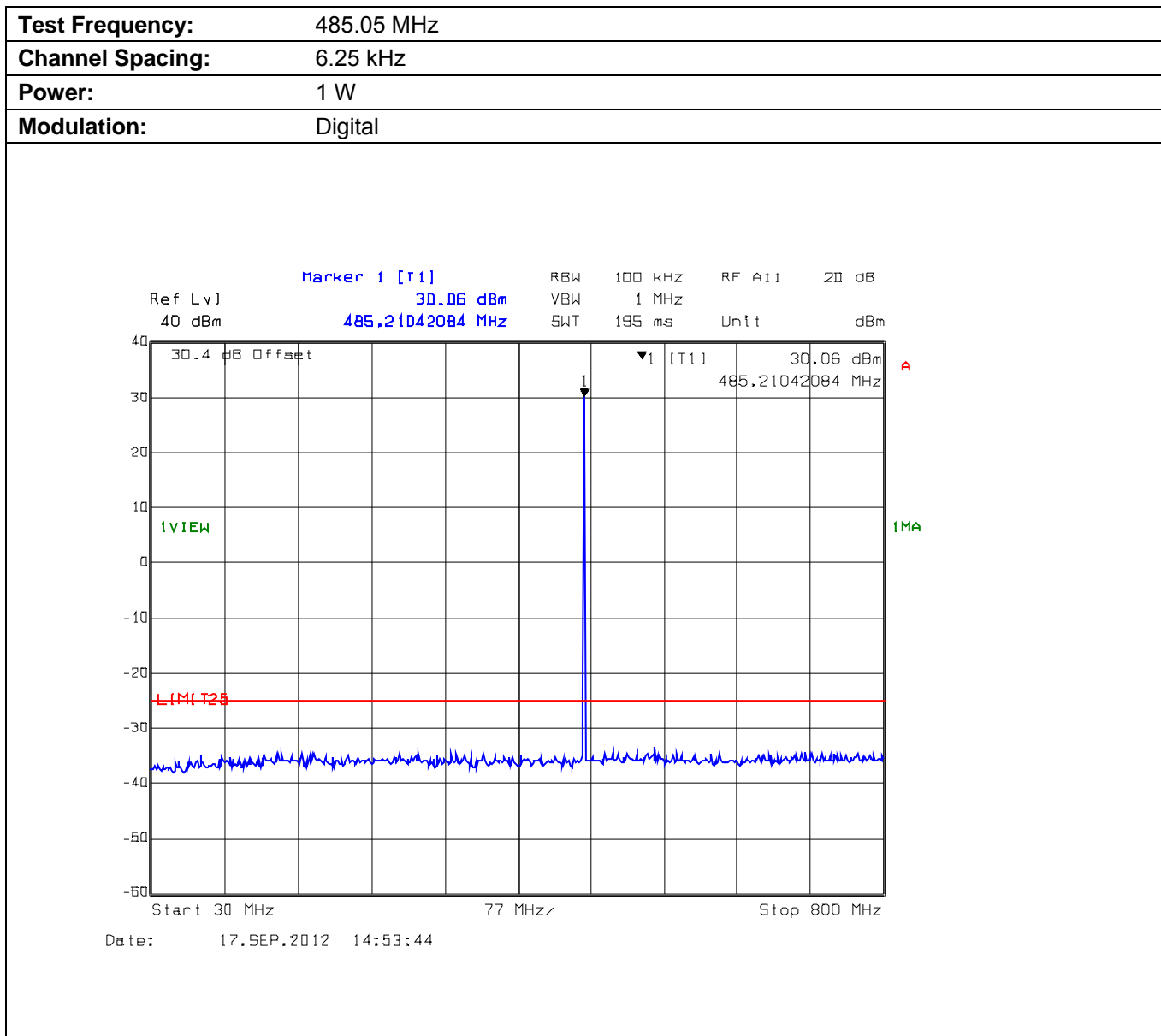
Plot 5.9.4.2.3. Conducted Transmitter Spurious Emissions for 485.05 MHz, Low Power, 30 MHz - 800 MHz
