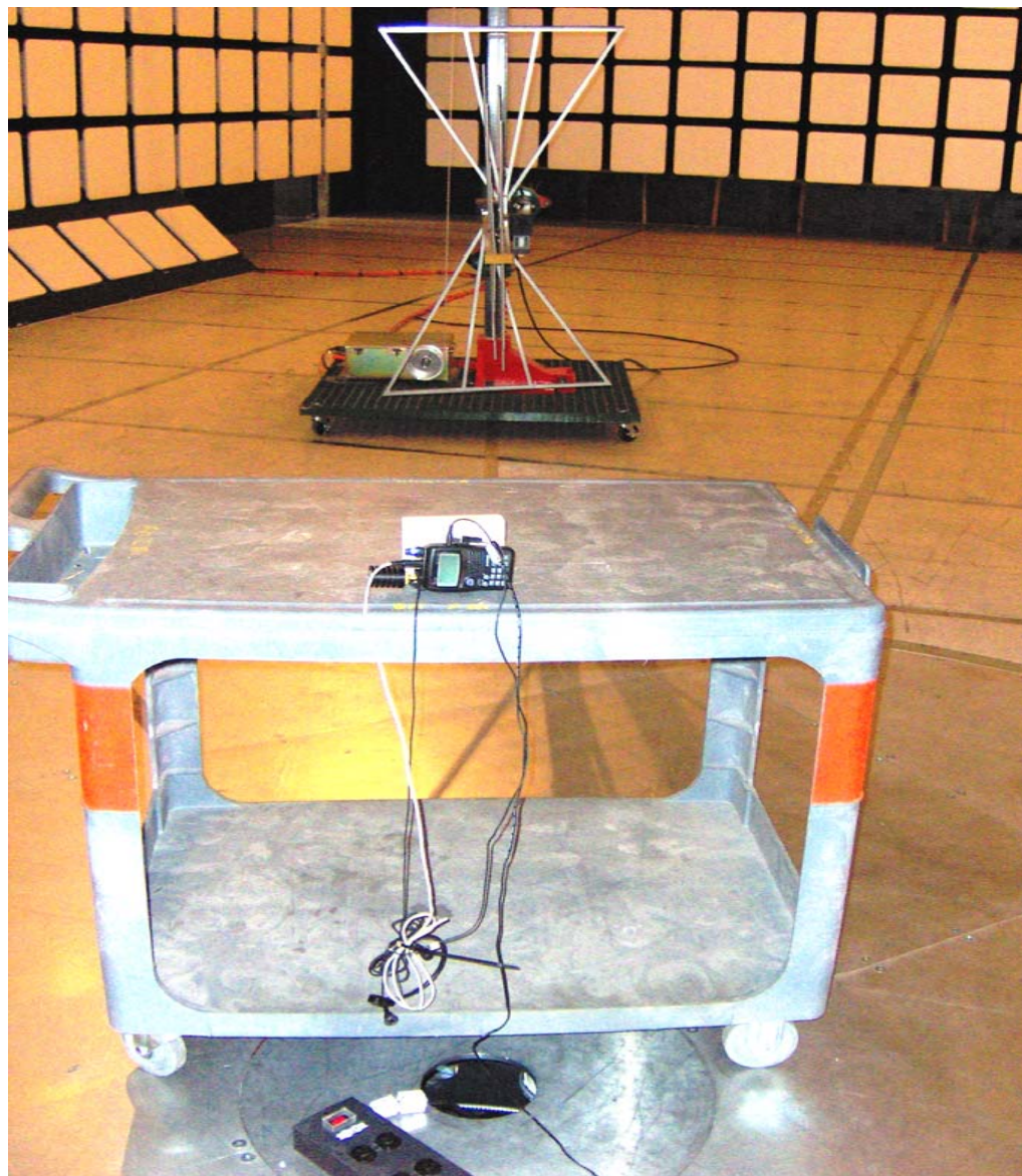
Photo # 5: Radiated Emissions at 3 meters OFTS
