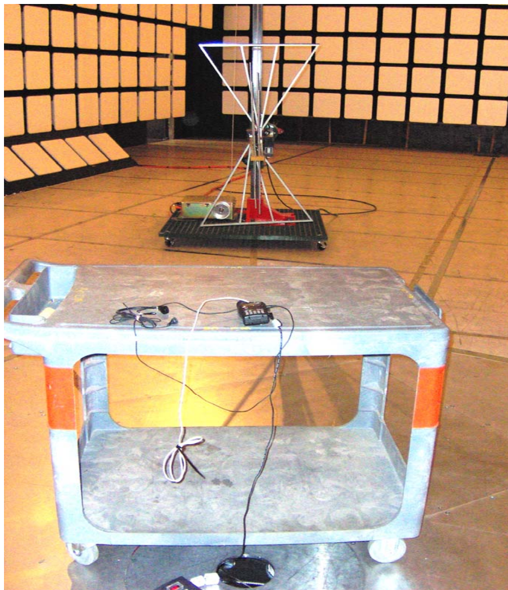
Photo #3: Receiver Radiated Emissions at 3 meters OFTS
