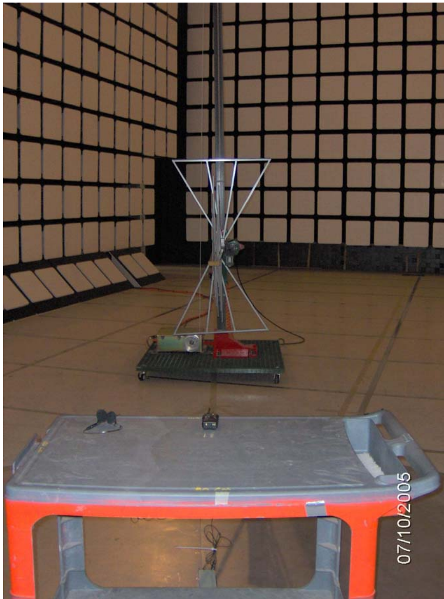
Photo #4: Receiver Radiated Emissions at 3 meters OFTS – EUT's Orthogonal Position #2
