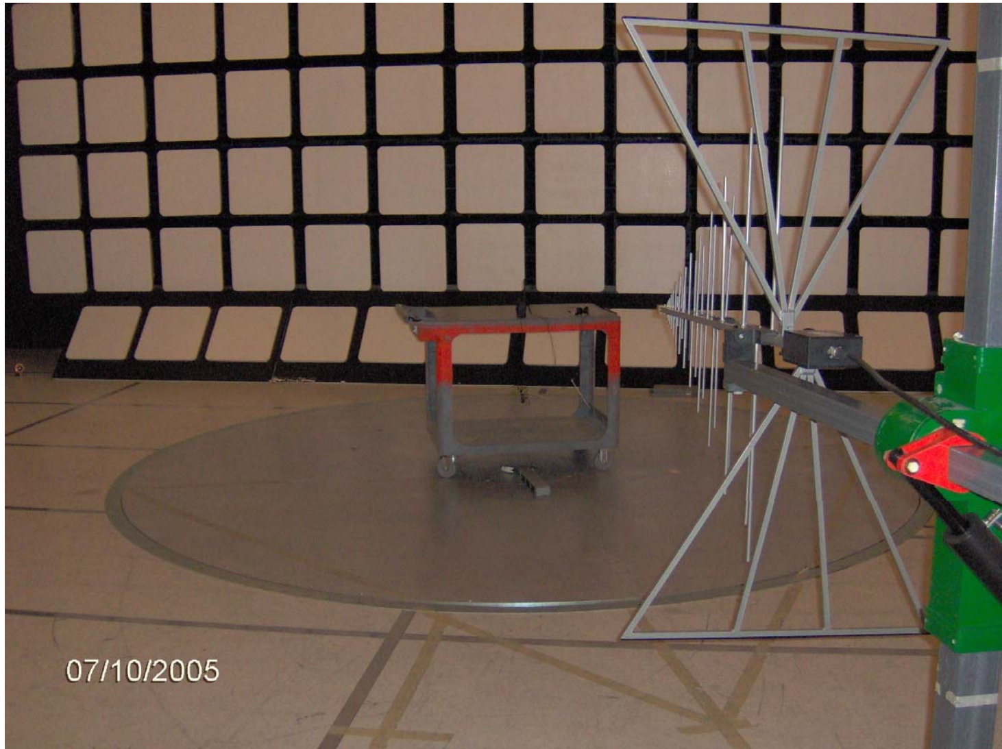
Photo #3: Receiver Radiated Emissions at 3 meters OFTS – EUT's Orthogonal Position #1
