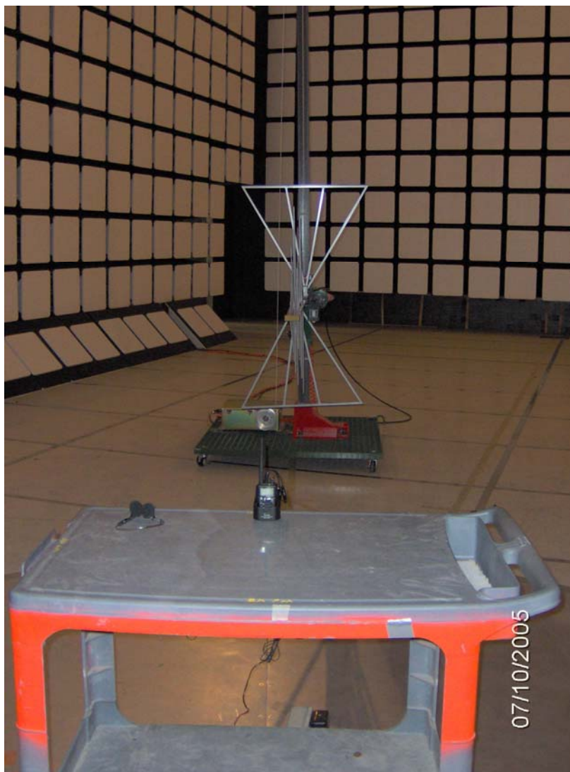
Photo #6: Radiated Emissions at 3 meters OFTS with Desktop Battery Charger and AC/DC Power Supply
