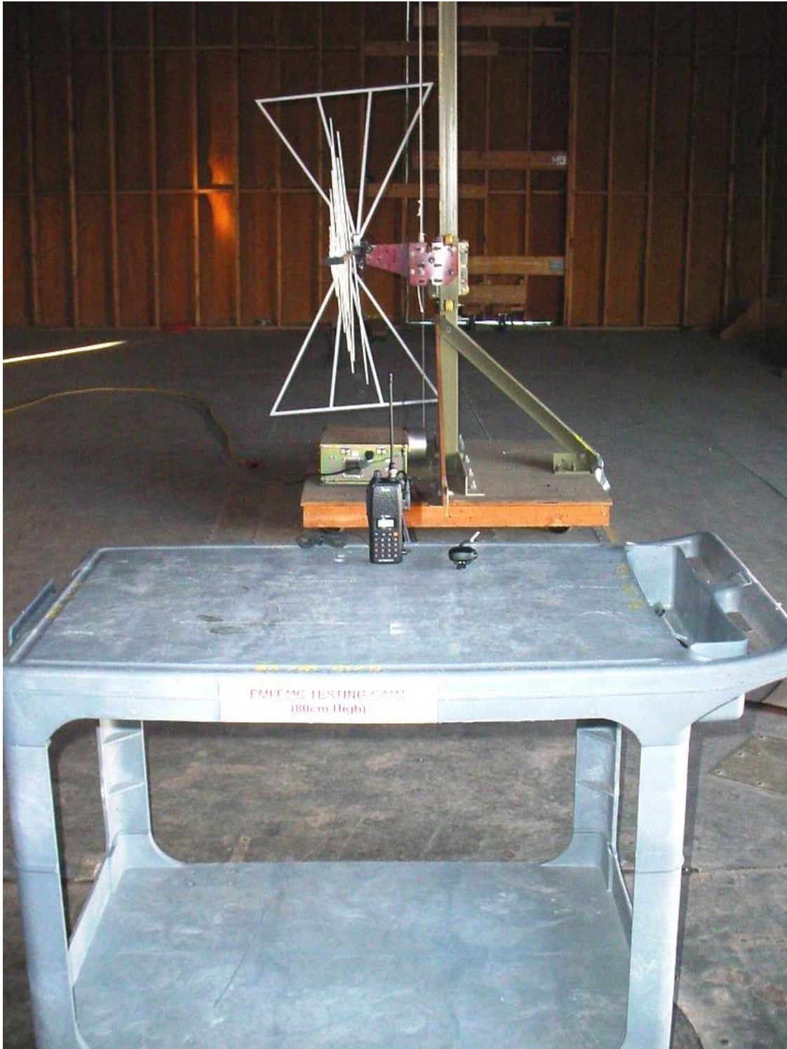
Radiated Emissions at 3 Meters (Orthogonal Position 1)
