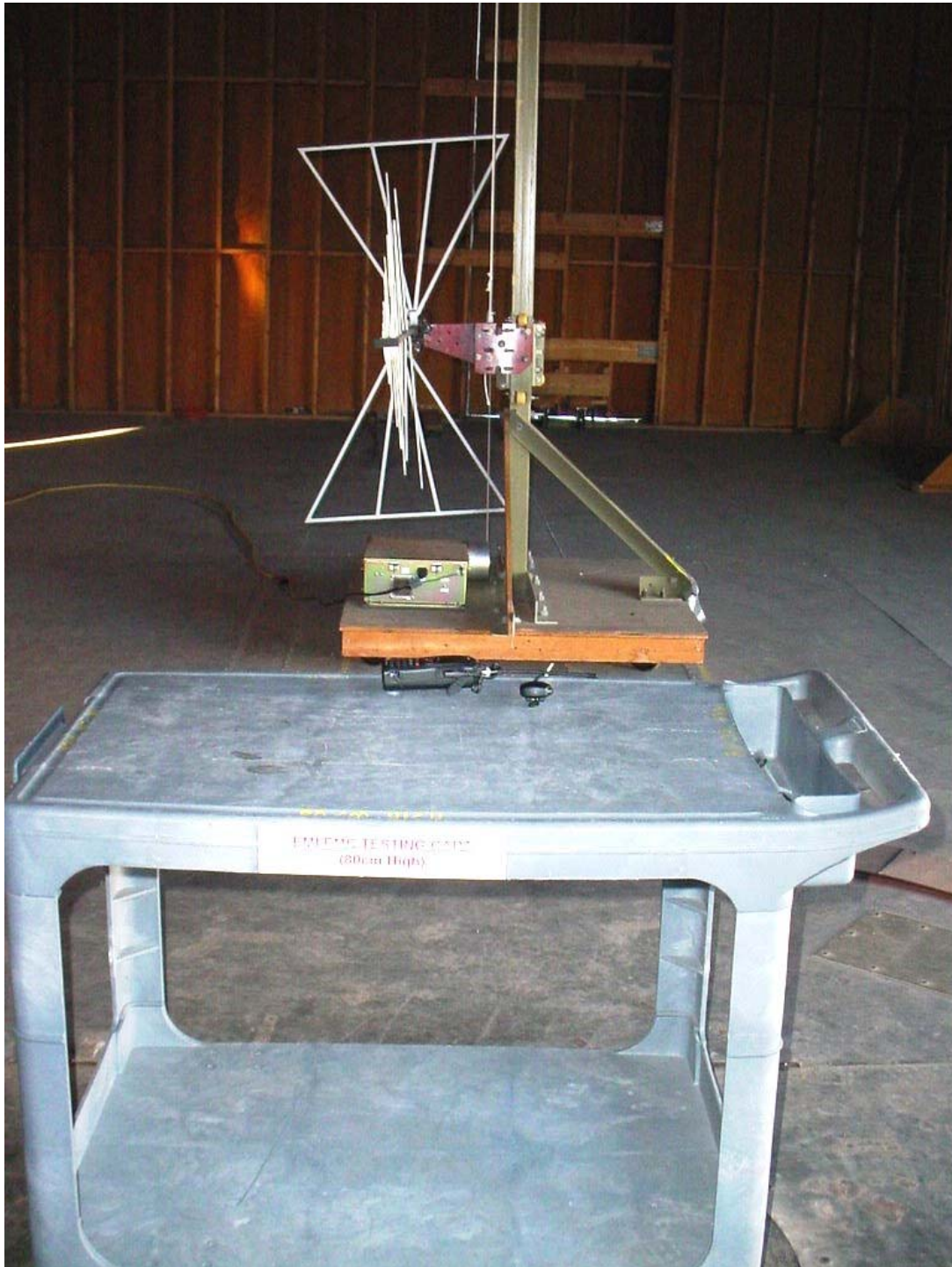
Radiated Emissions at 3 Meters (Orthogonal Position 3)
