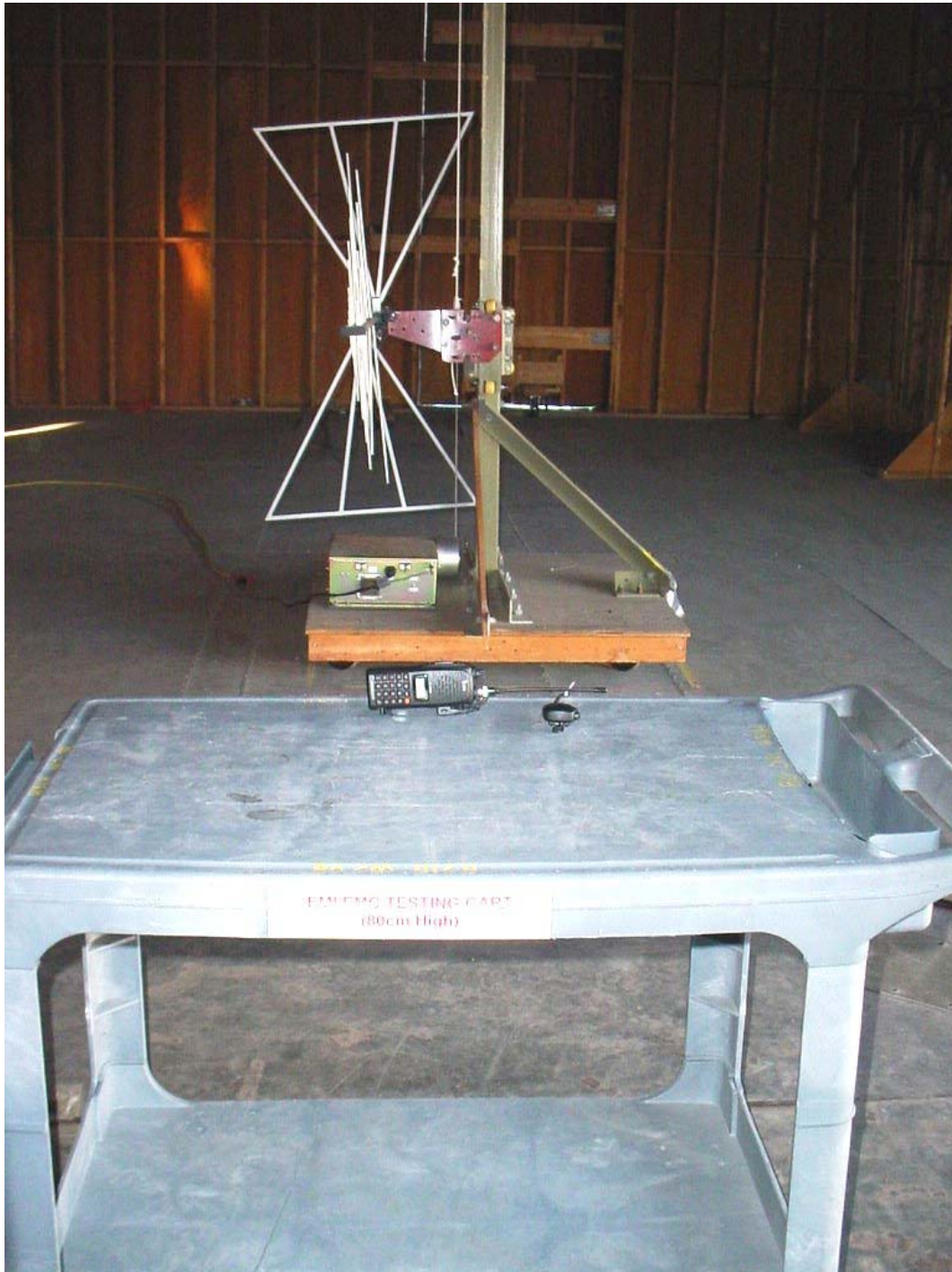
Radiated Emissions at 3 Meters (Orthogonal Position 2)
